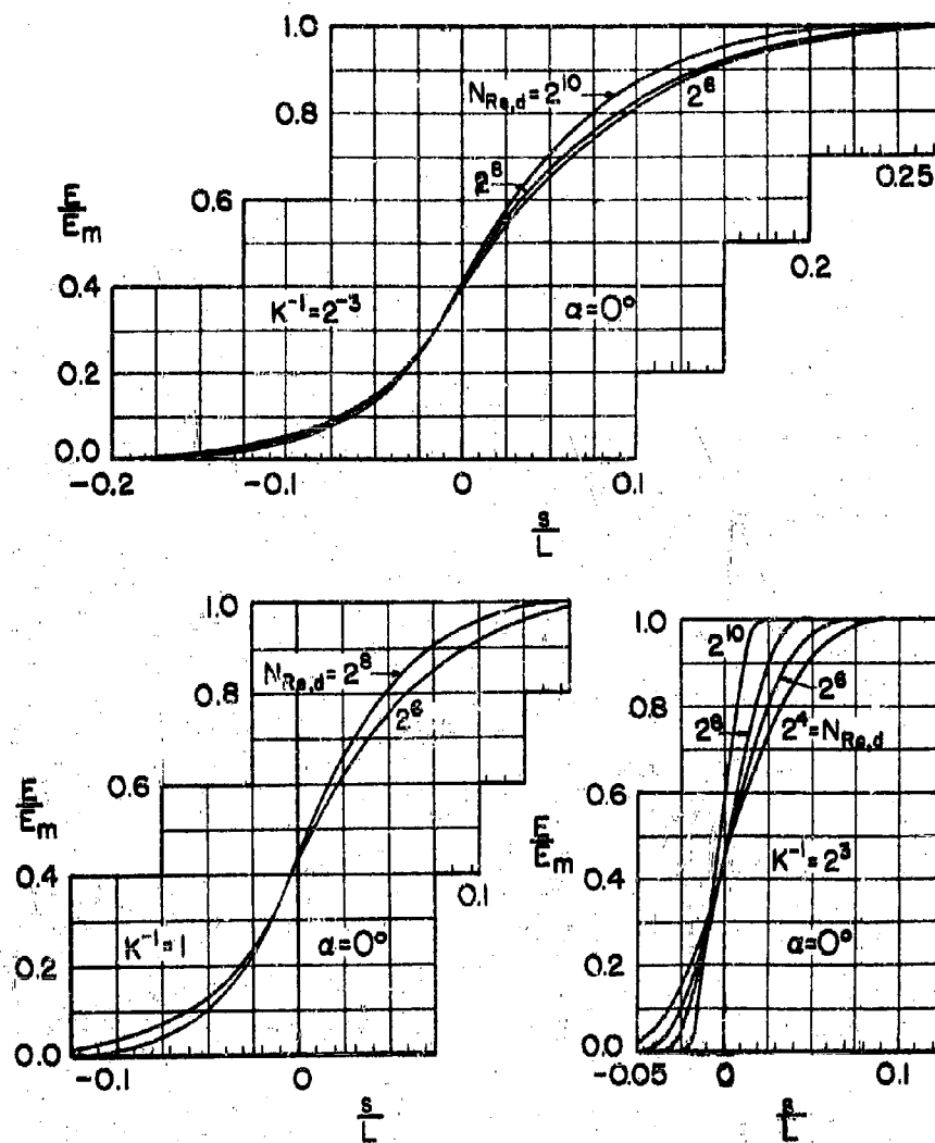
FIG. 3-38 ACCUMULATED COLLECTION EFFICIENCY FOR JOUKOWSKI CAMBERED 15 PER- CENT AIRFOIL AT 0^\circ ANGLE OF ATTACK
