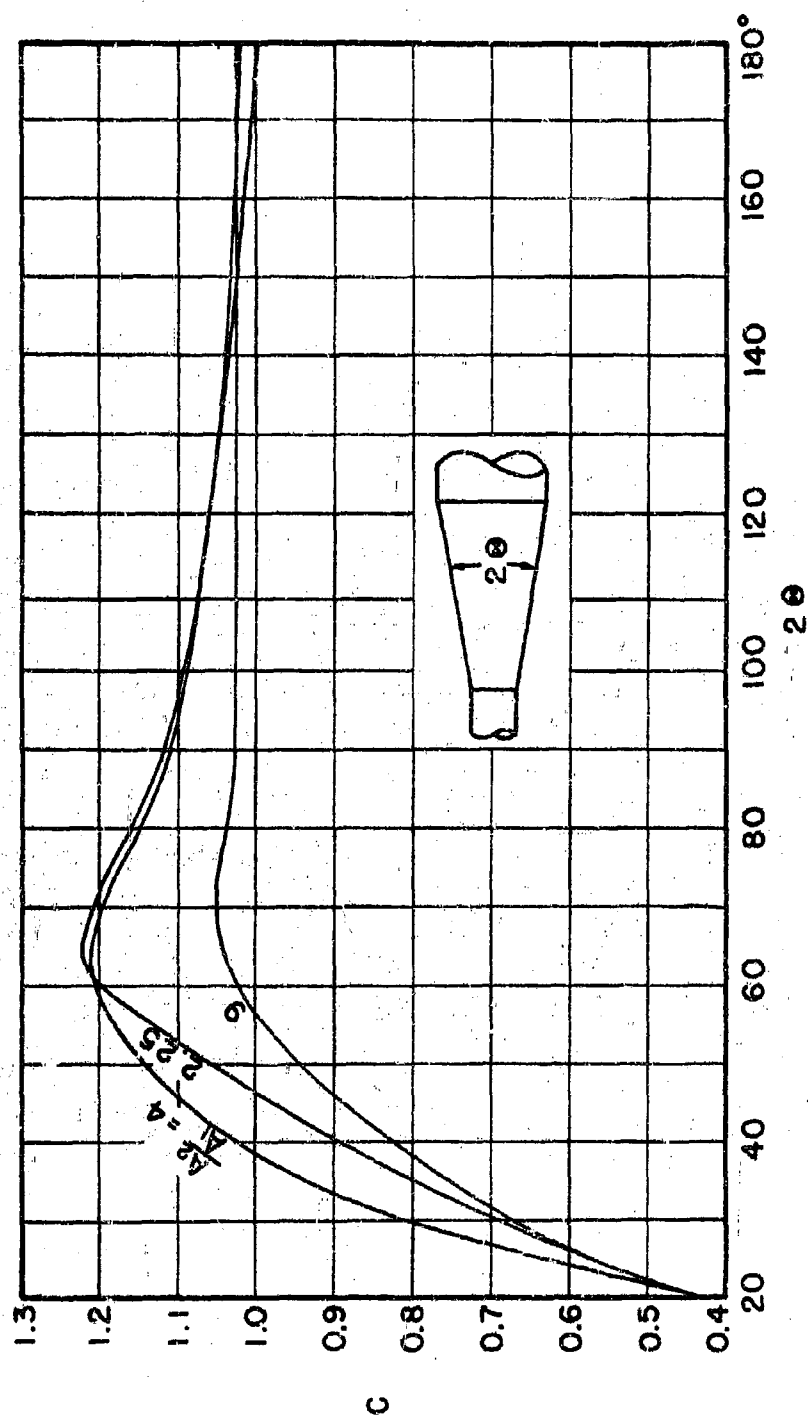
FIG. 2-23 TOTAL-PRESSURE - LOSS-COEFFICIENT FACTOR FOR CIRCULAR DIFFUSERS
