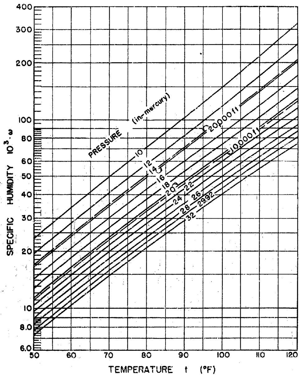
FIG. 5-4 (CONT.) SPECIFIC HUMIDITY OF SATURATED AIR
