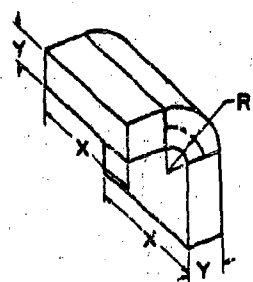
FIG. 2-7 TOTAL-PRESSURE-LOSS COEFFICIENTS FOR RECTANGULAR 90° BENDS
