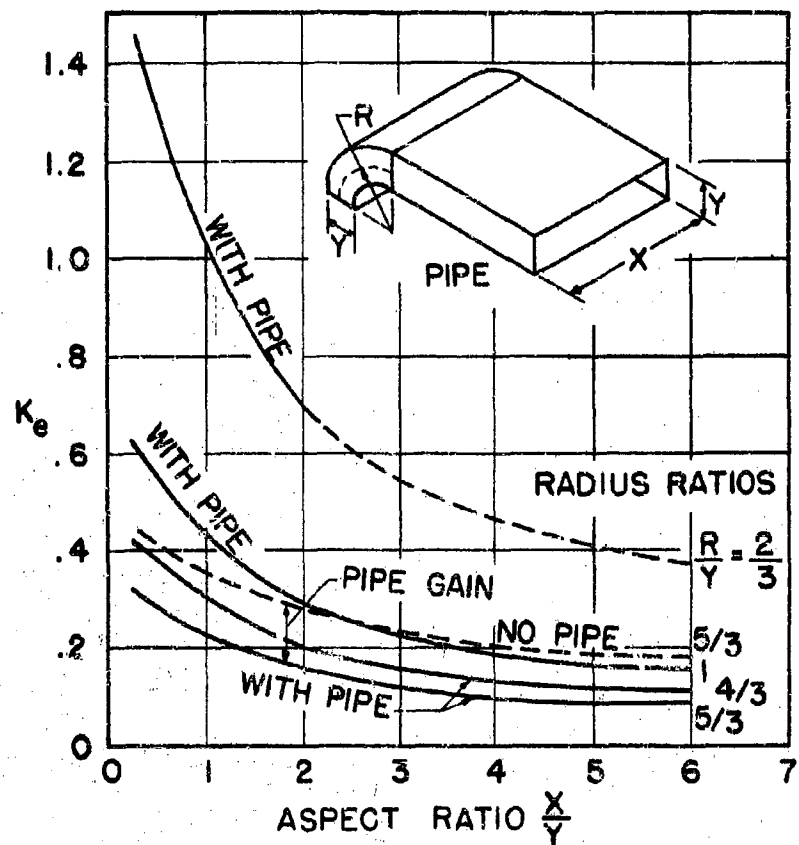
FIG. 2-6 PRESSURE-LOSS COEFFICIENTS OF RECTANGULAR ELBOWS
