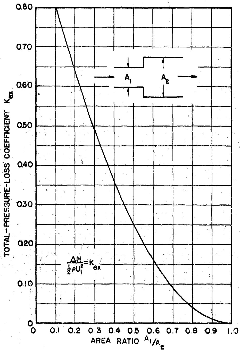
FIG. 2-21 TOTAL-PRESSURE-LOSS COEFFICIENT FOR SUDDEN SHARP-EDGE EXPANSION
