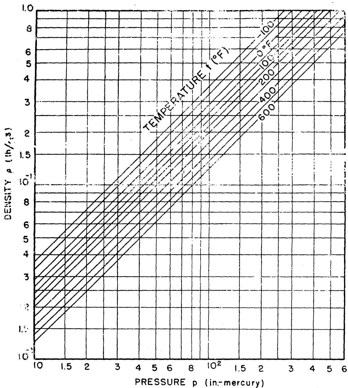
FIG. A- 0 DENSITY OF DRY AIR
