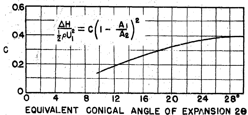
FIG. 2-24 TOTAL-PRESSURE-LOSS-COEFFICIENT FACTOR C FOR CURVED WALL CONICAL DIFFUSER
