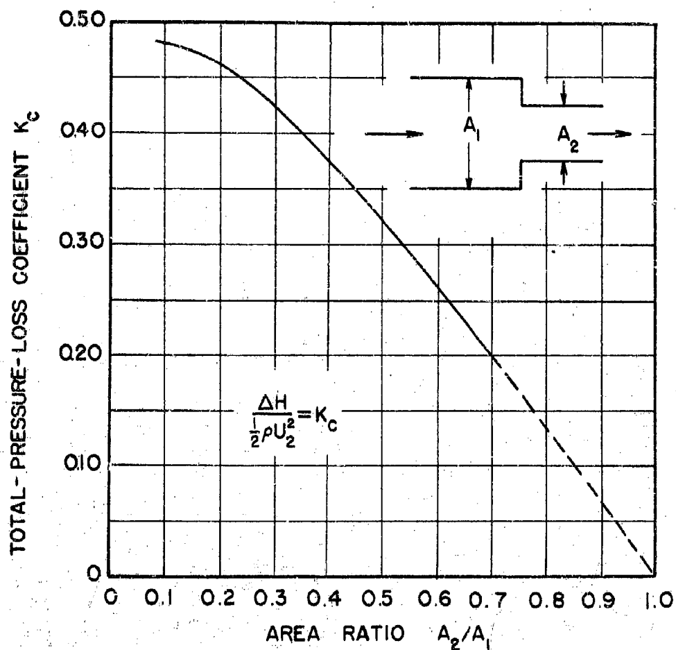
FIG. 2-20 TOTAL-PRESSURE-LOSS COEFFICIENT FOR SUDDEN SHARP-EDGE CONTRACTION
