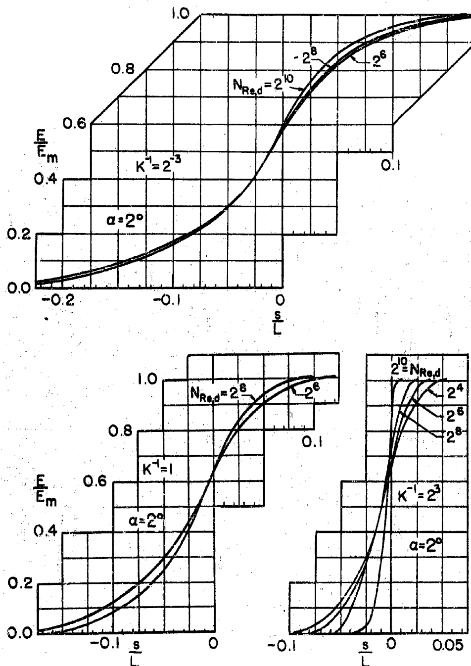
FIG. 3-30 ACCUMULATED COLLECTION EFFICIENCY FOR JOUKOWSKI SYMMETRICAL 15 PER-CENT AIRFOIL AT 2^\circ ANGLE OF ATTACK
