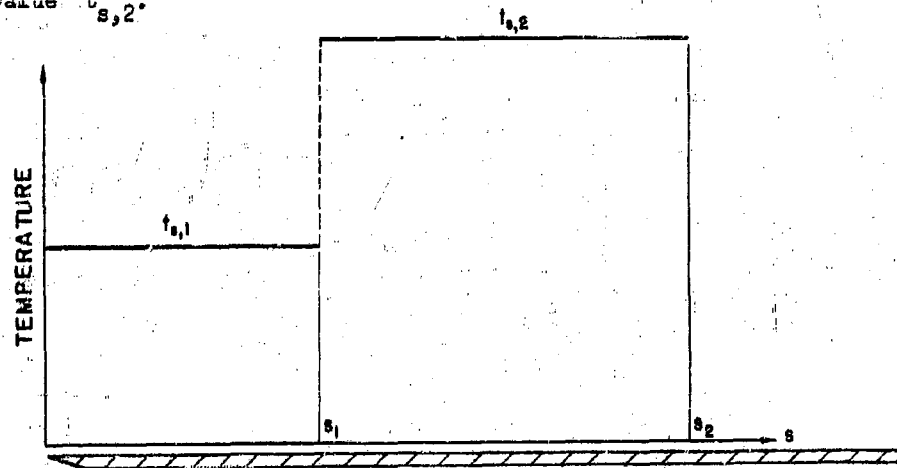
FIG. 4-11 STEPWISE TEMPERATURE DISTRIBUTION ON A FLAT PLATE
