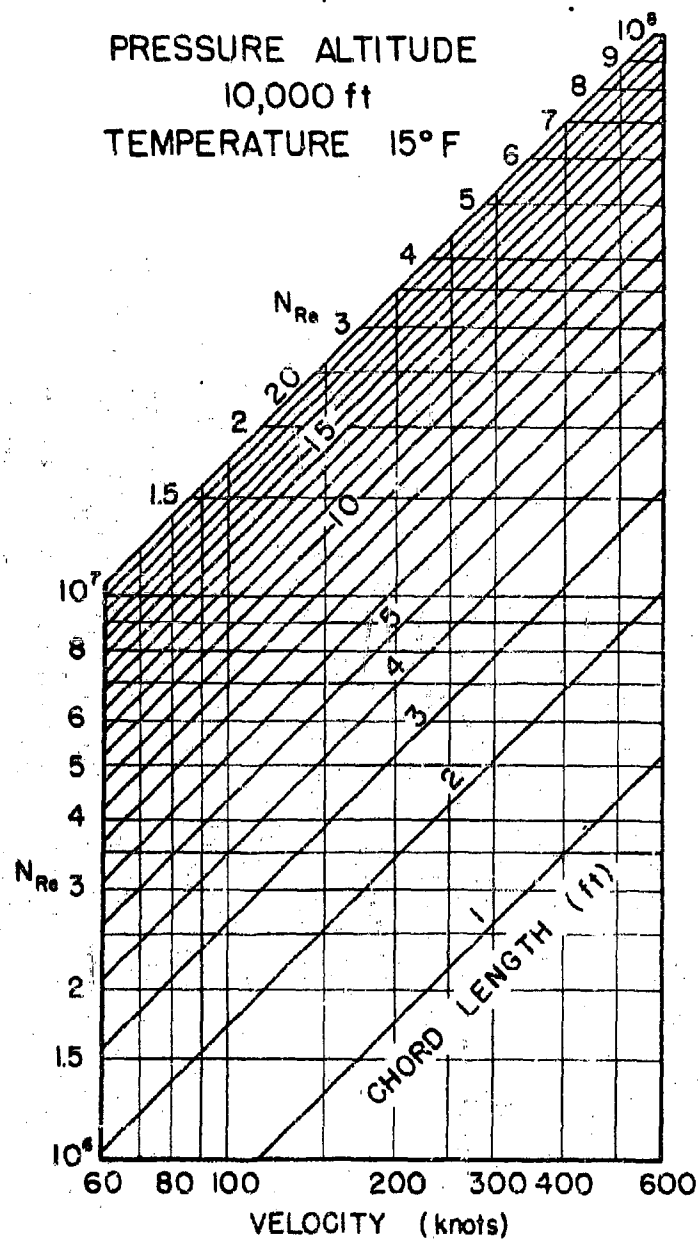
FIG. 4-7 CHART OF REYNOLDS NUMBER FOR 10,000 ft AND 15° F
