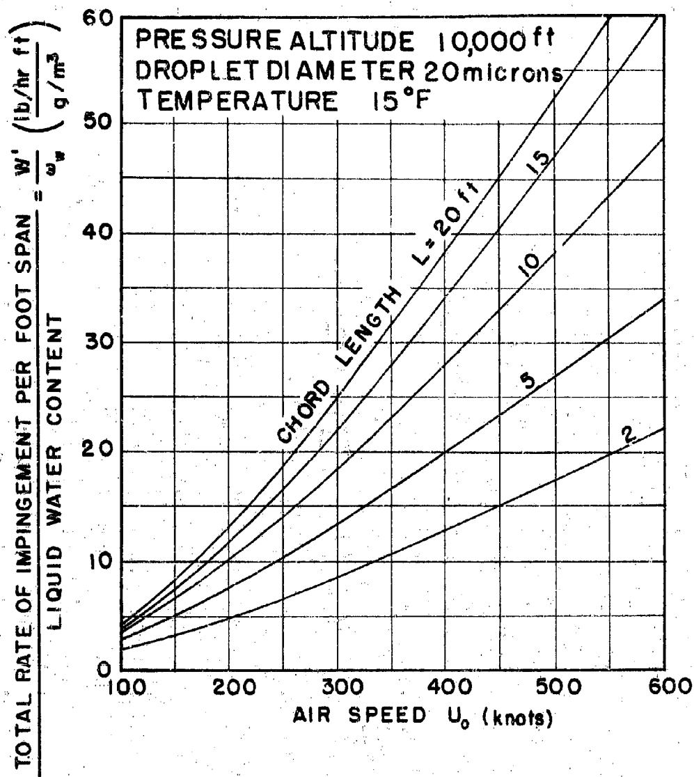
FIG. 3-14 RATE OF WATER IMPINGEMENT ON NACA 65A004 AIRFOIL AT 4° ANGLE OF ATTACK (10,000 ft)
