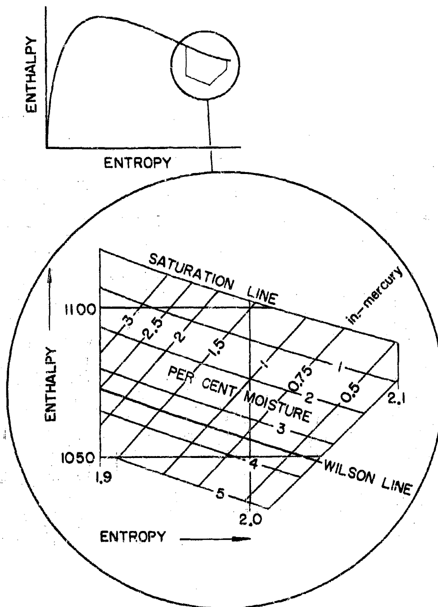
FIG. 5-3 WILSON LINE IN AN ENTHALPY-ENTROPY DIAGRAM OF STEAM
