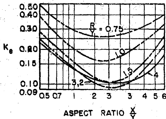
FIG. 2-8 TOTAL-PRESSURE-LOSS COEFFICIENTS FOR ELLIPTICAL 90° BENDS
