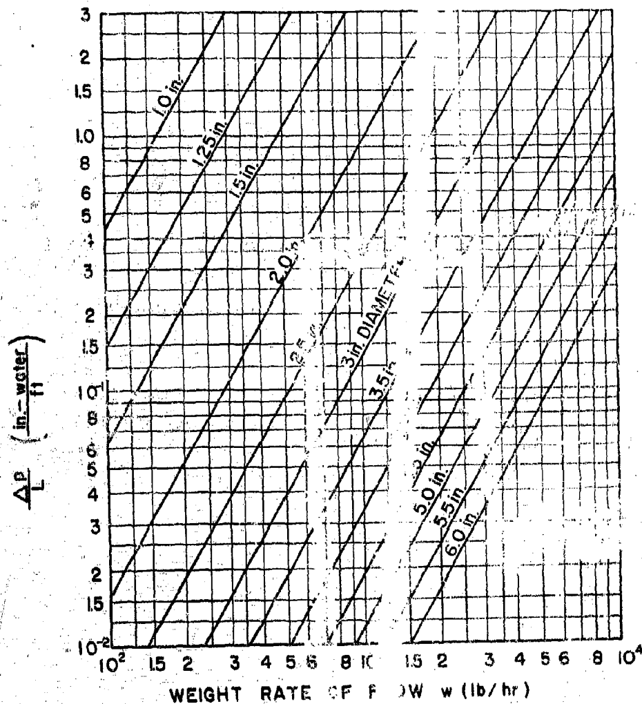
FIG. 2-2 PRESSURE DROP STRAIGHT TUBES FOR AIR AT 300°F AND 29.92 IN.-MERCURY
