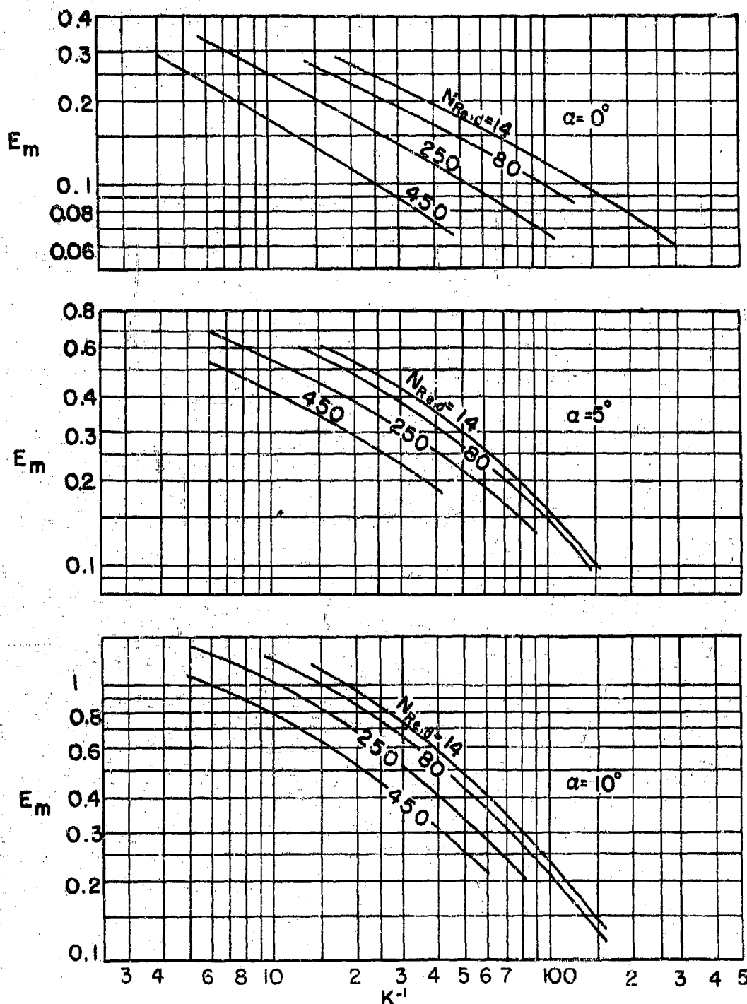
FIG. 3-9 TOTAL COLLECTION EFFICIENCY ON NACA 65A005 AIRFOIL AT VARIOUS ANGLES OF ATTACK
