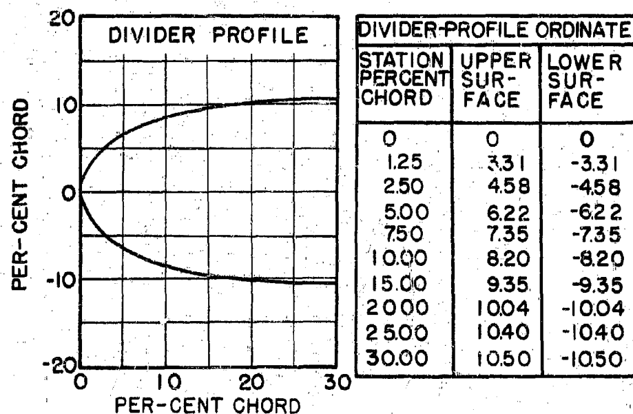
FIG. 2-28 DESIGN OF A BRANCHED DUCT (DIVIDER PROFILE NACA 0021 NOSE SECTION)
