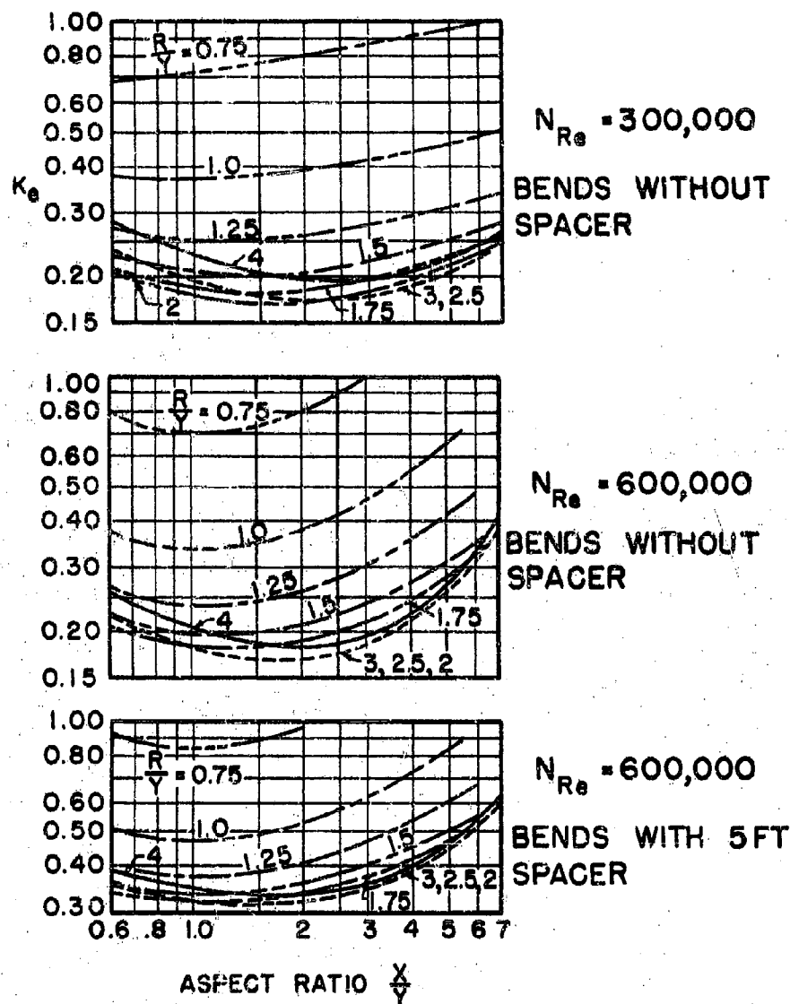
FIG. 2-12 TOTAL-PRESSURE-LOSS COEFFICIENTS FOR COMPOUND RECTANGULAR U, Z, AND 90° OFFSET BENDS
