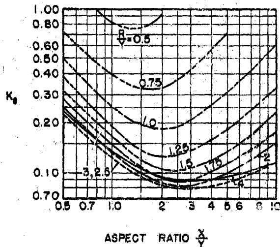
FIG. 2-7 TOTAL-PRESSURE-LOSS COEFFICIENTS FOR RECTANGULAR 90° BENDS
