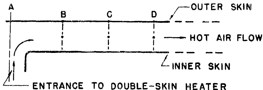
FIG. 6-4 DIVISIONS OF A DOUBLE-SKIN HEAT EXCHANGER
