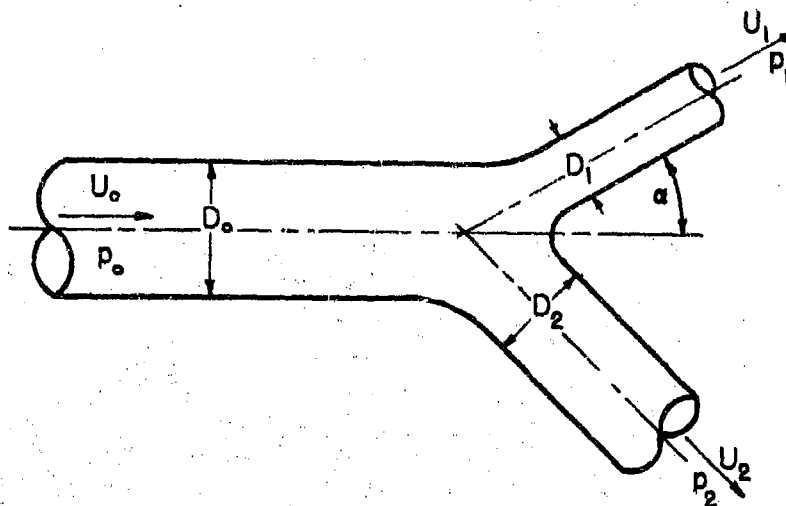
FIG. 2-29 STRAIGHT DUCT BRANCHING INTO TWO DUCTS
