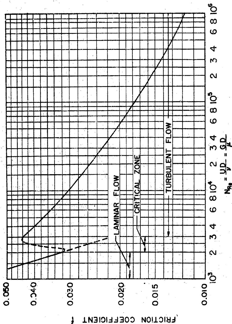
FIG. 2-1 FRICTION COEFFICIENT FOR SMOOTH TUBES
