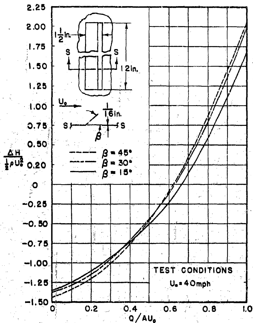
FIG. 2-25 TOTAL-PRESSURE-LOSS COEFFICIENT FOR EXTERNAL FLAP OUTLET IN A FLAT PLATE
