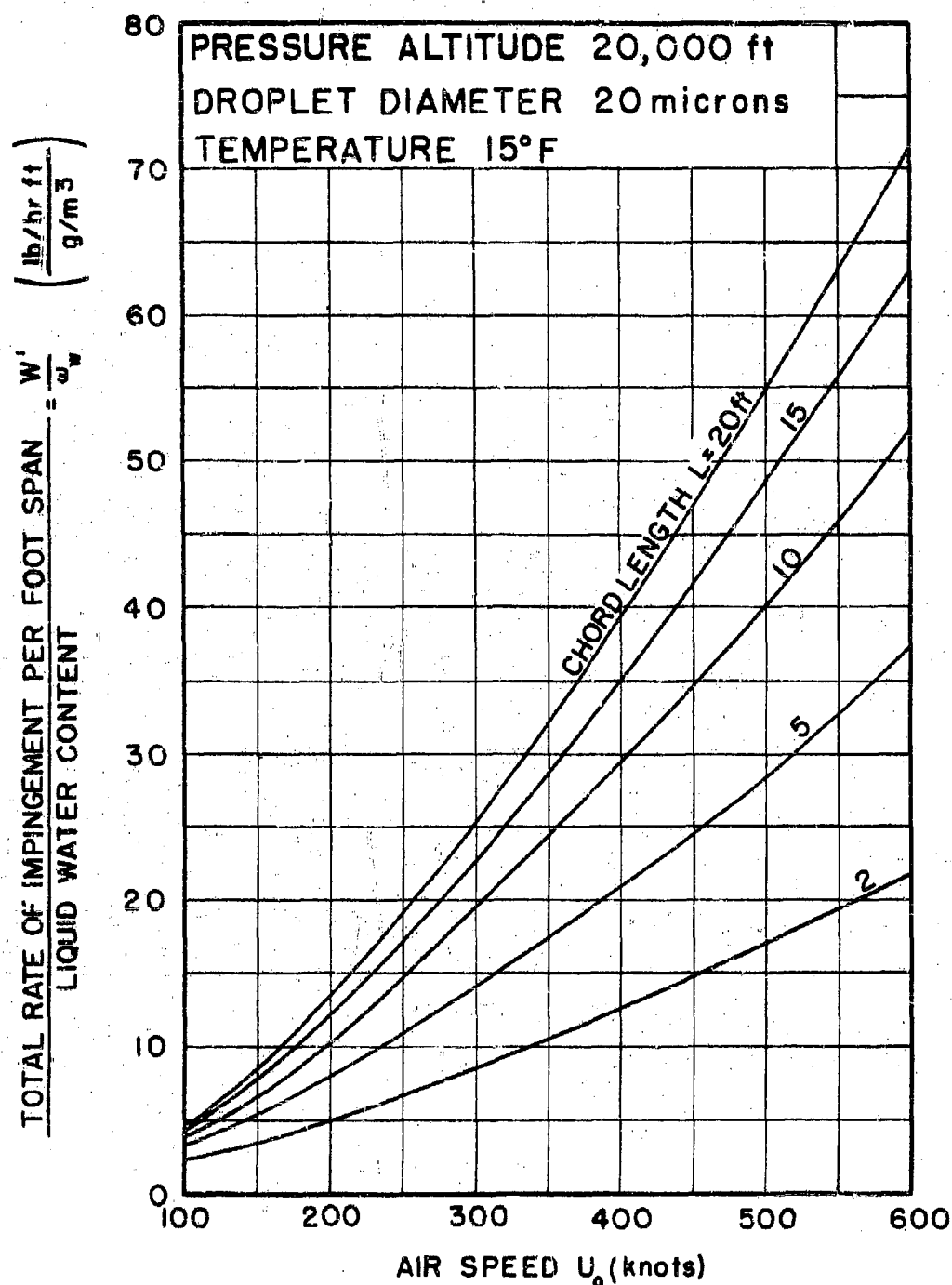
FIG.3-15 RATE OF WATER IMPINGEMENT ON NACA 65A004 AIRFOIL AT 4° ANGLE OF ATTACK (20,000 ft)
