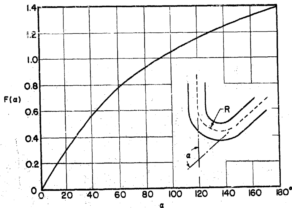
FIG. 2-9 ANGLE FACTOR OF TOTAL-PRESSURE LOSS IN ACUTE AND OBLIQUE ELBOWS
