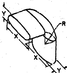
FIG. 2-8 TOTAL-PRESSURE-LOSS COEFFICIENTS FOR ELLIPTICAL 90° BENDS
