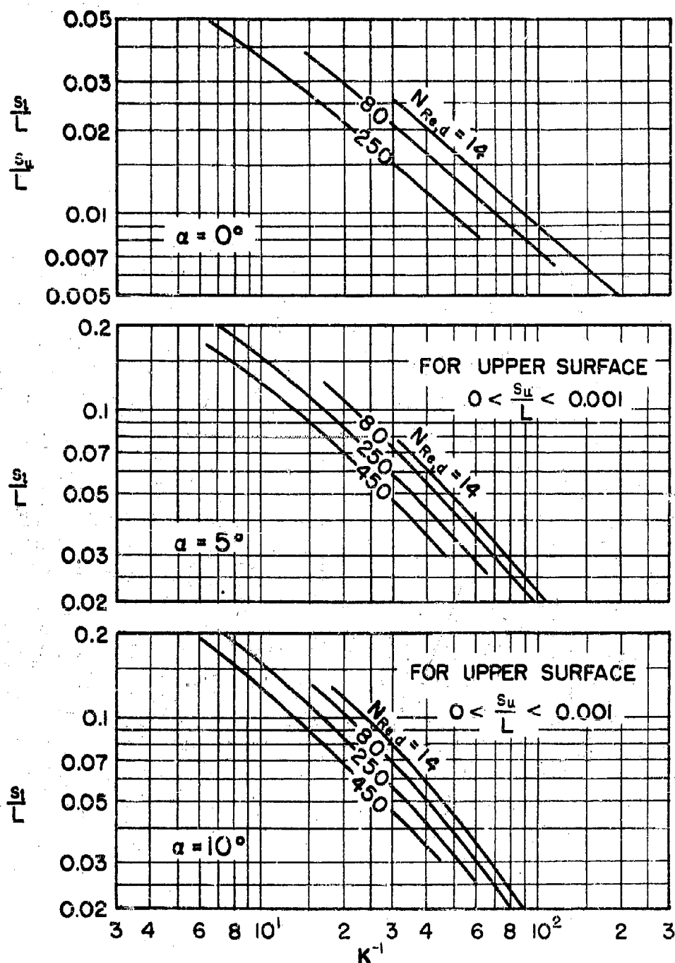
FIG3-27 IMPINGEMENT AREA ON NACA 65A005 AIRFOIL AT VARIOUS ANGLES OF ATTACK
