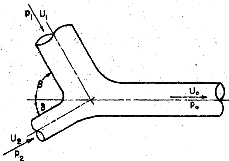
FIG. 2-30 TWO STRAIGHT DUCTS DISCHARGING INTO ONE DUCT
