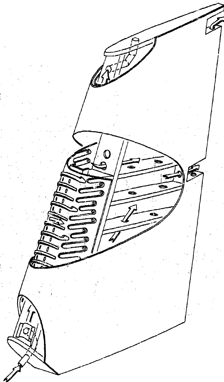
FIG. 1-5 DOUBLE-SKIN HEATER IN THE LEADING EDGE OF A VERTICAL STABILIZER
