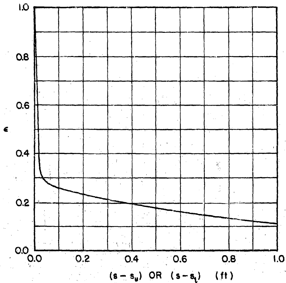
FIG. 5-1 SURFACE-WETNESS FRACTION BEYOND IMPINGEMENT AREA
