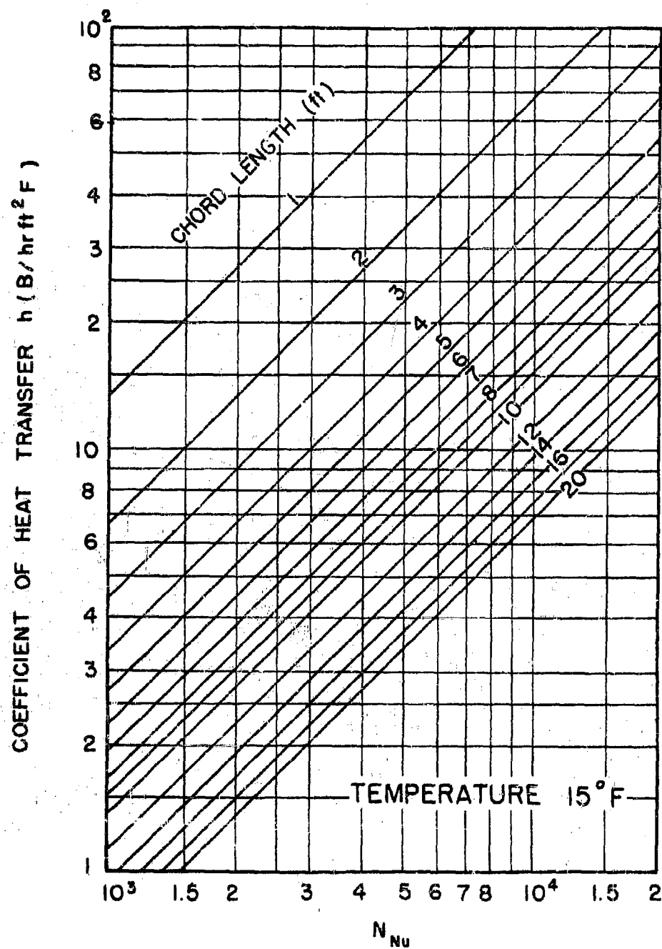
FIG. 4-9 CHART OF NUSSELT NUMBER FOR AIR AT 15°F
