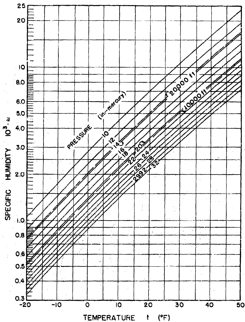
FIG. 5-4 SPECIFIC HUMIDITY OF SATURATED AIR
