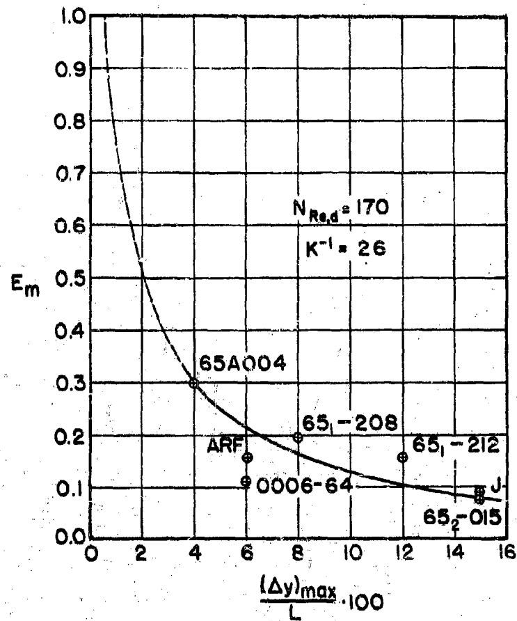
FIG. 3-57 TOTAL COLLECTION EFFICIENCY PLOTTED AGAINST THICKNESS OF AIRFOIL AT 4° ANGLE OF ATTACK
