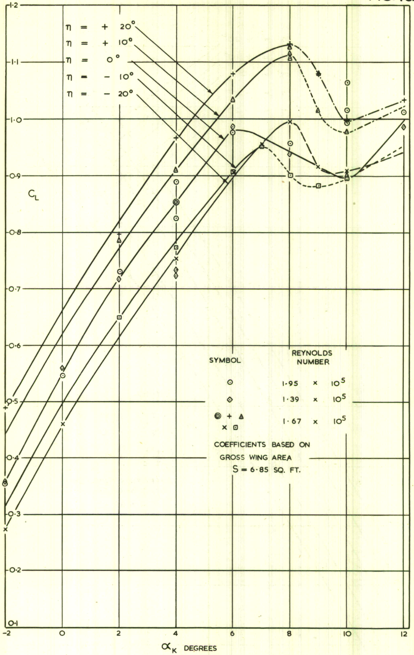
LIFT CURVES WITH FAIRINGS
