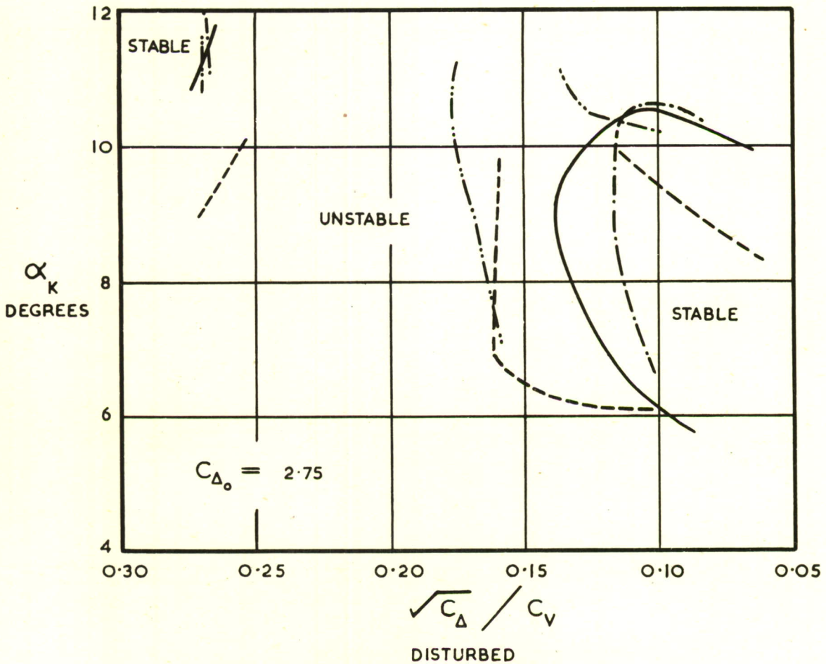
COMPARISON OF LONGITUDINAL STABILITY LIMITS ON A \sqrt{C_D} / C_V BASE. MODEL A
