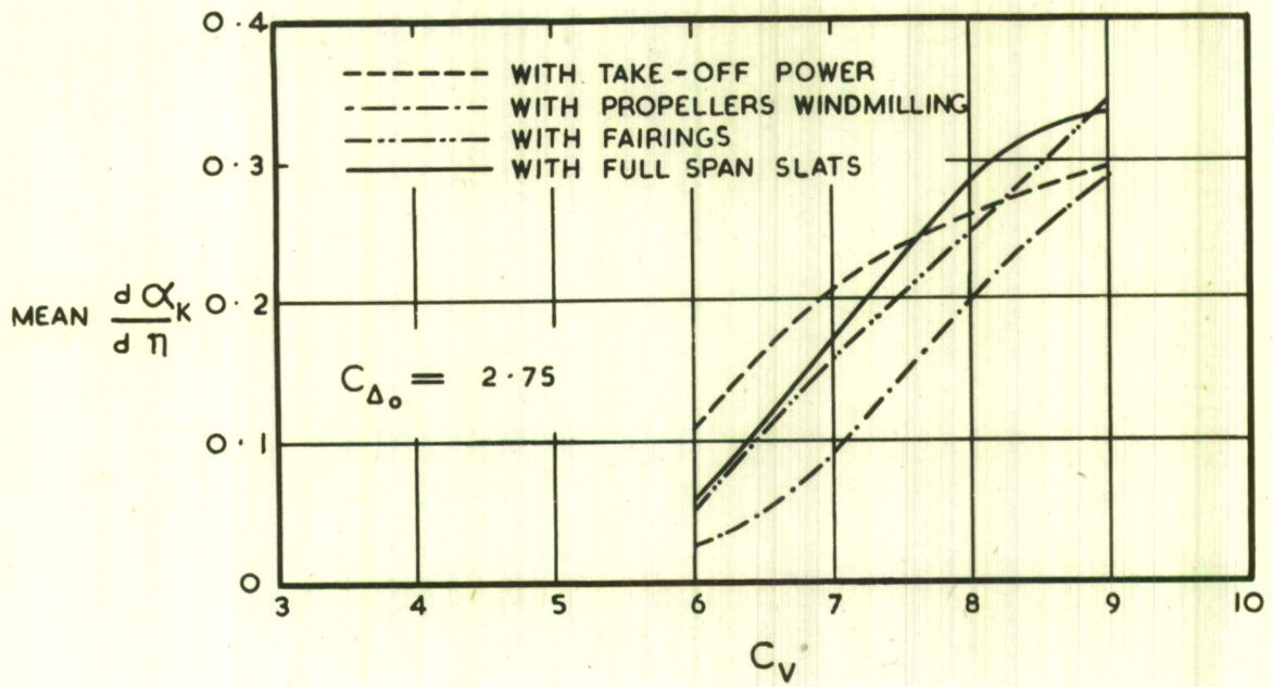
FIG. 15. COMPARISON OF ELEVATOR EFFECTIVENESS
