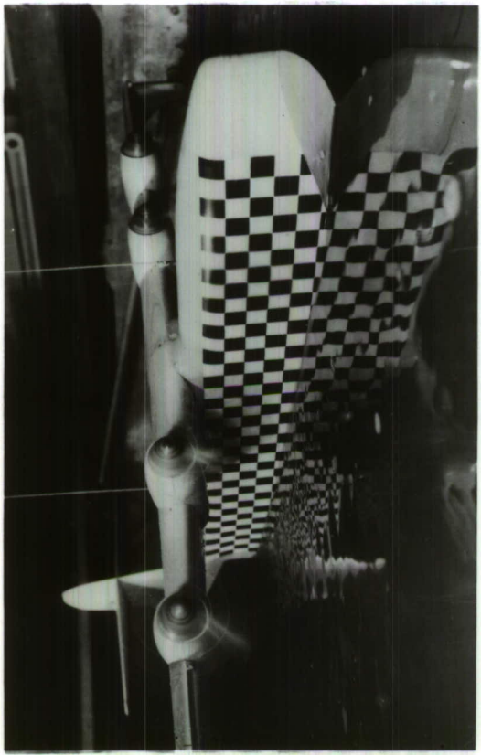
WITH TAKE-OFF POWER
