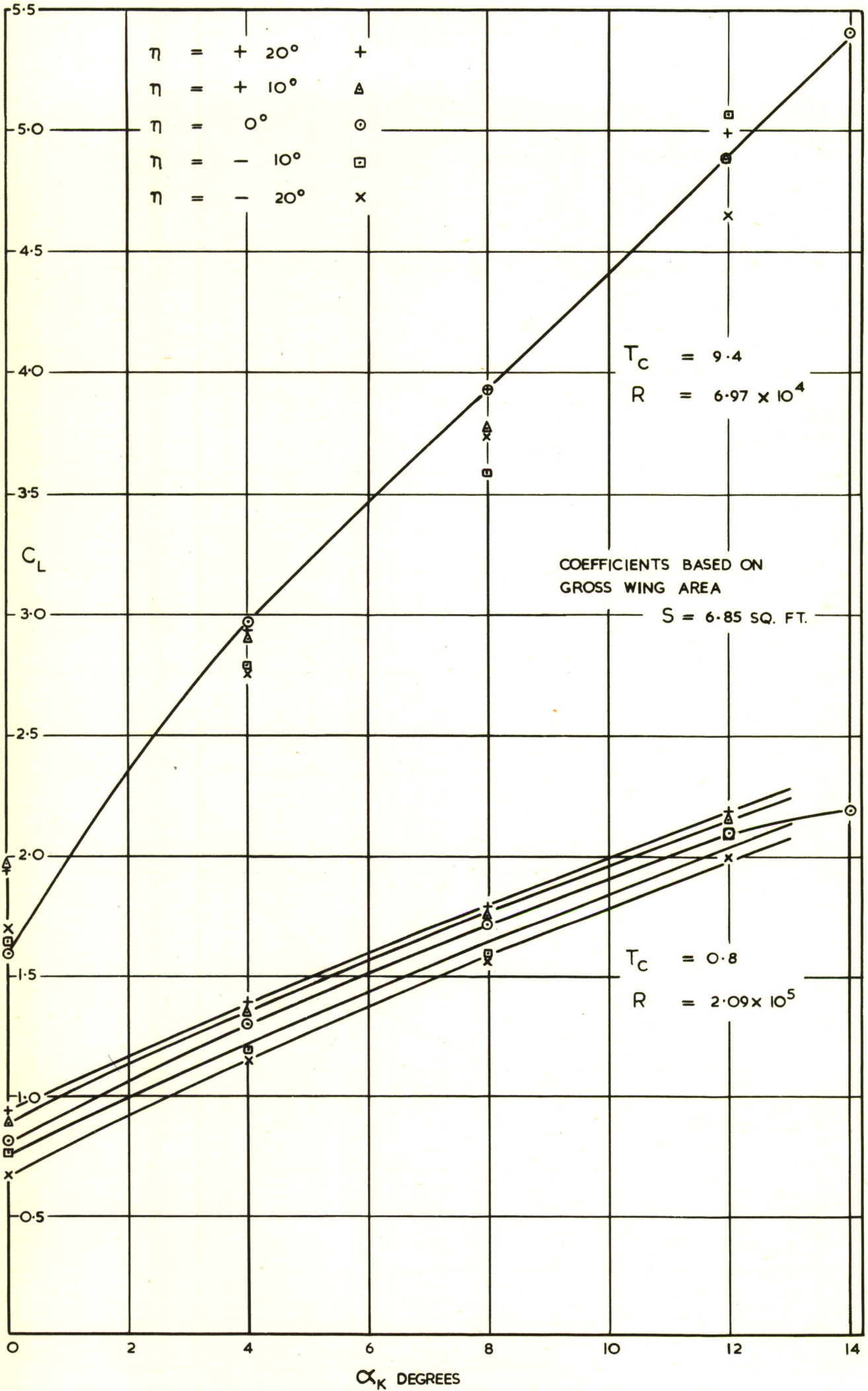
LIFT CURVES WITH TAKE-OFF POWER (I)
