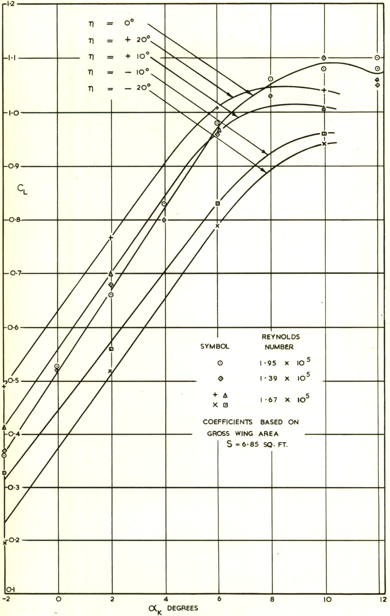
FIG.4b.
