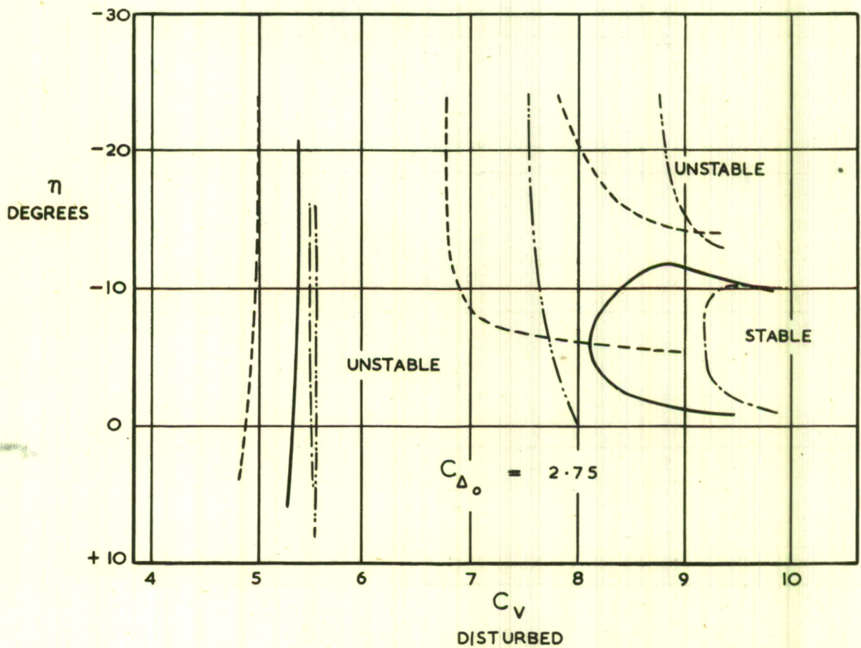
RELATION BETWEEN ELEVATOR SETTING AND STABILITY LIMITS
