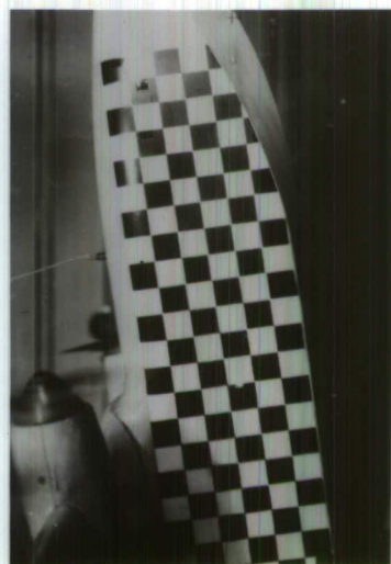
MODEL A SPRAY PHOTOGRAPHS WITH TAKE-OFF POWER (2)
