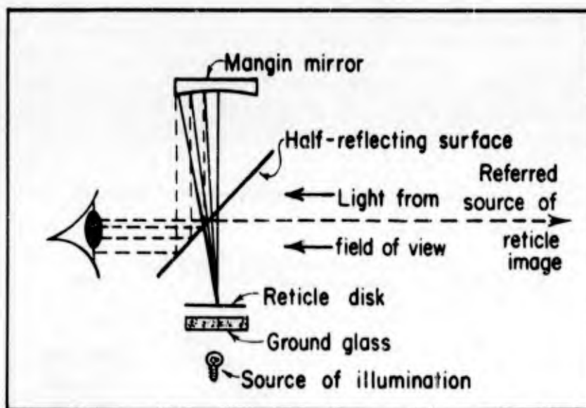
Fig. 2.--Schematic side view of a reflex sight; adapted from (2) and (3).
