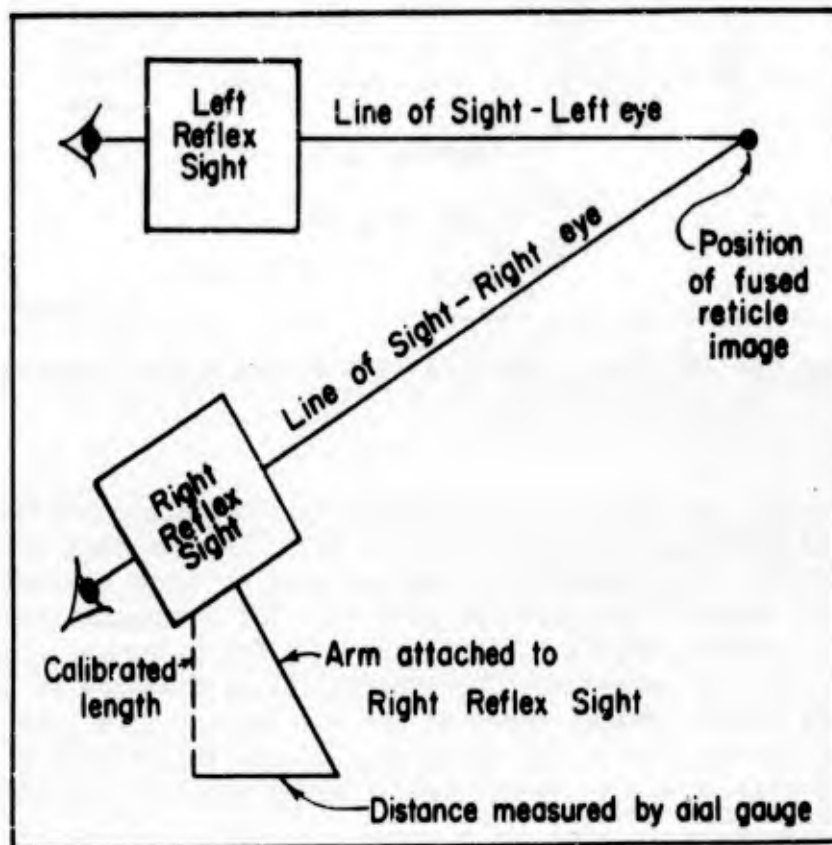
Fig. 1.—Schematic top view of stereoptometer; adapted from (2) and (3).
