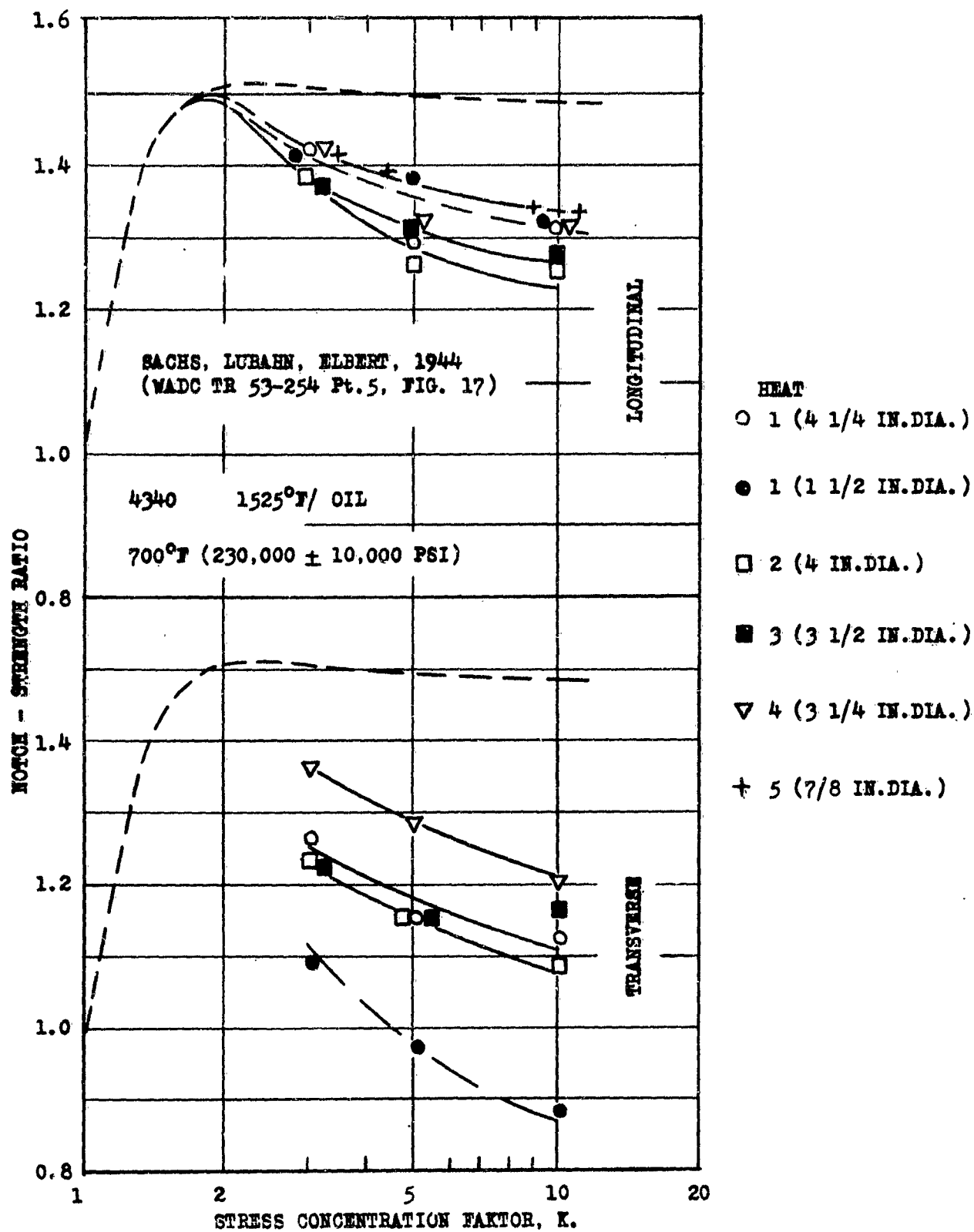
FIG. 17 VARIATION OF NOTCH-STRENGTH RATIO OF VARIOUS 4340 STEEL HEATS WITH STRESS CONCENTRATION FOR 0.3 IN.DIA.SPECIMENS.
