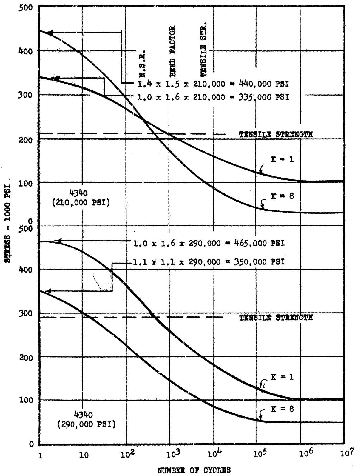
FIG. 43 S-N CURVES FOR SMOOTH AND NOTCHED ROTATING BEAM FATIGUE SPECIMENS FROM 4340 STEEL.
