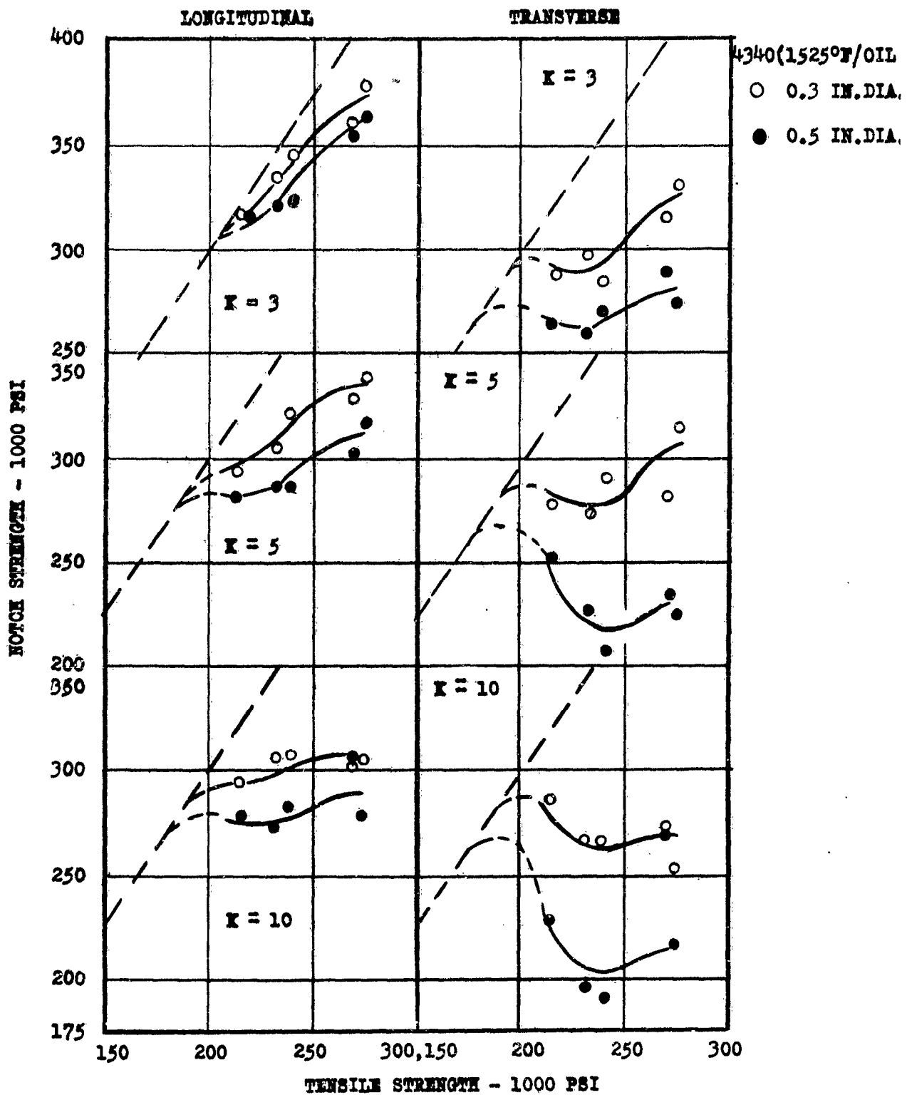
FIG. 19. NOTCH STRENGTH FOR 0.3 AND 0.5 IN. DIA. LONGITUDINAL AND TRANSVERSE SPECIMENS FROM 4340 STEEL (HEAT NO. 1)
