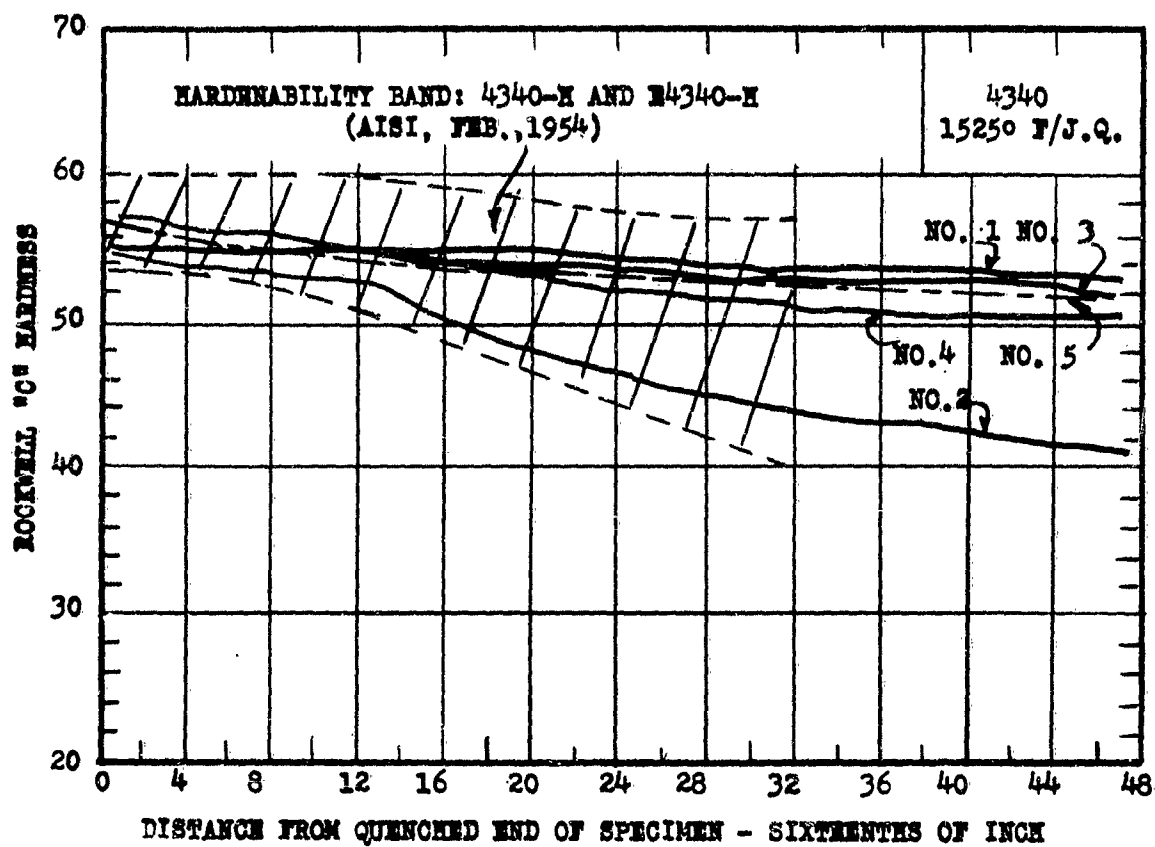
FIG. 12 JOMINY HARDENABILITY OF VARIOUS HEATS OF 4340 STEEL
