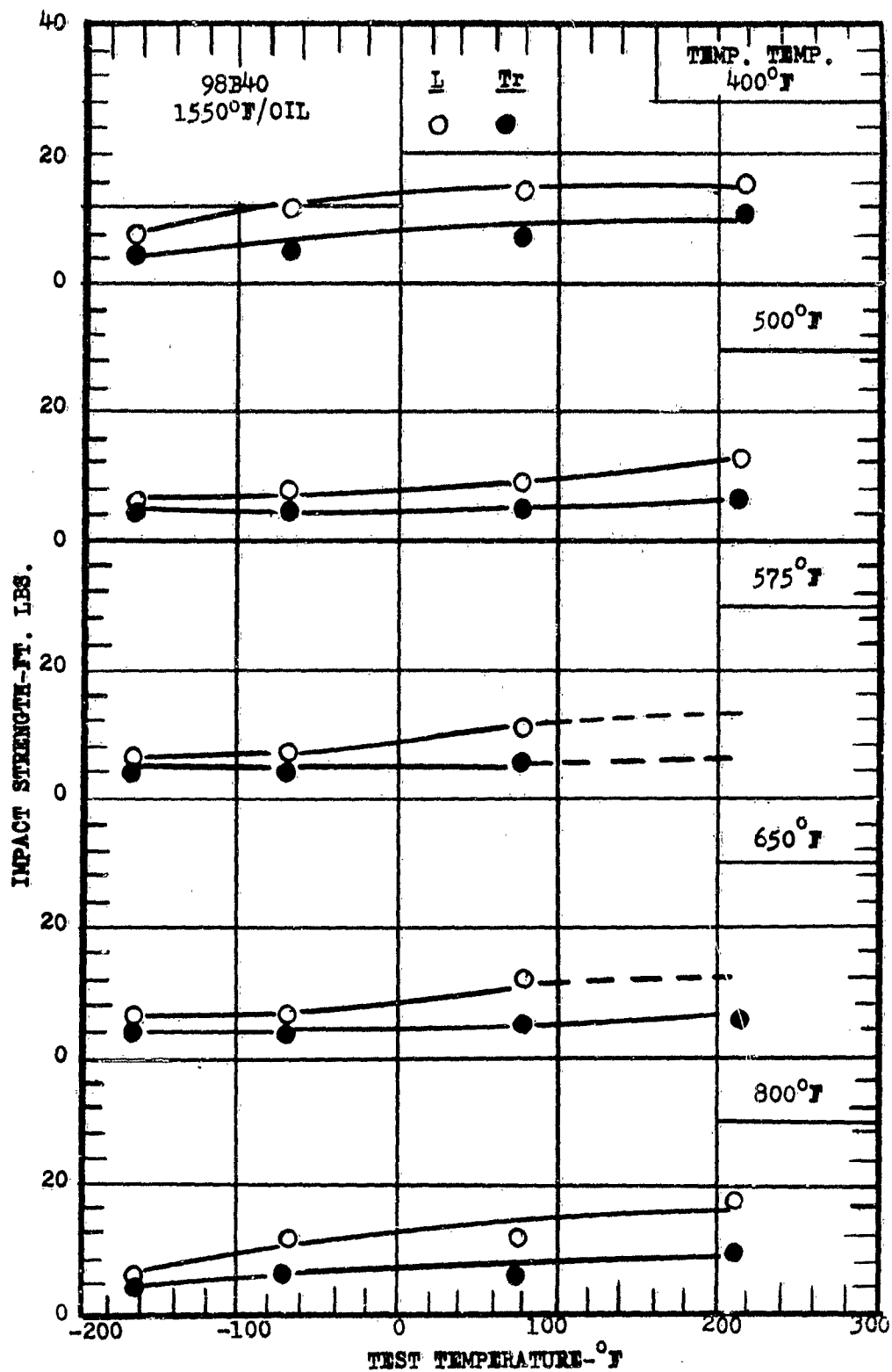
FIG. 35 VARIATION OF IMPACT STRENGTH WITH TEST TEMPERATURE FOR 98B40 STEEL
