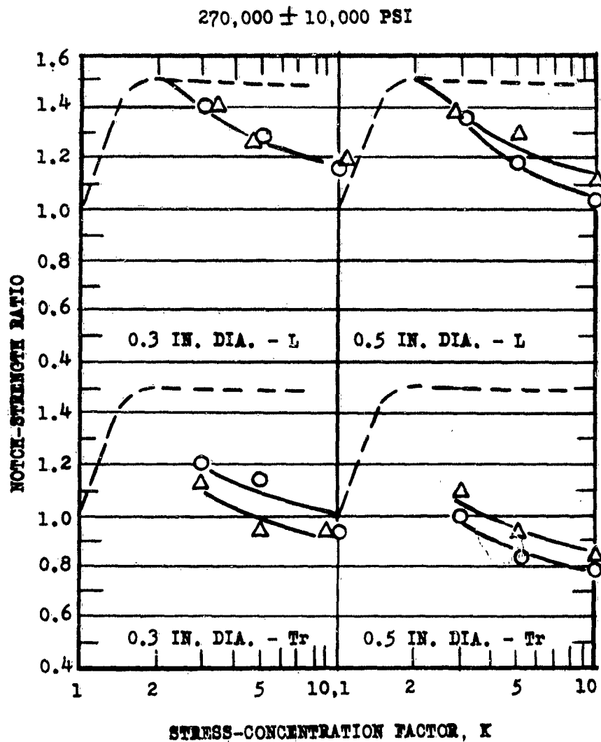
FIG. 69 EFFECT OF STRESS CONCENTRATION ON THE NOTCH-STRENGTH RATIO OF 4340 AND V-MOD. 4330 AT APPROX. 270,000 PSI.
