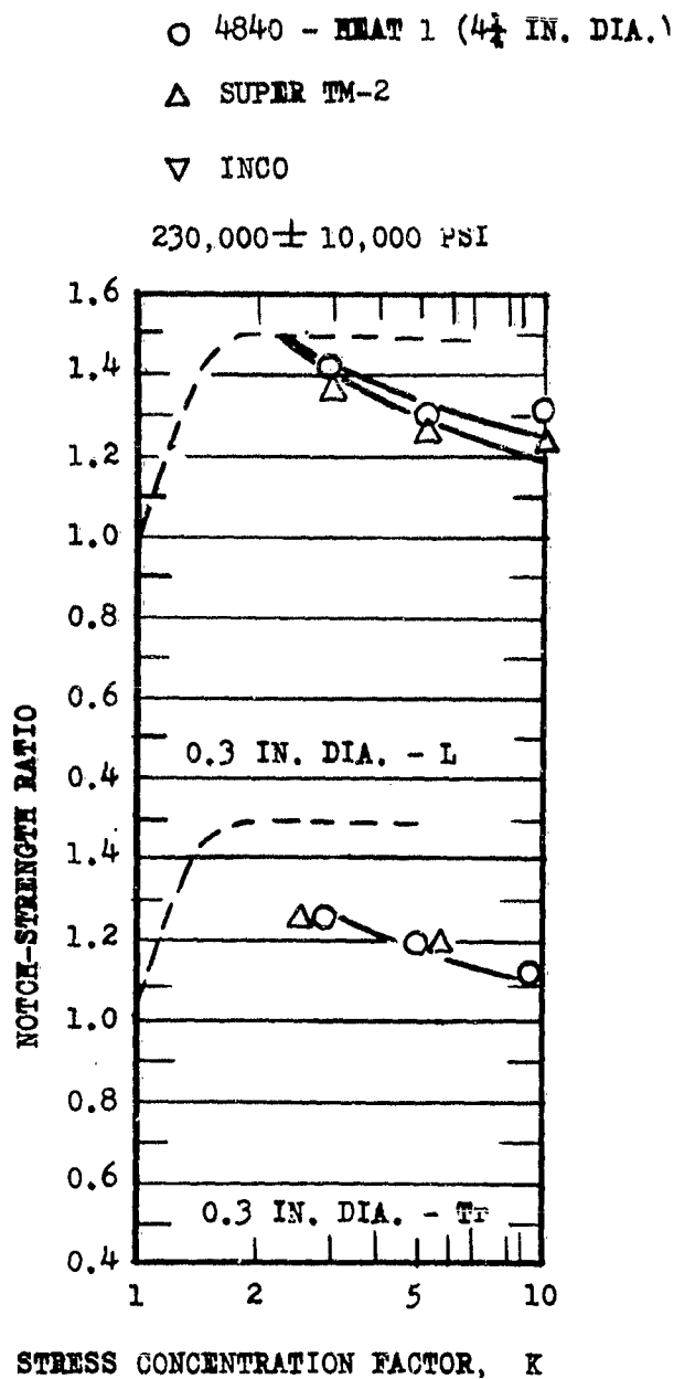
FIG. 62 EFFECT OF STRESS CONCENTRATION ON THE NOTCH-STRENGTH RATIO OF 4340, SUPER TM-2 AND INCO AT APPROX. 230,000 PSI.
