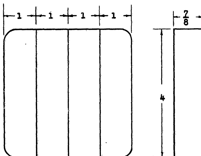
TRANSVERSE 0.5 IN. DIA. NOTCH-TENSILE SPECIMENS
