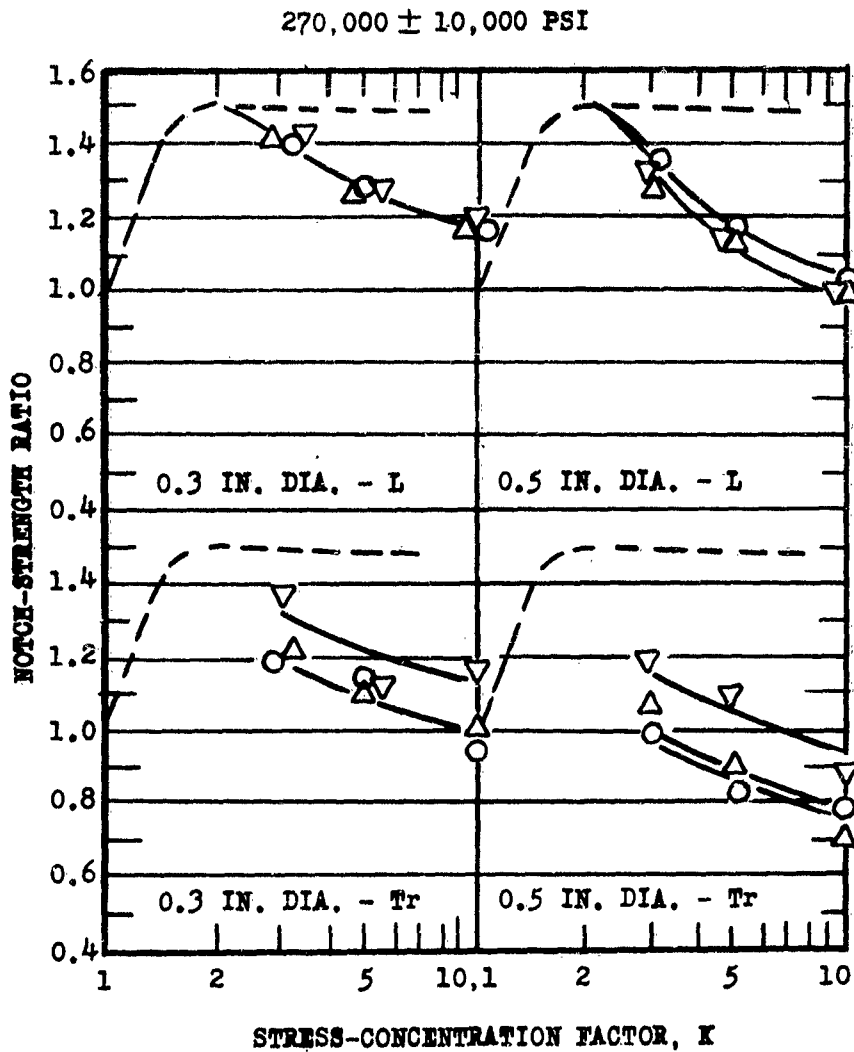
FIG. 68 EFFECT OF STRESS CONCENTRATION ON THE NOTCH-STRENGTH RATIO OF 4340, SUPER TM-2 AND INCO AT APPROX. 270,000 PSI.
