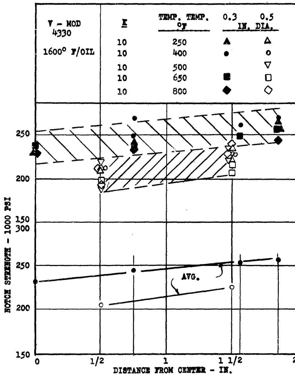
FIG. 7b NOTCH STRENGTH AS A FUNCTION OF DISTANCE FROM CENTER OF V - MOD, 4330 STEEL BAR FOR SHARPLY NOTCHED TRANSVERSE SPECIMENS.
