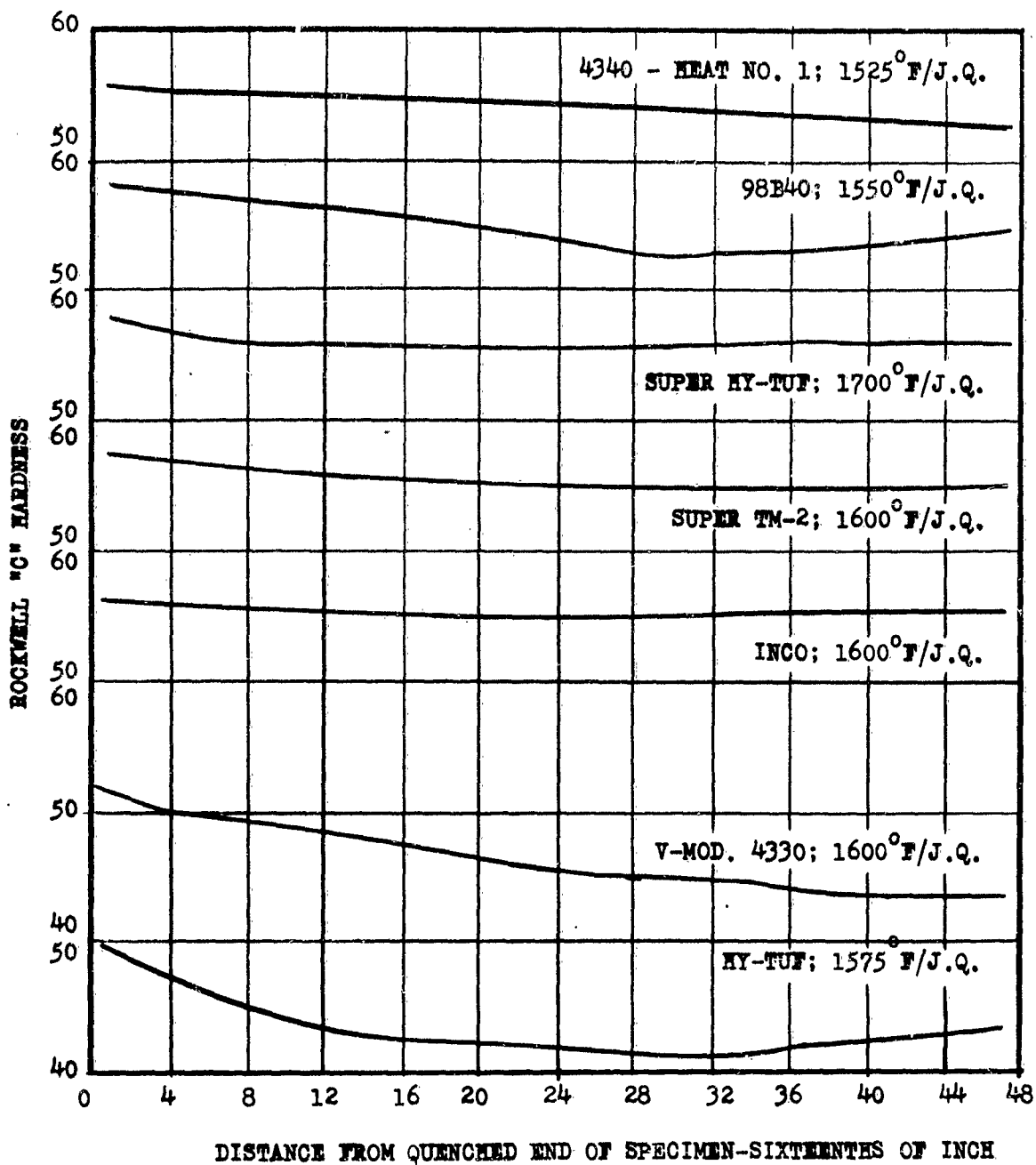
FIG. 52 JOMINY HARDENABILITY OF VARIOUS HIGH-STRENGTH STEELS.
