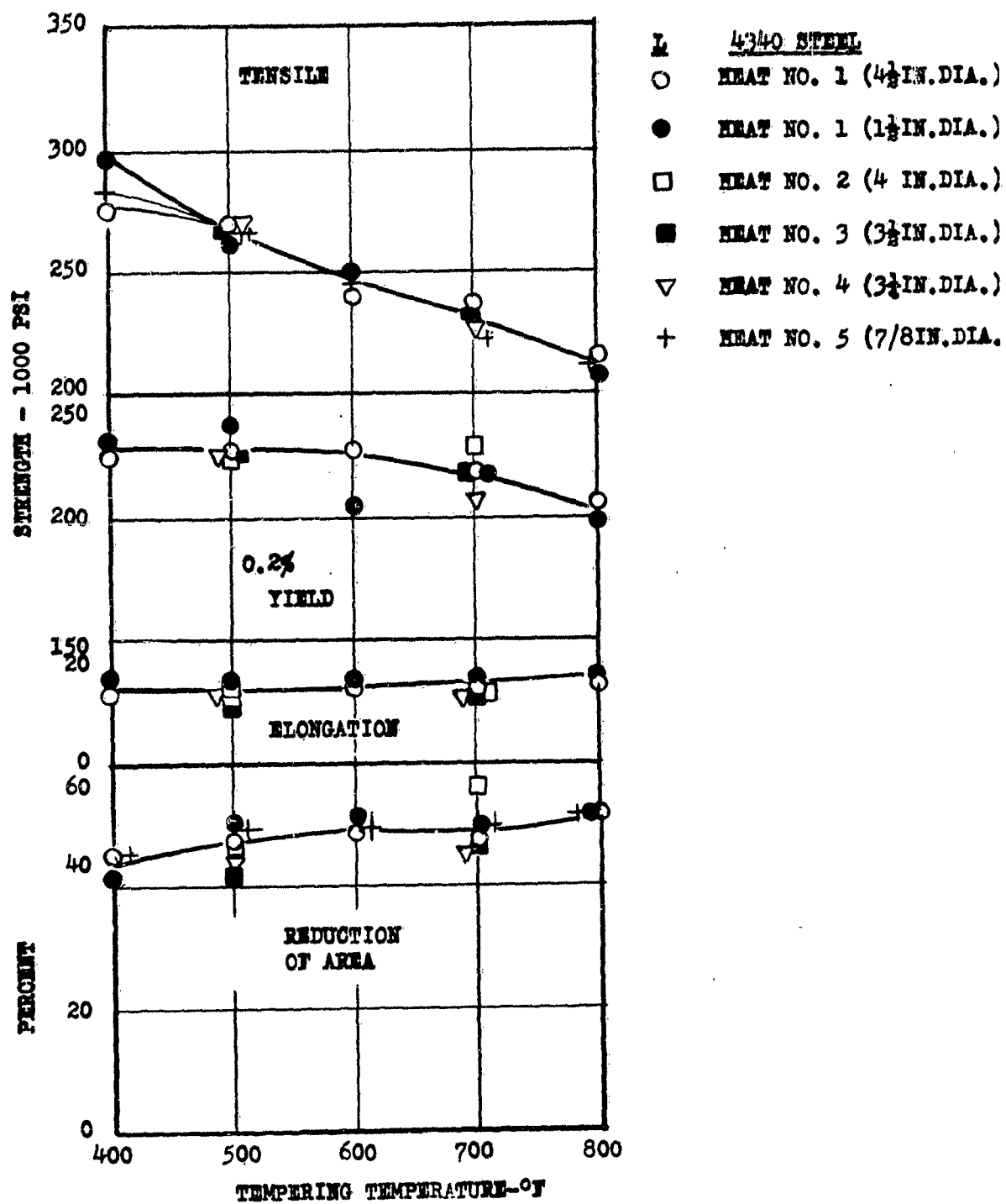
FIG. 13. EFFECT OF TEMPERING ON THE LONGITUDINAL, TENSILE STRENGTH, YIELD STRENGTH, ELONGATION, AND REDUCTION OF AREA OF 4340 STEEL.
