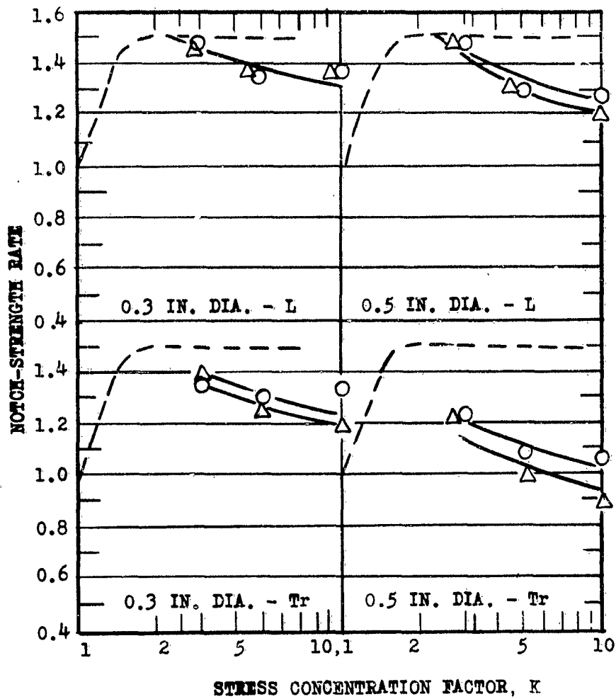
FIG. 59 EFFECT OF STRESS CONCENTRATION ON THE NOTCH STRENGTH RATIO OF 4340 AND 98B40 AT APPROX. 210,000 PSI.
