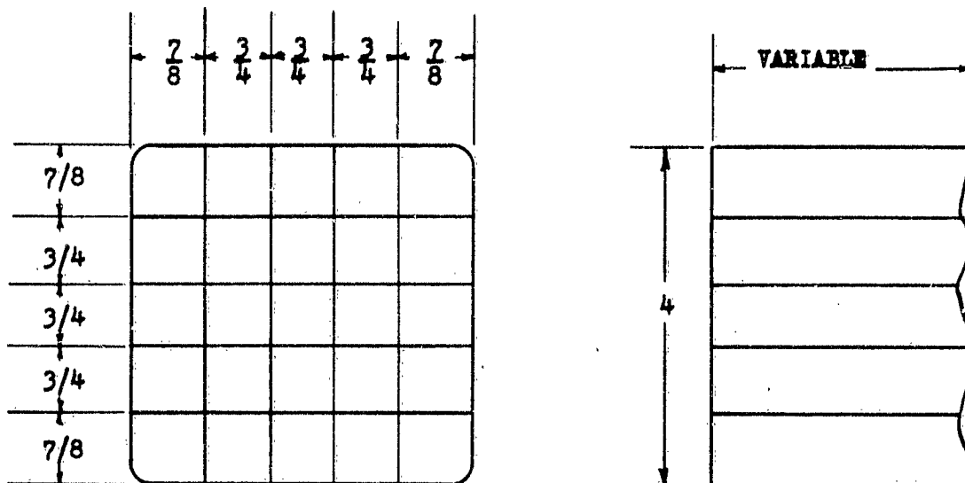
LONGITUDINAL SPECIMENS (0.3 IN. DIA. TENSILE AND NOTCH-TENSILE, IMPACT, AND FATIGUE)
