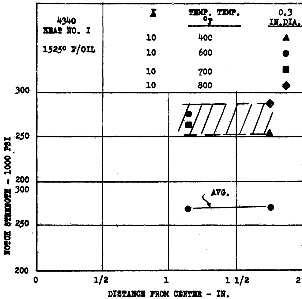
FIG. 9 NOTCH STRENGTH AS A FUNCTION OF DISTANCE FROM CENTER OF 4340 STEEL BAR (HEAT NO. 1) FOR SHARPLY NOTCHED TRANSVERSE SPECIMENS.
