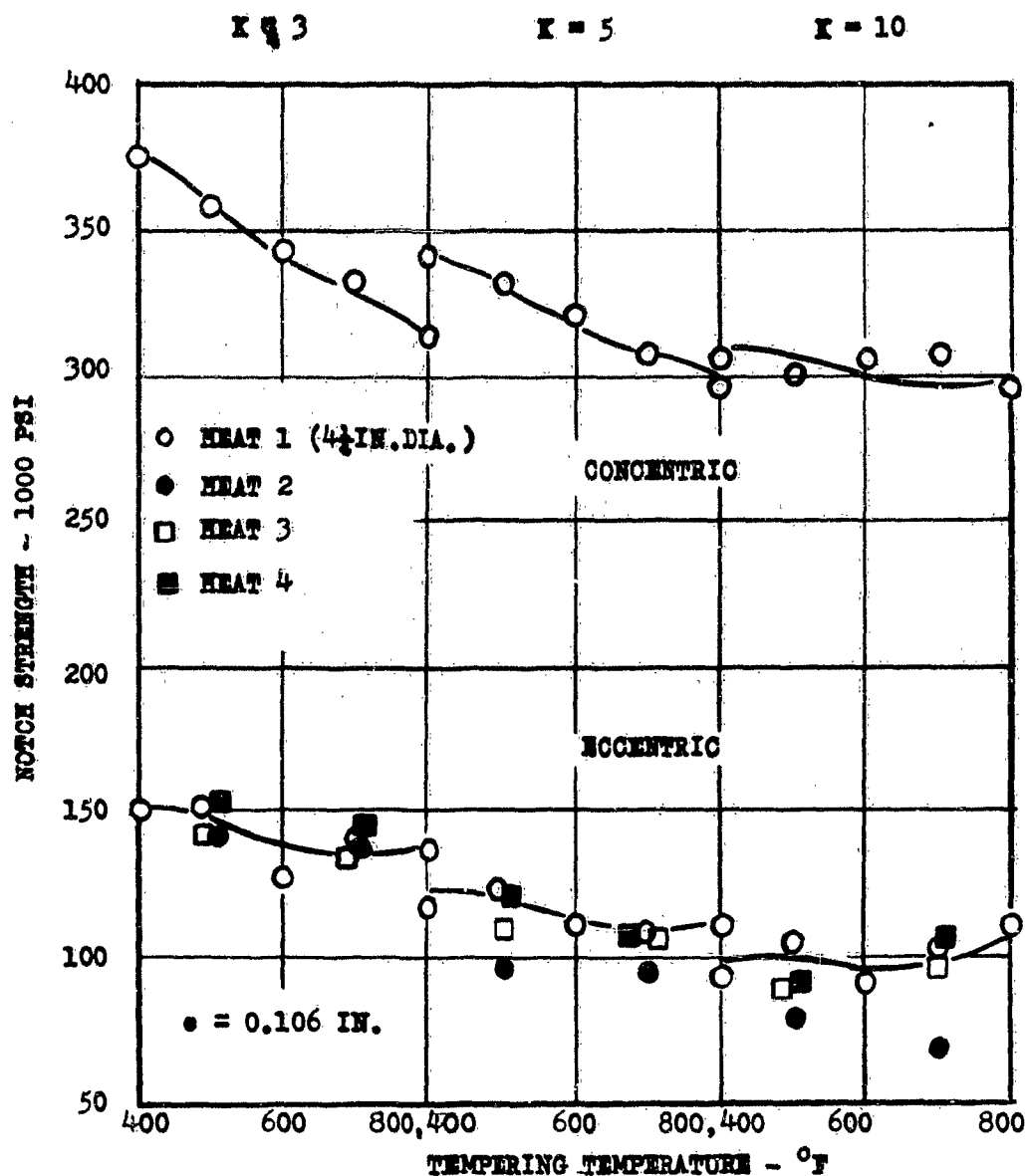
FIG. 25 CONCENTRIC AND ECCENTRIC NOTCH-STRENGTH OF FOUR HEATS OF 4340 STEEL AS A FUNCTION OF TEMPERING TEMPERATURE FOR 0.3 IN. DIA. LONGITUDINAL SPECIMENS.
