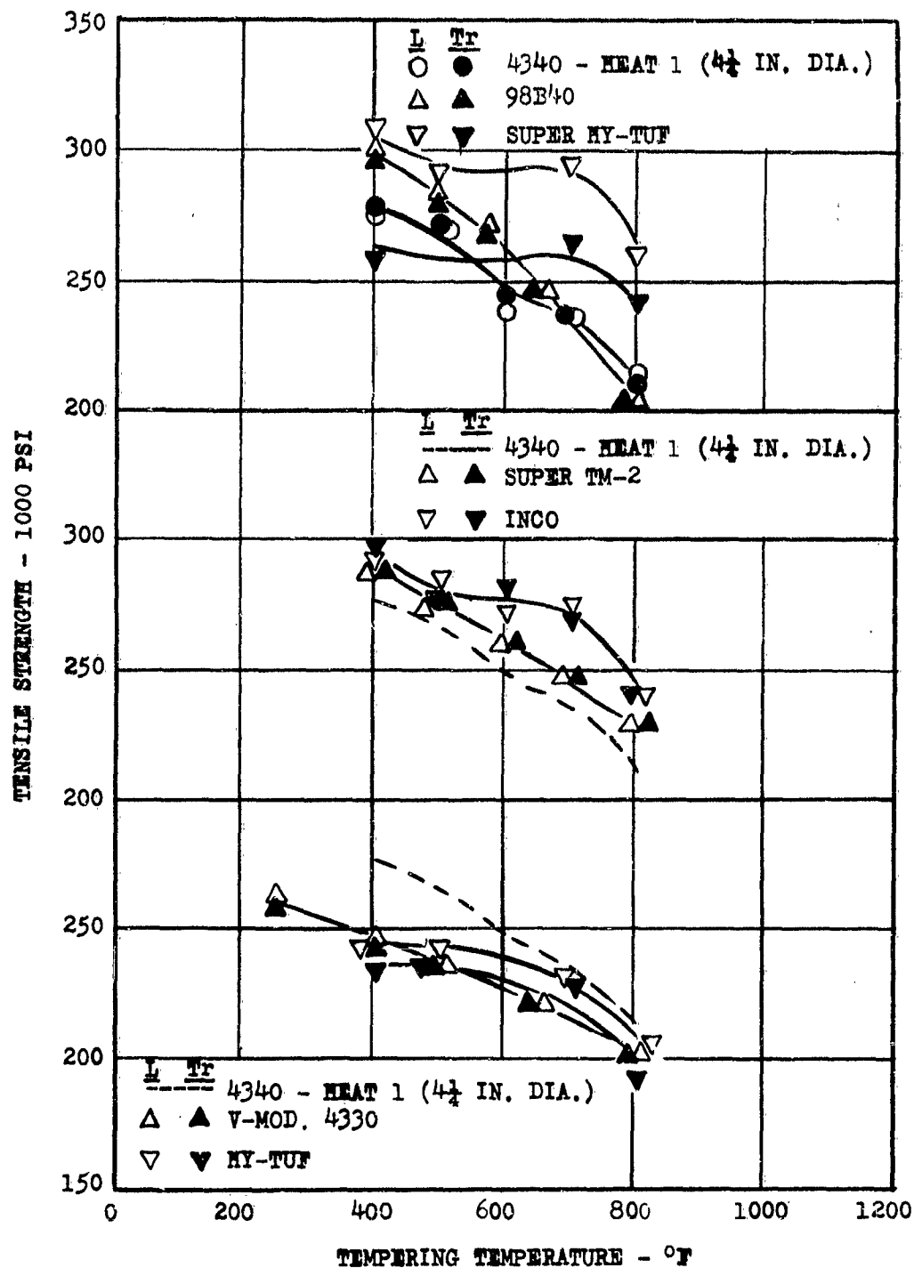
FIG. 54 TENSILE STRENGTH OF 4340, 98B40, SUPER HY-TUF, SUPER TM-2, INCO, V-MOD. 4330 AND HY-TUF AS A FUNCTION OF OF TEMPERING TEMPERATURE.
