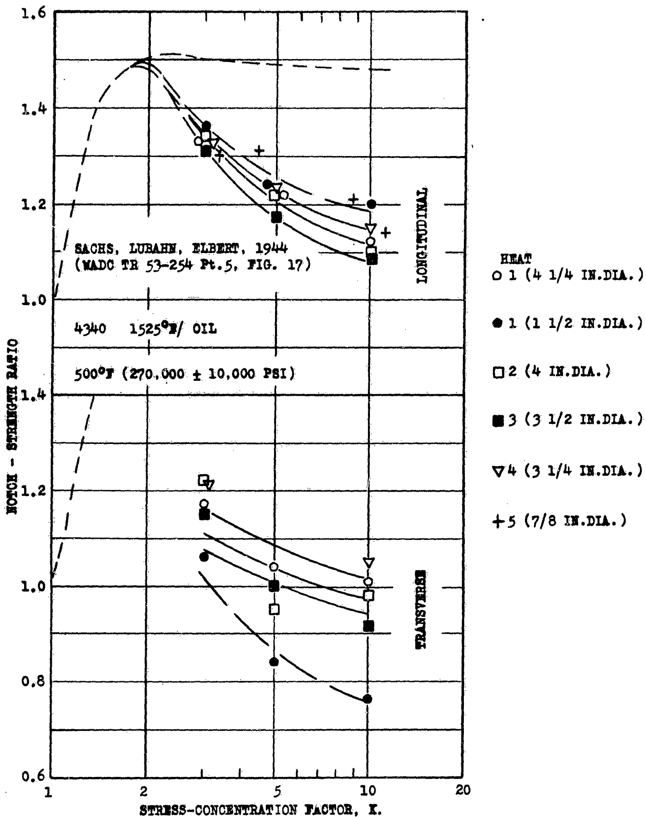
FIG. 18 VARIATION OF NOTCH-STRENGTH RATIO OF VARIOUS 4340 STEEL HEATS WITH STRESS CONCENTRATION FOR 0.3 IN.DIA.SPECIMENS.
