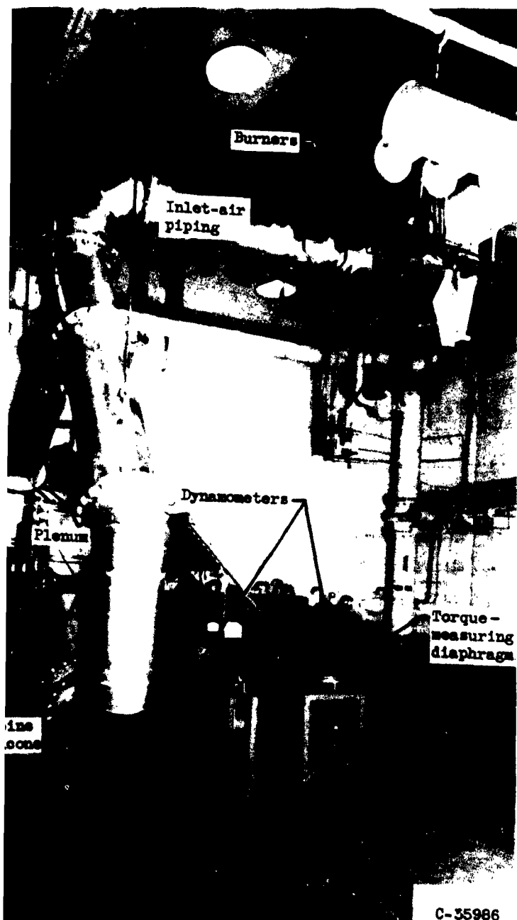
of J71-132 experimental three-stage turbine in full-scale facility.
