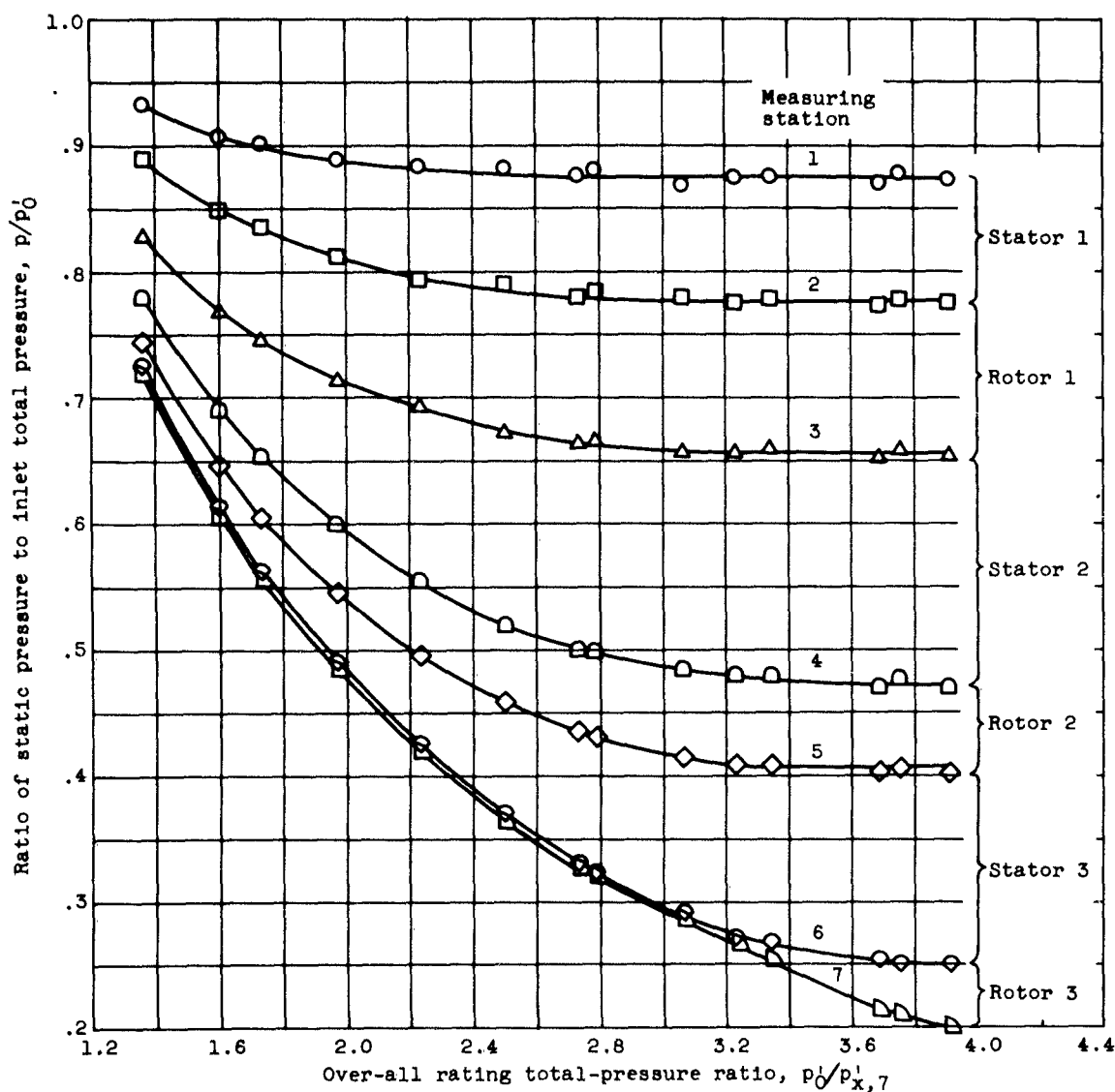
(a) Equivalent speed, 80-percent design.
