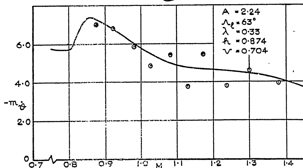
FIG. 31(b) VARIATION OF m_{\delta} WITH MACH NO. FOR AIRCRAFT MODEL WITH SWEEP BACK WING AND UNSWEEP TAILPLANE.
