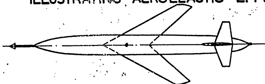
FIG. 31(a). VARIATION OF m_{\delta} WITH MACH NO. FOR TAILLESS SWEEP BACK WING MODEL ILLUSTRATING AEROELASTIC EFFECTS.
