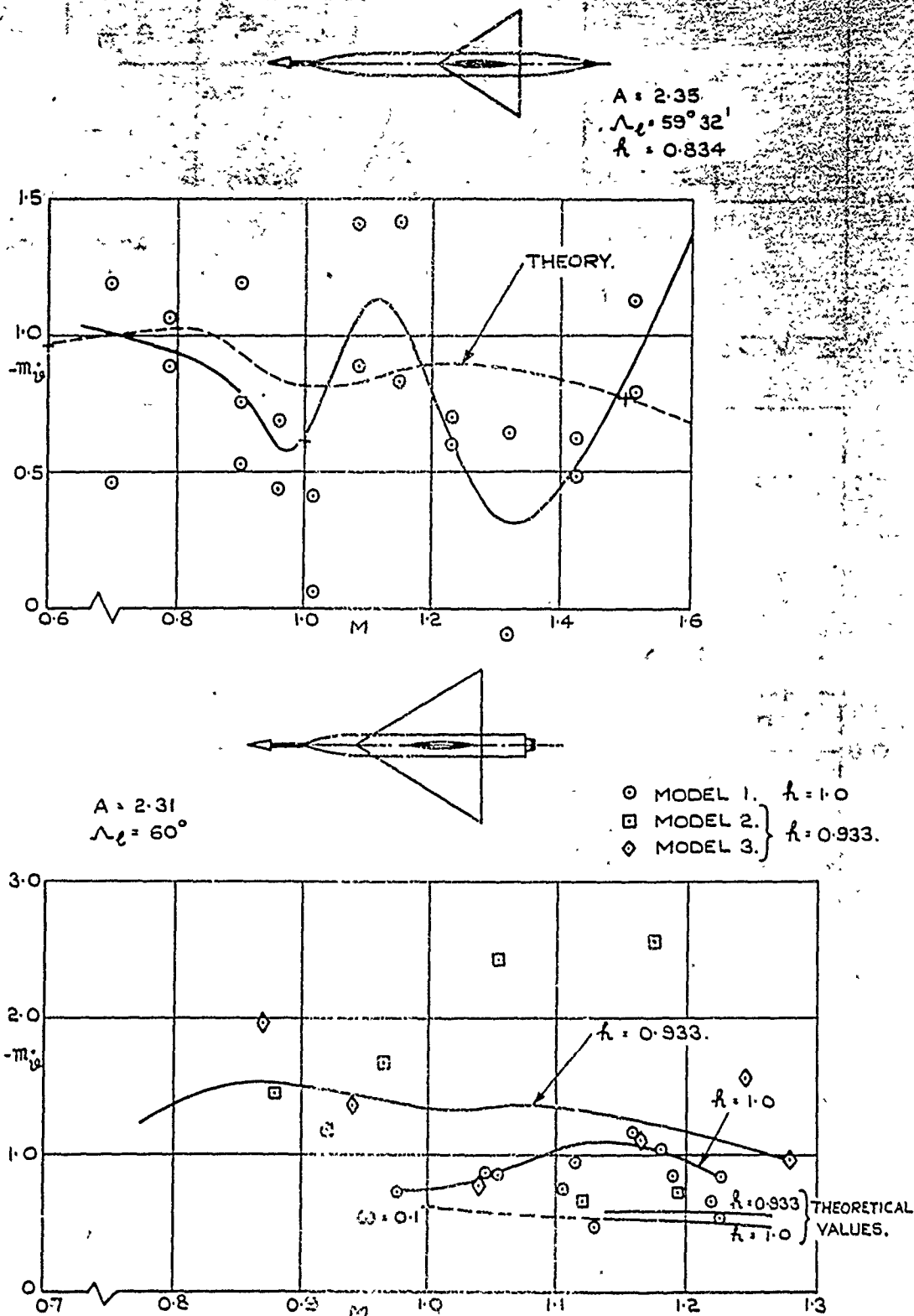
FIG. 24. VARIATION OF m_g WITH M FOR TWO TAILLESS DELTA WING CRUCIFORM MISSILES AS DETERMINED FROM GROUND LAUNCHED ROCKET TESTS.
