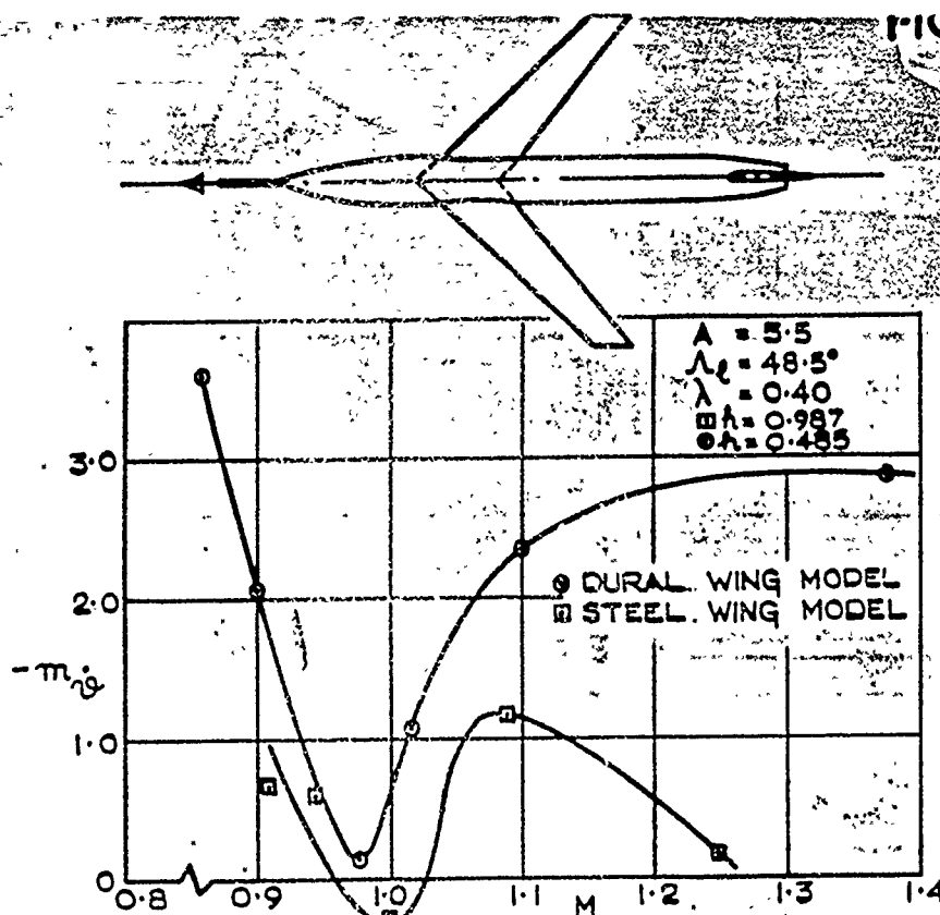
FIG. 31(a). VARIATION OF m_{\delta} WITH MACH NO. FOR TAILLESS SWEEP BACK WING MODEL ILLUSTRATING AEROELASTIC EFFECTS.
