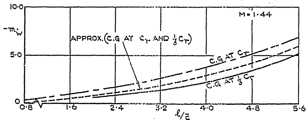
FIG. 12. COMPARISON OF "EXACT" & APPROXIMATE Z_w & m_w FOR DELTA WING-TAIL COMBINATIONS AT VARIOUS C.G. POSITIONS, & MACH NUMBERS (FROM REF. T 38)
