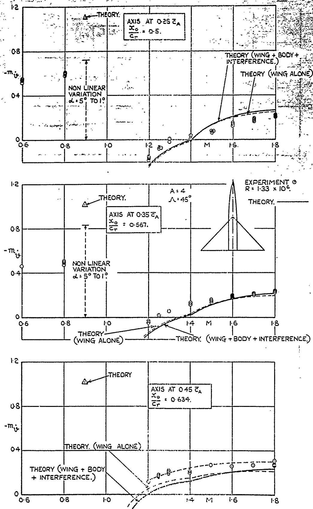
FIG.20. COMPARISON OF THEORY AND WIND TUNNEL TEST RESULTS FOR DELTA WING, A = 4 , \Lambda_\ell = 45^\circ .
