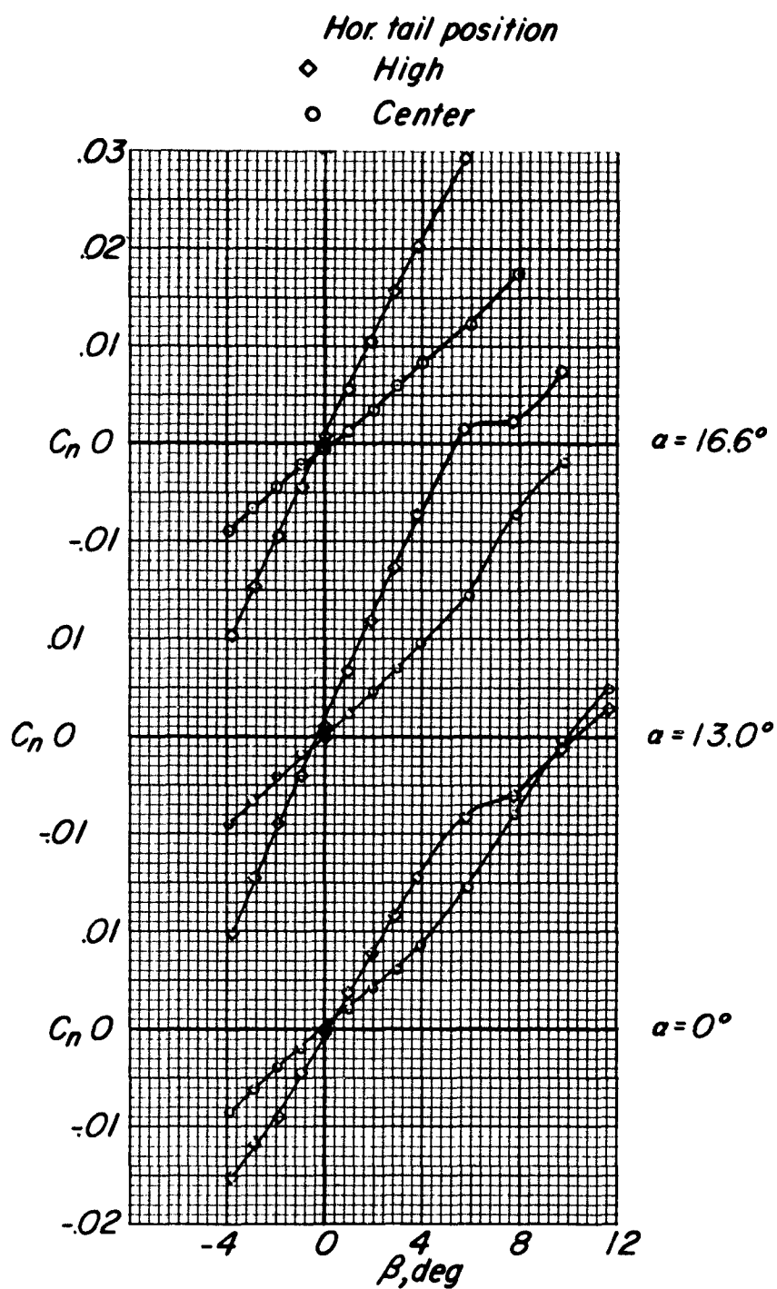
(b) C_n against \beta .
