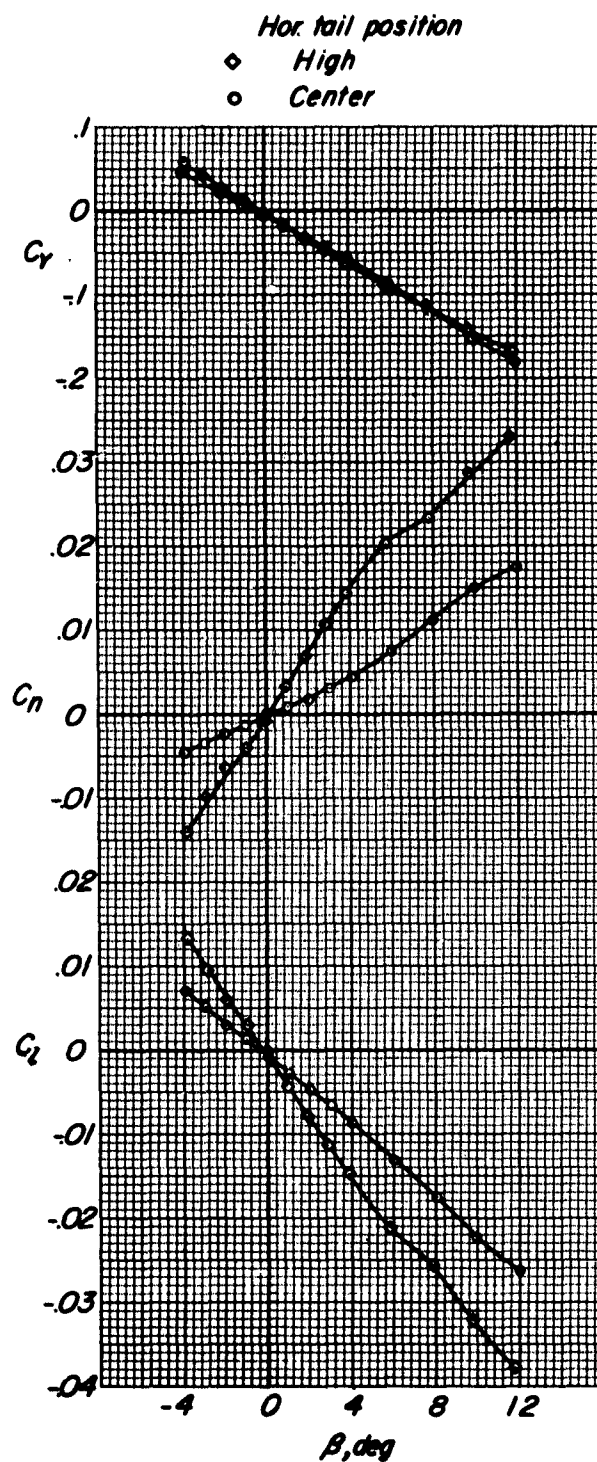
Figure 17.- Variation of lateral aerodynamic characteristics with angle of sideslip of high-wing-fuselage model with horizontal tail in center and high positions. M = 0.92 ; \alpha = 0^\circ .
