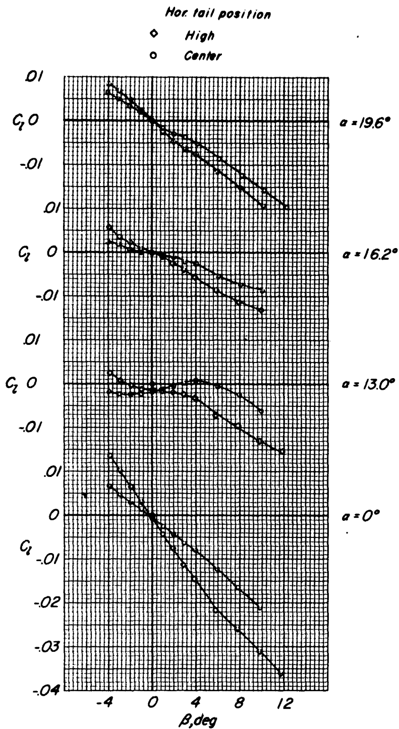
(c) C_l against \beta .
