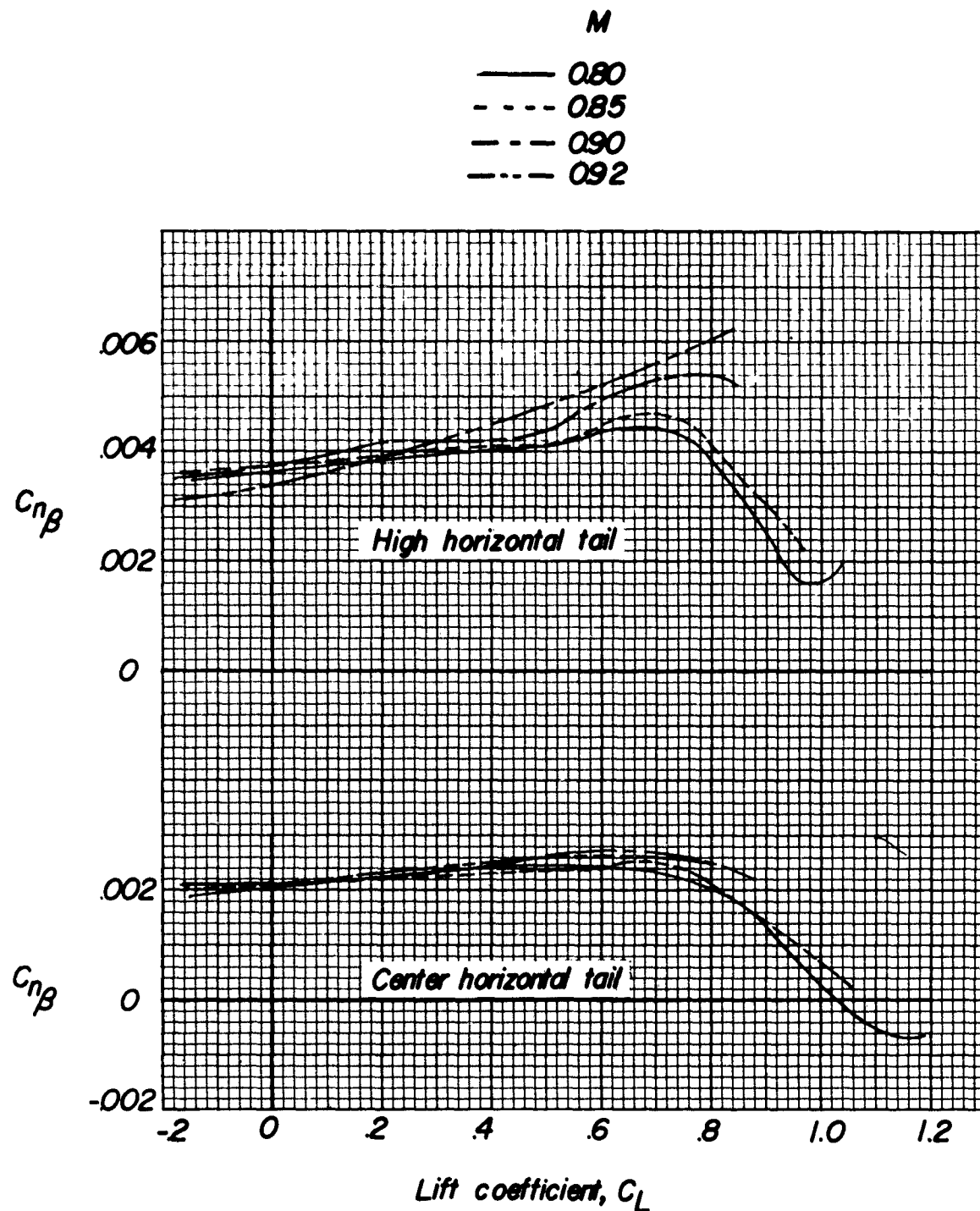
Figure 12.- Effect of Mach number on the variation of C_{n\beta} with C_L for two horizontal-tail locations.
