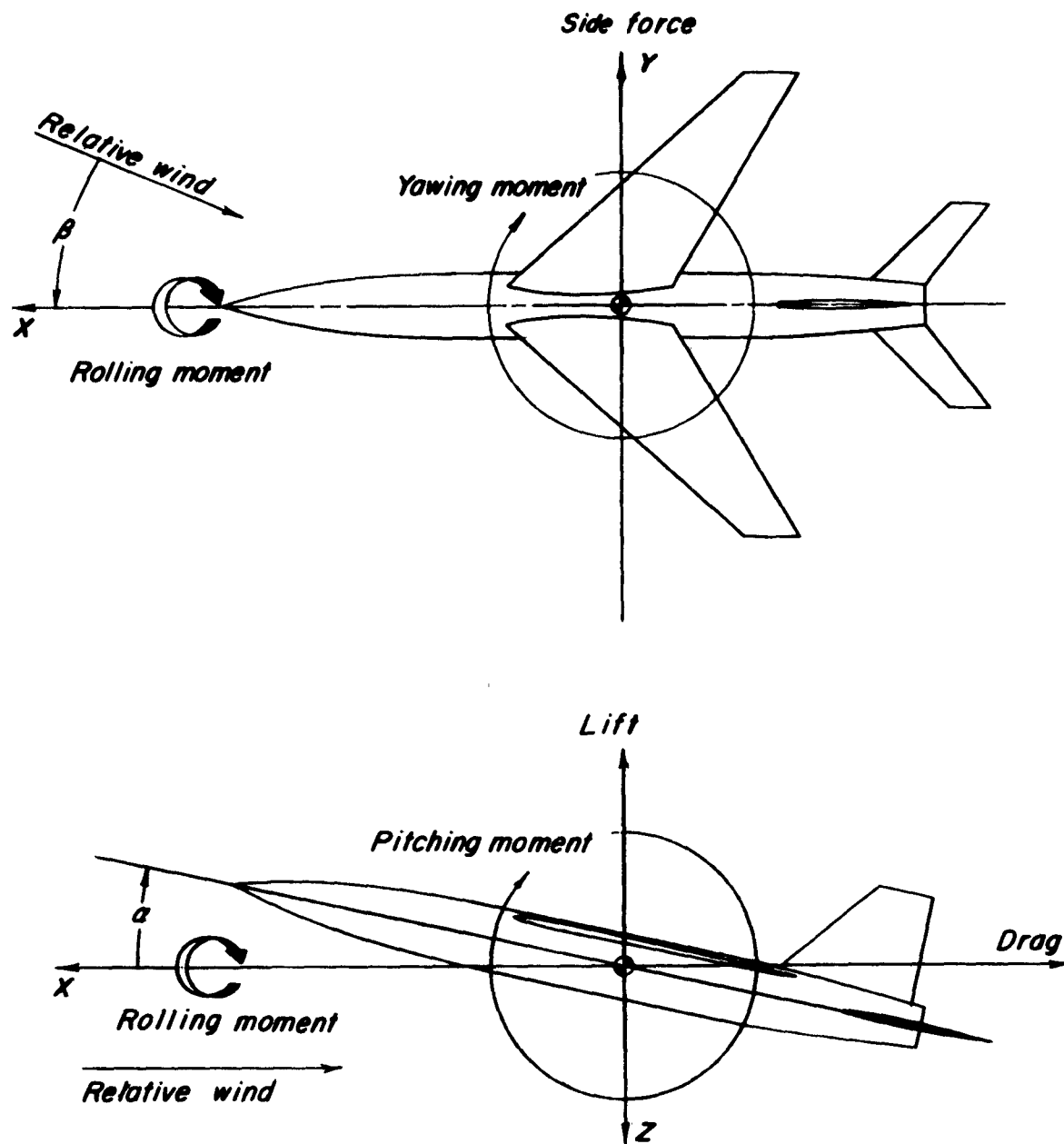
Figure 1.- Stability system of axes. Positive directions of forces, moments, and angles are indicated by arrows.
