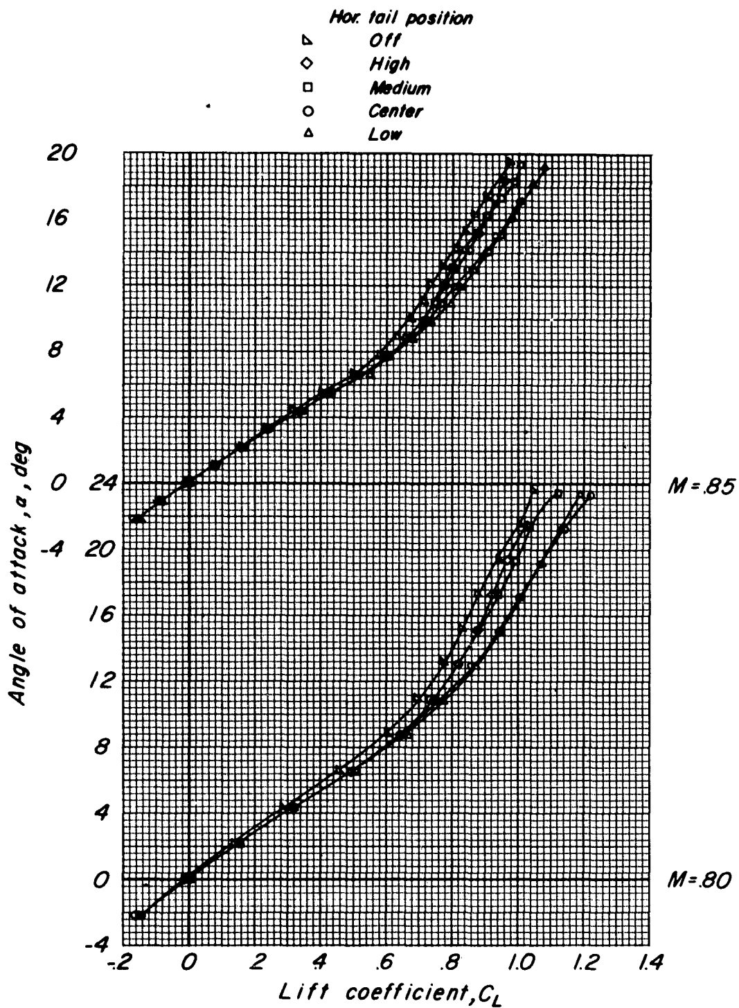
Figure 5.- Variation of lift coefficient with angle of attack of high-wing-fuselage model without and with horizontal tail at various vertical locations.
