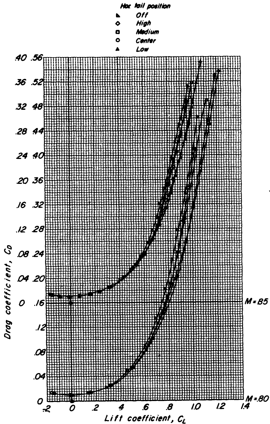
Figure 6.- Variation of drag coefficient with lift coefficient of high-wing-fuselage model without and with horizontal tail at various vertical locations.
