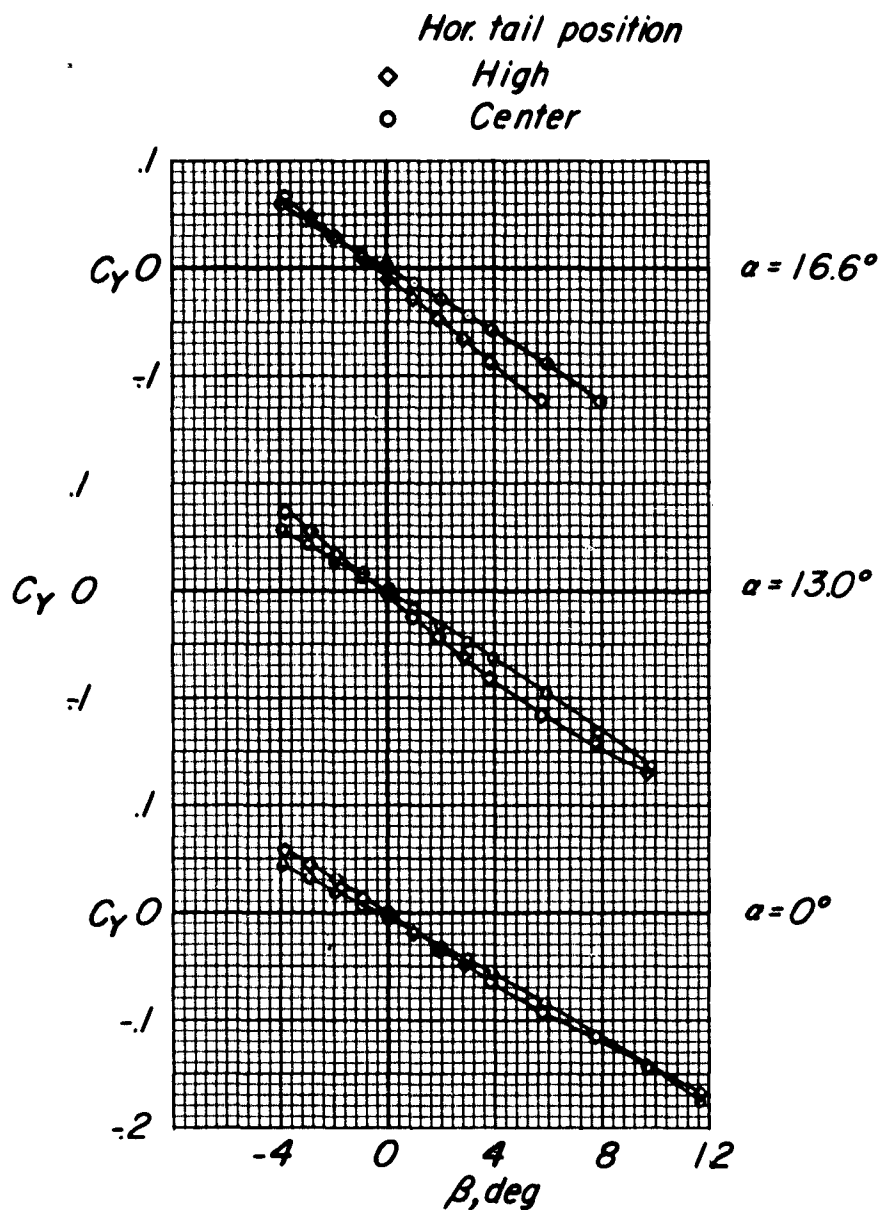
(a) C_y against \beta .
