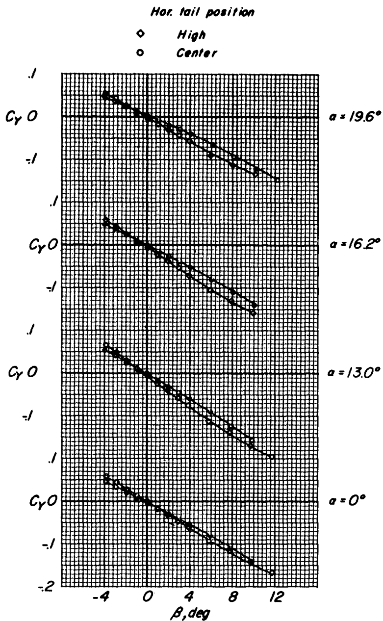
(a) C_Y against \beta .
