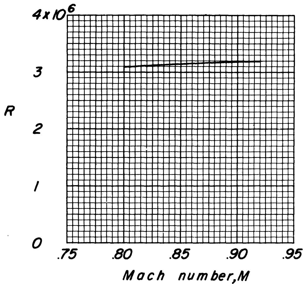
Figure 4.- Variation with Mach number of Reynolds number (based on wing mean aerodynamic chord).
