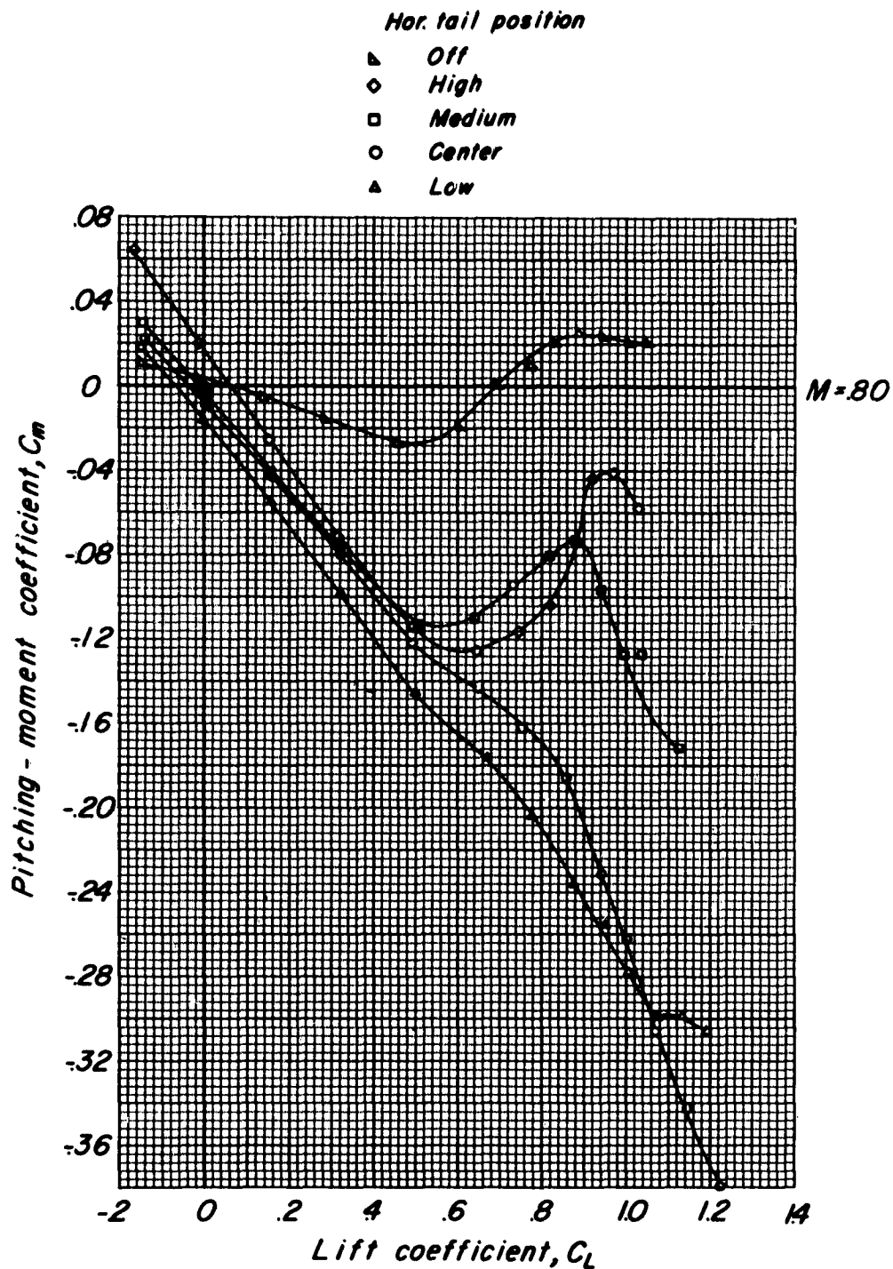
Figure 7.- Variation of pitching-moment coefficient with lift coefficient of high-wing-fuselage model without and with horizontal tail at various vertical locations.
