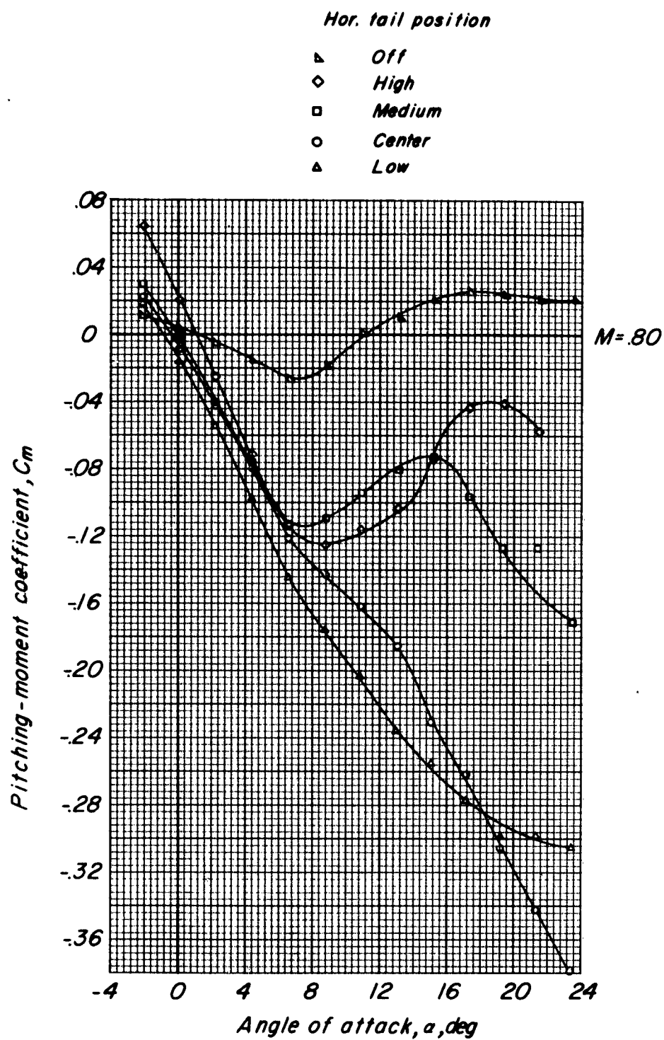
Figure 8.- Variation of pitching-moment coefficient with angle of attack of high-wing-fuselage model without and with horizontal tail at various vertical locations.
