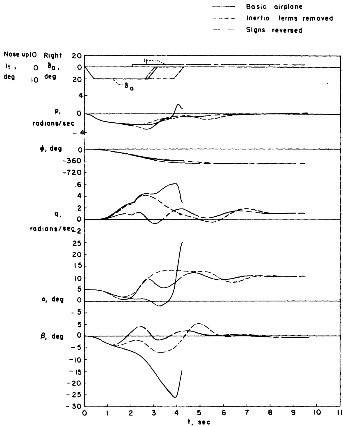
Figure 6.- Time histories of control motion and computed airplane response in 360^\circ rolls made with 20^\circ left total aileron. Stabilizer moved 2^\circ in direction to produce positive pitching moment when roll angle reached 180^\circ . Curves shown for basic airplane, roll coupling terms omitted from equations, and signs of roll coupling terms reversed.
