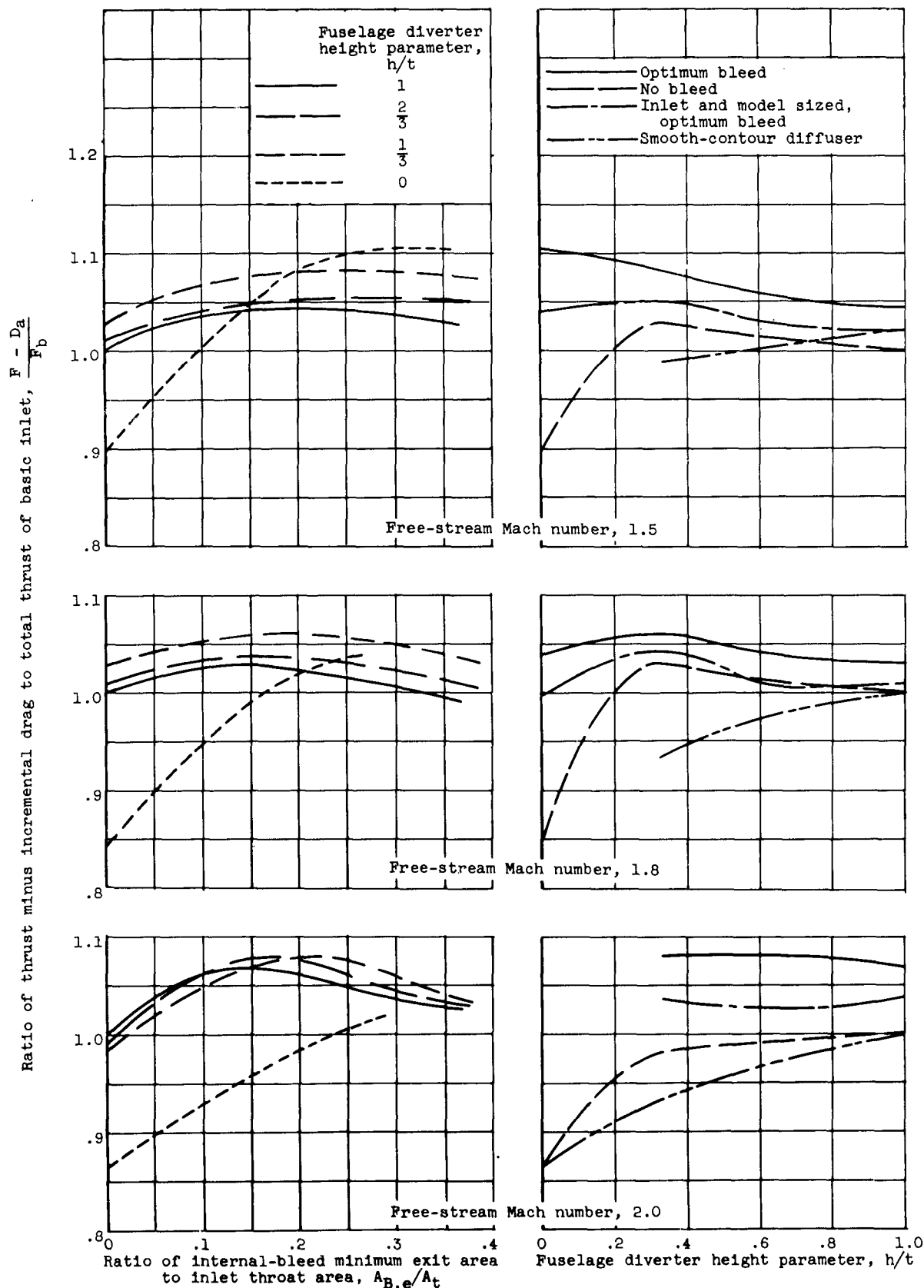
(a) Effect of internal-bleed area.
