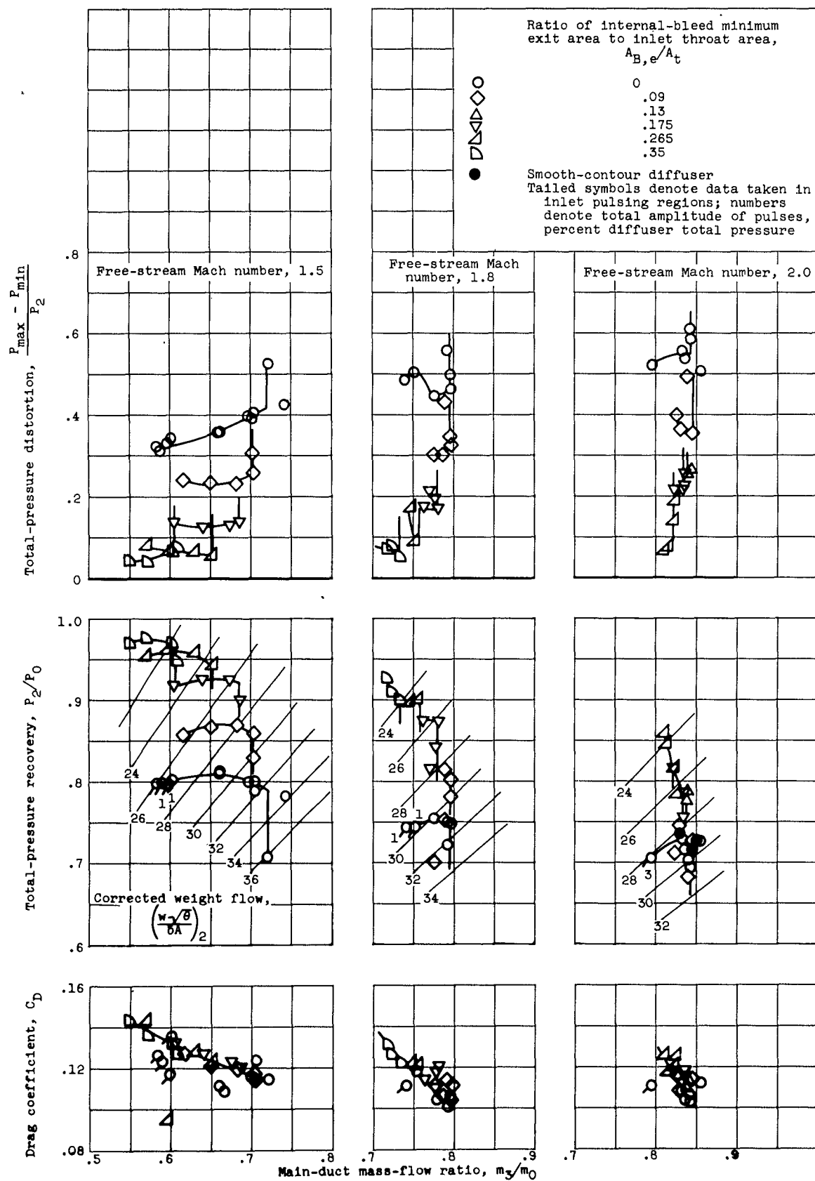
Figure 4. - Concluded. Effect of inlet throat bleed on inlet performance.
