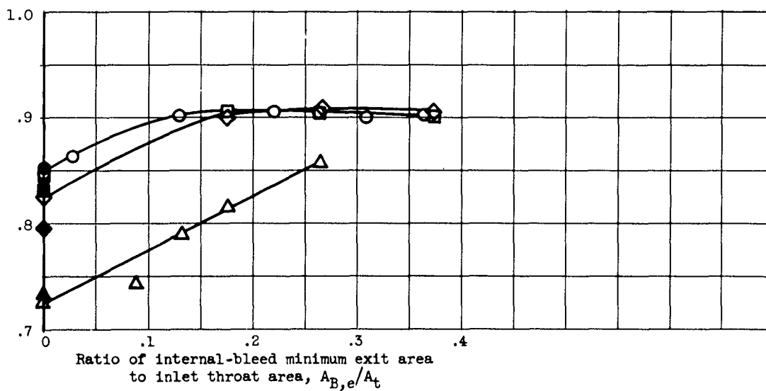
(c) Free-stream Mach number, 2.0.
