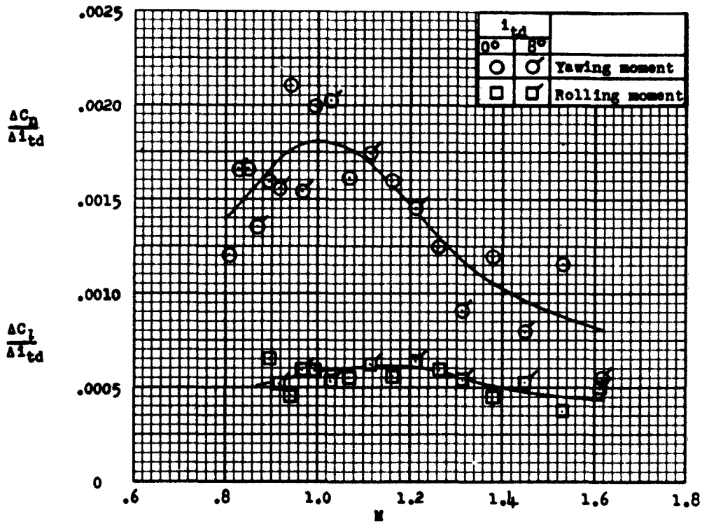
Figure 11.- Variation with Mach number of yawing-moment effectiveness \frac{\Delta C_n}{\Delta i_{td}} and rolling effectiveness \frac{\Delta C_l}{\Delta i_{td}} of differentially deflected tail surfaces.
