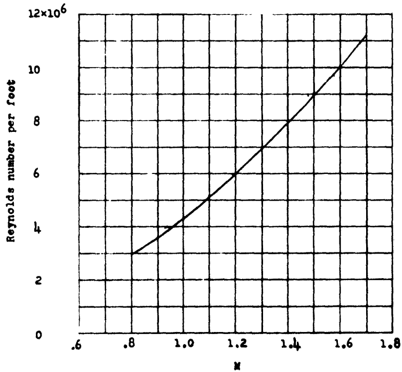
Figure 5.- Reynolds number of test.
