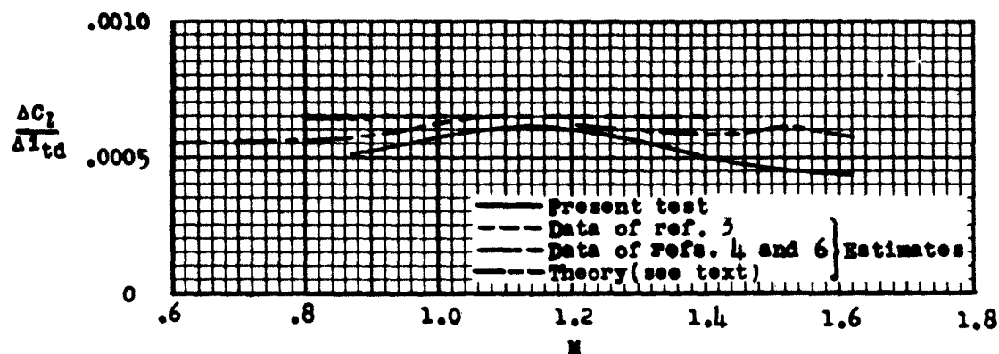
Figure 12.- Comparison of rolling-moment effectiveness with other results.
