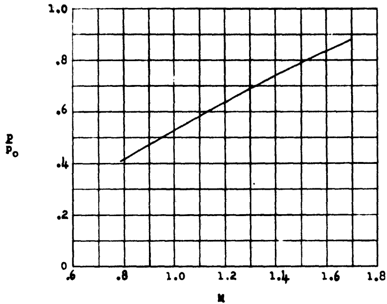
Figure 4.- Static-pressure ratio.
