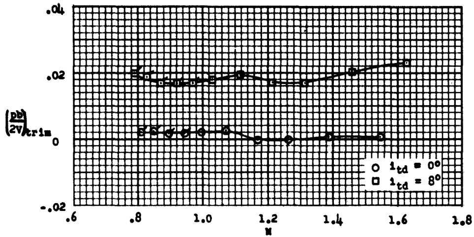
Figure 10.- Variation of rolling-effectiveness parameter (\frac{pb}{2V})_{trim} with Mach number. Flagged symbols indicate that trim condition is uncertain.
