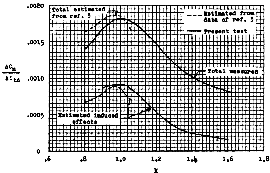
Figure 13.- Comparison of yawing-moment effectiveness with other results.
