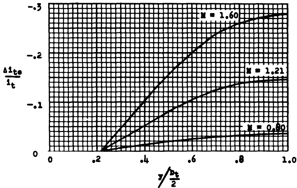
(a) Twist distribution.
