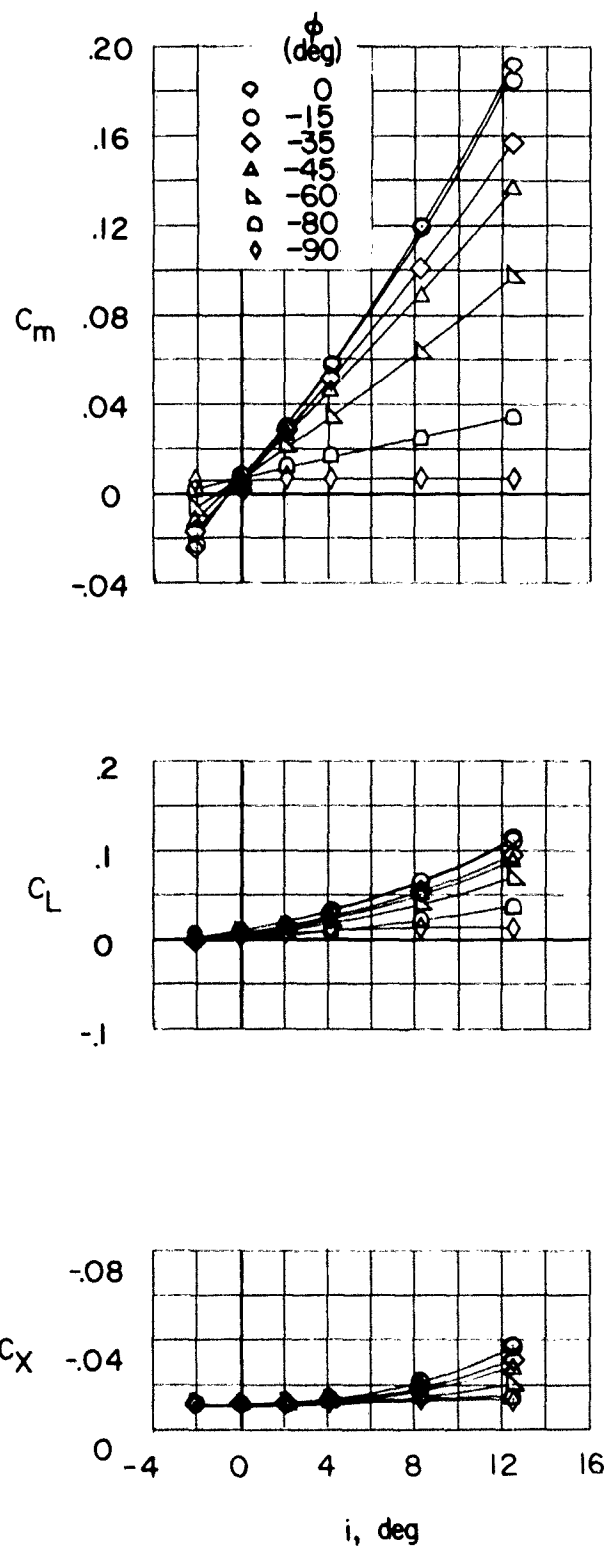
Figure 9.- The variation of the basic coefficients with incidence angle i for configuration BC; \delta_H = 0^\circ .
