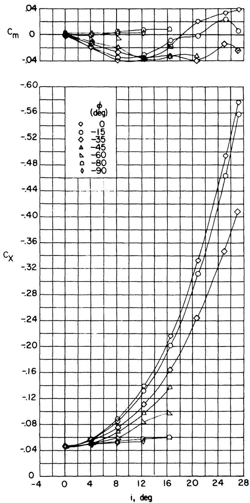
Figure 7.- The variation of basic coefficients with incidence angle i for configuration BWCN; \delta v = -10^\circ .
