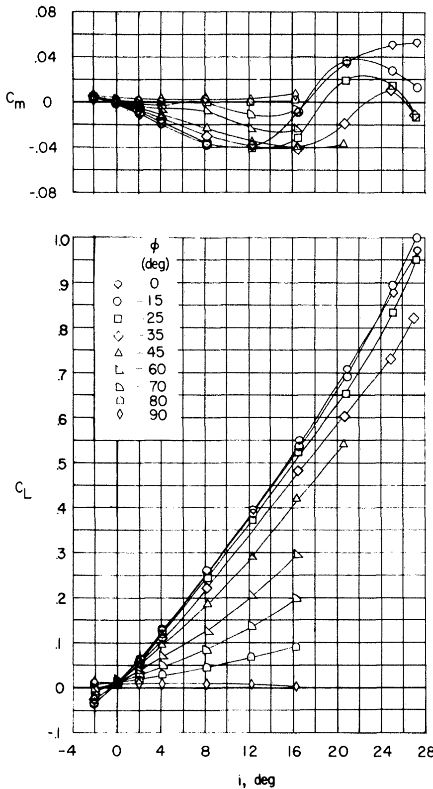
Figure 4.- The variation of the basic coefficients with incidence angle i for configuration BWCN; \delta_H = 0^\circ .
