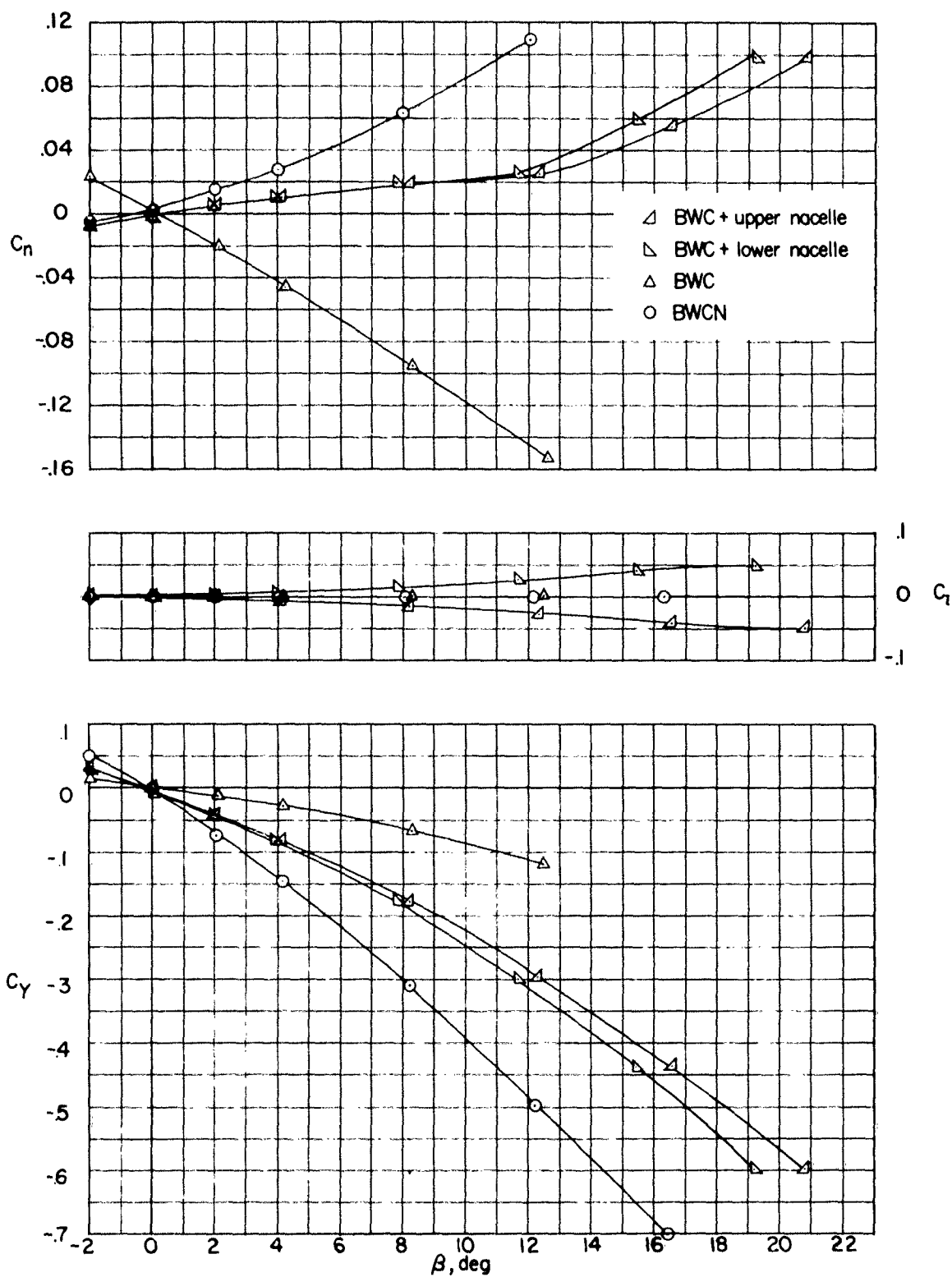
Figure 21.- Effect of nacelle location on the aerodynamic characteristics in sideslip; \alpha = 0^\circ .
