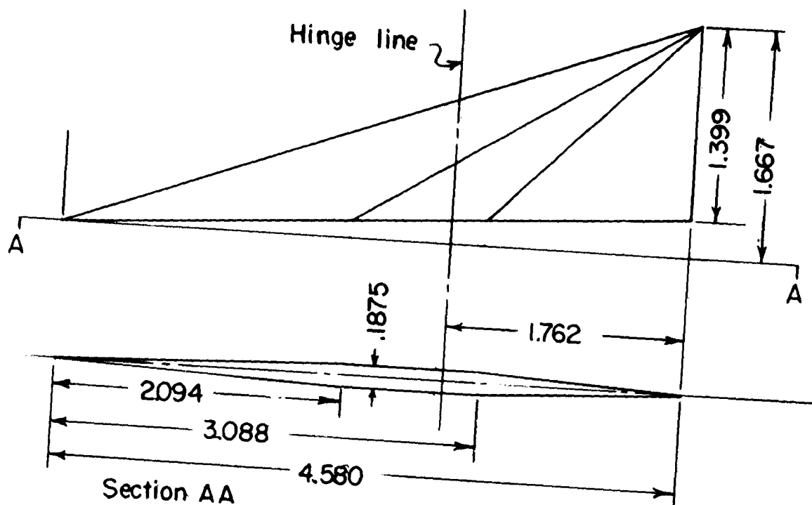
Horizontal canard
