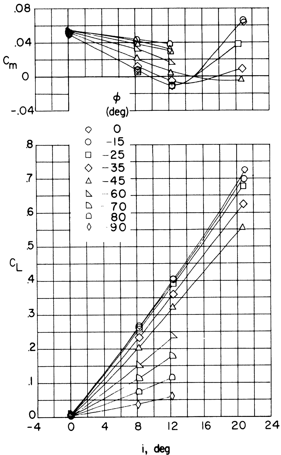
Figure 5.- The variation of the basic coefficients with incidence angle i for configuration BWCN; \delta_H = -8^\circ .
