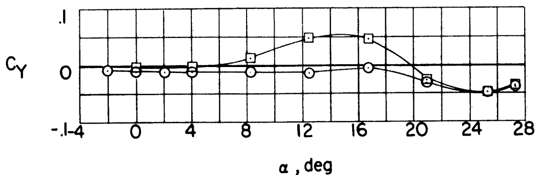
Figure 22.- Effect of vertical canard deflection on the aerodynamic characteristics in pitch; \beta = 0^\circ .
