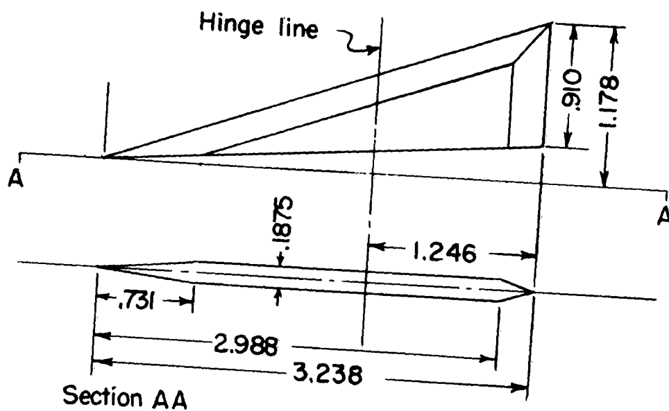
Vertical canard
