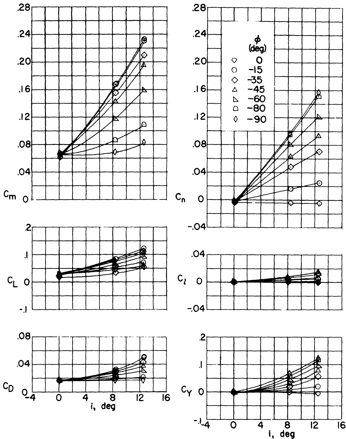
Figure 11.- The variation of the basic coefficients with incidence angle i for configuration BC; \delta_H = -12^\circ .
