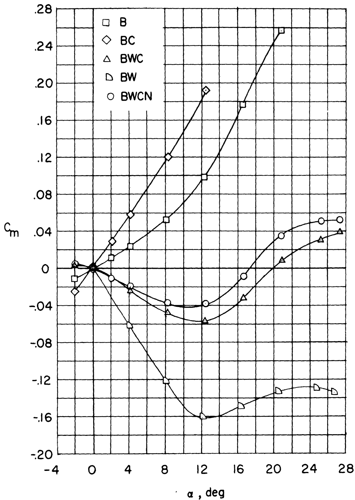
Figure 16.- Aerodynamic characteristics in pitch of the complete model and various combinations of its components; \beta = 0^\circ .
