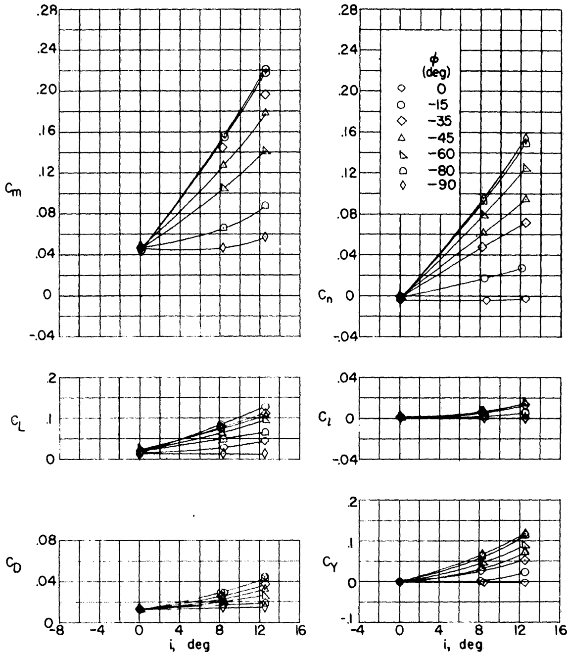
Figure 10.- The variation of the basic coefficients with incidence angle i for configuration BC; \delta_H = -8^\circ .
