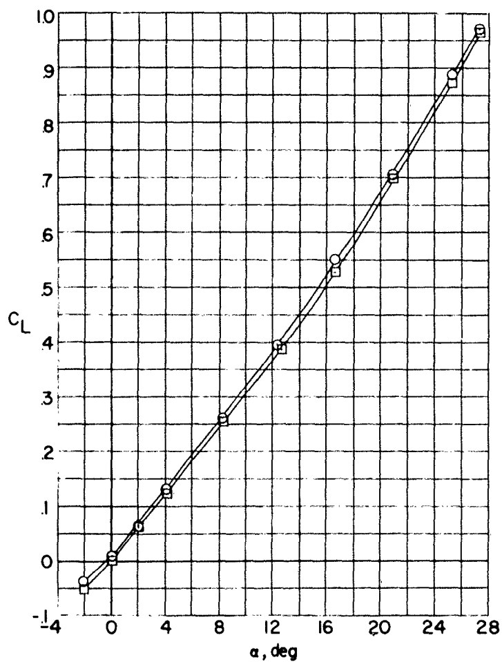
Figure 24.- Effect of aileron deflection on the aerodynamic characteristics in pitch; \beta = 0^\circ .
