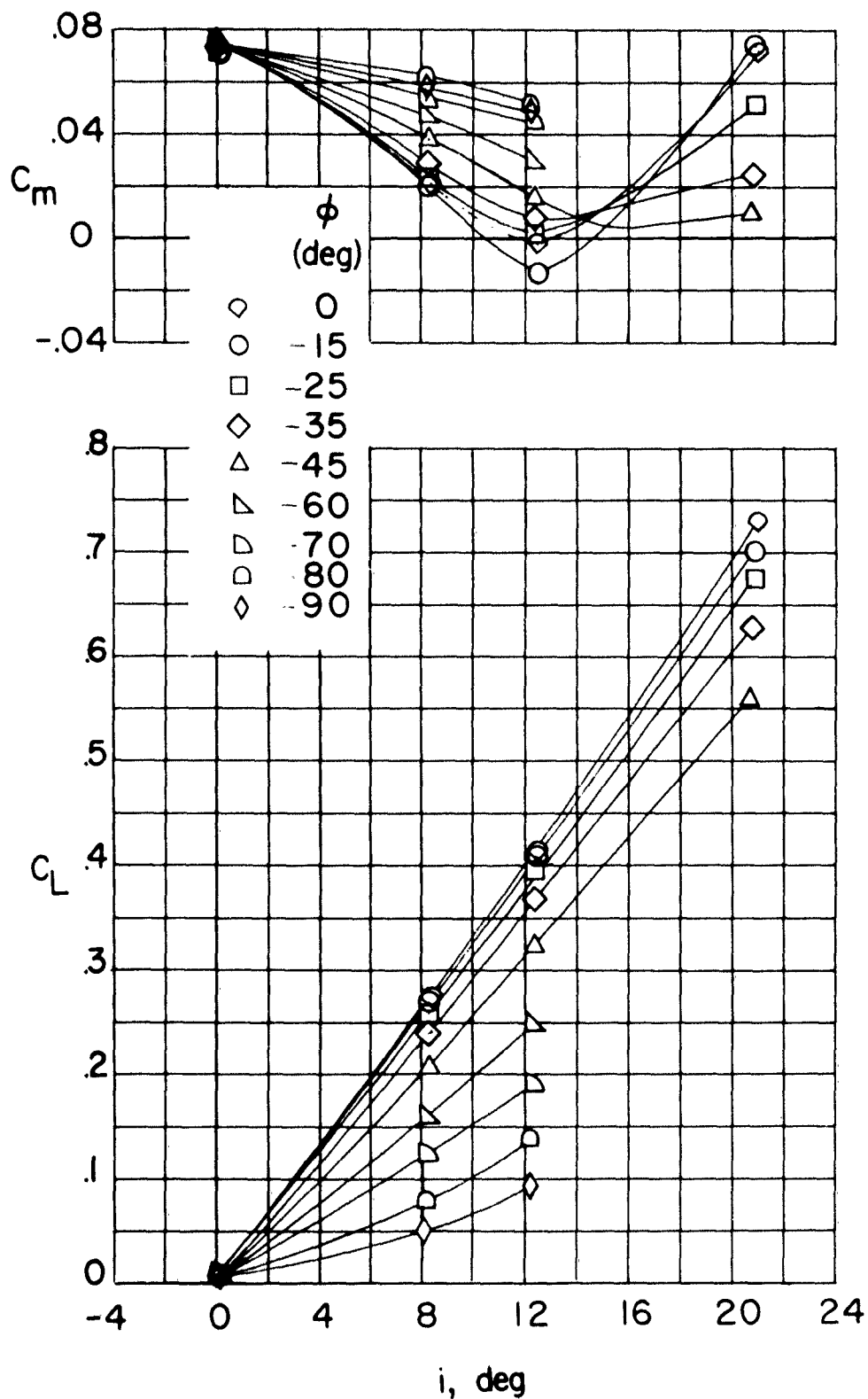
Figure 6.- The variation of the basic coefficients with incidence angle i for configuration BWCN; \delta_H = -12^\circ .
