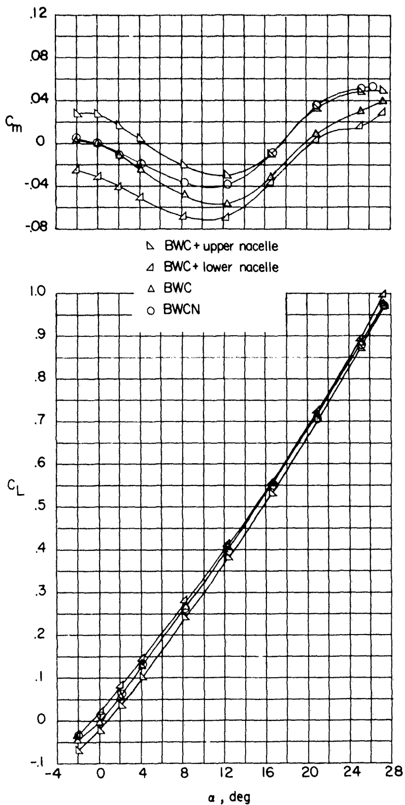
Figure 18.- Effect of nacelle location on the aerodynamic characteristics in pitch; \beta = 0^\circ .
