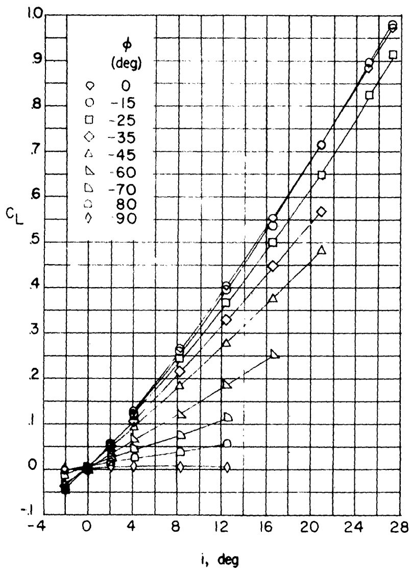
Figure 13.- The variation of the basic coefficients with incidence angle i for configuration BWC; \delta_H = 0^\circ .
