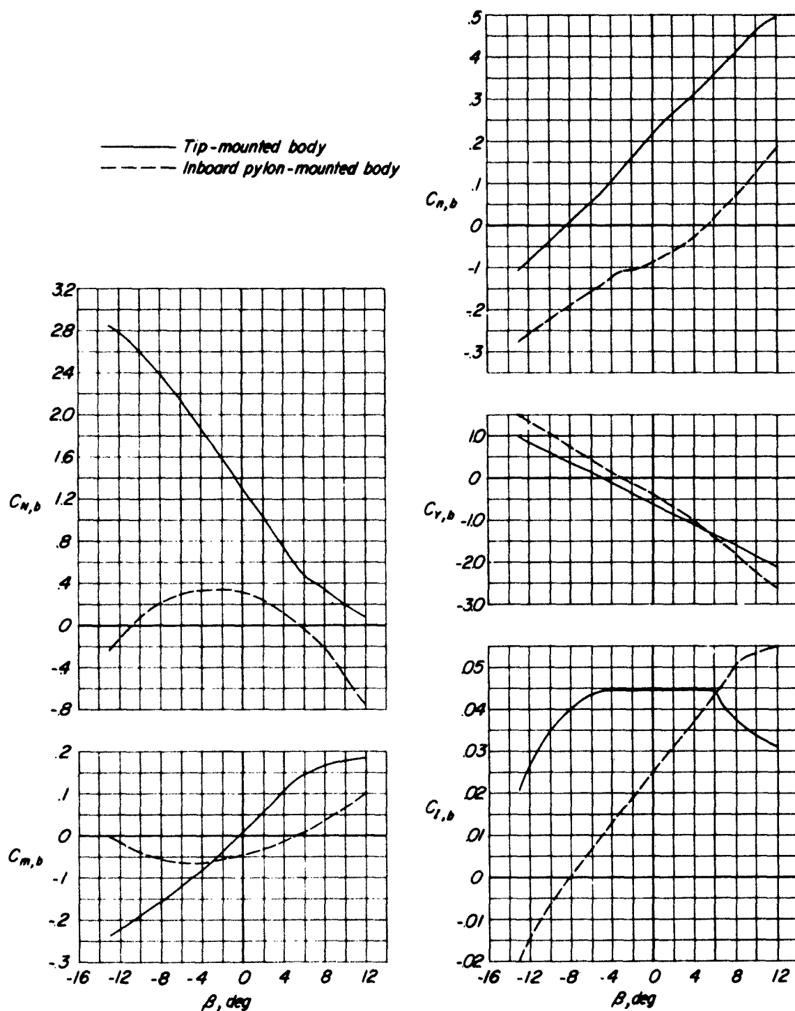
Figure 11.- Comparison of aerodynamic characteristics of a body mounted on the left wing tip and from a pylon under the left wing of a wing-fuselage model. Fins on; M = 0.50 ; \alpha = 6.3^\circ ; moment center at 0.462l_p .
