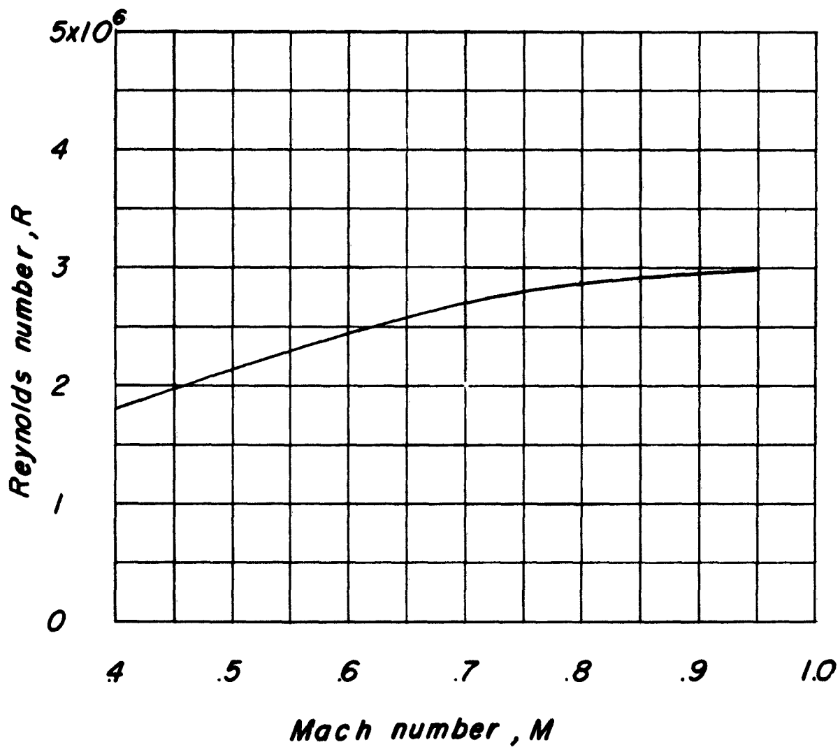
Figure 5.- Variation of average Reynolds number with Mach number. Reynolds number based on wing mean aerodynamic chord (0.765 foot).
