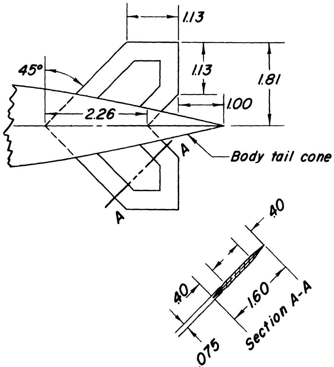
Figure 3.- Details of stabilizing fins. All dimensions are in inches.
