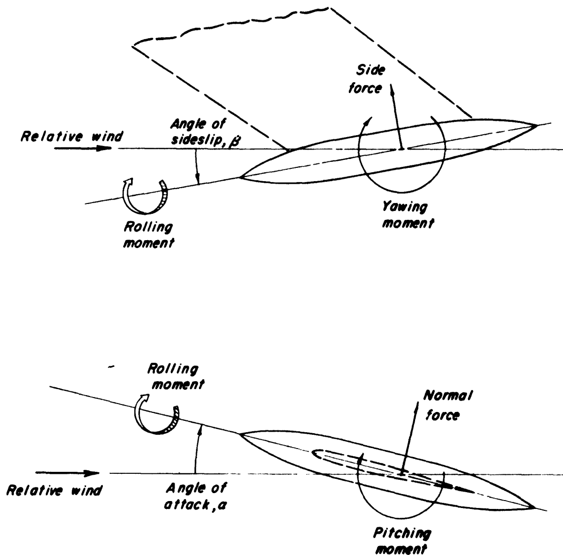
Figure 1.- Positive directions of body forces, moments, and angles.
