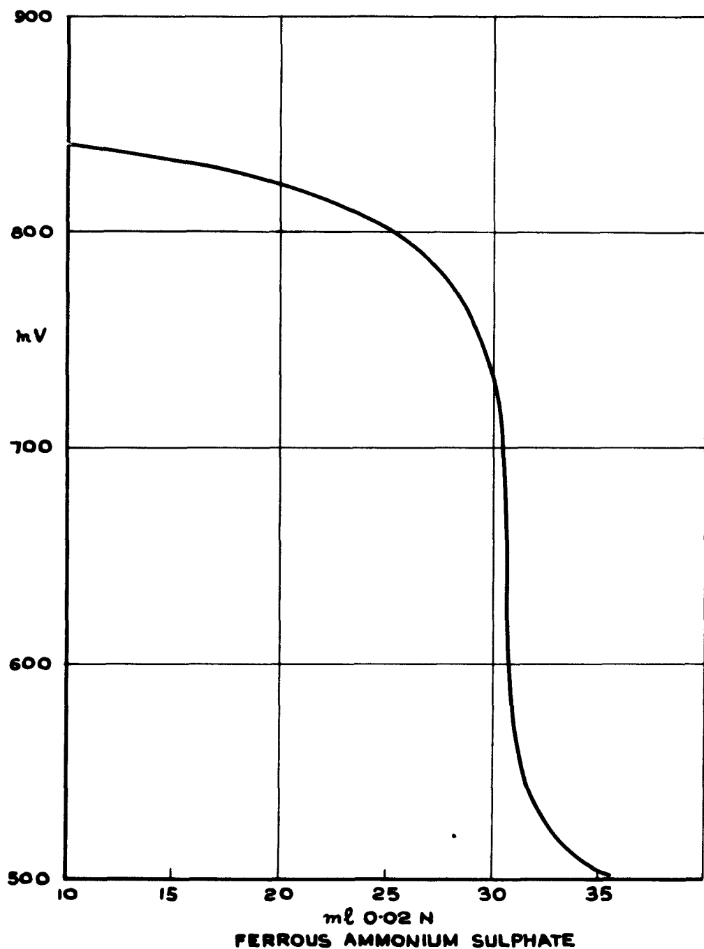
FIG. I - REDUCTION OF VANADATE WITH FERROUS AMMONIUM SULPHATE
