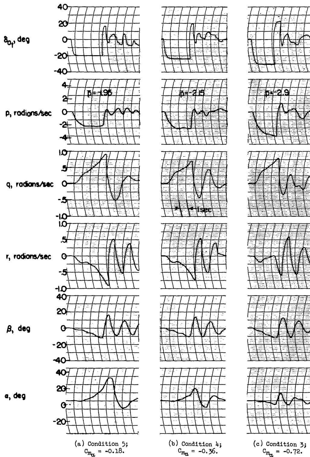
Figure 10.- Representative time histories for swept-wing configuration. Input B; C_{n\beta} = 0.228 .
