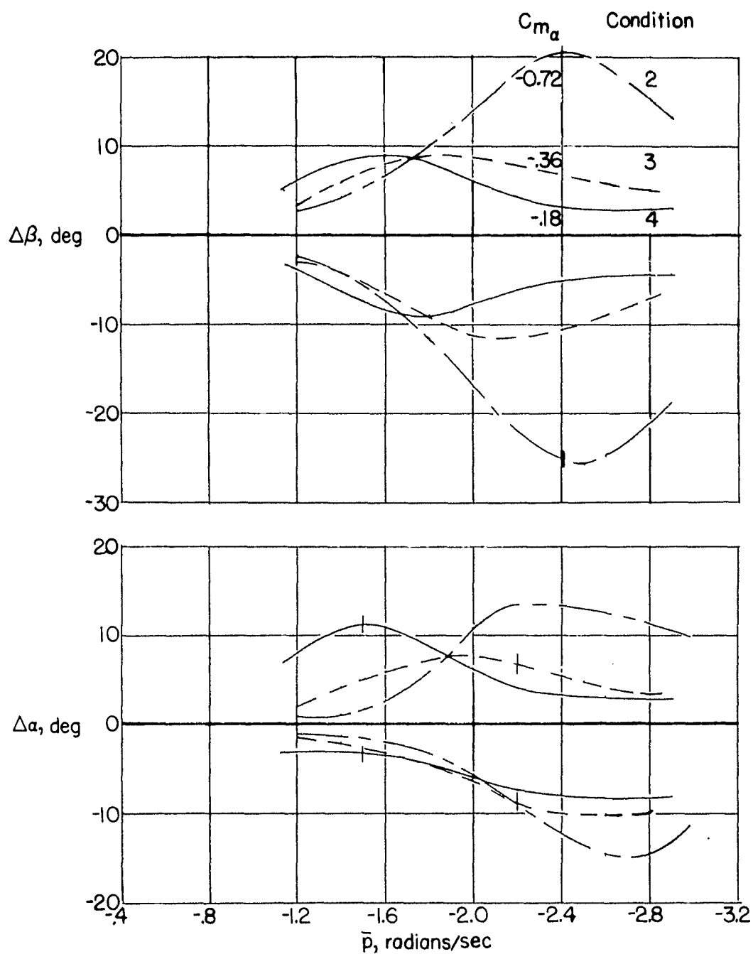
Figure 5.- Effect of C_{m_\alpha} variation. Swept-wing configuration; C_{n_\beta} = 0.114 ; input B.
