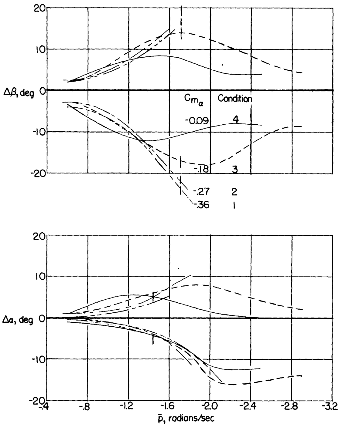
Figure 13.- Effect of C_{m_\alpha} variation. Delta-wing configuration; M = 0.8 ; input A.
