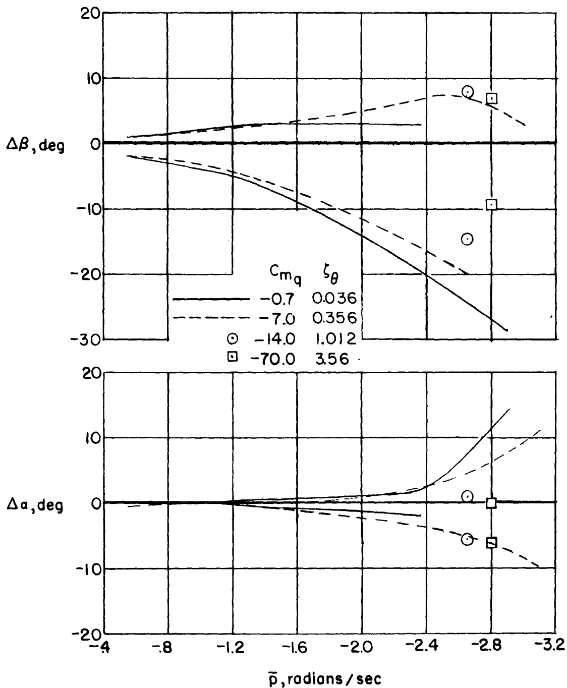
Figure 32.- Effects of increasing C_{mq} . Delta-wing configuration. M = 1.20 ; input A.
