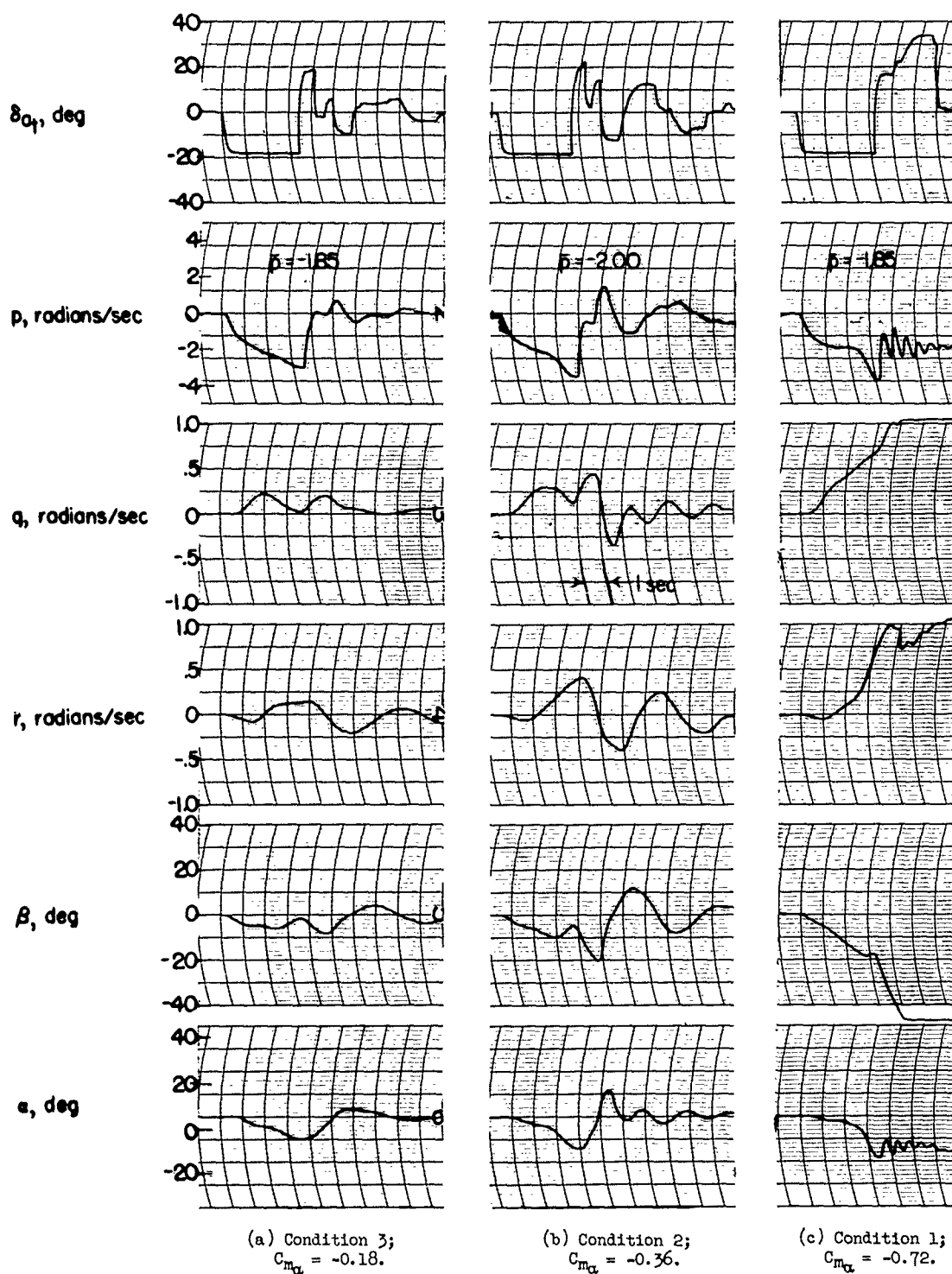
Figure 8.- Representative time histories for swept-wing configuration. Input B; C_{n\beta} = 0.057 .
