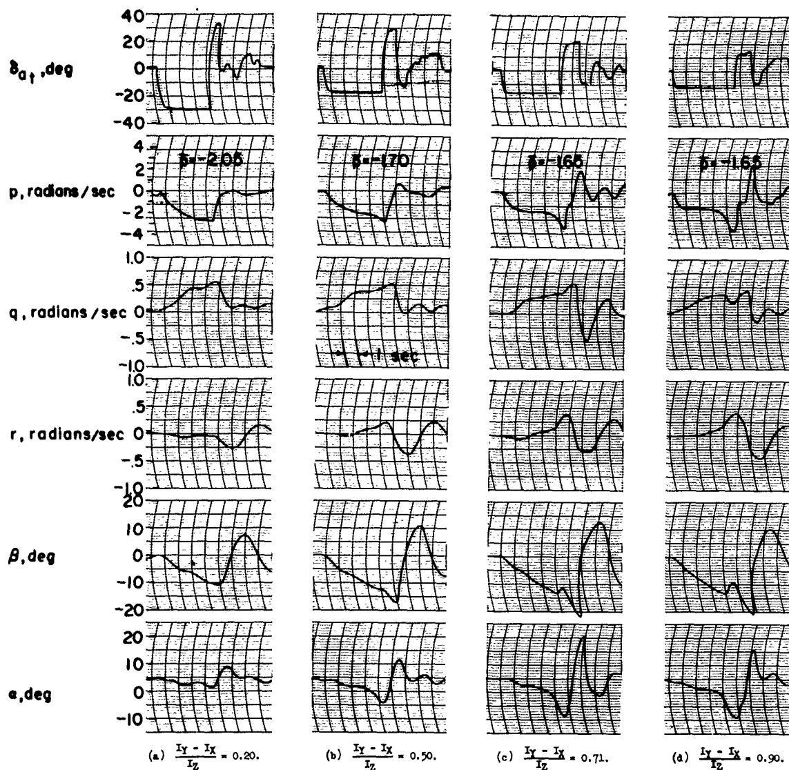
Figure 47.- Time histories showing effects of variations in mass distribution. Swept-wing configuration. C_{n\beta} = 0.057.
