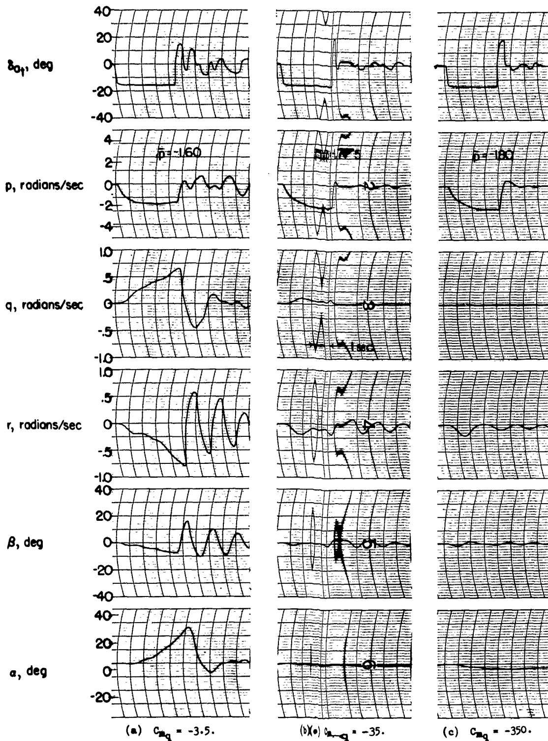
Figure 29.- Time histories showing effects of increasing C_{m_q} . Swept-wing configuration. Input B; C_{m_{\dot{\alpha}}} = -0.18 ; C_{n_{\beta}} = 0.228 .
