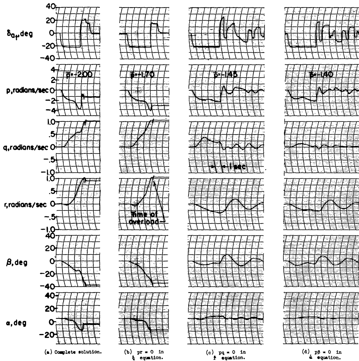
Figure 11.- Relative importance of various terms in equations of motions. Swept-wing configuration. Input B; C_{m\alpha} = -0.72 ; C_{n\beta} = 0.057 .
