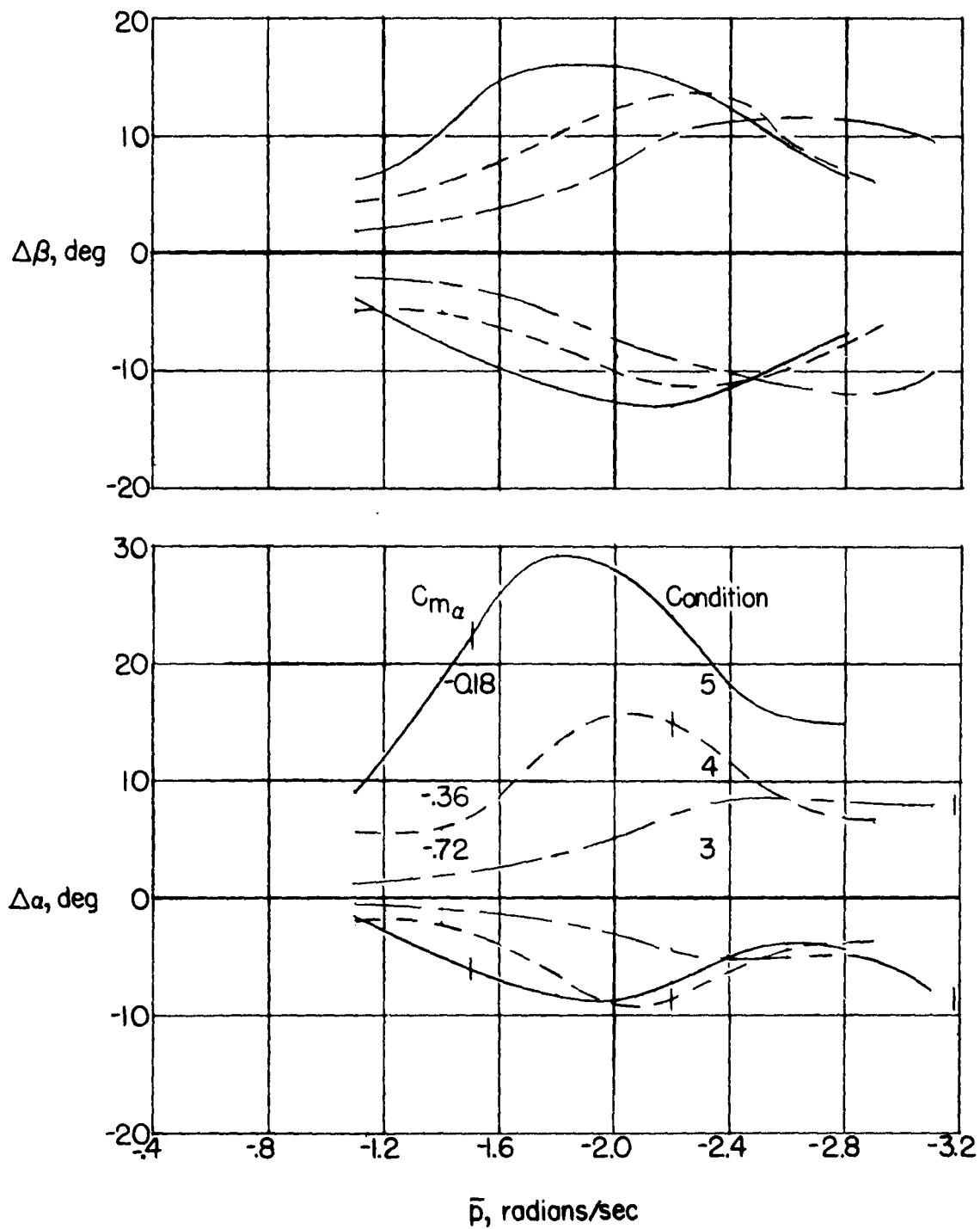
Figure 6.- Effect of C_{m_\alpha} variation. Swept-wing configuration; C_{n_\beta} = 0.228 ; input B.
