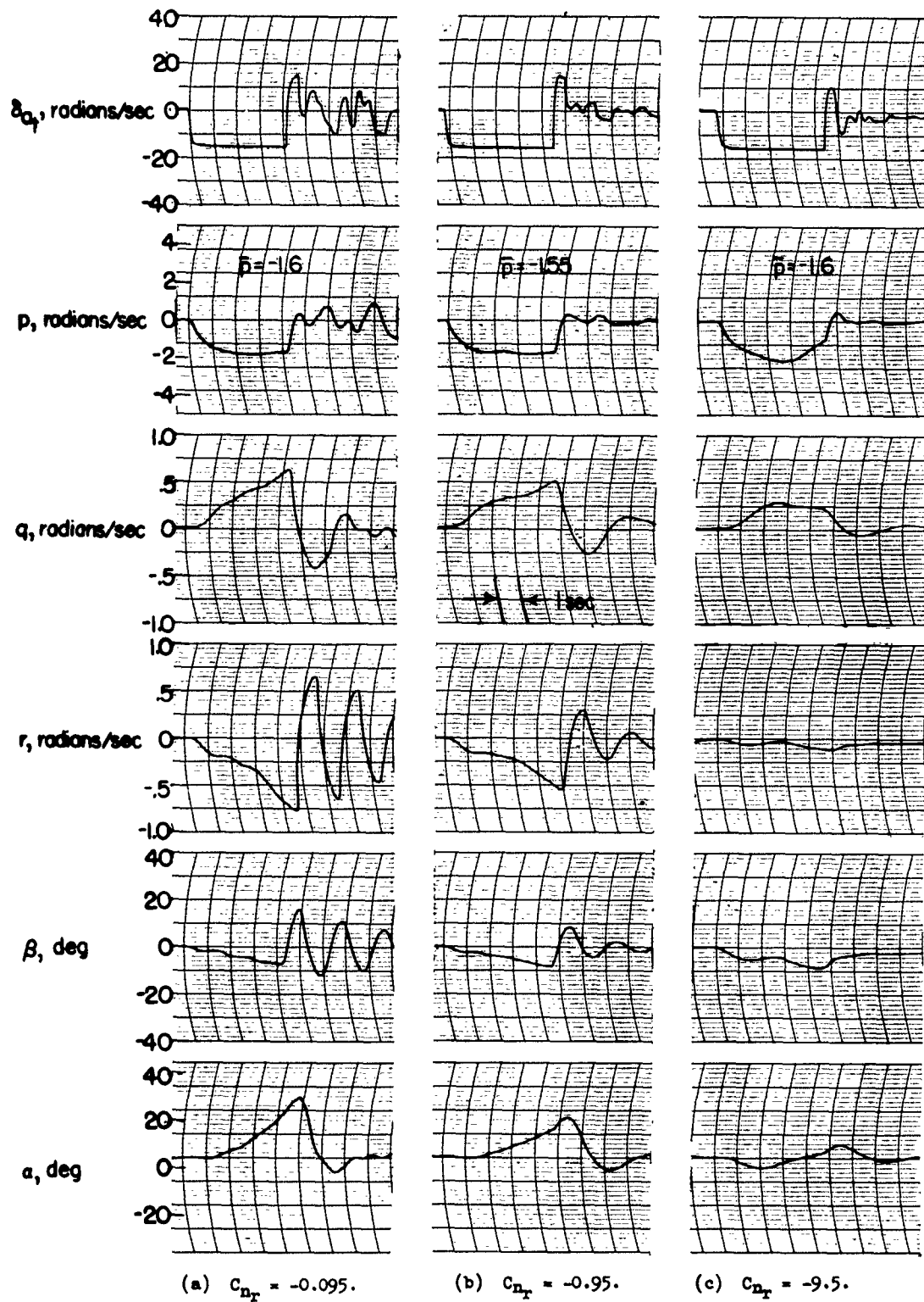
Figure 25.- Time histories showing effects of increasing C_{n_r} . Swept-wing configuration. Input B; C_{m_\alpha} = -0.18 ; C_{n_\beta} = 0.228 .
