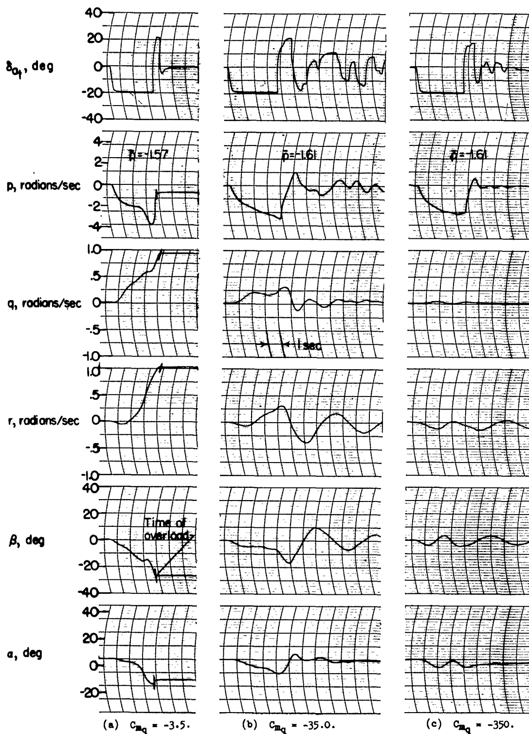
Figure 28.- Time histories showing effects of increasing C_{m_q} . Swept-wing configuration. Input B; C_{m_{\alpha}} = -0.72 ; C_{n_{\beta}} = 0.057 .
