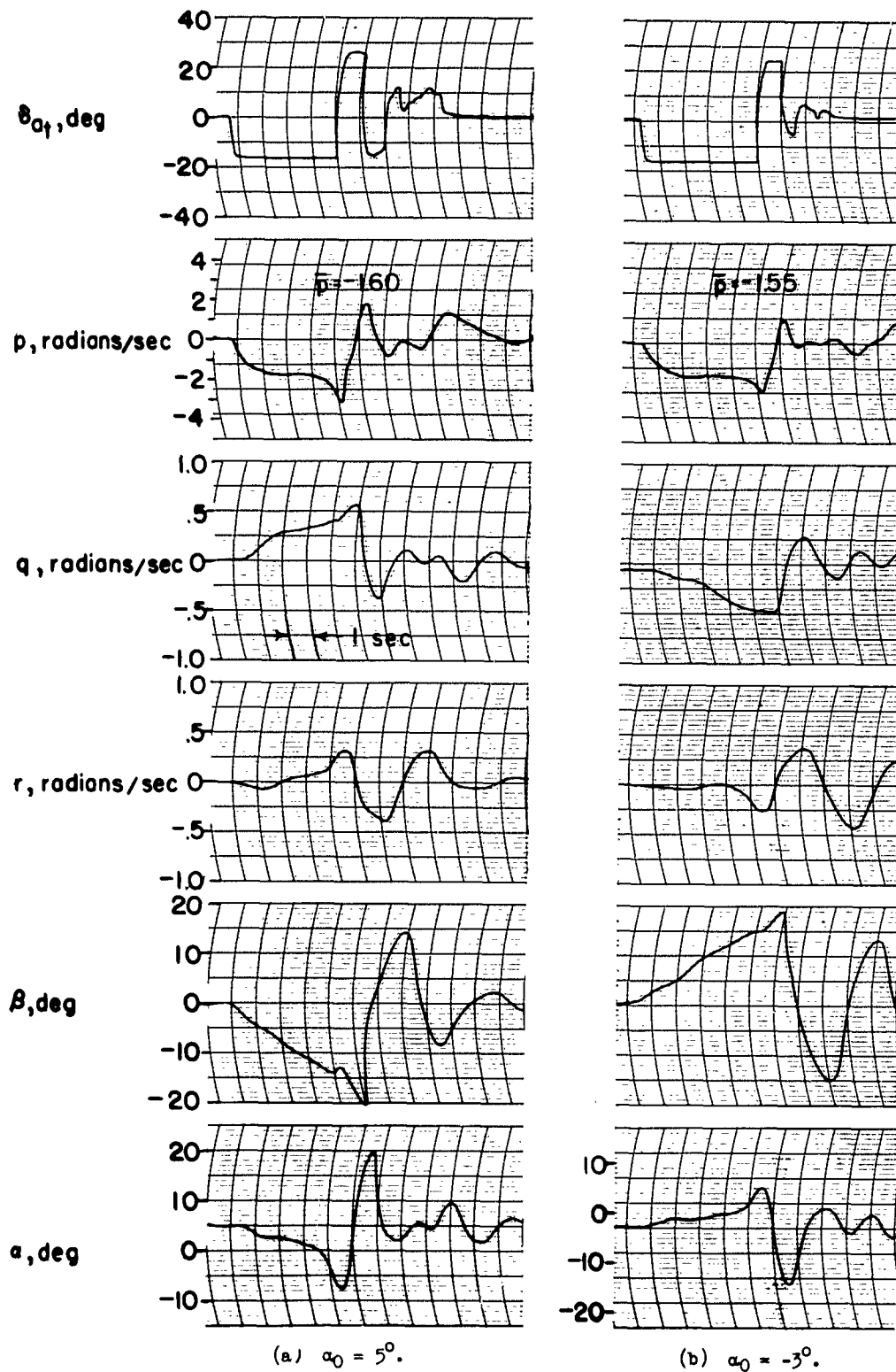
Figure 37.- Time histories showing effects of different initial angles of attack. Swept-wing configuration. \epsilon = 1^\circ .
