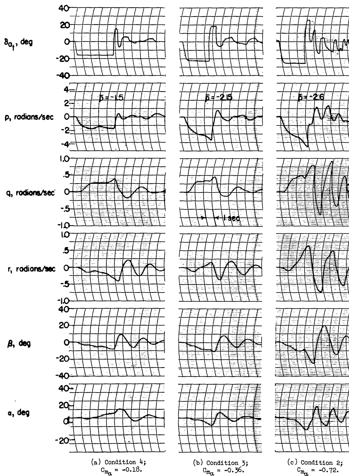
Figure 9.- Representative time histories for swept-wing configuration. Input B; C_{n\beta} = 0.114 .
