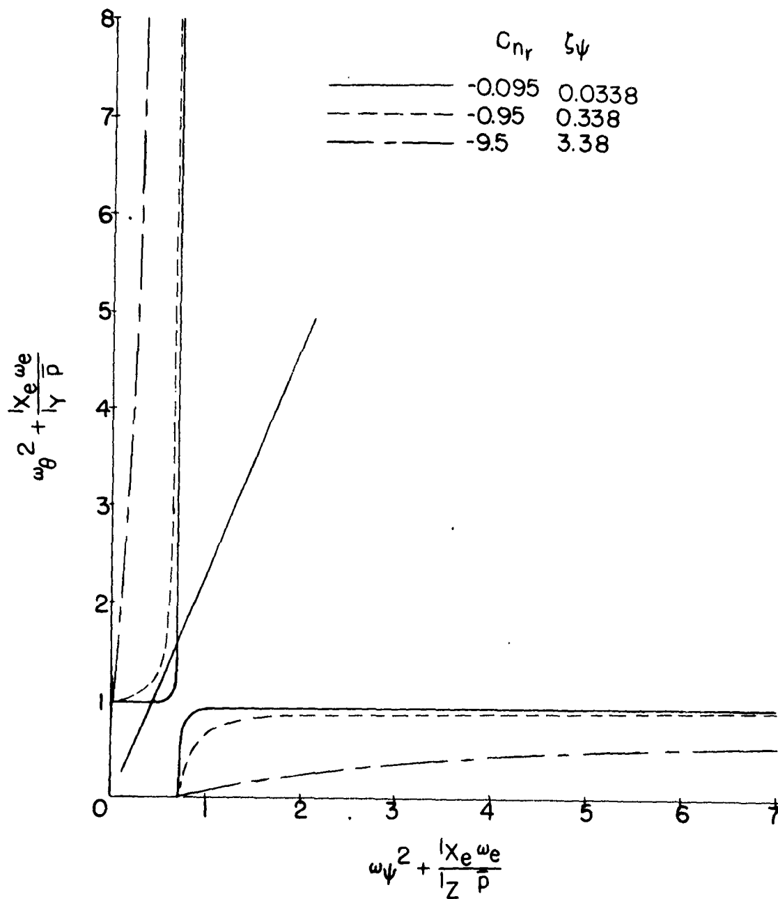
Figure 23.- Stability chart illustrating effects of increasing C_{nr} . Swept-wing configuration. Left rolls.
