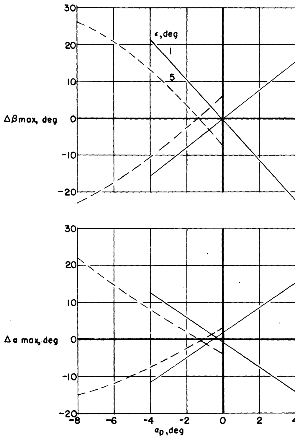
Figure 39.- Variation of peak motions with initial angle of attack of principal axis. Swept-wing configuration.
