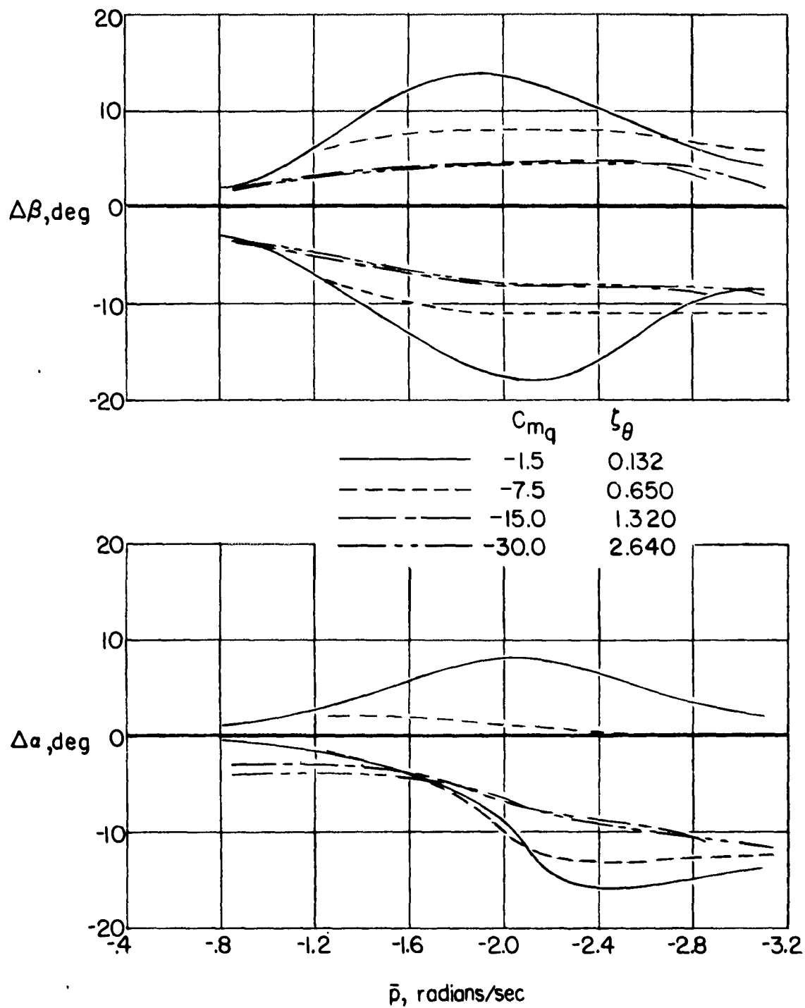
Figure 30.- Effect of increasing C_{mq} . Delta-wing configuration.
