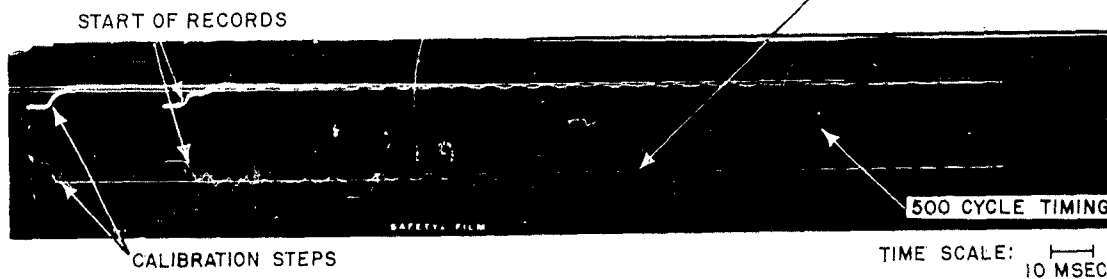
2d INDUCTANCE GAGE RECORD-LOW SPEED
