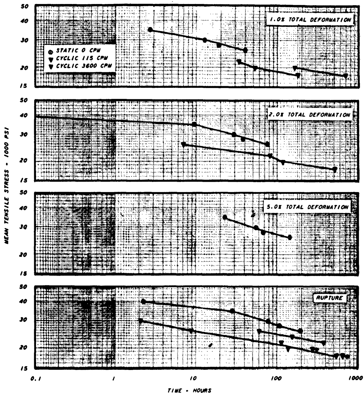
Figures 5 STRESS-TIME RELATIONSHIPS OF ANNEALED LOW CARBON N-155 SHEET DYNAMICALLY STRESSED AT 1350°F FOR STRESS AMPLITUDES OF 0 AND 67% AT VARIOUS STRESSING FREQUENCIES.
