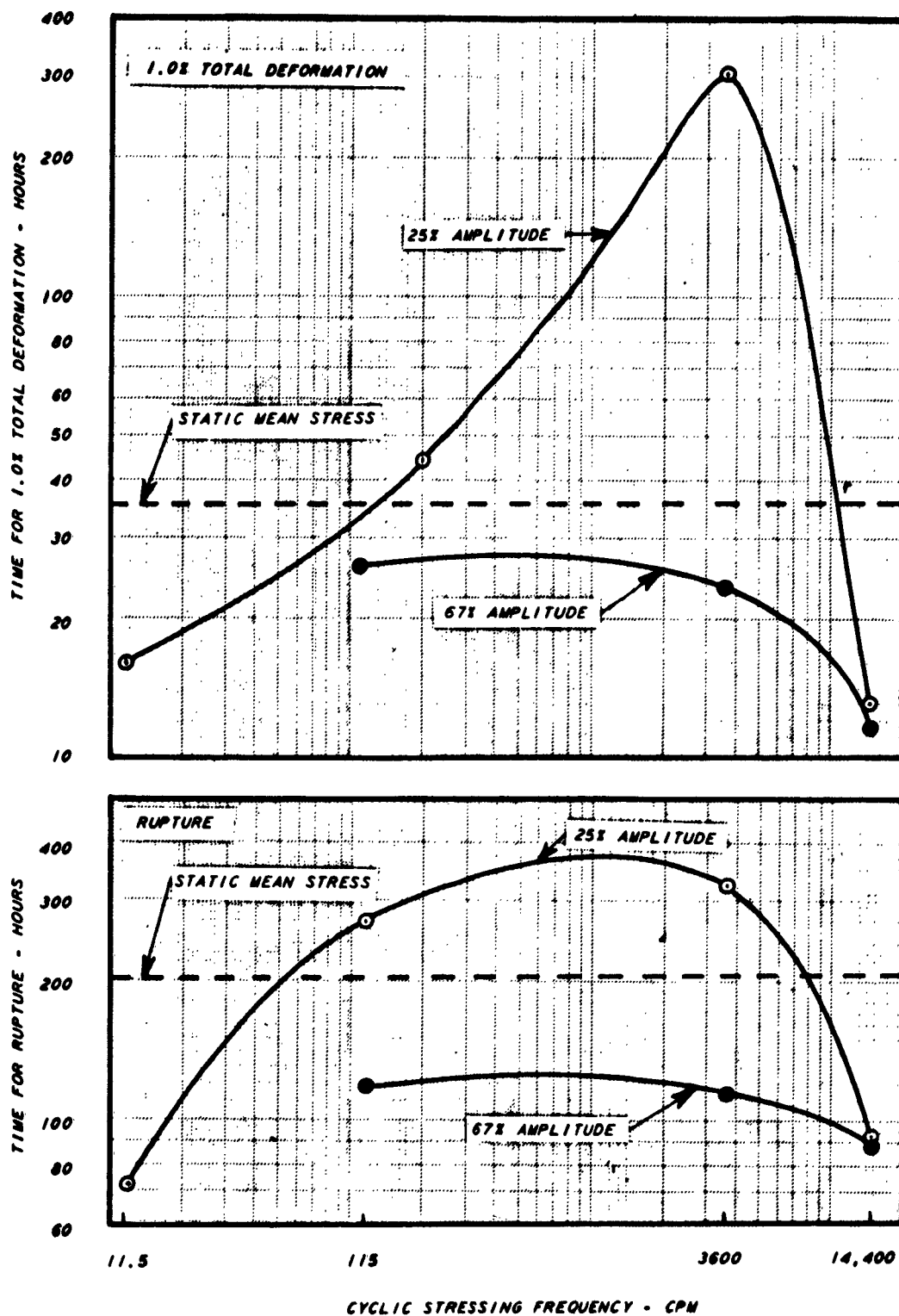
Figure 28 EFFECT OF CYCLIC STRESSING FREQUENCY AND AMPLITUDE ON THE DEFORMATION AND RUPTURE CHARACTERISTICS OF TYPE 321 STAINLESS STEEL SHEET AT 1500°F FOR A CONSTANT MEAN STRESS OF 5000 PSI
