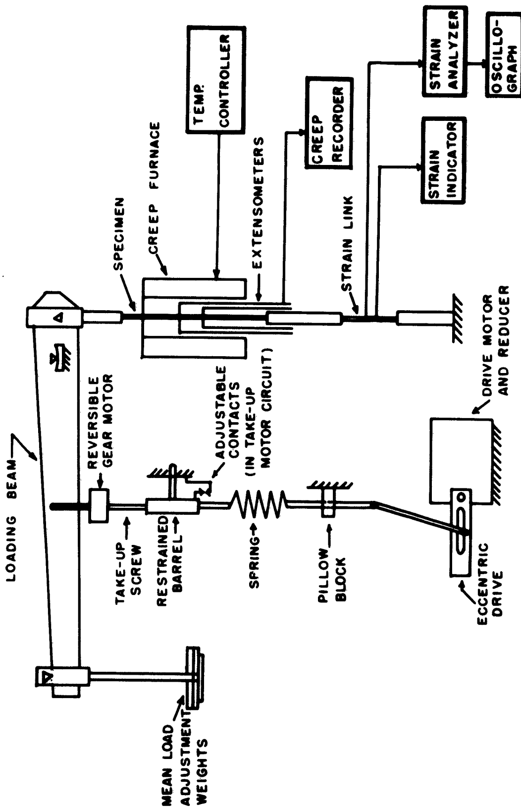
FIGURE 2 SCHEMATIC DIAGRAM OF 11.5 & 115 CPM. CYCLIC STRESS TEST UNITS
