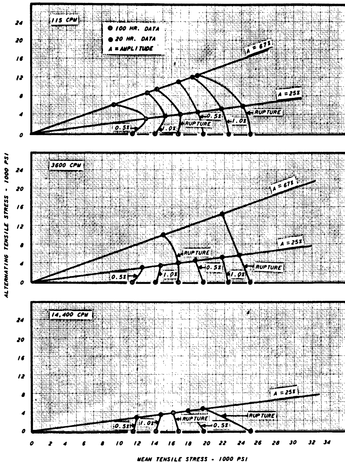
Figure 16 STRESS COMBINATIONS AT VARIOUS FREQUENCIES FOR TOTAL DEFORMATION AND RUPTURE OF AGED INCONEL X SHEET AT 1500°F
