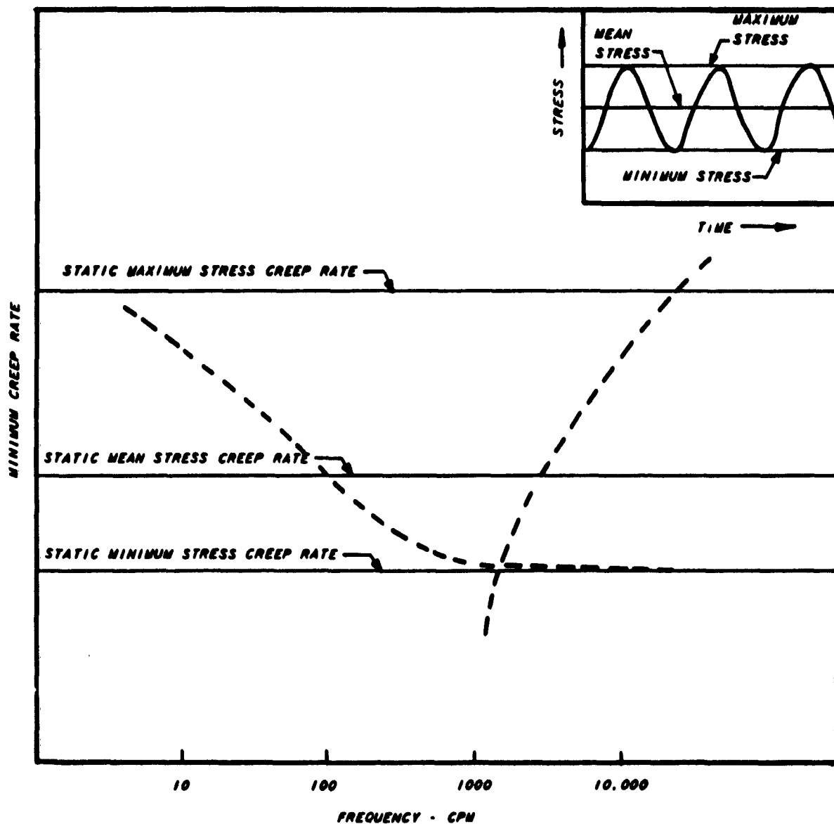
Figure 22 SCHEMATIC REPRESENTATION OF CREEP RATE vs. FREQUENCY OF AN ALLOY AT CONSTANT TEMPERATURE, CONSTANT MEAN STRESS, AND CONSTANT AMPLITUDE
