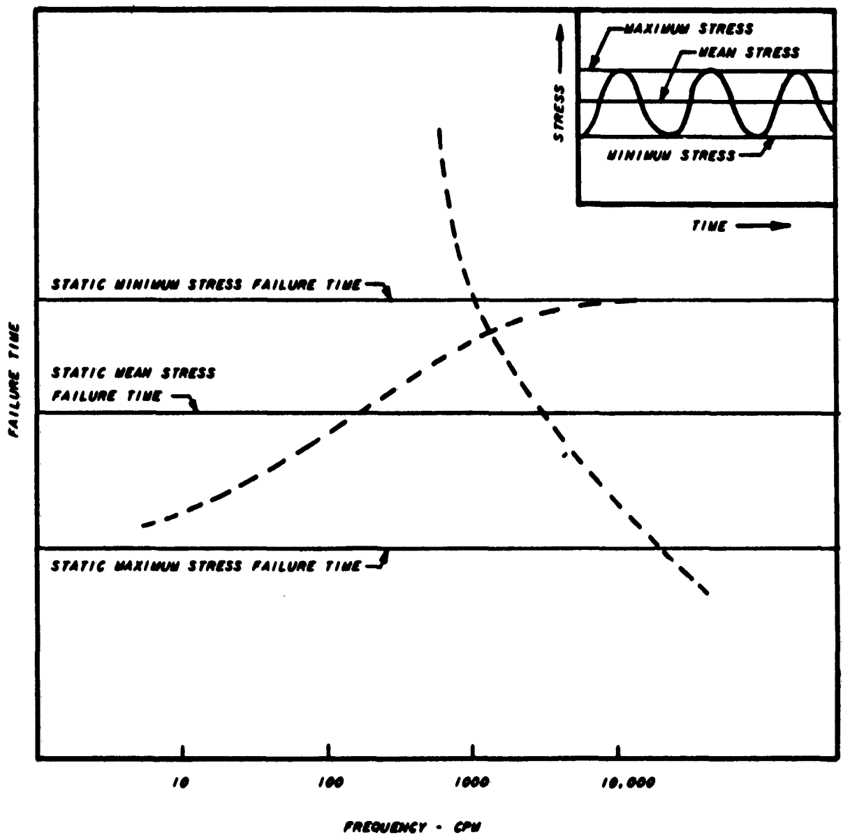
Figure 23 SCHEMATIC REPRESENTATION OF FAILURE TIME Vs. FREQUENCY OF AN ALLOY AT CONSTANT TEMPERATURE, CONSTANT MEAN STRESS, AND CONSTANT AMPLITUDE
