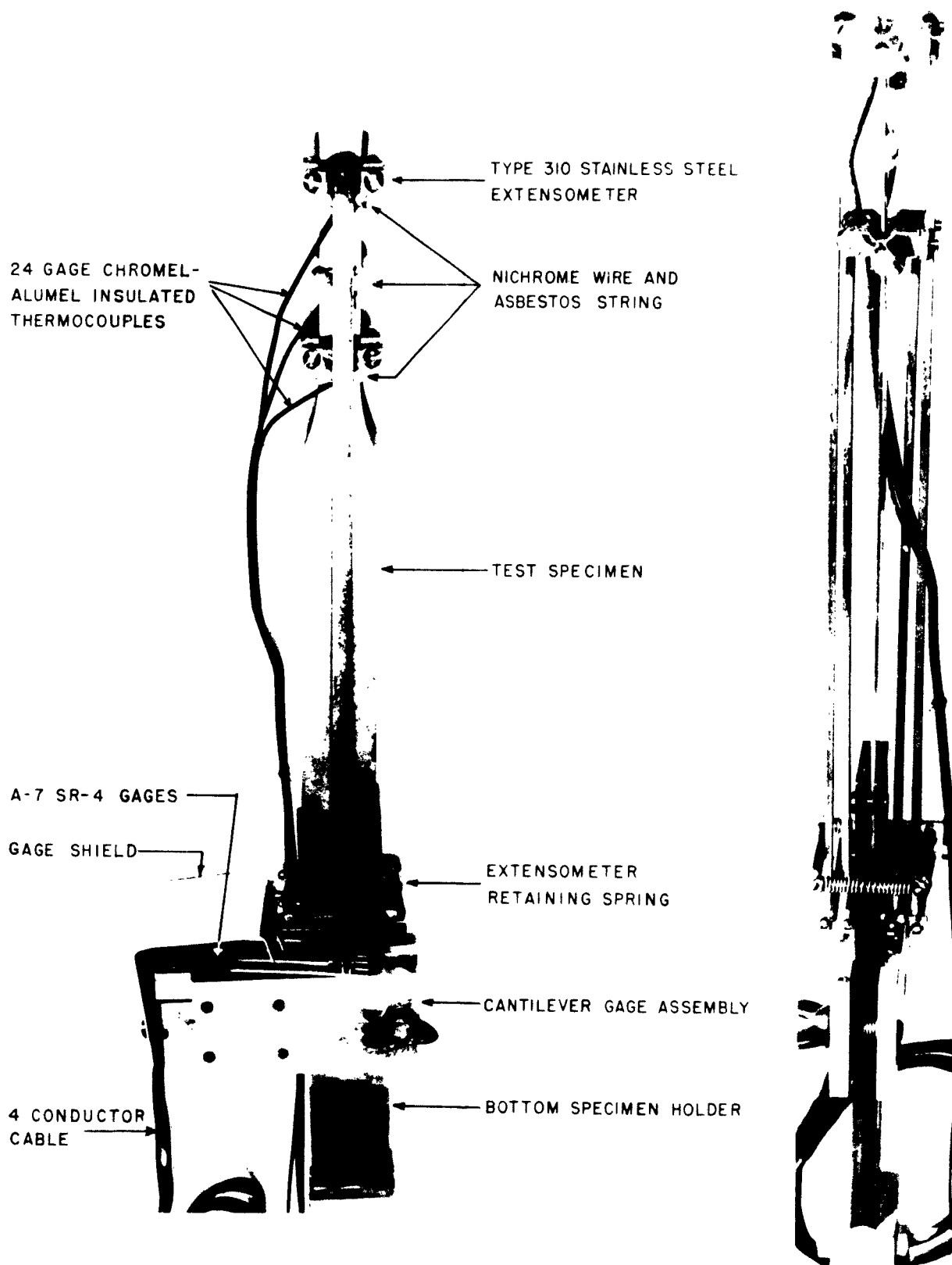
FIGURE 1 SPECIMEN - EXTENSOMETER - THERMOCOUPLE ASSEMBLY
