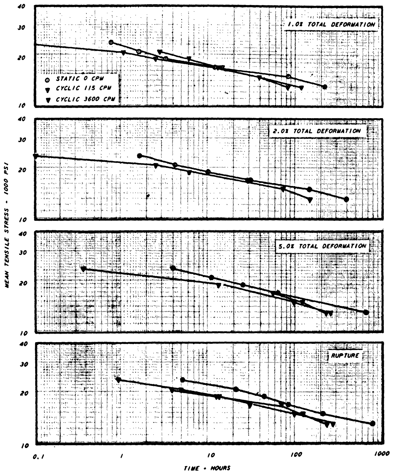
Figure 7 STRESS-TIME RELATIONSHIPS OF ANNEALED LOW CARBON N-155 SHEET DYNAMICALLY STRESSED AT 1500°F FOR STRESS AMPLITUDES OF 0 AND 67% AT VARIOUS STRESSING FREQUENCIES.
