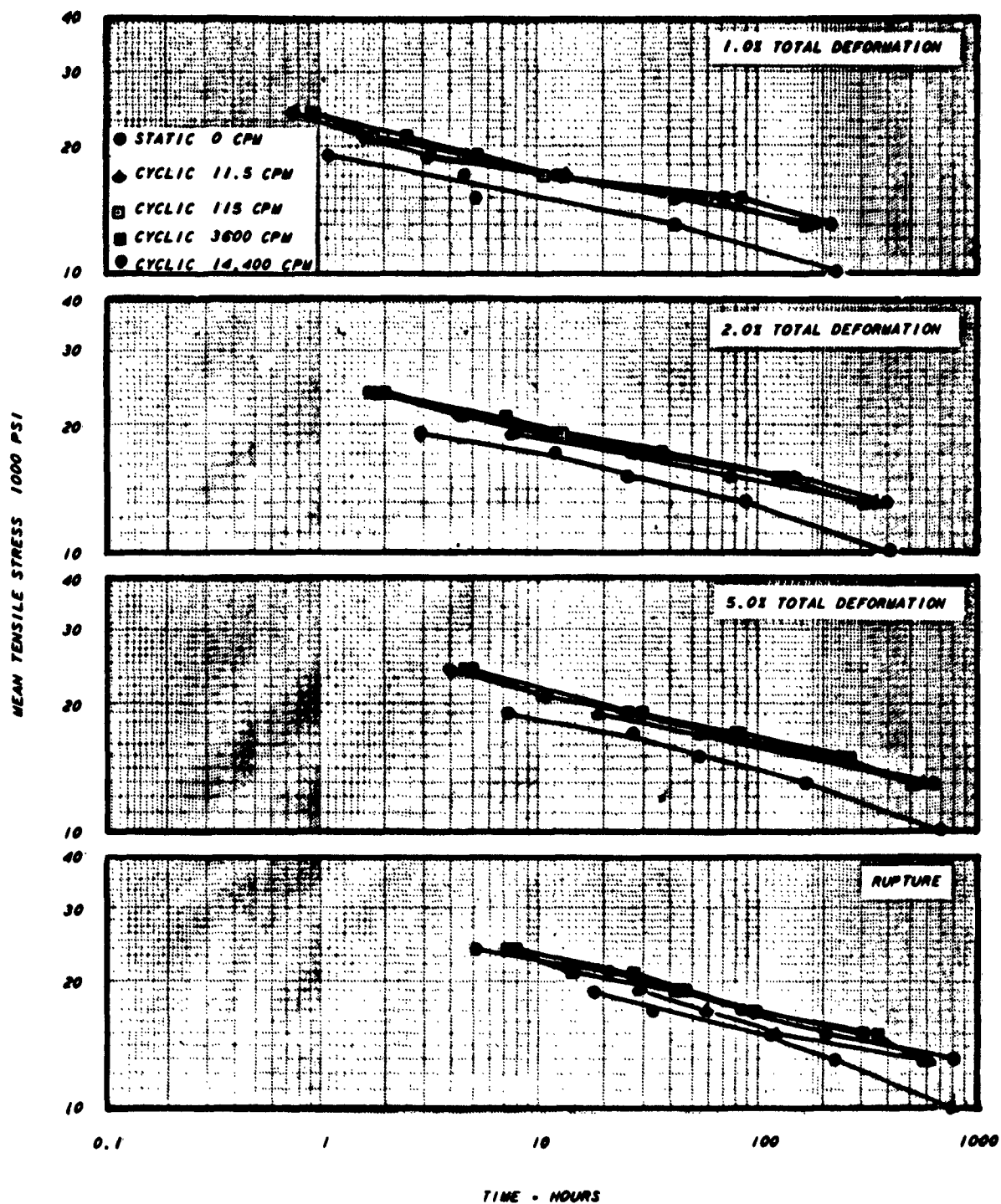
Figure 6 STRESS-TIME RELATIONSHIPS OF ANNEALED LOW CARBON N-155 SHEET DYNAMICALLY STRESSED AT 1500°F FOR STRESS AMPLITUDES OF 0 AND 25% AT VARIOUS STRESSING FREQUENCIES
