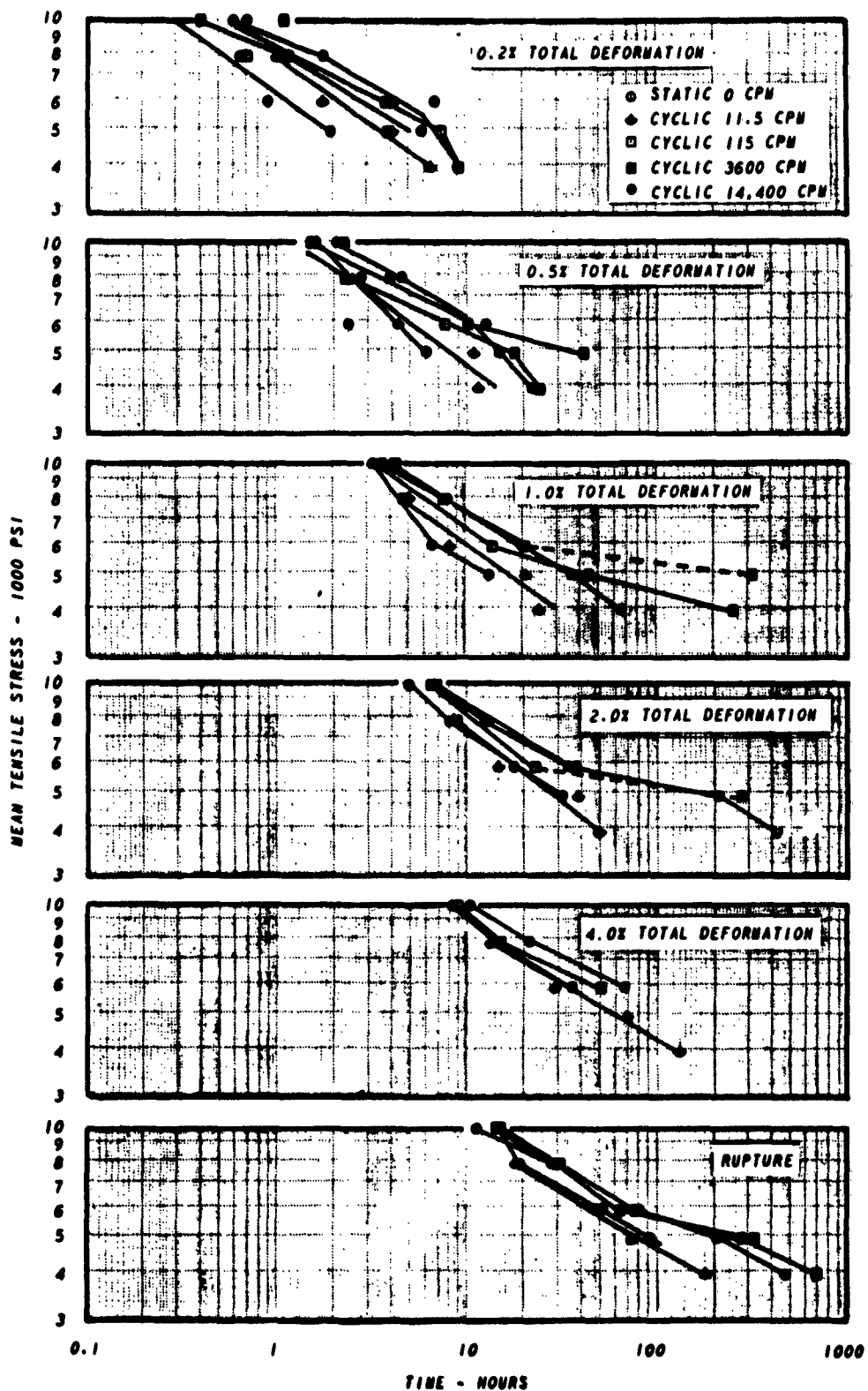
Figure 10 STRESS-TIME RELATIONSHIPS OF TYPE 321 STAINLESS STEEL SHEET DYNAMICALLY STRESSED AT 1800°F FOR STRESS AMPLITUDES OF 0 AND 25% AT VARIOUS STRESSING FREQUENCIES
