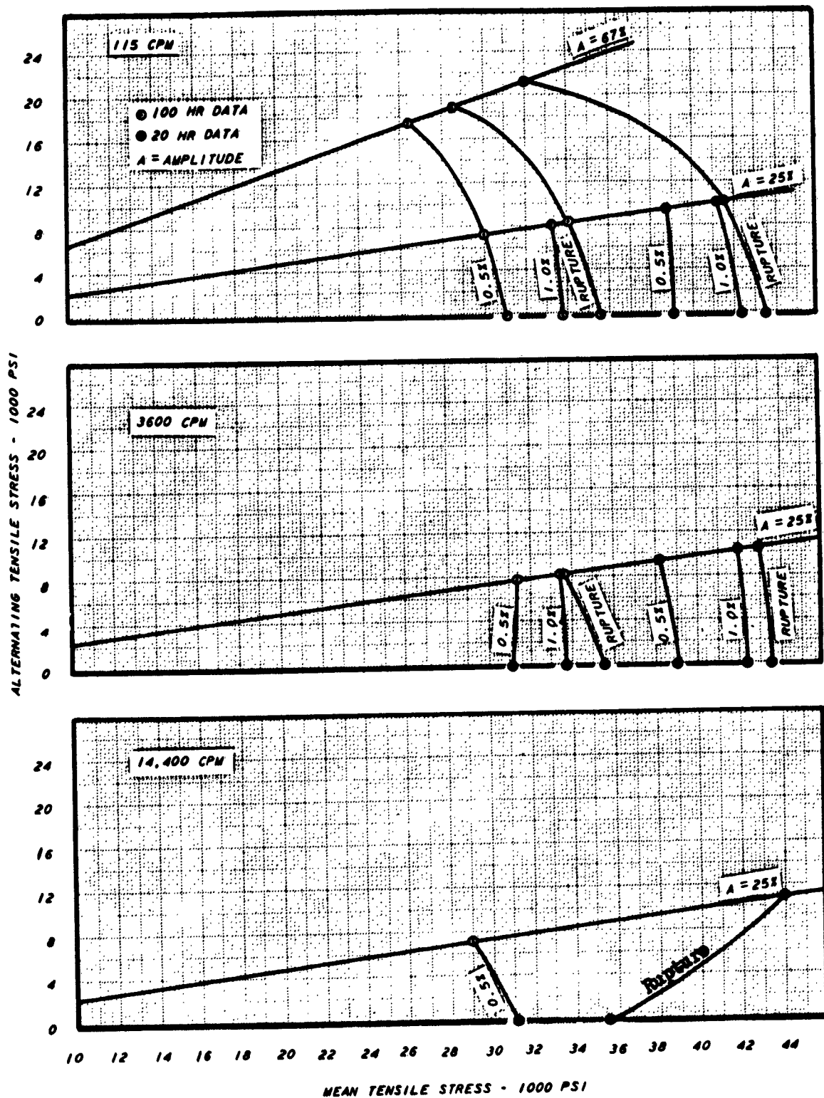
Figure 15 STRESS COMBINATIONS AT VARIOUS FREQUENCIES FOR TOTAL DEFORMATION AND RUPTURE OF AGED INCONEL X SHEET AT 1350°F
