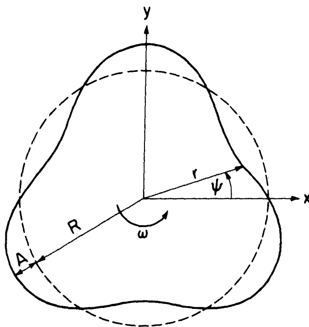
Figure 3.- Cross section of the cylinder corrugated by m = 3 waves.
