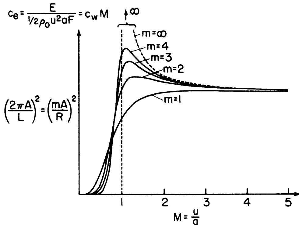
Figure 5.- Energy radiation for rotation of the wavy cylinder.
