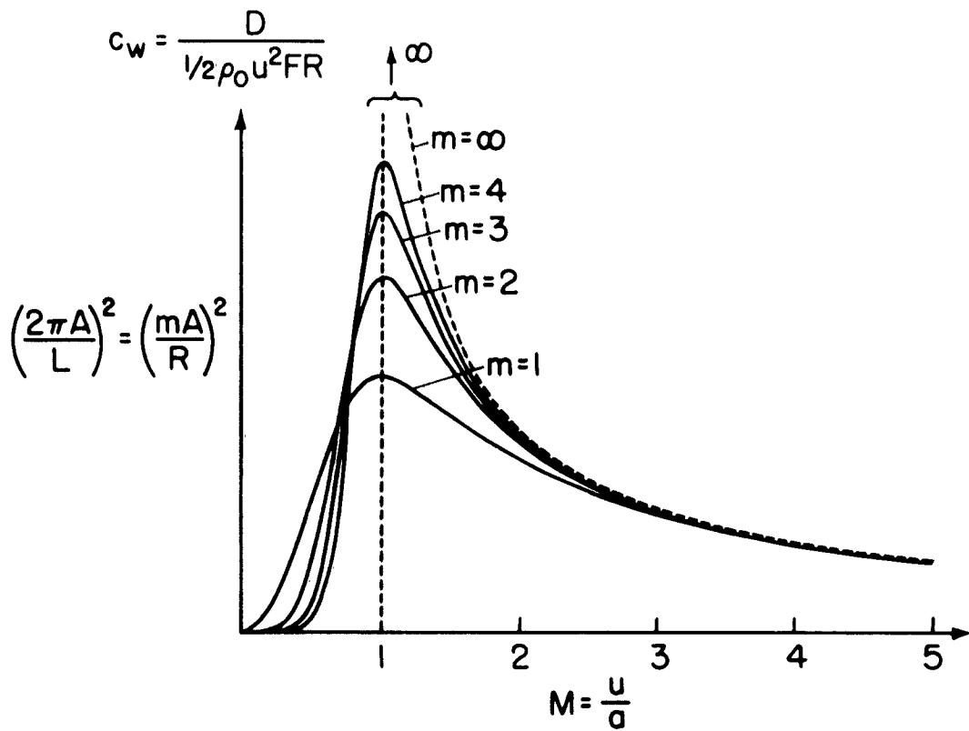
Figure 4.- Resistance for rotation of the wavy cylinder.
