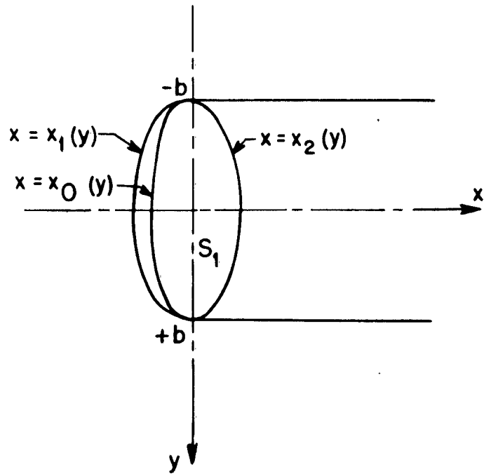
Figure 2.- Location of the bound vortex line and areas of integration.
