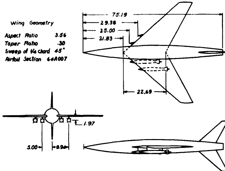
Figure 1.- Configuration utilized as a basis for equivalent body tests in part I of the current investigation. All dimensions are in inches.
