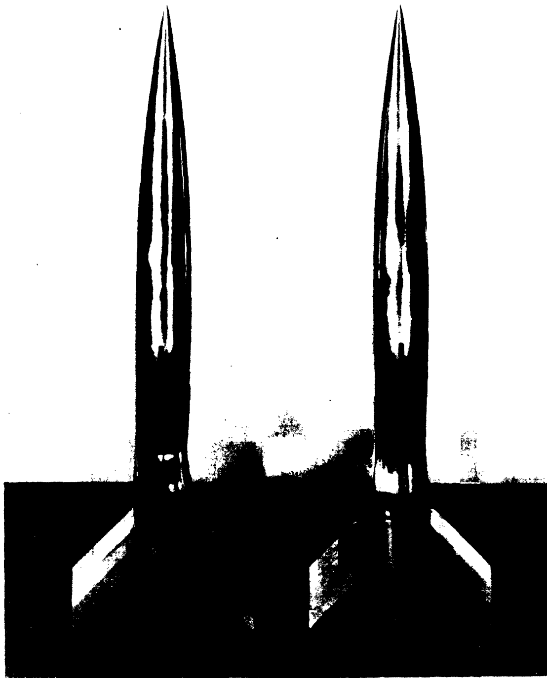
Figure 7.- Photograph of models 6 and 7 showing fuselage indentations and typical construction details.
