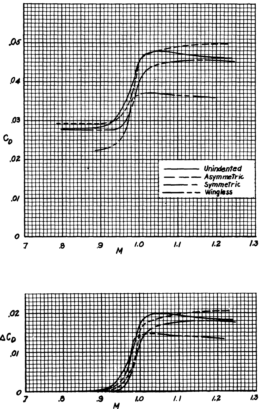
Figure 12.- Drag coefficient and pressure drag coefficient for part II models.
