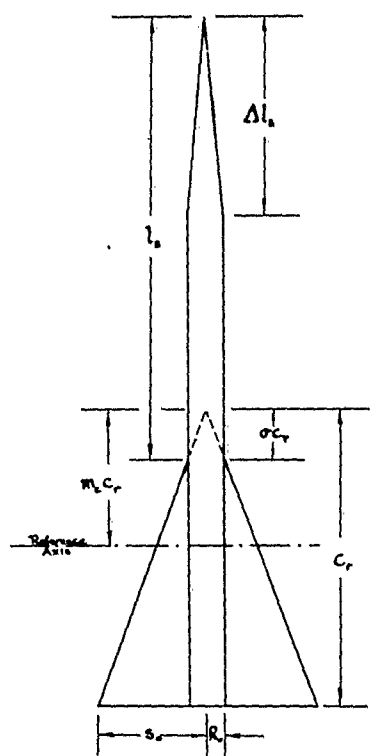
WING-BODY COMBINATION
