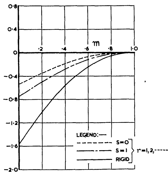
DAMPING DERIVATIVE m_z FOR TRIANGULAR WING
