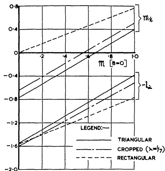
'CROSS' DAMPING DERIVATIVES FOR RIGID WINGS
