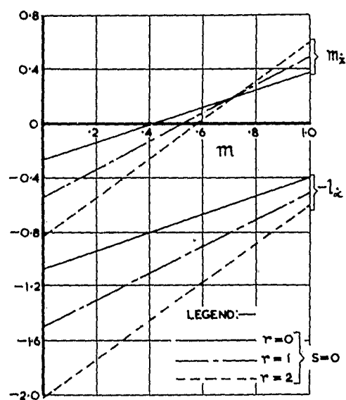
'CROSS' DAMPING DERIVATIVES FOR DEFORMING WING [ \lambda=0 ]
