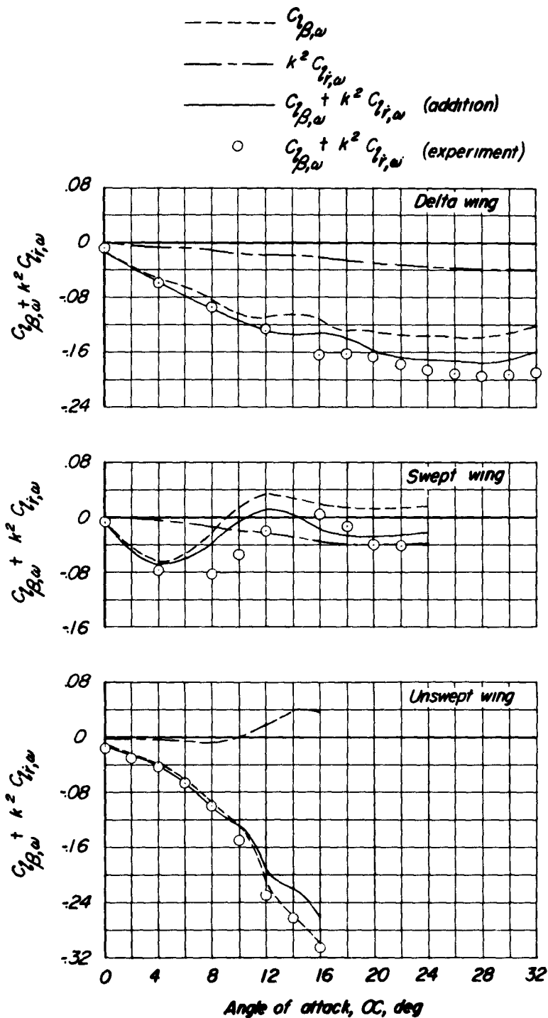
Figure 22.- Comparison of the component and the combination derivatives making up the effective dihedral. \omega b/2V = 0.22 ; \psi_0 = 6^\circ or 8^\circ .
