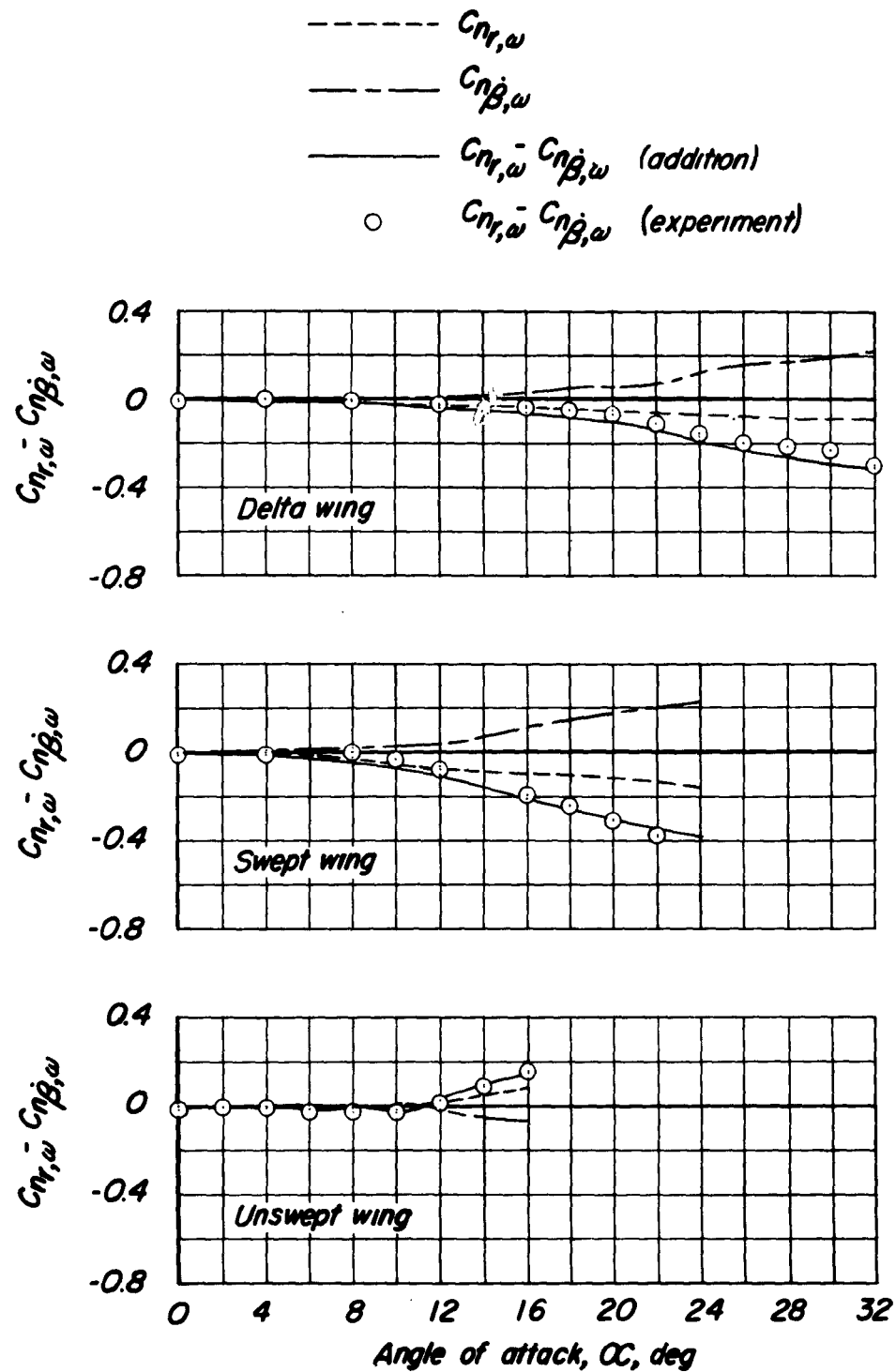
Figure 19.- Comparison of the component and the combination derivatives making up the damping in yaw. \omega b/2V = 0.22 ; \psi_0 = 6^\circ or 8^\circ .
