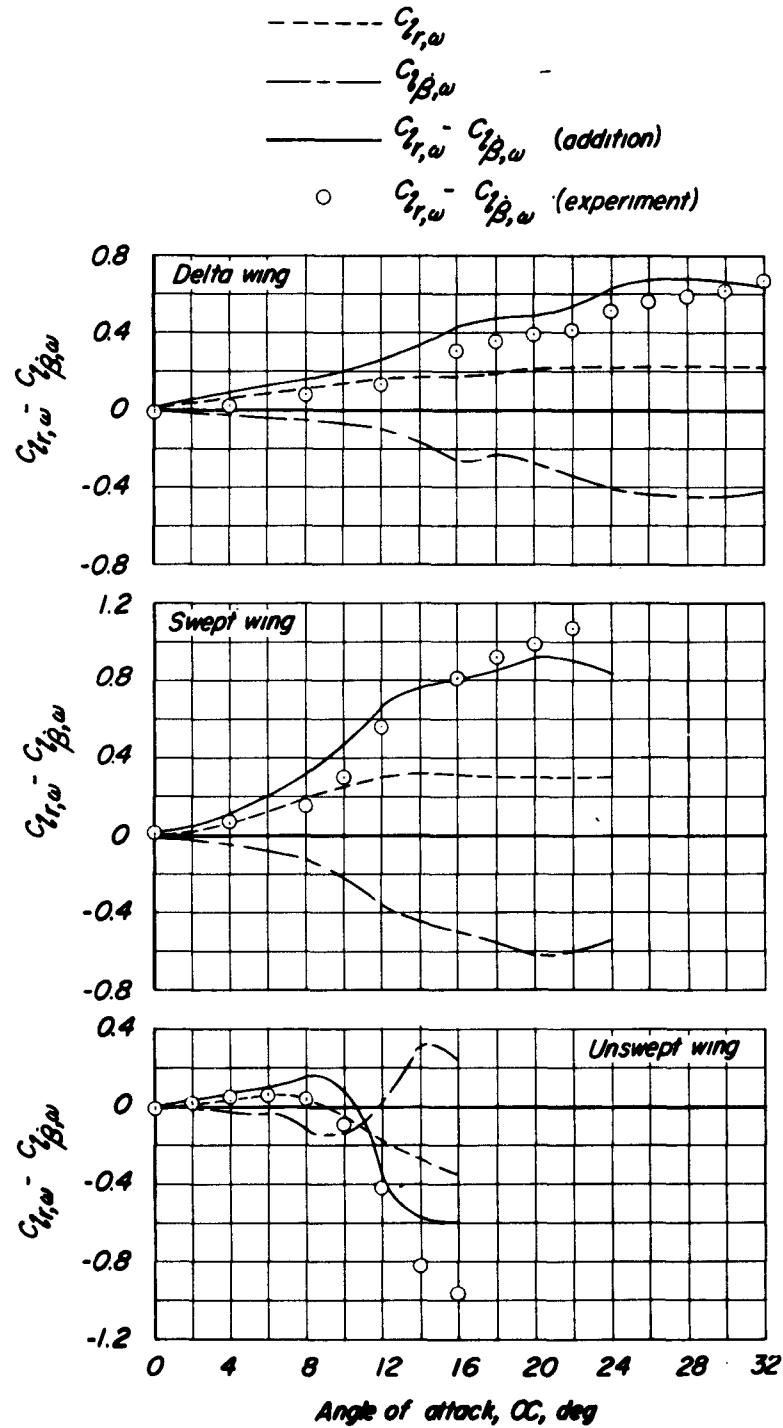
Figure 20.- Comparison of the component and the combination derivatives making up the rolling moment due to yawing. \omega b/2V = 0.22 ; \psi_0 = 6^\circ or 8^\circ .
