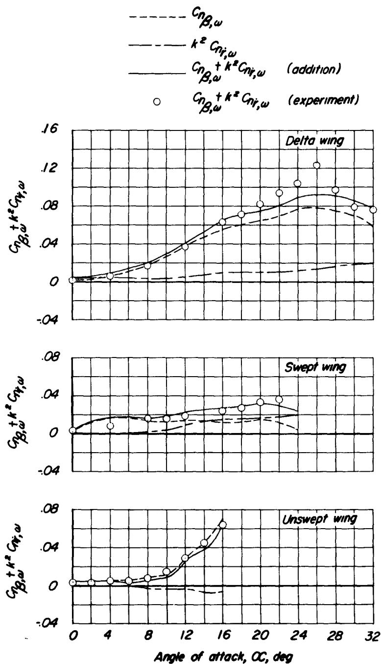
Figure 21.- Comparison of the component and the combination derivatives making up the directional stability \omega b/2V = 0.22 ; \psi_0 = 6^\circ or 8^\circ .
