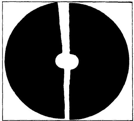
NI/CR BONDED TIC (CARBOMETAL) x3 \Delta T = 1000^{\circ}\text{C} h = 0.04 \text{ ch.u./ft}^2\text{s}^{\circ}\text{C} 10 CYCLES.
