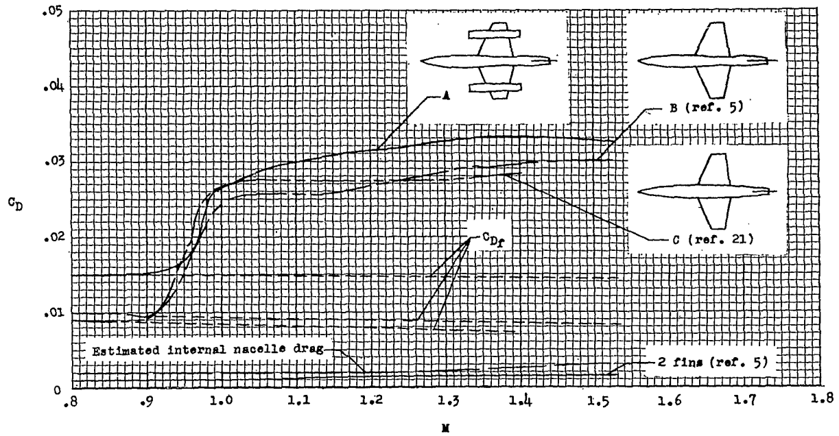
(a) Total drag.
