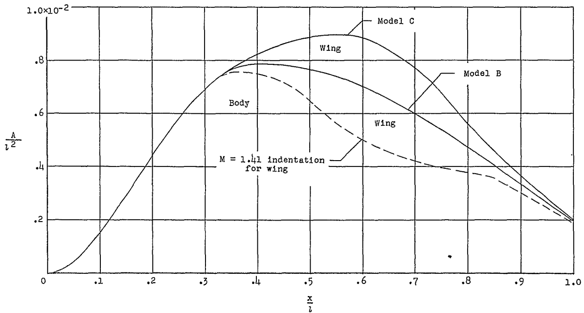
(d) Average area distributions for M = 1.41 . Models B and C.
