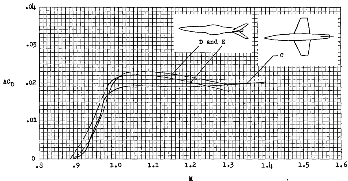
(b) Pressure drag.
