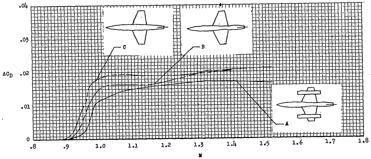
(b) Pressure drag.
