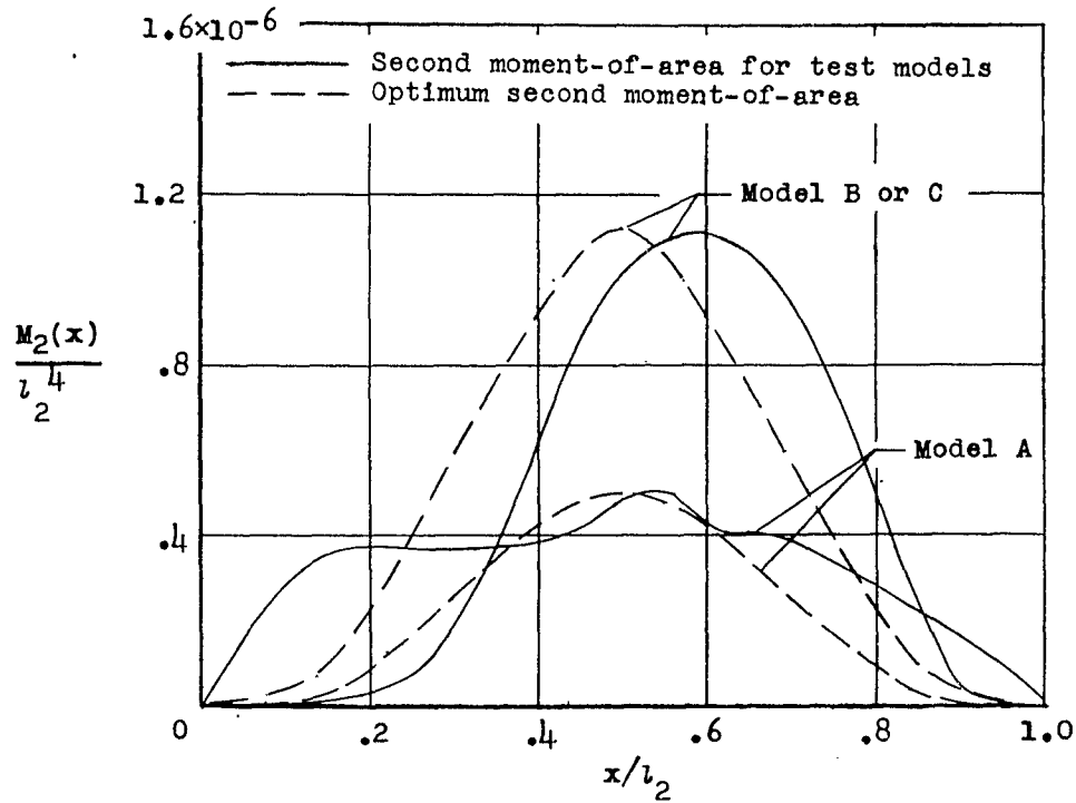
(a) Nondimensionalized area moment of inertia distribution.
