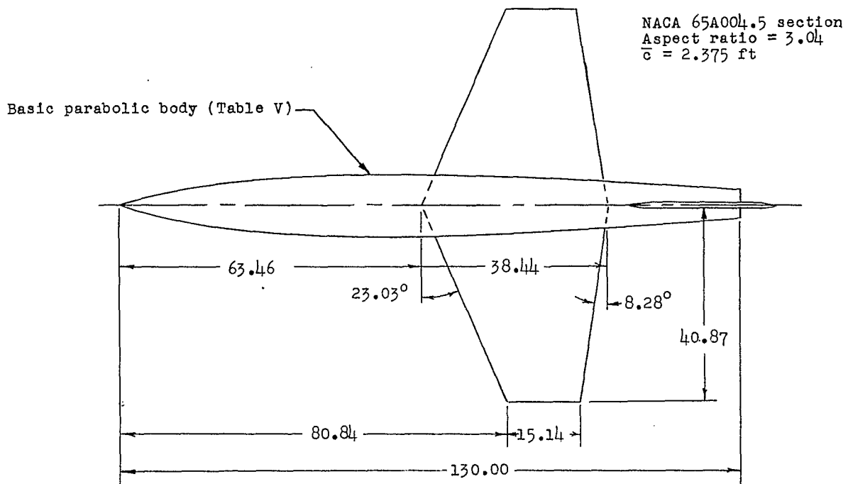
(c) Basic wing-body configuration (ref. 21). Model C.
