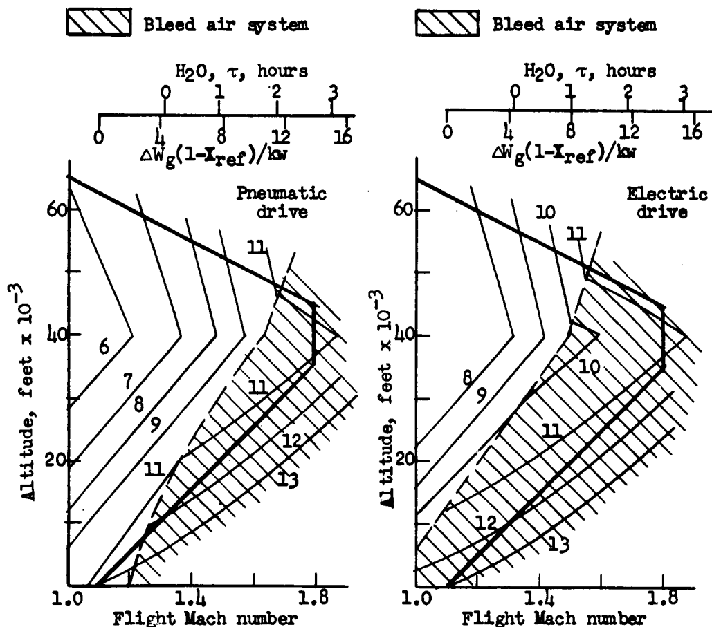
Figure II-51. Gross weight penalty of indirect bleed air versus indirect vapor cycle cooling systems with electric or pneumatic drive. T_{Es} = 590^{\circ}\text{R} . \alpha = 2 . L_D = 200 feet.
