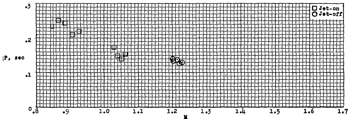
Figure 24.- Variation of the period of the short period pitching oscillations with Mach number for jet-on and jet-off flight.
