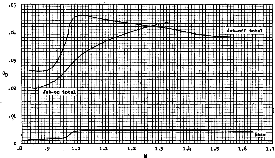
Figure 13.- The variation of jet-on, jet-off, and base drag coefficients with Mach number.
