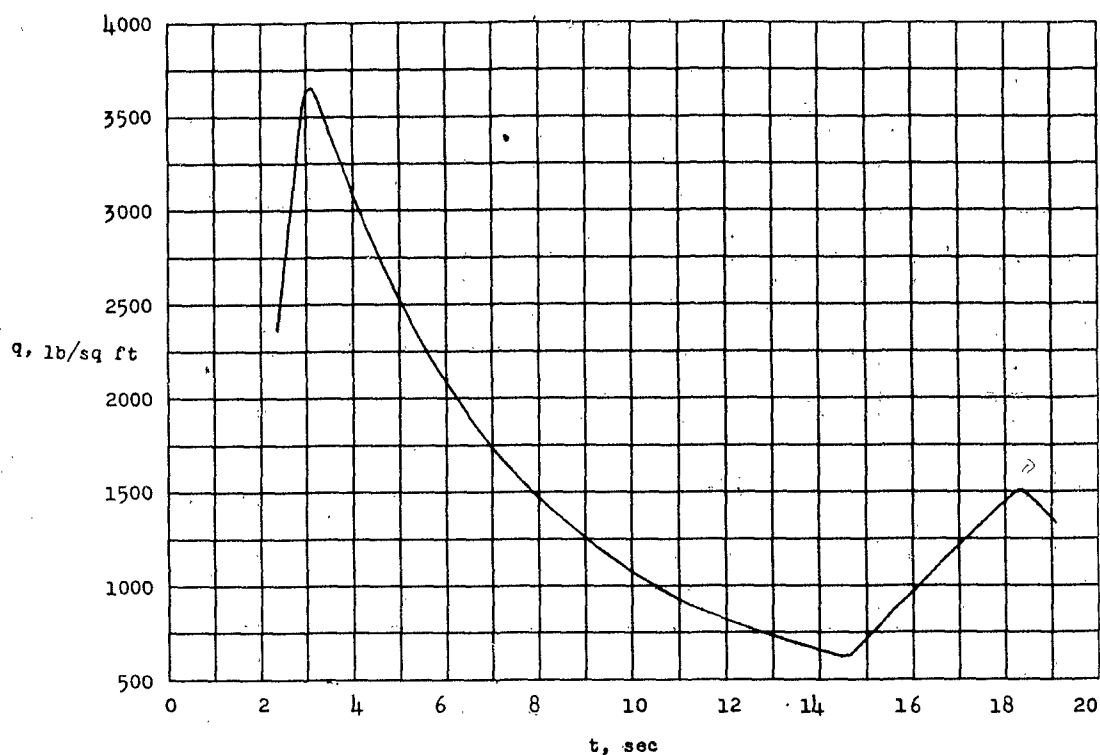
Figure 9.- Variation of dynamic pressure with time.
