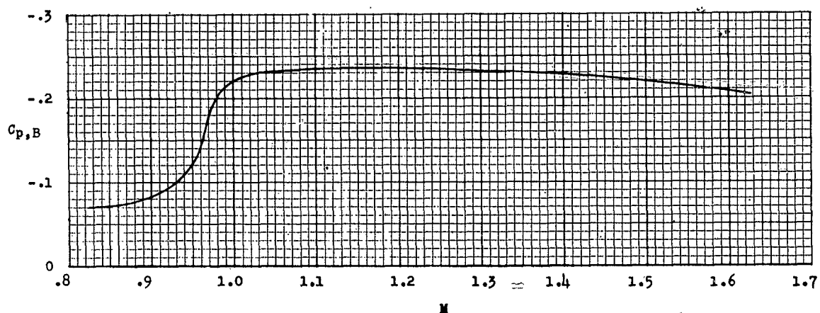
Figure 19.- The variation of the base pressure coefficient of the engine pod with Mach number.
