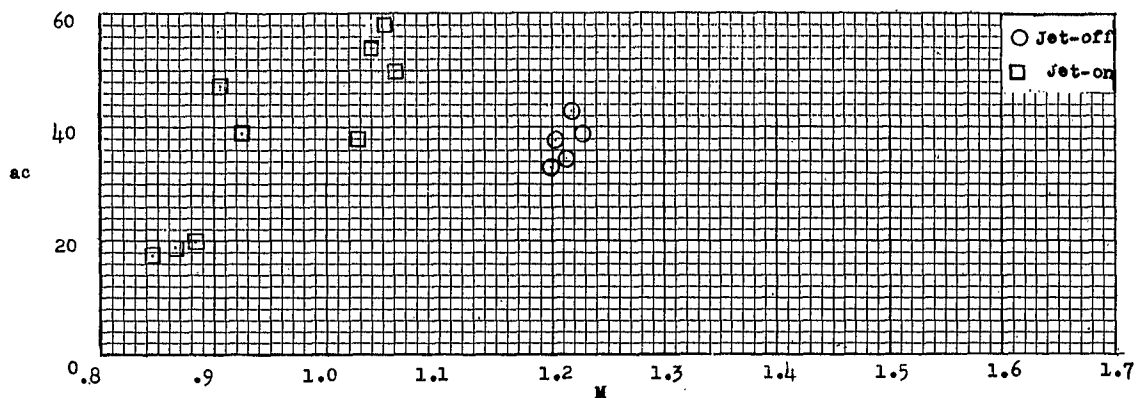
Figure 26.- Variation of aerodynamic center with Mach number for jet-on and jet-off flight.
