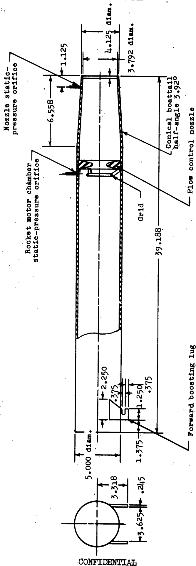
Figure 2.- Drawing of turbojet simulator. All dimensions are in inches.
