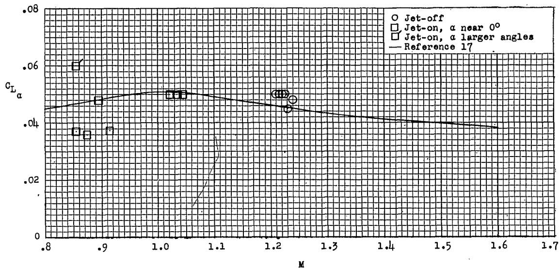
Figure 21.- The variation of lift-curve slope with Mach number.
