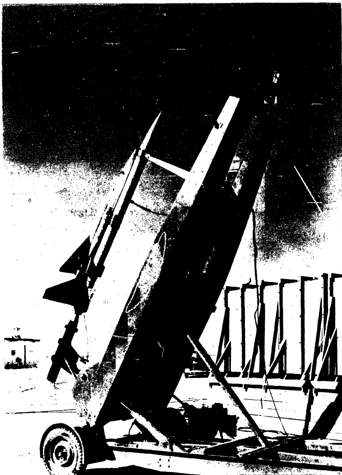
Figure 5.- Model and booster on mobile launcher. L-89053.1
