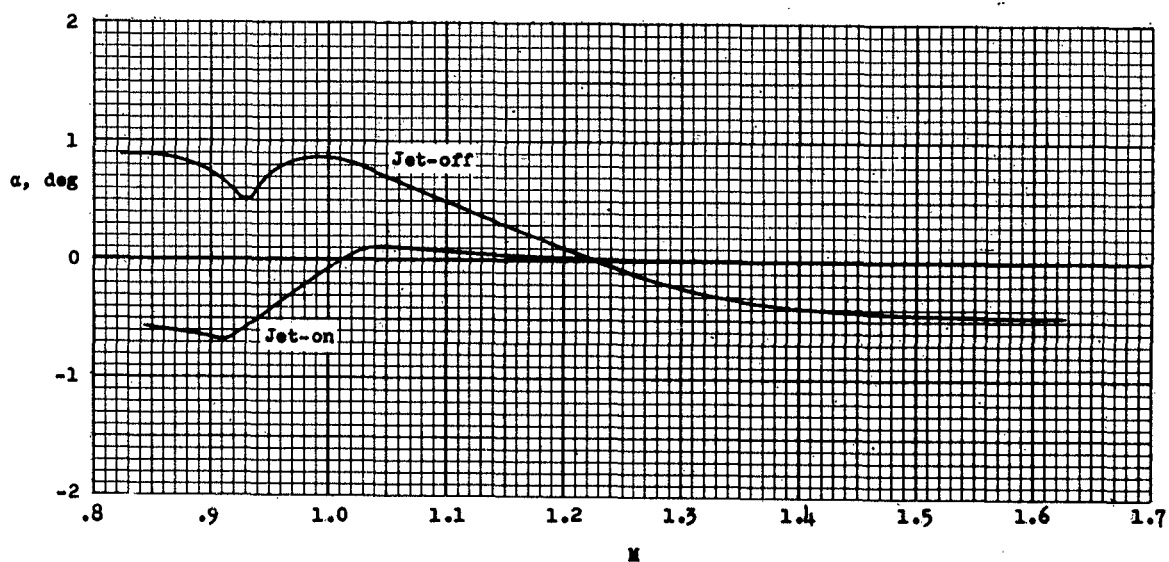
Figure 14.- The variation of trim angle of attack for jet-on and jet-off flight with Mach number.
