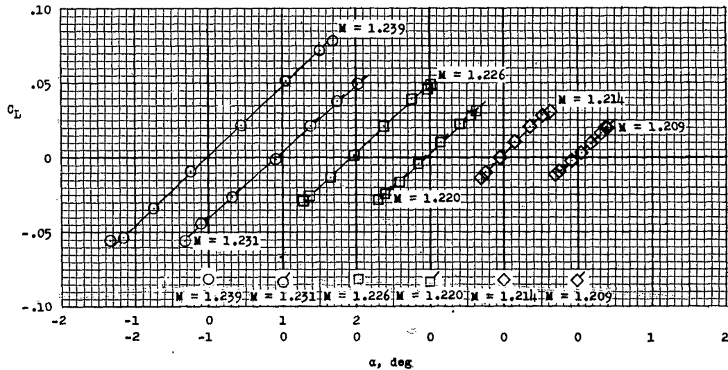
(b) Jet-off lift coefficients.
