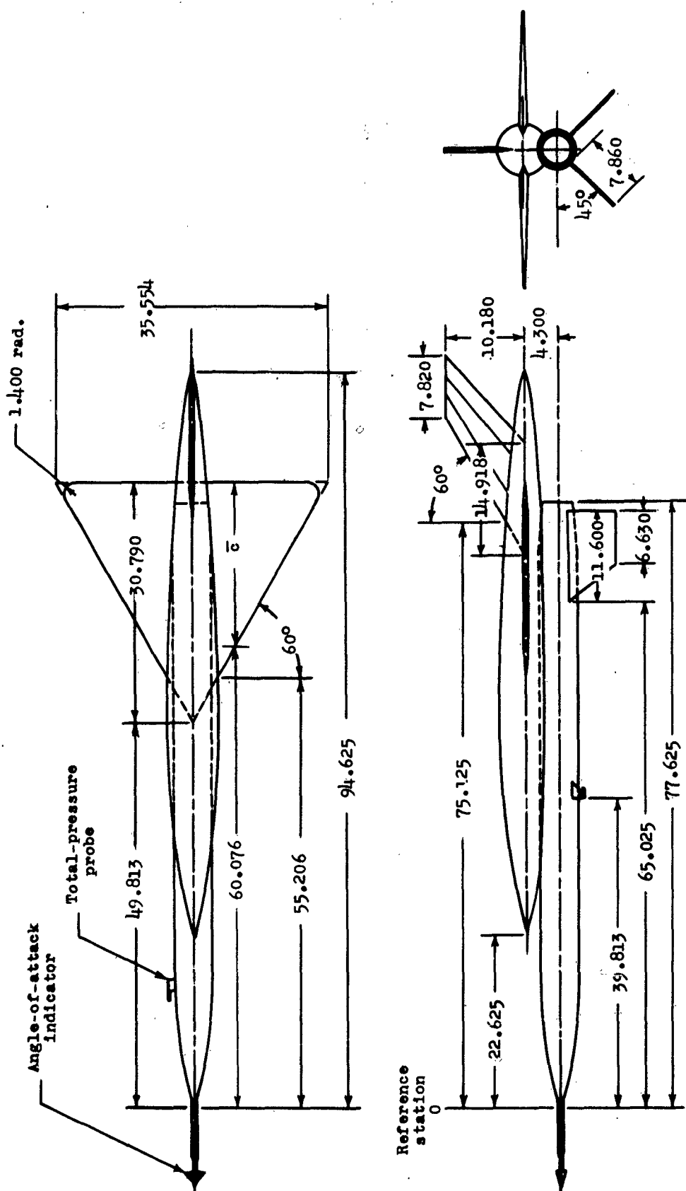
Figure 1.- Three-view drawing of the flight test model. All dimensions are in inches.
