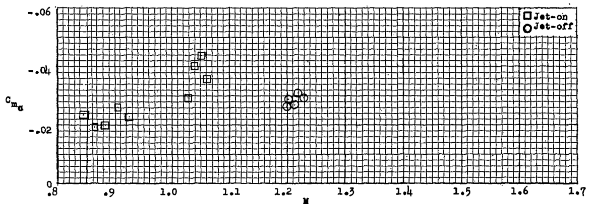
Figure 25.- Variation of static-stability derivative with Mach number for jet-on and jet-off flight.
