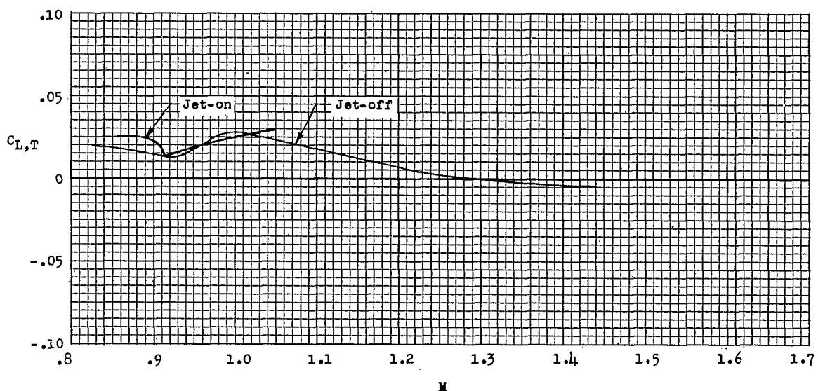
Figure 22.- The variation of trim-lift coefficient with Mach number.
