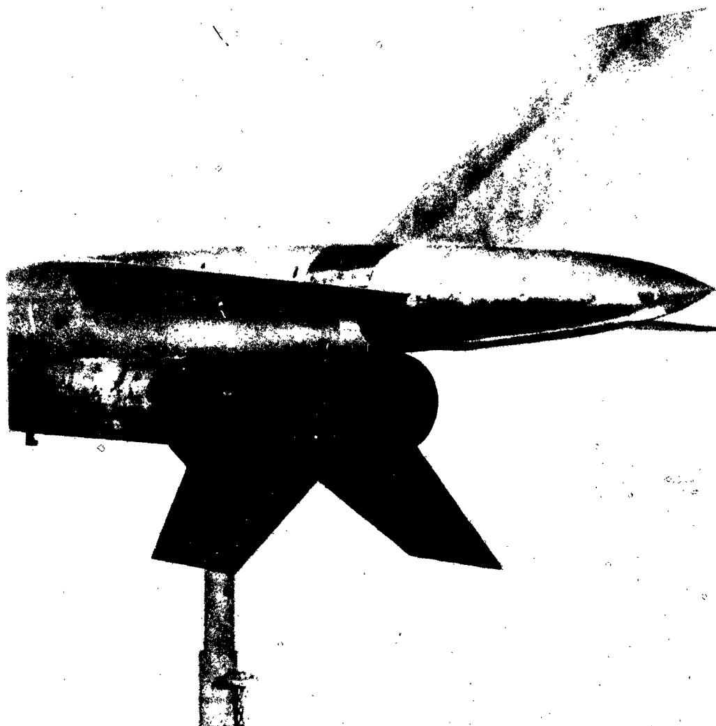
Figure 4.- Photograph of tail section of flight model. L-88340
