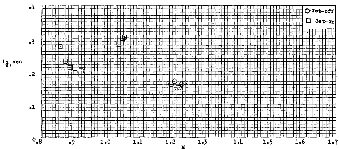
Figure 27.- Variation of the time to damp to one-half amplitude with Mach number for jet-on and jet-off flight.
