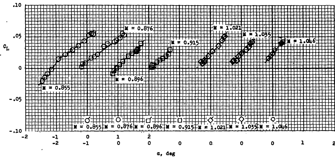
(a) Jet-on lift coefficients.
