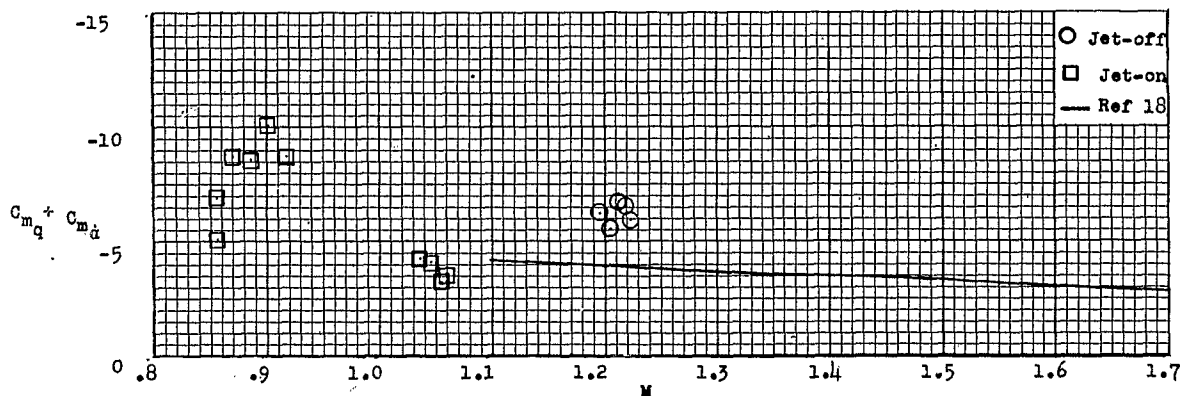
Figure 28.- Variation of damping derivatives with Mach number for jet-on and jet-off flight.
