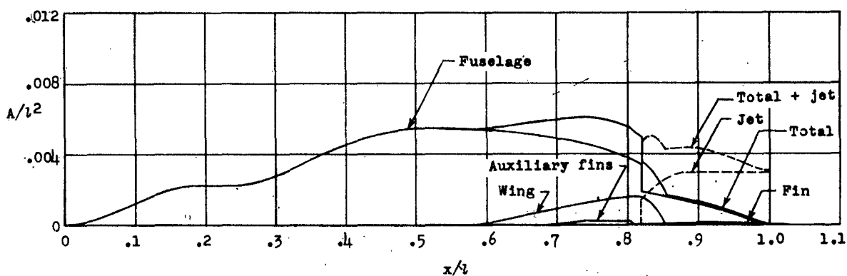
(c) Cross-sectional area distribution of the configuration with and without the jet.
