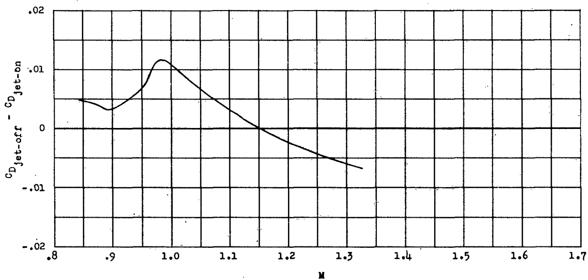
Figure 16.- The variation of the difference between jet-off and jet-on drag coefficients with Mach number.
