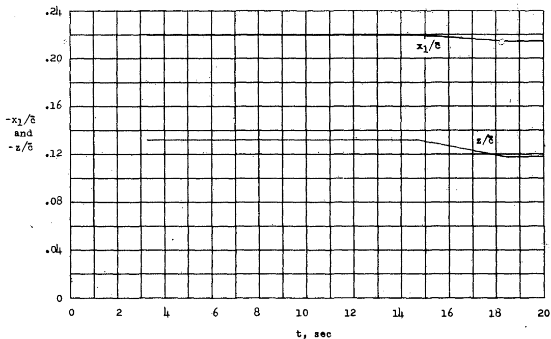
Figure 10.- The variation of center-of-gravity position, measured from the leading edge of the wing mean aerodynamic chord, with time.
