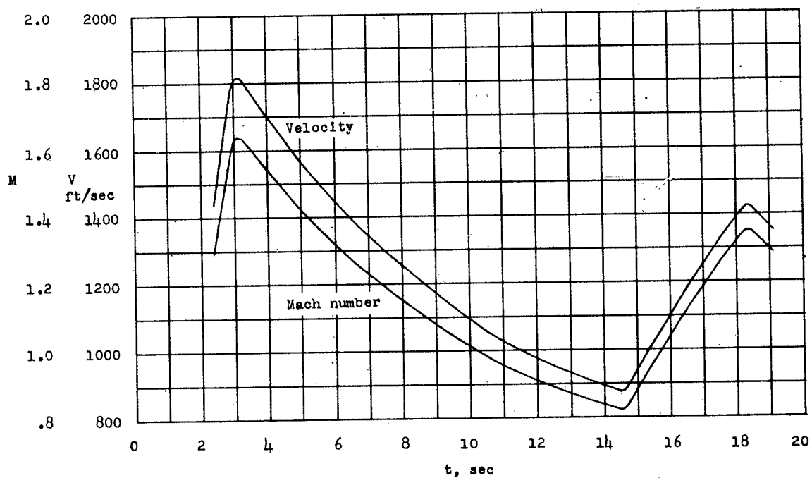
Figure 8.- Variation of model velocity and Mach number with time.
