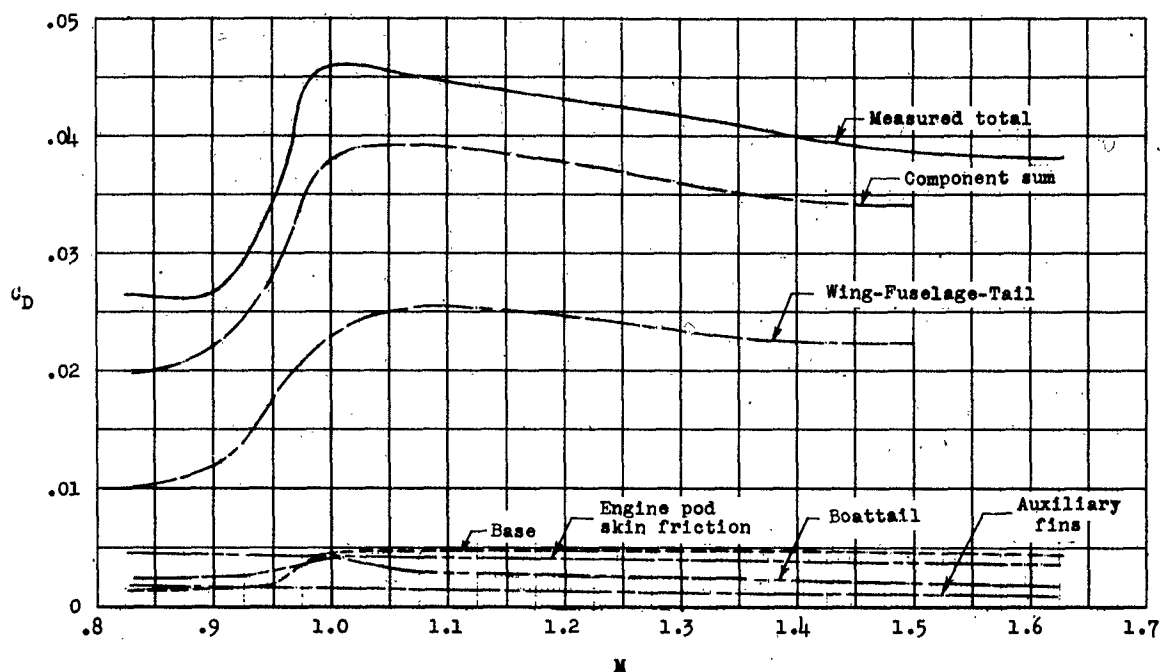
Figure 18.- The variation of the measured and estimated total-drag coefficients and the drag coefficients of the components with Mach number.
