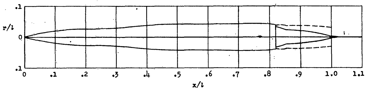
(b) Equivalent body of revolution for the configuration with and without the jet.
