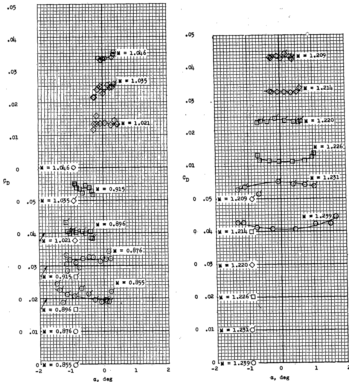
(a) Jet-on drag coefficients.
