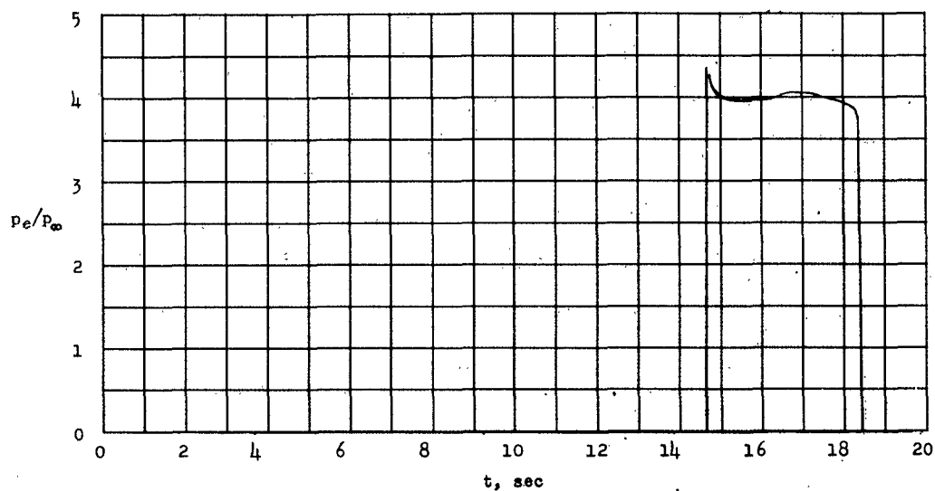
Figure 15.- The variation of jet static-pressure-ratio with time.
