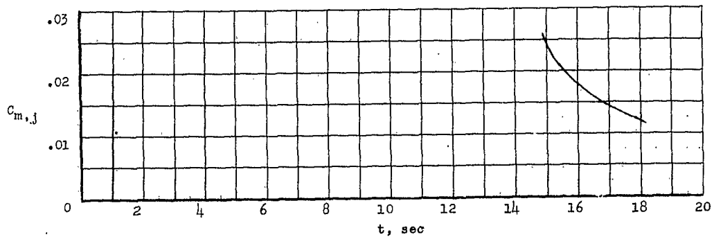
Figure 23.- Variation of jet-on pitching-moment coefficient with time.
