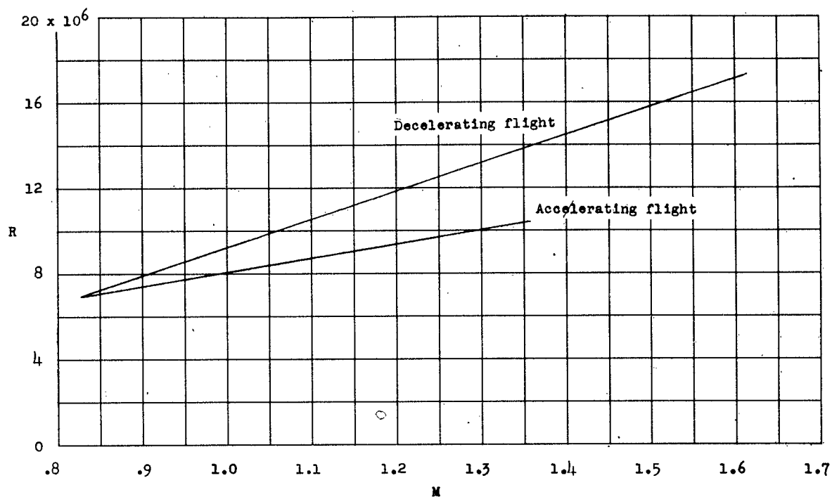
Figure 7.- Variation of Reynolds number with Mach number.
