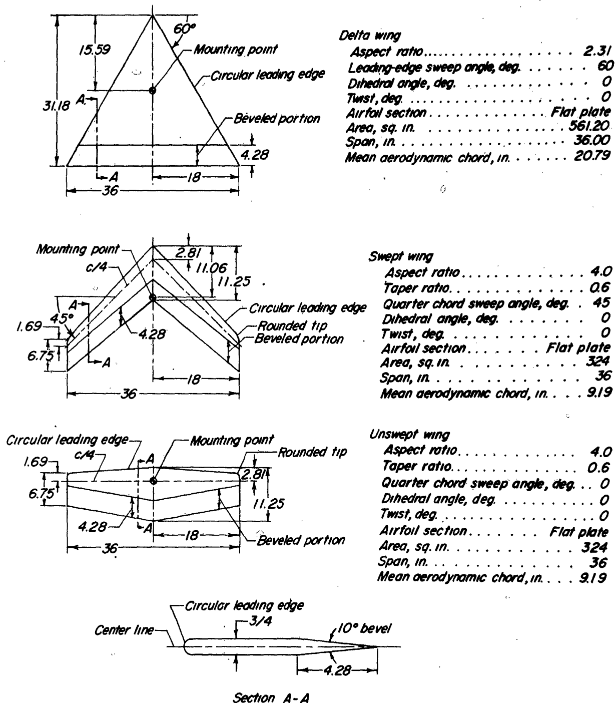
Figure 4.- Sketches and geometric characteristics of the three wing models investigated. All dimensions are in inches.
