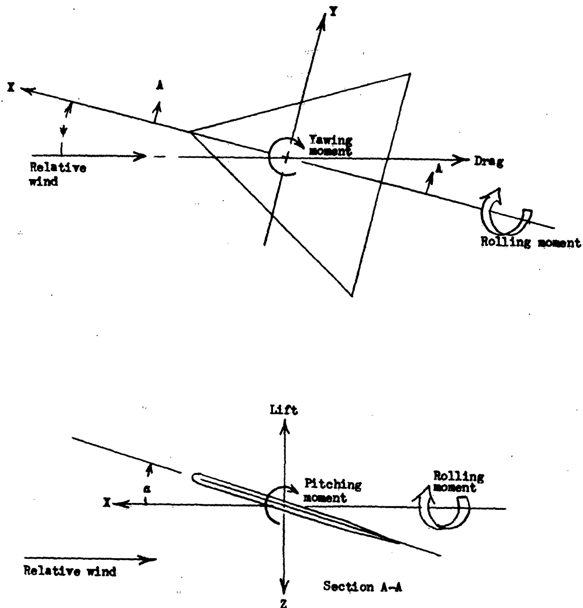
Figure 1.- System of stability axes. Arrows indicate positive forces, moments, and displacements.
