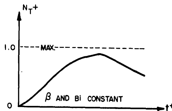
FIGURE 6 DIMENSIONLESS THERMAL FORCE
