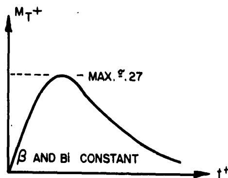
FIGURE 5 DIMENSIONLESS THERMAL MOMENT
