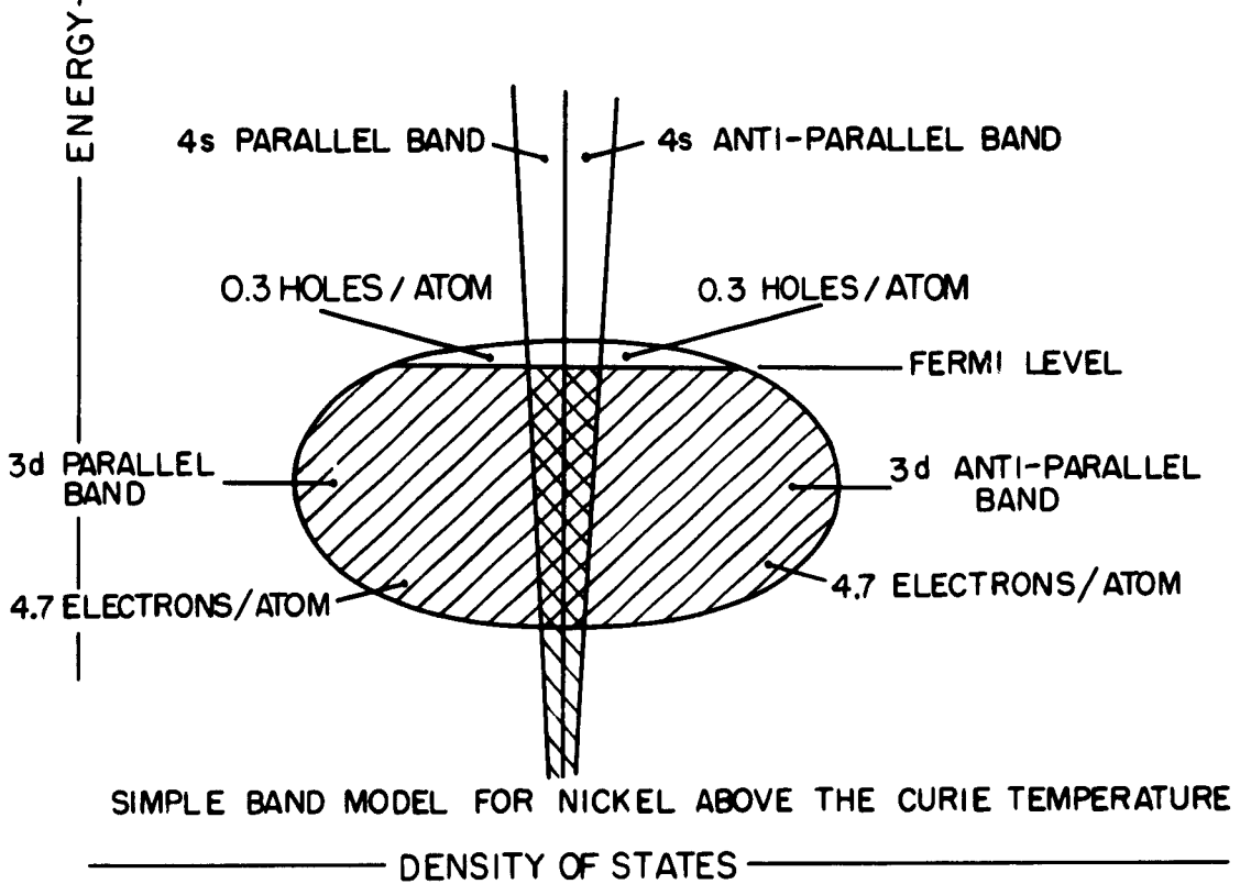
FIG.4 -9 A SIMPLE BAND MODEL FOR Ni
