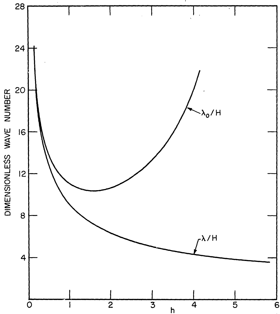
FIG. 4 DIMENSIONLESS WAVE NUMBER vs. h
