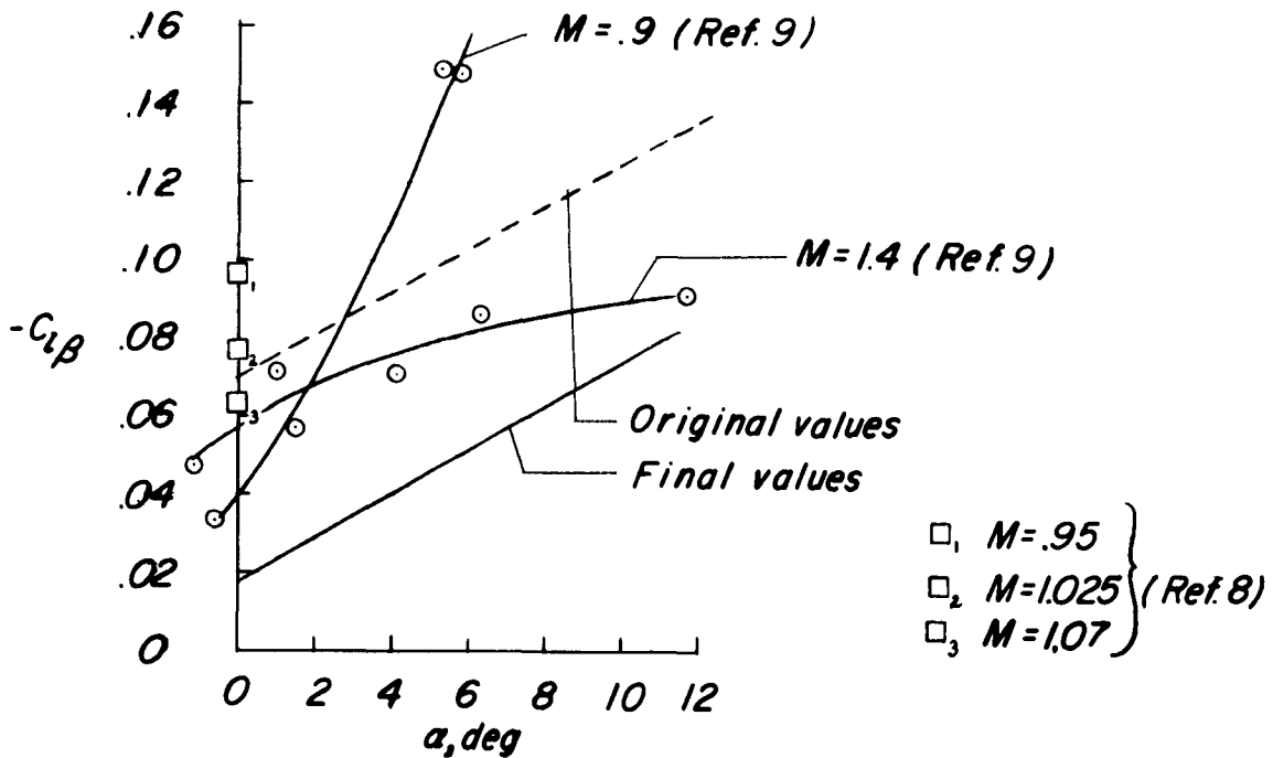
Figure 3.- Variations of the sideslip derivatives C_{n\beta} and C_{l\beta} with angle of attack from various sources and those used in the calculations.
