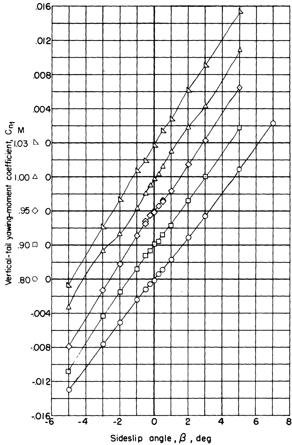
(b) Vertical-tail yawing moment.
