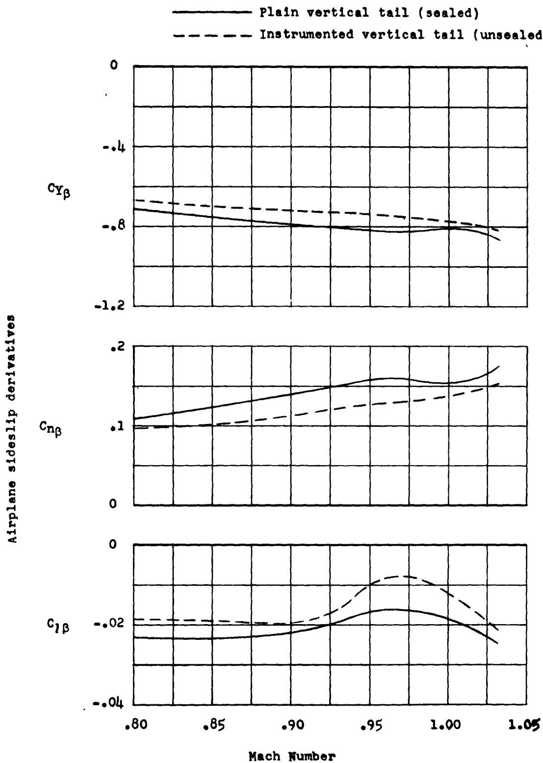
Figure 6.- Effect of unsealed vertical-tail root on the airplane sideslip derivatives. \alpha = 0^\circ .
