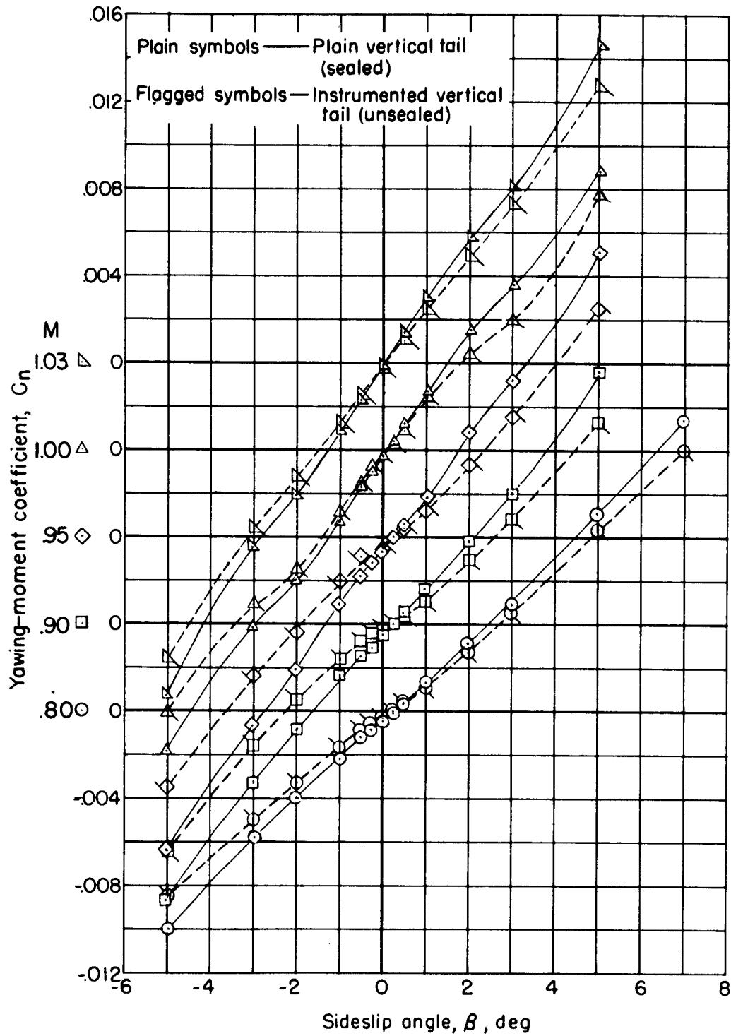
(b) Yawing moment.
