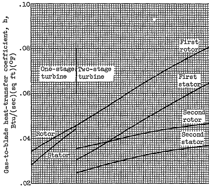
(c) Gas-to-blade heat-transfer coefficient. Turbine-inlet temperature, 2800^\circ\text{R} .
