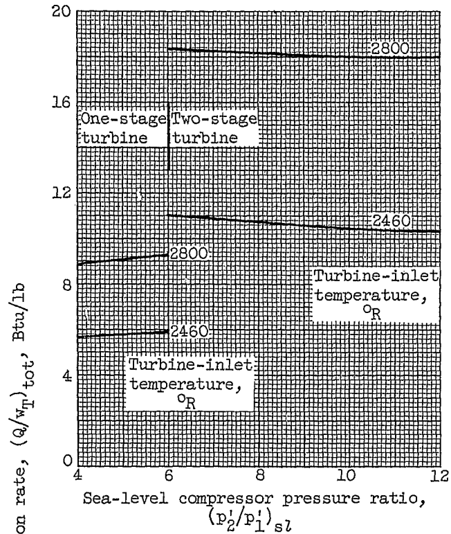
(a) Effect of compressor pressure ratio. Flight Mach number, 2.0.
