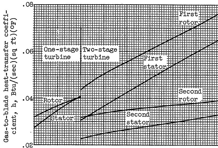
(a) Gas-to-blade heat-transfer coefficient. Turbine-inlet temperature, 2460° R.
