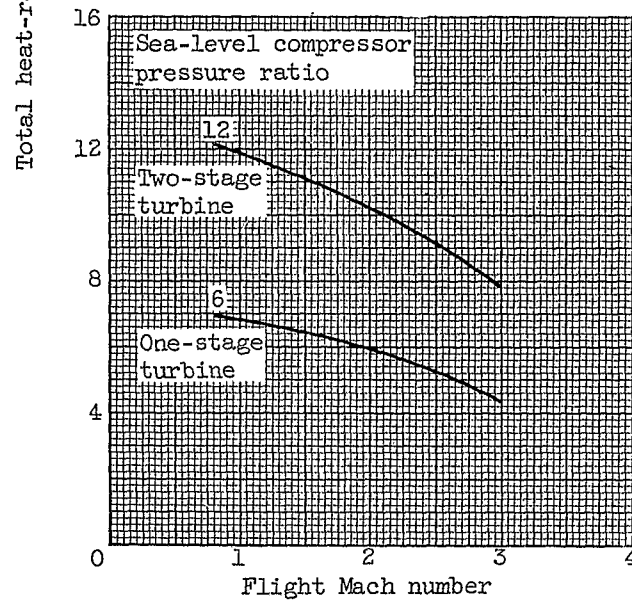
(b) Effect of flight Mach number. Turbine-inlet temperature, 2460° R.
