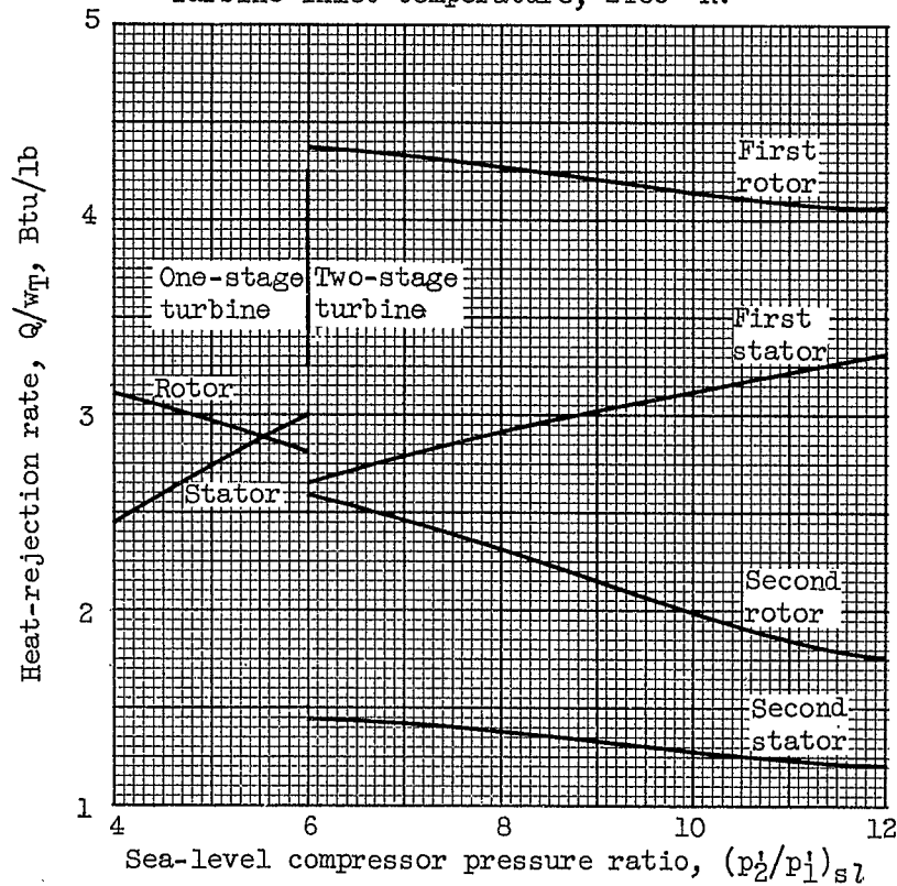
(b) Heat-rejection rate. Turbine-inlet temperature, 2460° R.
