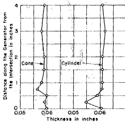
Figure 60 - Thickness Measurements on 0-Degree Generator of Cone and Cylinder of Model CC-8A
