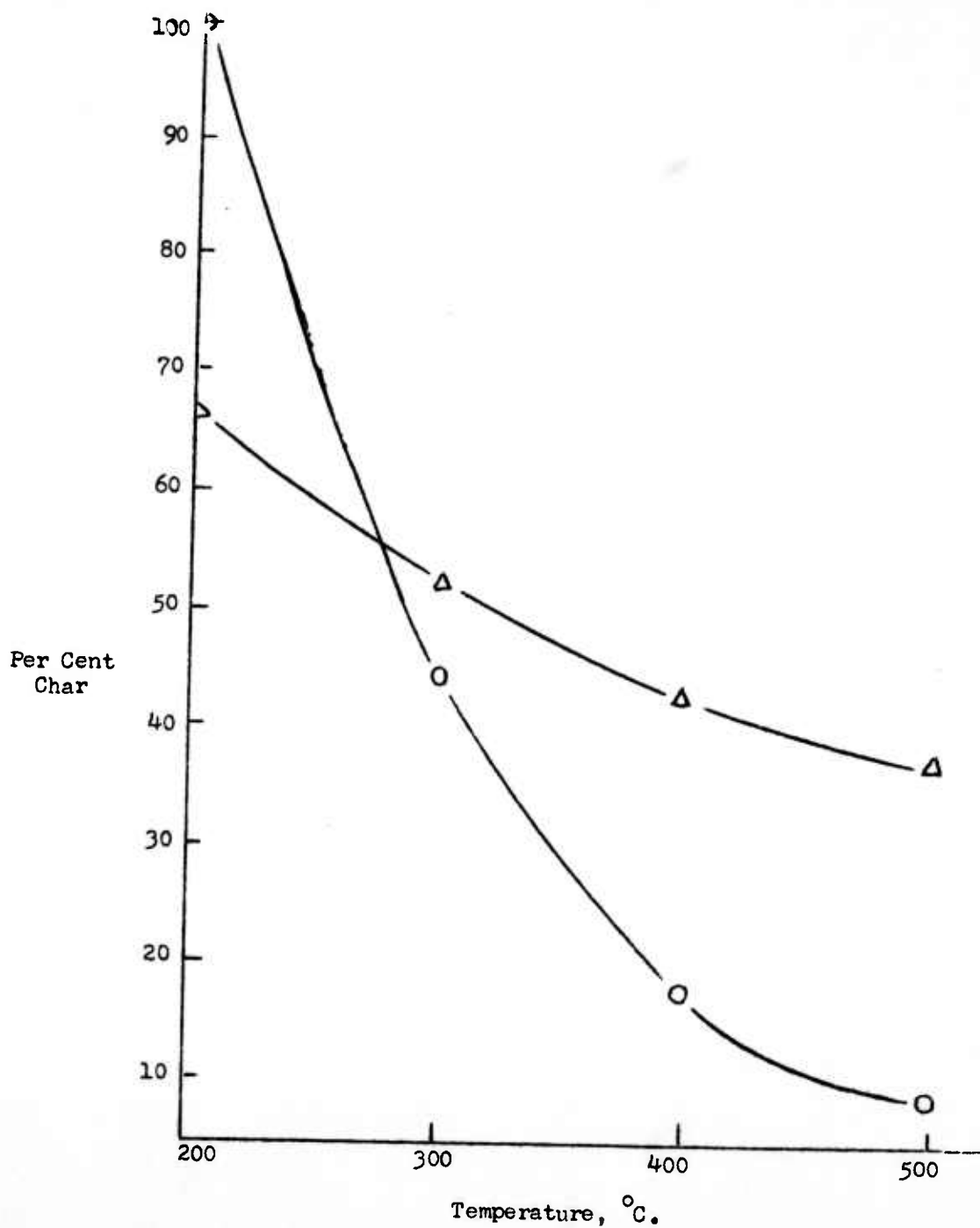
Figure 15. Pyrolysis of levoglucosan: untreated, O; 90% levoglucosan + 10% (\text{NH}_4)_2 \text{HPO}_4 , Δ.
