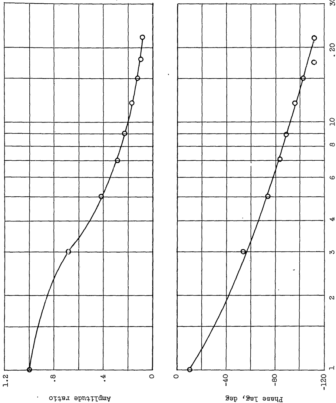
Figure 2. - Dynamic response of bypass door.
