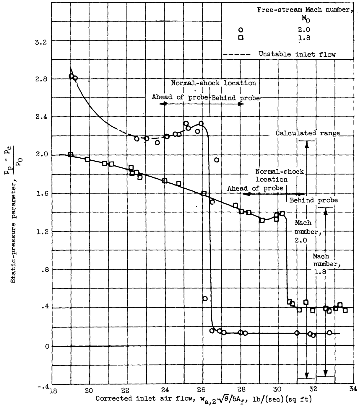
Figure 3. - Steady-state variation of static-pressure parameter.
