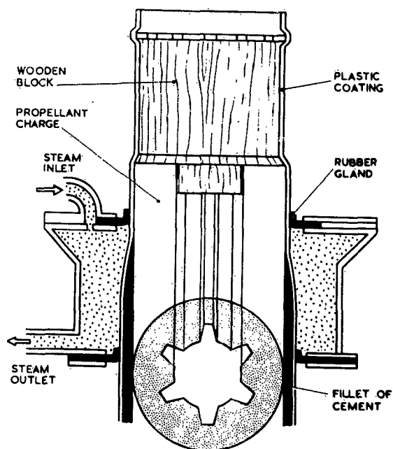
Fig. 18. Coating operation in stress relief technique
