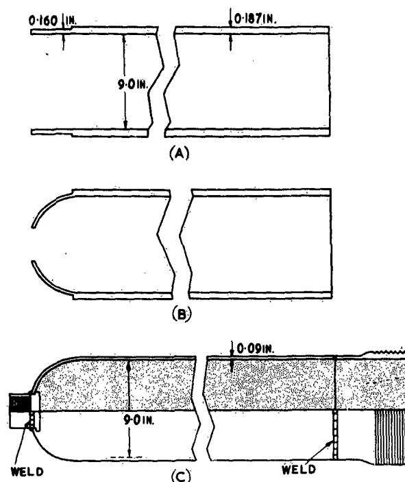
Fig. A6. Stages in manufacture of thin-walled Mayfly tube
