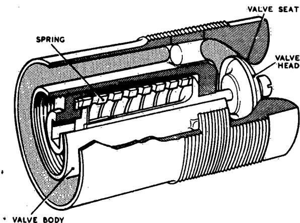
Fig. 45. Valve nozzle
