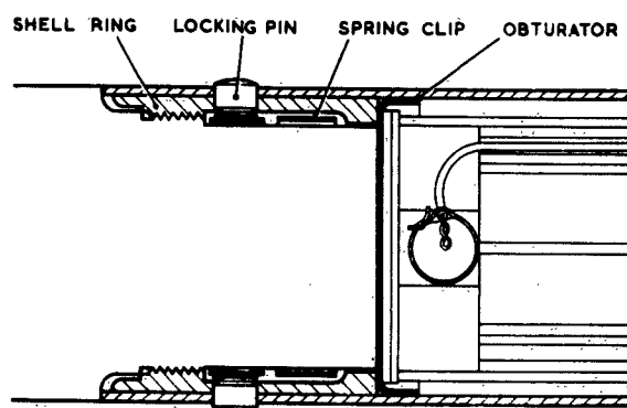
Fig. 34. Obturation to seal end closures
