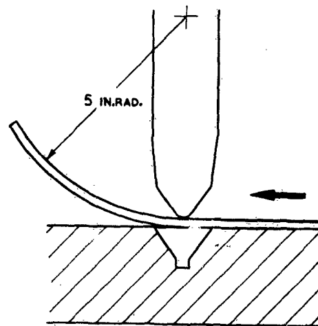
Fig. A15. Brake press used for preforming metal sheet
