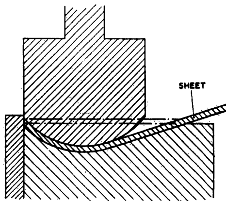
Fig. A9. Tools used for preforming sheet metal
