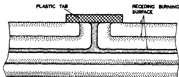
Fig. 14. How tabbed charges are supported
