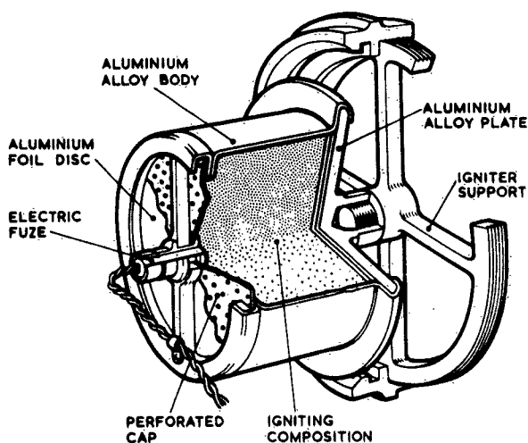
Fig. 38. Metal igniter housing used in 9-in. rocket
