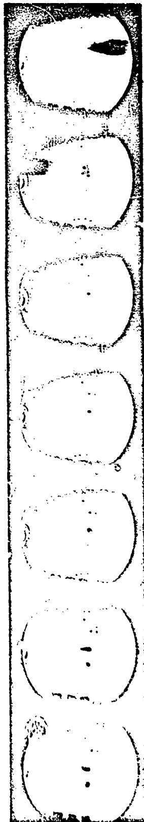
Shot No. 14. 20-mm Projectile, Speed 2660 ft./sec WADC TR 56-393. Vol. I
