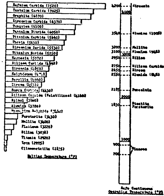
Fig. 1 Thermal properties of ceramic materials and metals
