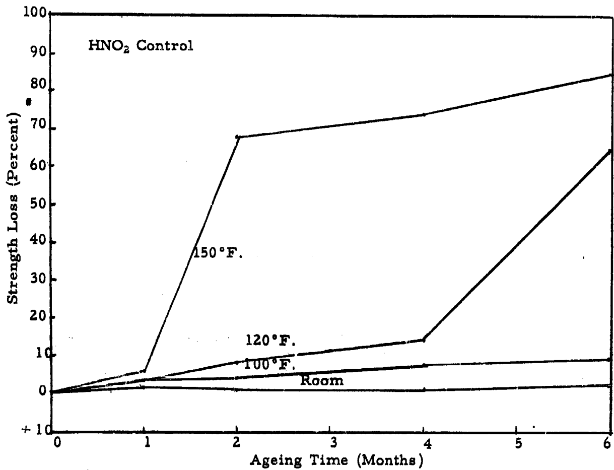
Figure 17 Loss in Strength vs. Ageing Time when nylon is treated in HNO 2 Control and aged in solution at different temperatures.
