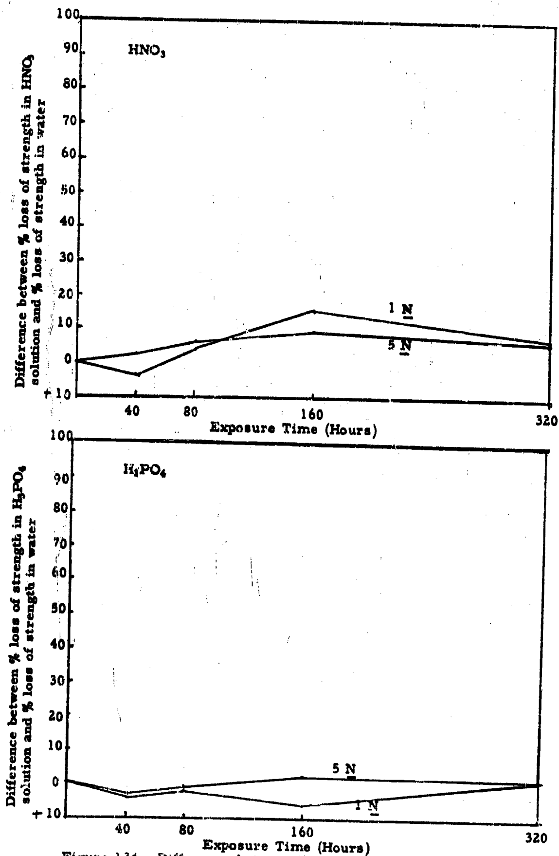
Figure 134. Difference between % loss of strength of Dacron (Type II) in \text{HNO}_3 and \text{H}_3\text{PO}_4 solutions and % loss of strength in water vs. exposure time in Fade-O-meter.
