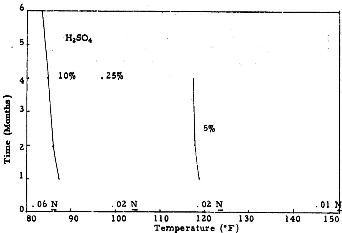
Figure 93. Time vs. Temperature to Effect Specific Strength Losses when nylon is treated in H_2O and H_2SO_4 and aged at high relative humidity; initial concentration of H_2SO_4 used at each temperature condition is shown.
