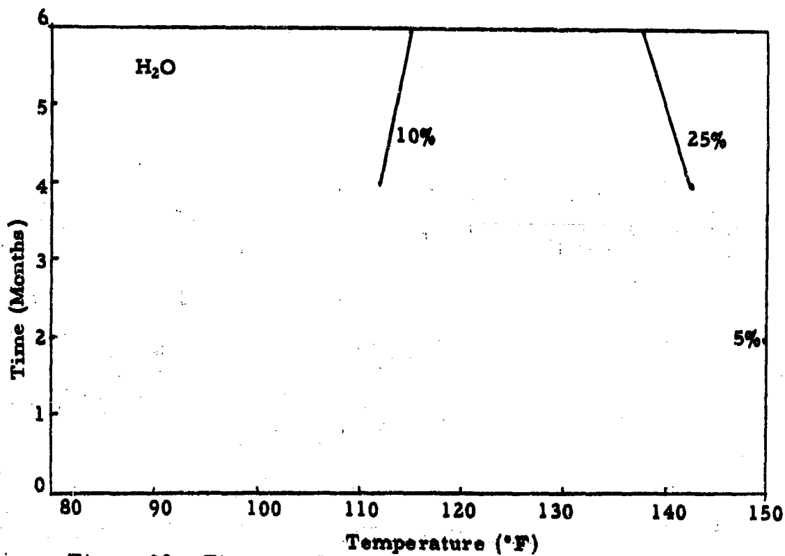
Figure 92. Time vs. Temperature to Effect Specific Strength Loss when nylon is in H 2 O and aged at low relative humidity.
