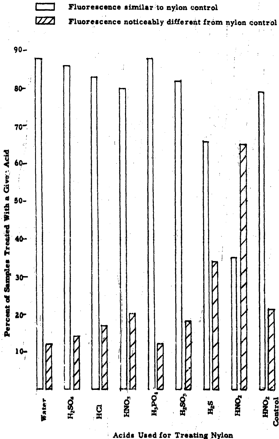
Figure 144 Percent of nylon samples treated with a given acid which fluoresce similar to and noticeably different from the nylon control under visible light vs. acids used for treating nylon.
