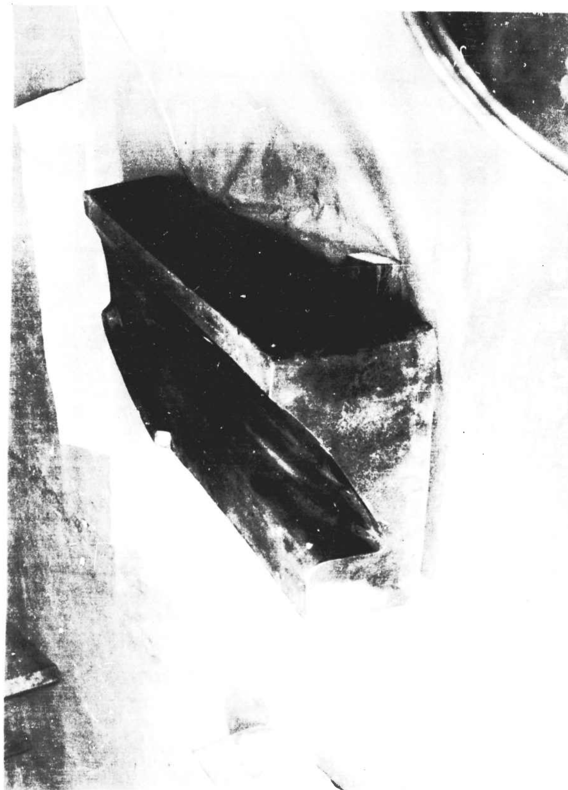
FIGURE 1 - AIRSIDE DEEP HAIRER DIE
