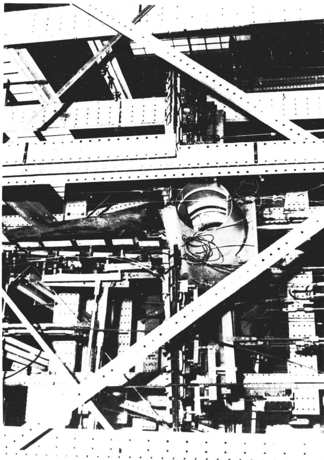
FIGURE 42 - MAGNESIUM F-80C EXPELLER AND FUSELAGE SUPPORTING 100 PERCENT ULTIMATE LOAD FOR COMBINATION B
