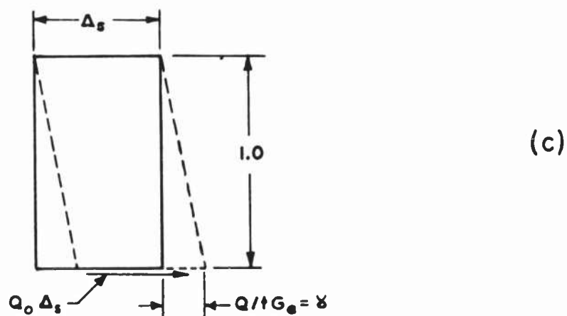
FIG.85 NOTATION FOR DETERMINATION OF WORK DUE TO TWISTING OF A SINGLE CELL.
