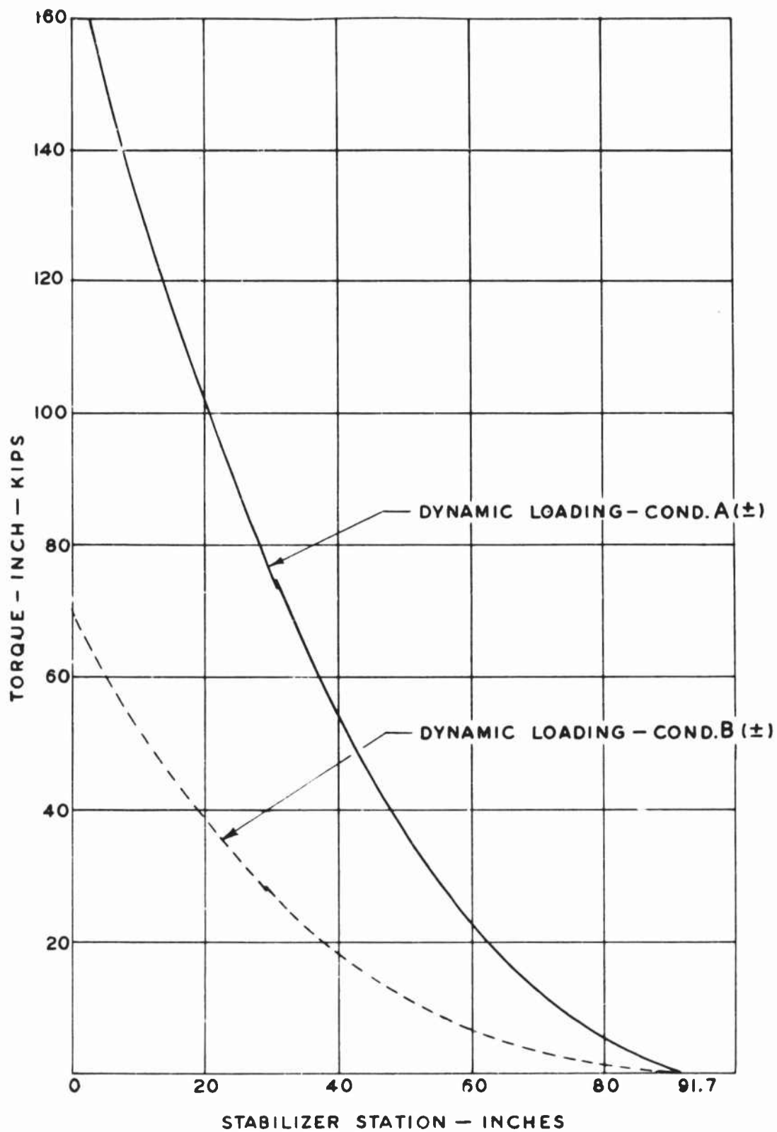
FIG. 86 NET STABILIZER TORQUES—ULTIMATE ABOUT REFERENCE AXIS (REF. TABLE 5)
