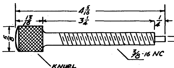
BUTTON FOR "C" CLAMP
