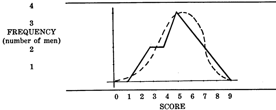
FIGURE 1 CURVE OF SCORE DISTRIBUTION IN EXHIBIT I
