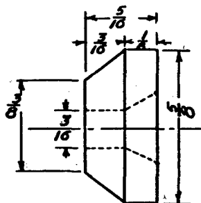
BUTTON FOR "C" CLAMP
