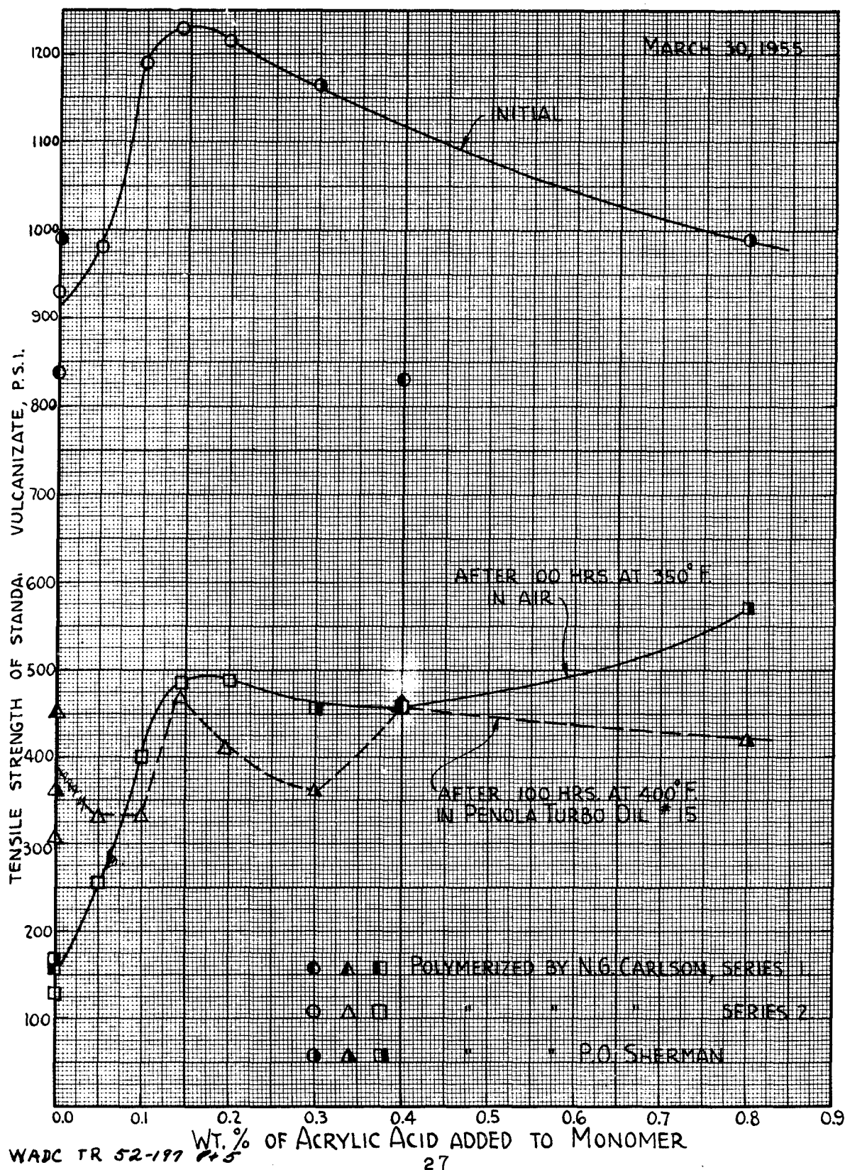
FIG. 1. PROPERTIES OF POLY-FBA MADE BY SULFAN PROCESS
