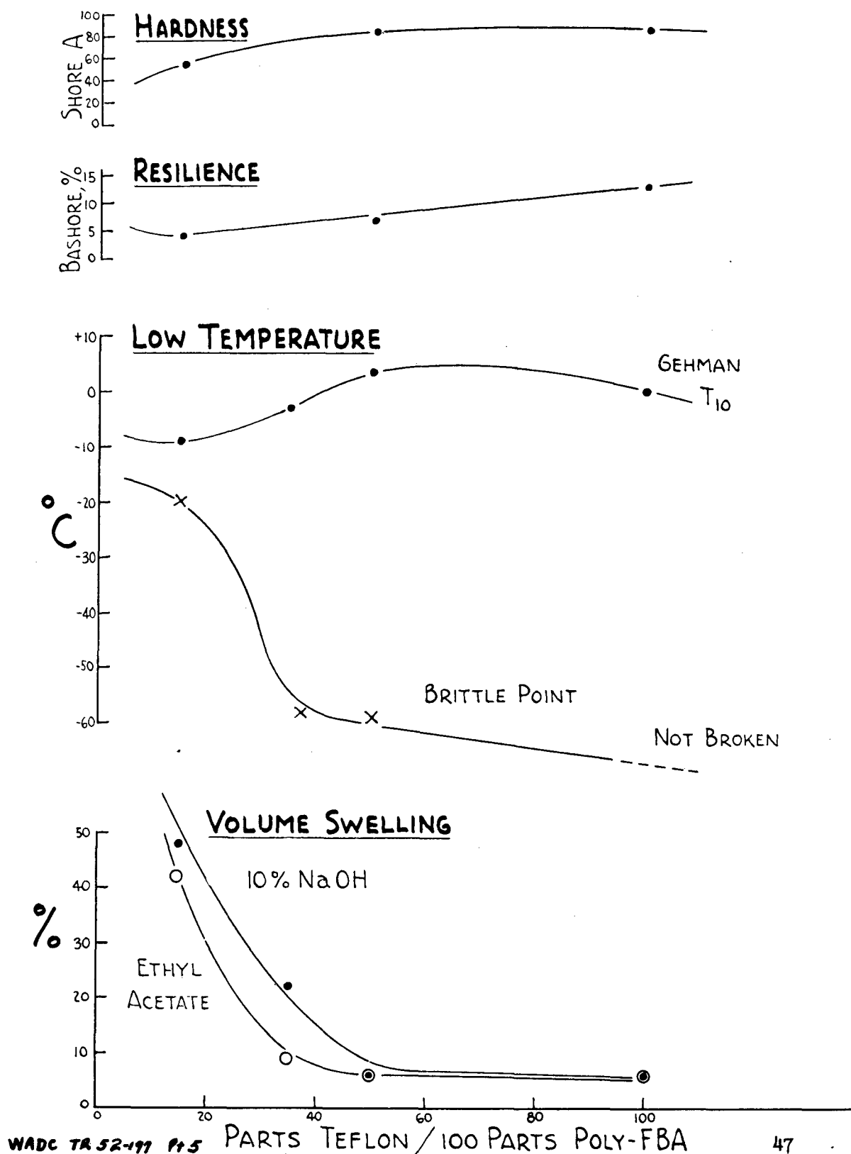
FIG 6 TEFLON - POLY-FBA BLENDS
