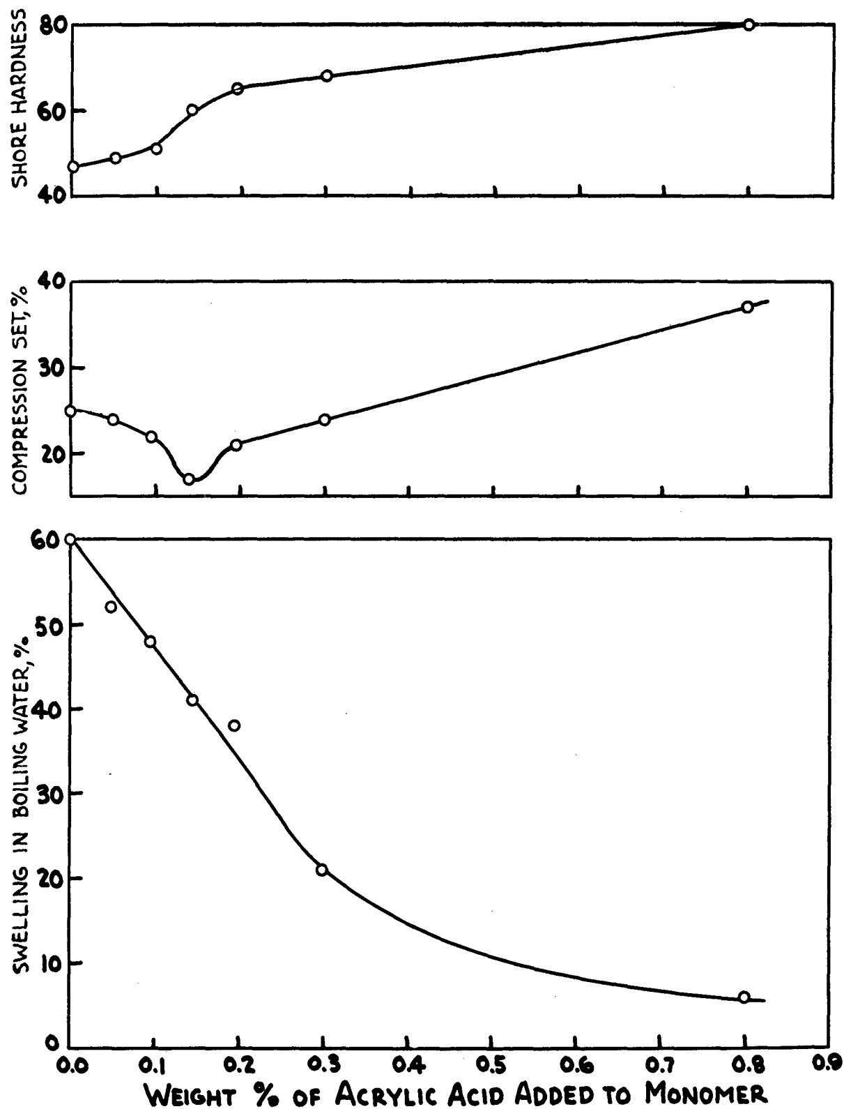
Figure 3. Properties of Standard Vulcanizate
