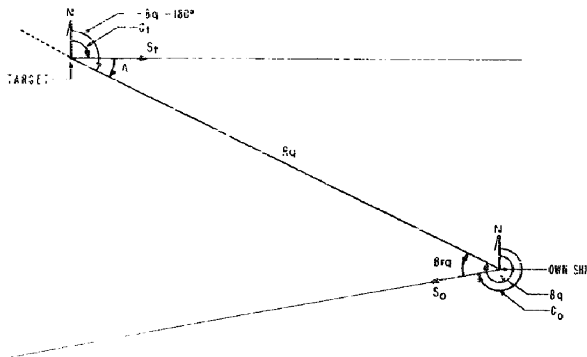
Fig. 2 - Geometry of relative ship motion
