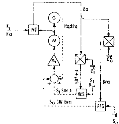
Fig. 5 - Bearing computer section of relative motion computer
