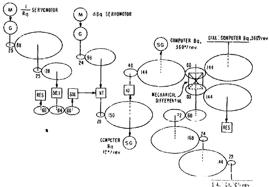
Fig. A2 - Range inversion and bearing-rate servos
