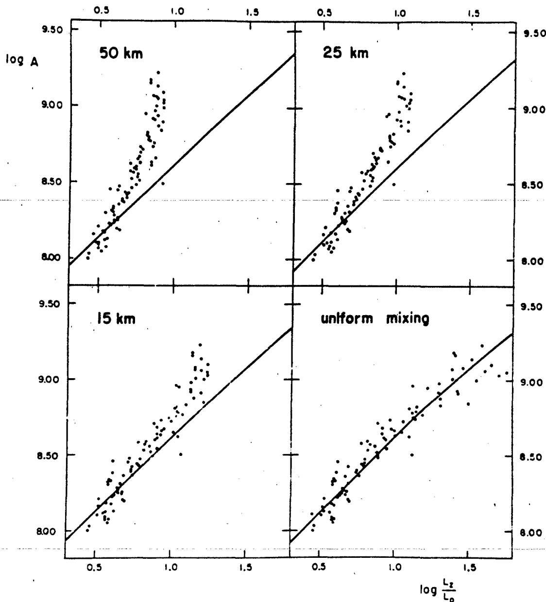
Courtesy of Leo Goldberg and Edith A. Muller, McMath-Hulbert Observatory, University of Michigan Fig. 5. Empirical curves of growth for \text{N}_2\text{O} assuming that \text{N}_2\text{O} is concentrated in a layer of uniform density 5-km thick at altitudes of (a) 50, (b) 25, and (c) 15 km, and (d) that \text{N}_2\text{O} has the same vertical distribution as the main body of the atmosphere.
