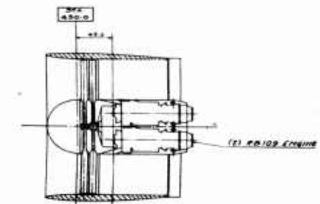
PLAN VIEW OUTBOARD ENGINES
