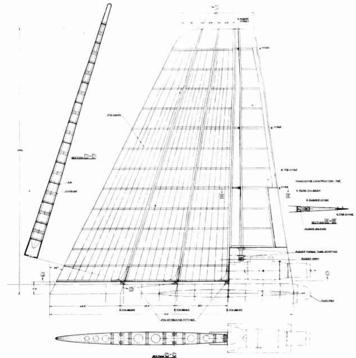
Figure 18. Dwg. No. D181-960-019; Sheet 2: Tail Surface Structural Assemblies
