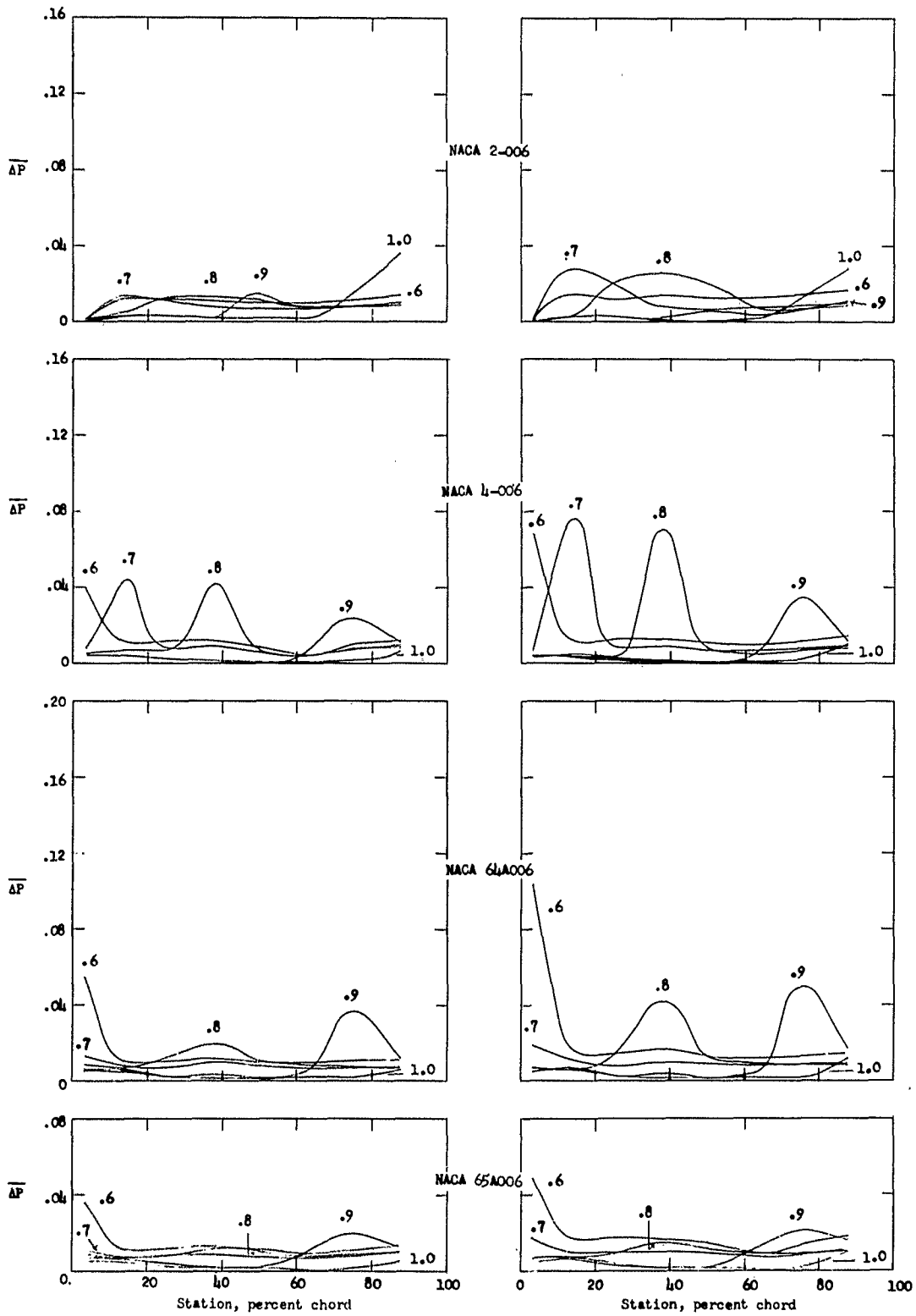
(a) c_n = 0.2 .
