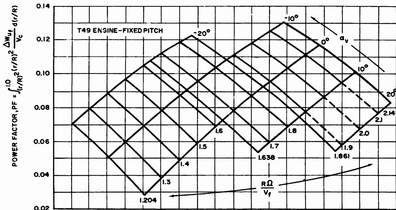
Figure 67. Power Factor Configuration No. 1
