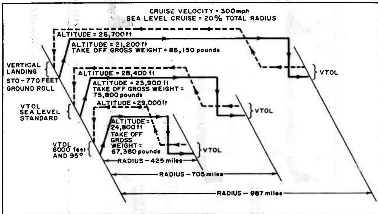
Figure 5. Mission Profiles
