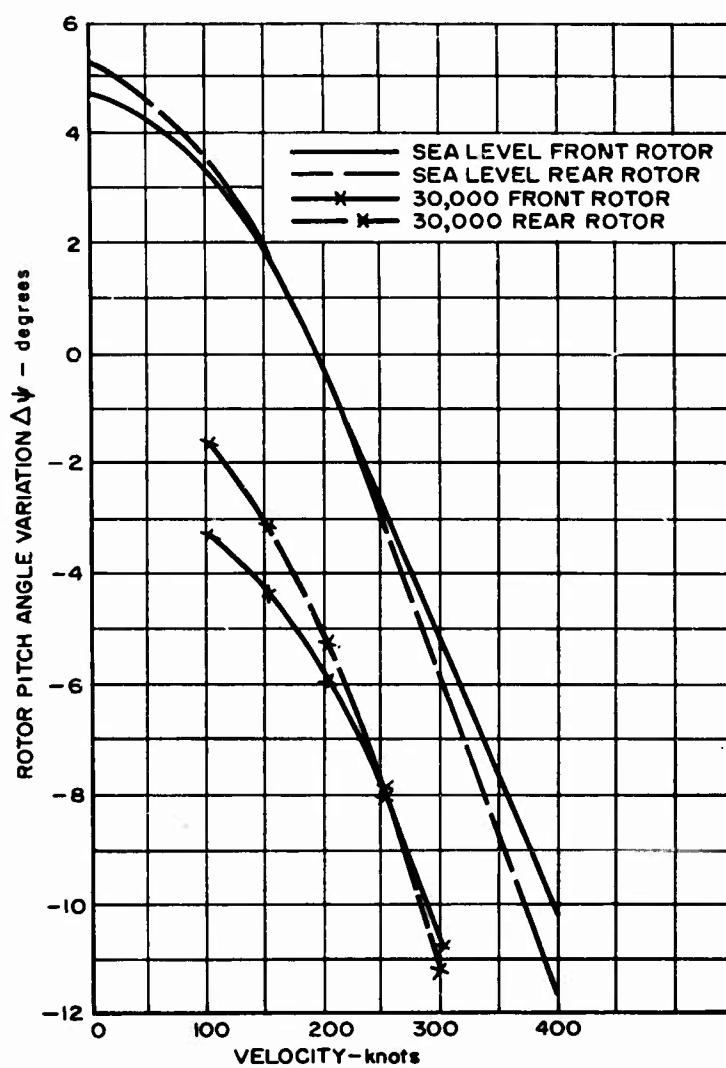
Figure 73. Contrarotating Propellers. Pitch Variation
