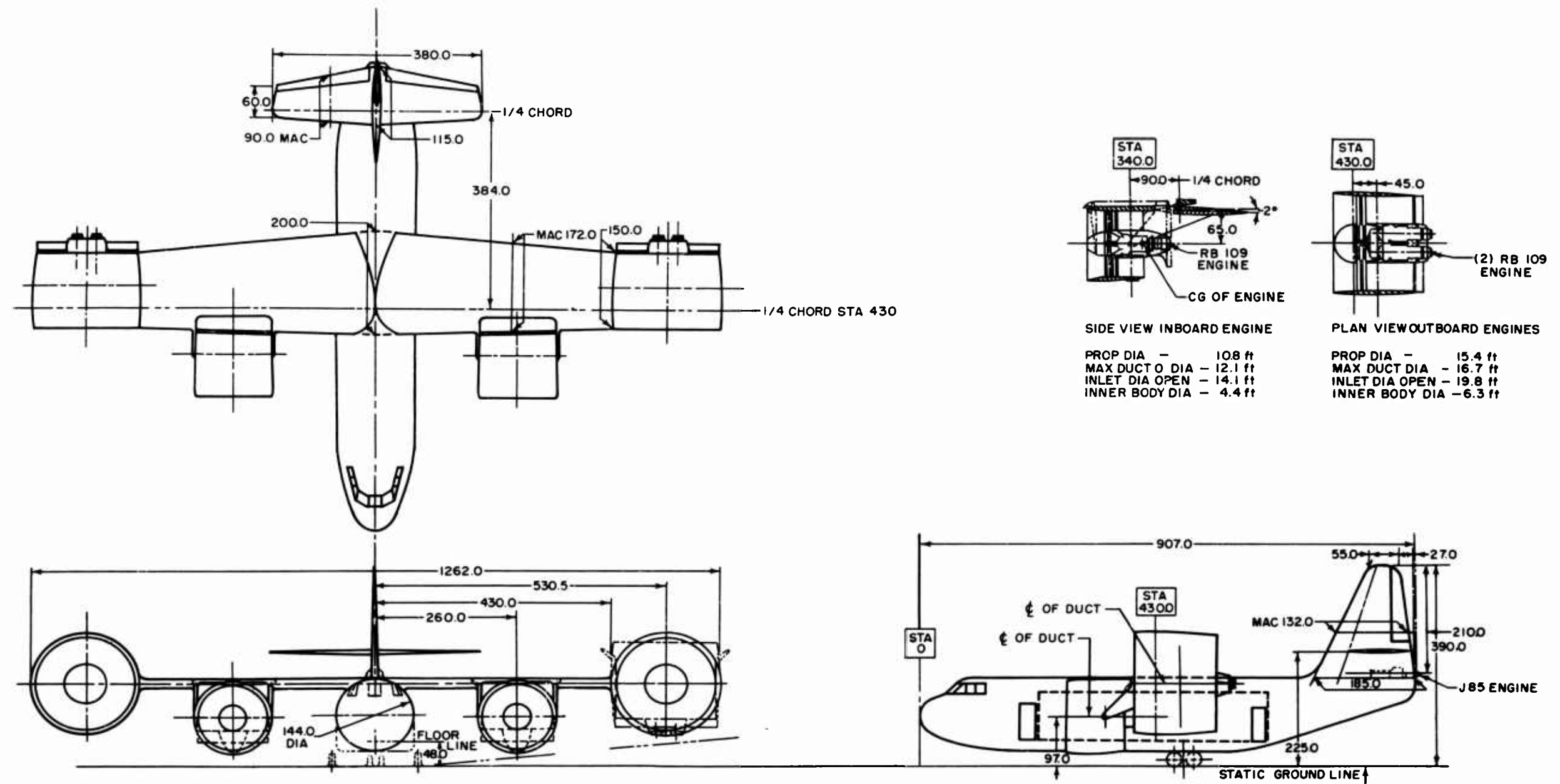
Figure 28. Ducted Propeller Medium Cargo Transport
