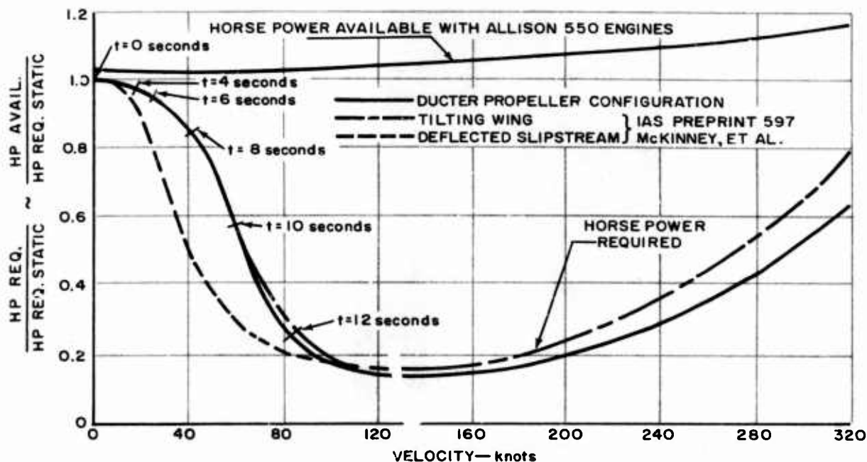
Figure 16. Transition Power Requirements
