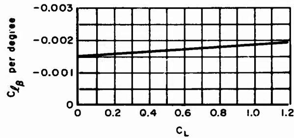
Figure 60. Rolling Stability of Airplane
