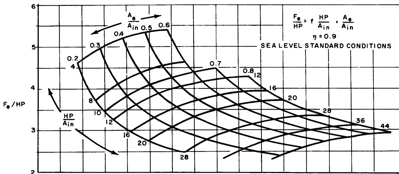
Figure 65. Ducted Fan Performance - Static
