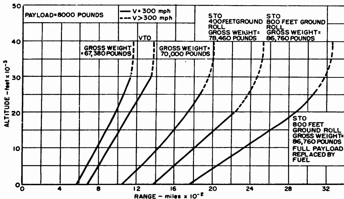
Figure 40. Ferry Range vs Cruise Altitude
