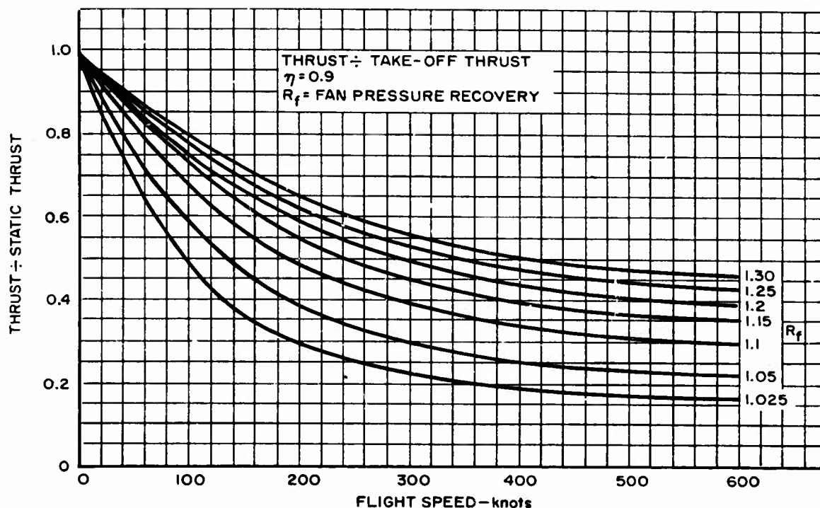
Figure 61. Typical Shaft - Power Turbine plus Fan Characteristics
