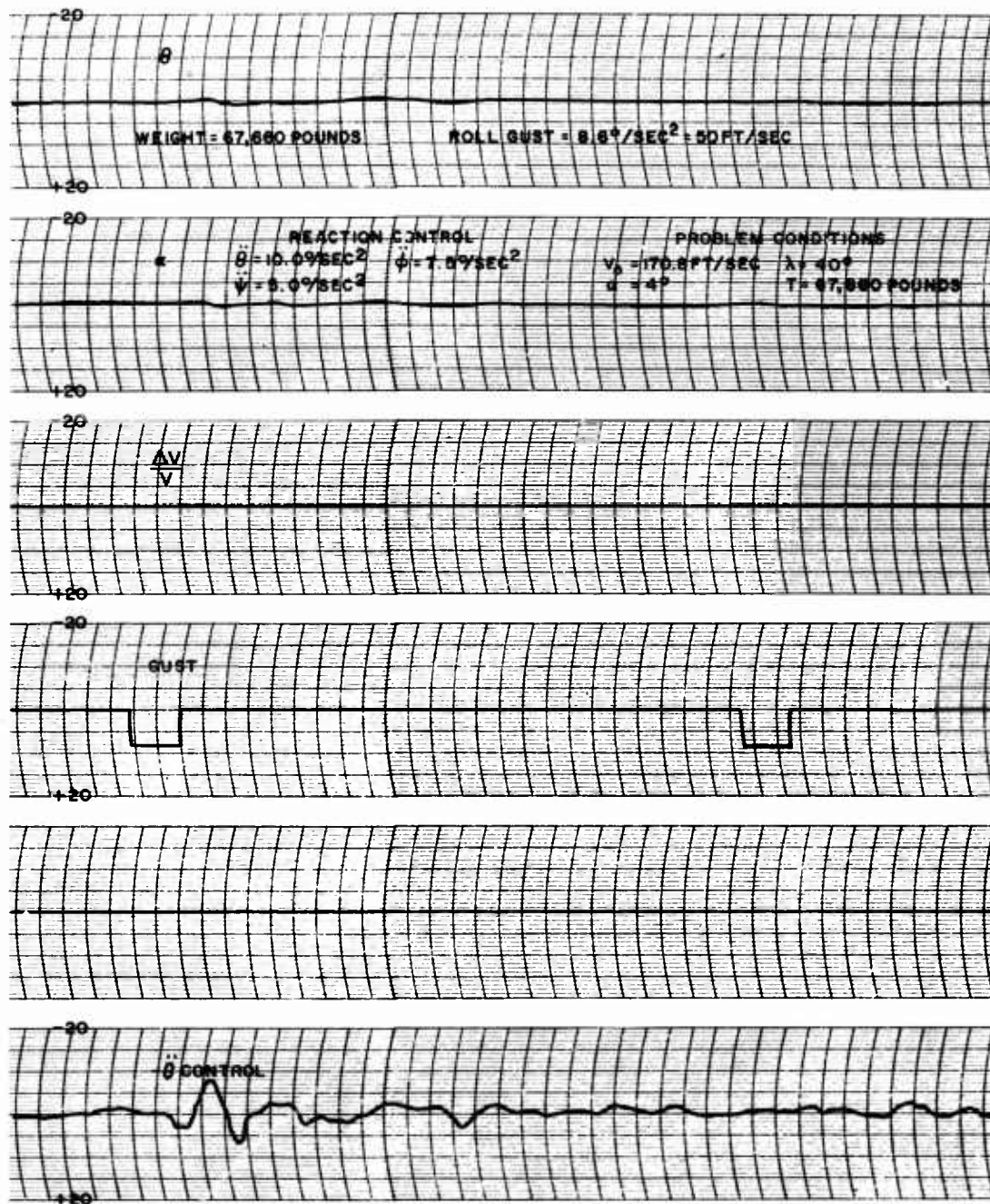
Figure 55b. Transition Longitudinal Traces
