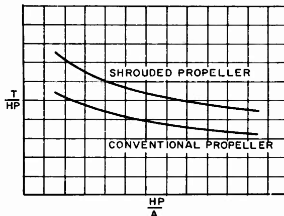
Figure 25. Static Thrust Comparison
