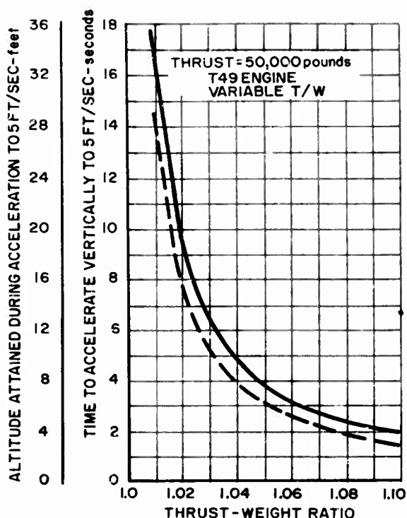
Figure 48. Vertical Take-Off Performance
