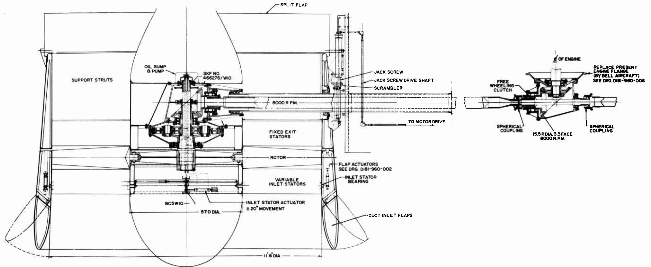
Figure 30. Propulsion System Assembly
