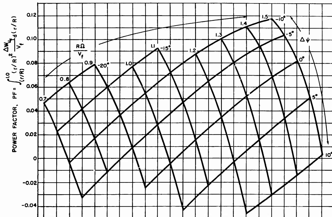
*Figure 72. Rear Rotor Performance for Allison 550-B1
