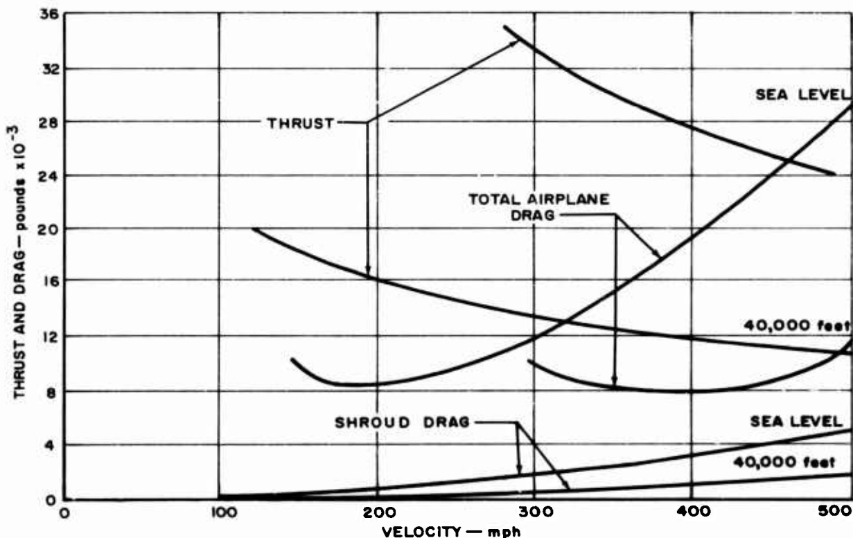
Figure 34. Thrust and Drag
