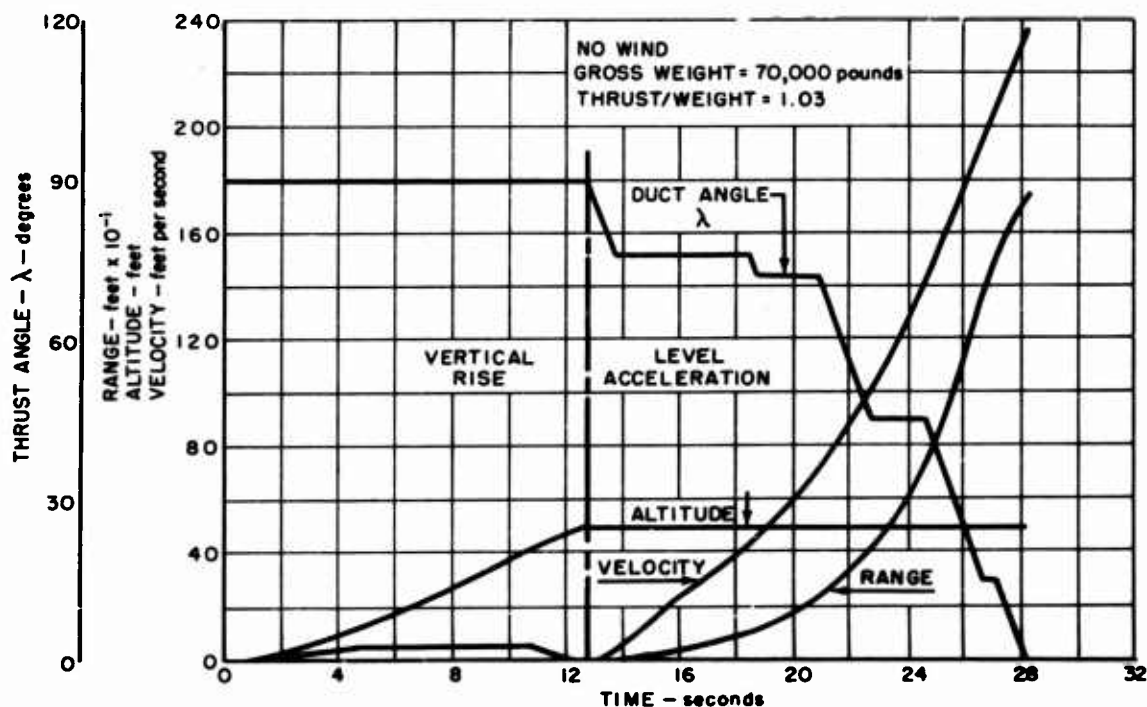
Figure 37. Vertical Take-Off and Transition
