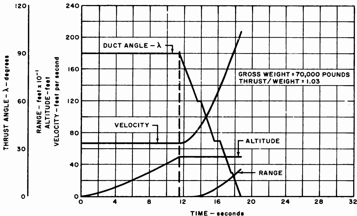
Figure 38. Vertical Take-Off and Transition in 40-Knot Wind
