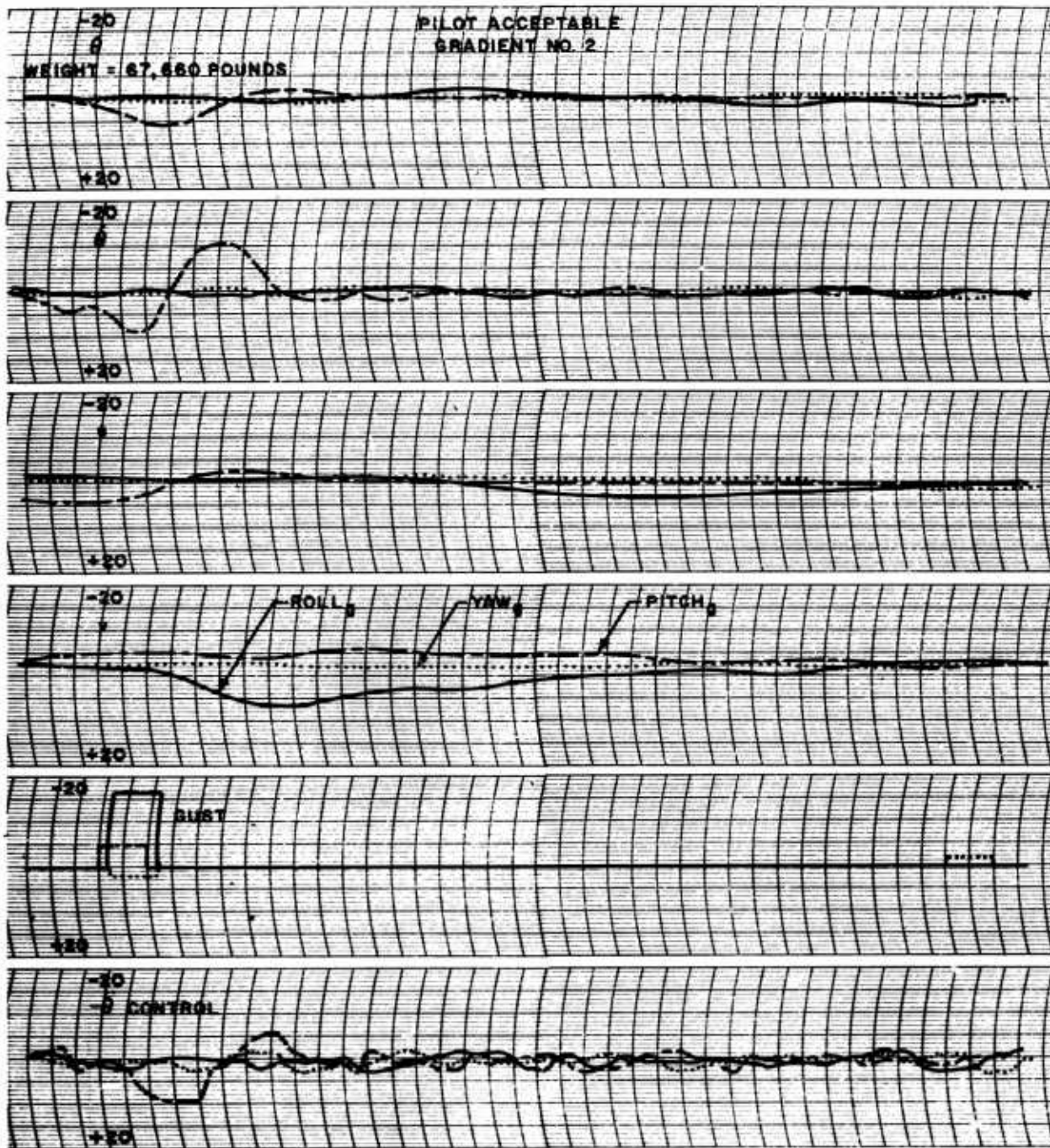
Figure 50b. Effect of Roll, Pitch, and Yaw Gusts at 50 feet per Second in Hovering. Longitudinal Dynamics
