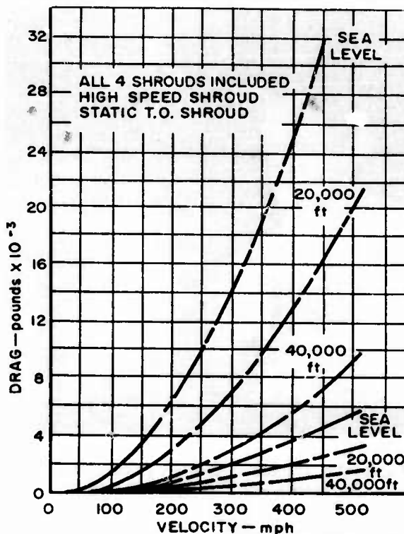
Figure 11. Shroud Drag
