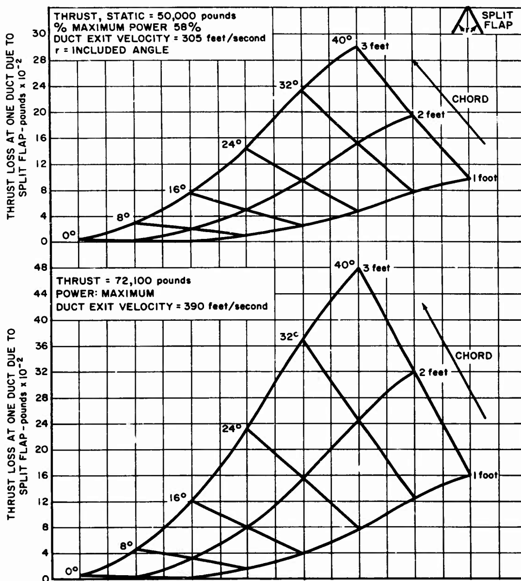
Figure 53. Roll Reaction Control Forces Developed by Split Flap at Exit of One Outboard Duct
