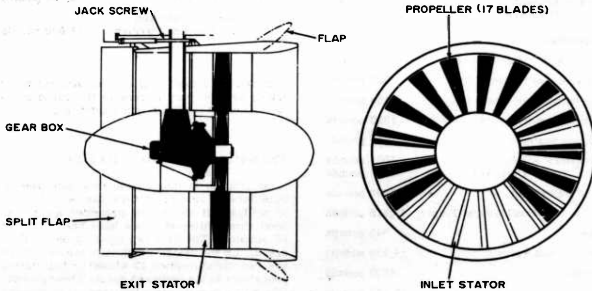
Figure 10. Fixed Rotor Ducted Propeller
