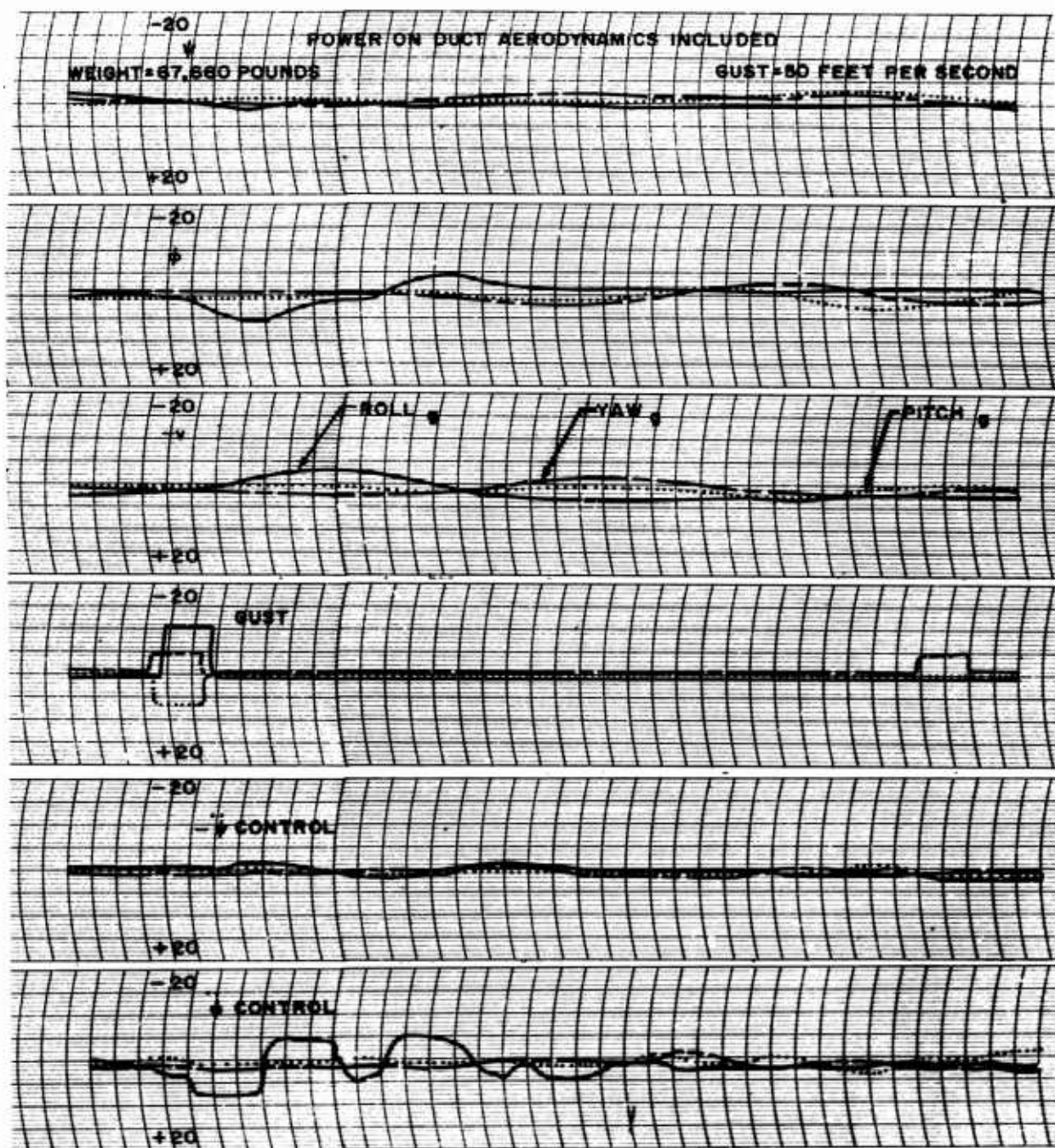
Figure 51a. Effect of Roll, Pitch, and Yaw Gusts in Hovering. Lateral Dynamics
