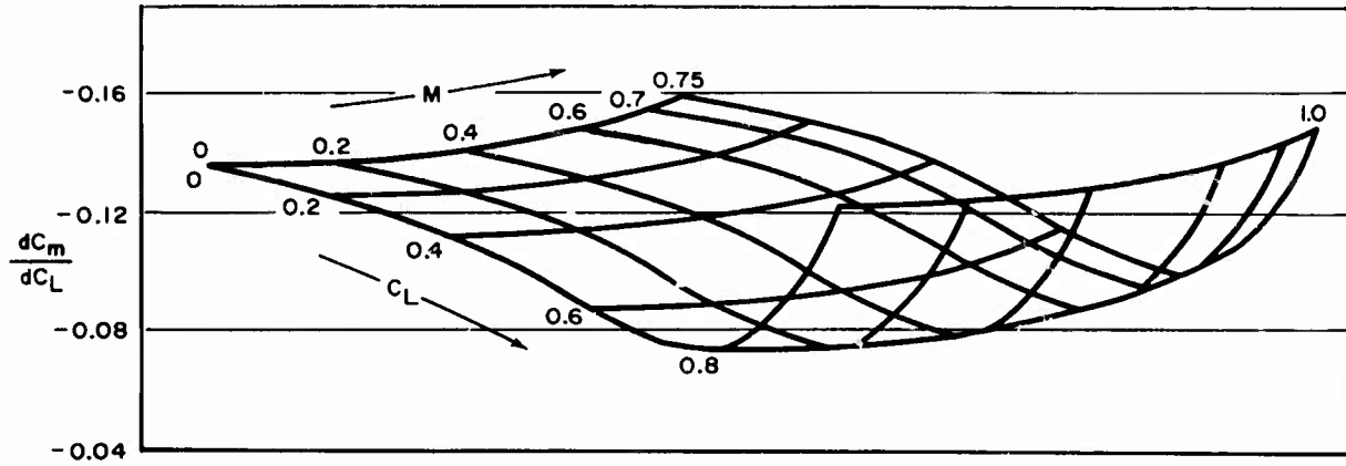
Figure 58. Airplane Longitudinal Stability
