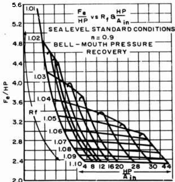
Figure 62. Static Momentum Data
