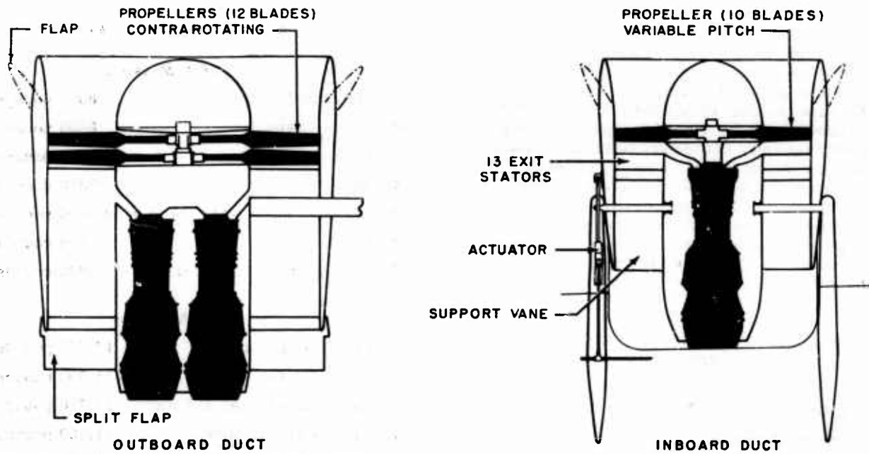
Figure 9. Duct and Propeller Cutaway
