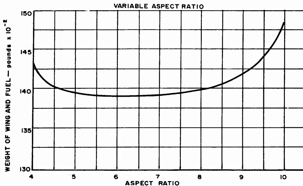
Figure 45. Weight of Wing and Fuel for Basic Mission
