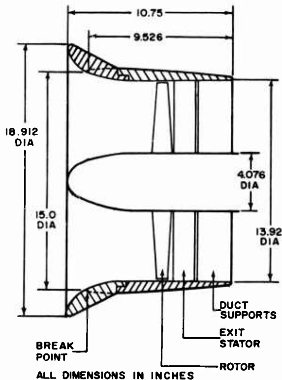
Figure 78. Wind Tunnel Model No. 2. Variable Pitch Rotor and Fixed and Fixed Exit Stators
