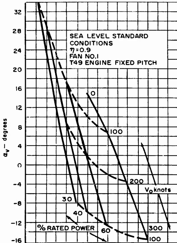
Figure 58. Inlet Guide Vane Angle Required at Various Settings
