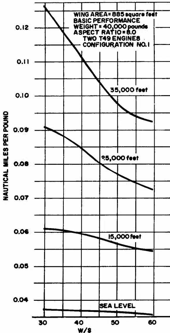
Figure 46. Cruise Parameter - Variable Gross Weight
