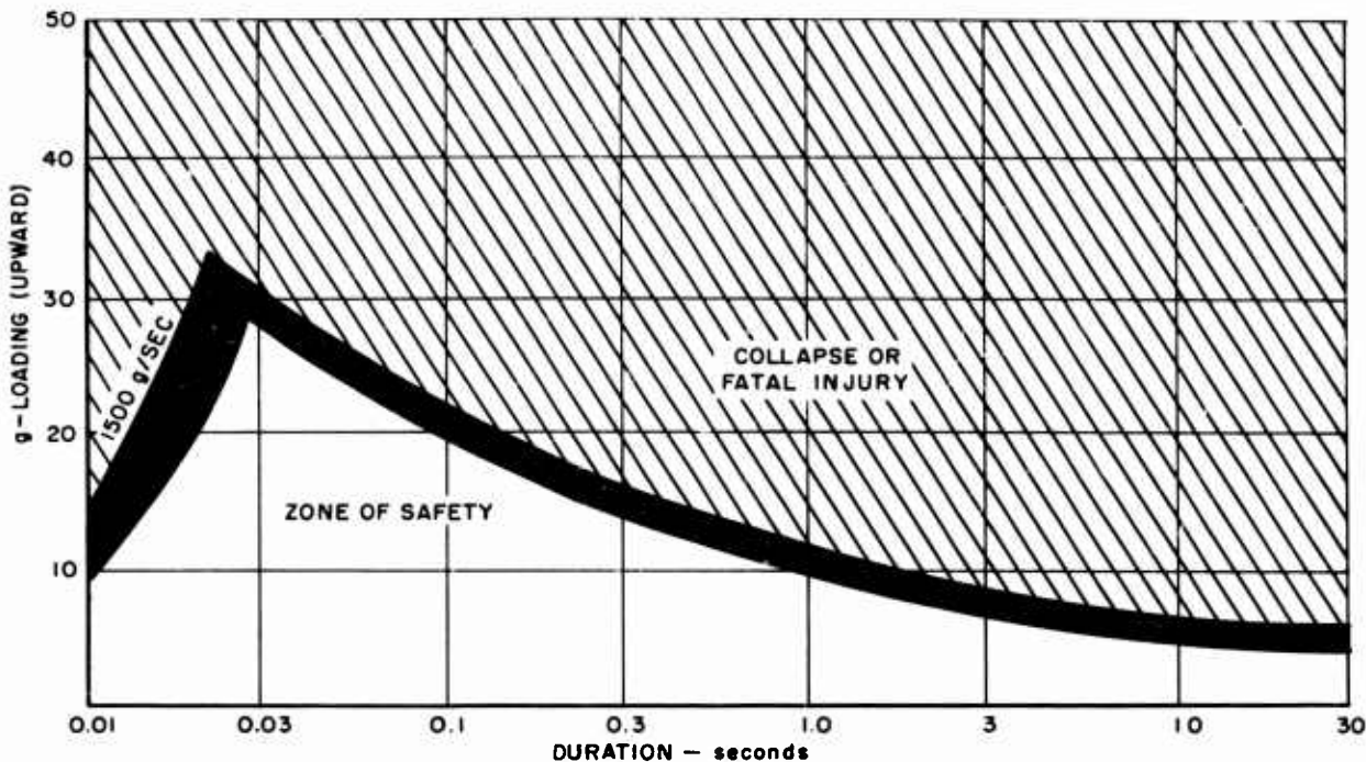
Figure 76. Limits of Human Tolerance for Escape Systems
