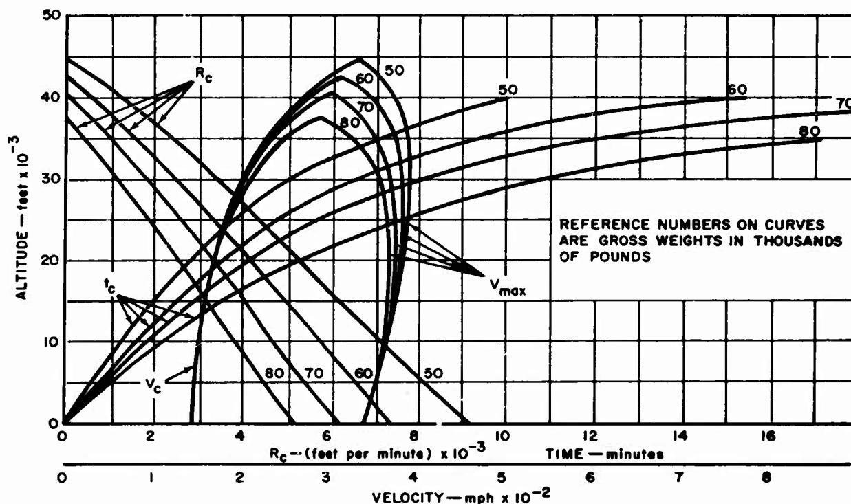
Figure 42. Classical Performance - D181-950-007 Configuration
