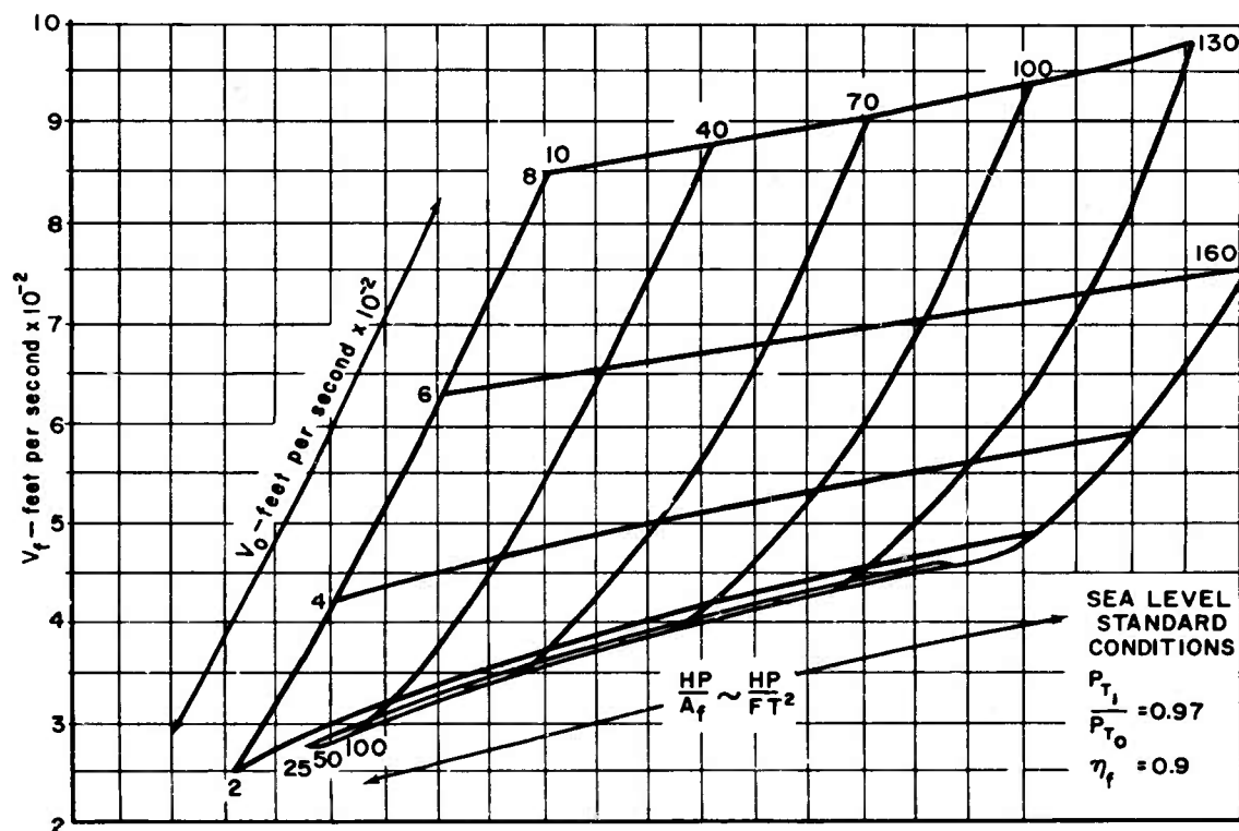
Figure 66. Inflight Ducted Propeller Performance. Axial Velocity
