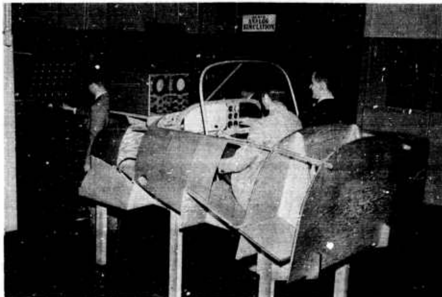
Figure 17. Computer and Cockpit Set-Up
