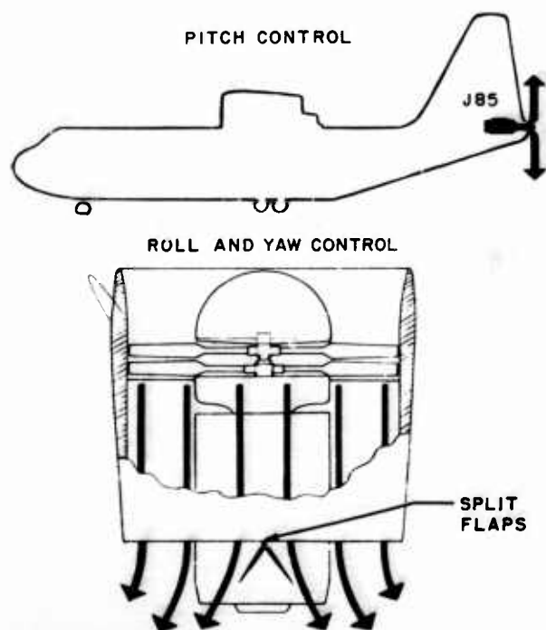
Figure 20. Hovering Control System
