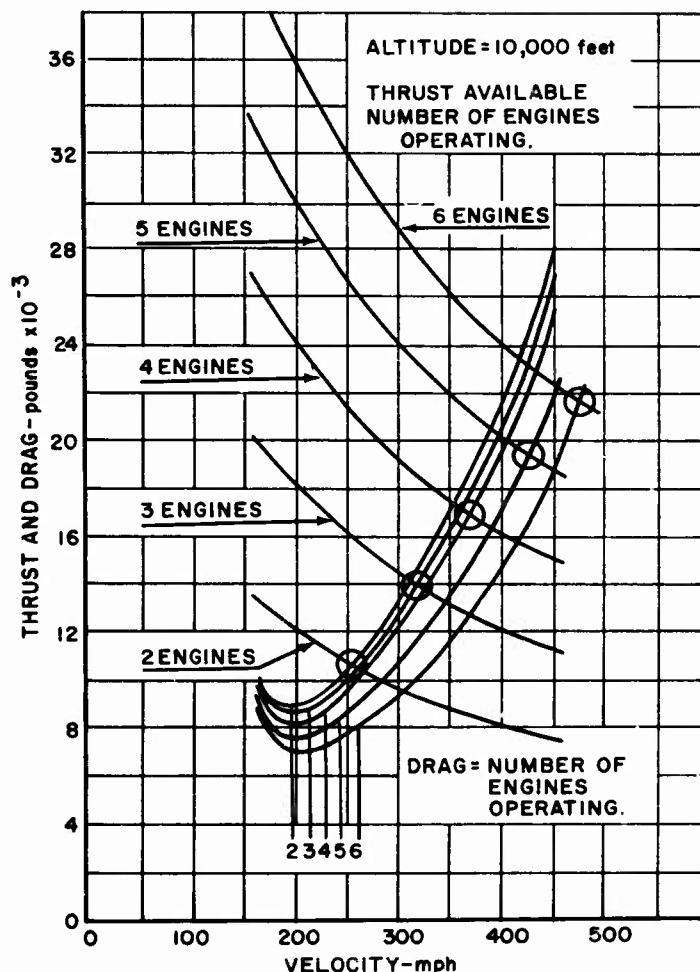
Figure 35. Emergency Operation under Reduced Power
