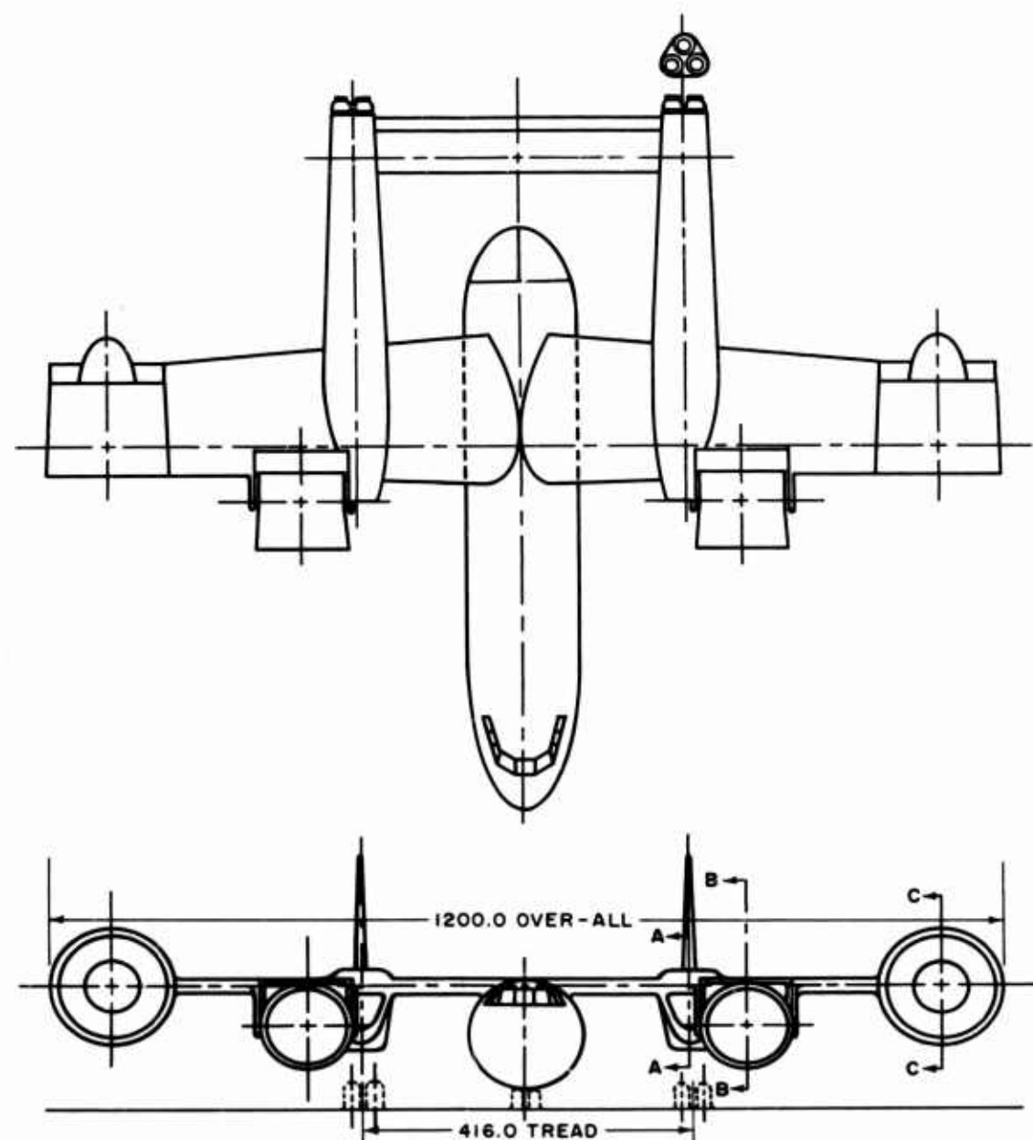
Figure 27. Ducted Propeller Twin-Boom Medium Cargo Transport
