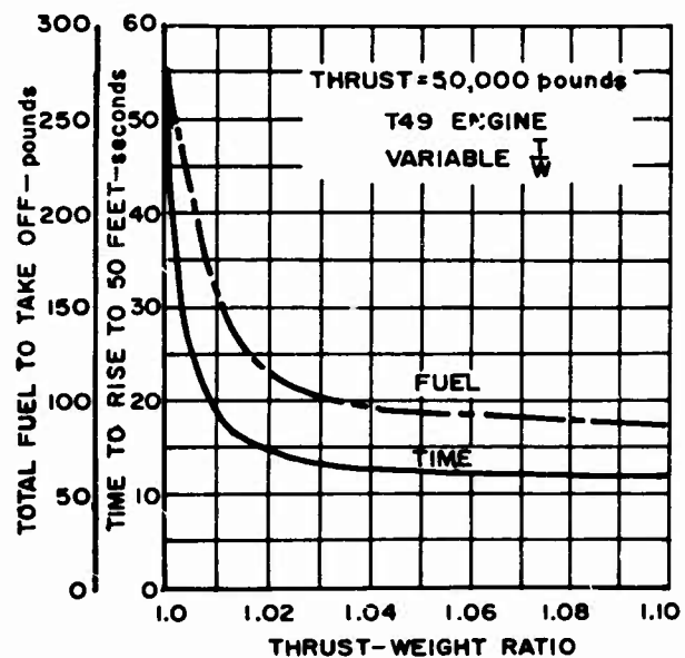
Figure 47. Vertical Take-Off Performance
