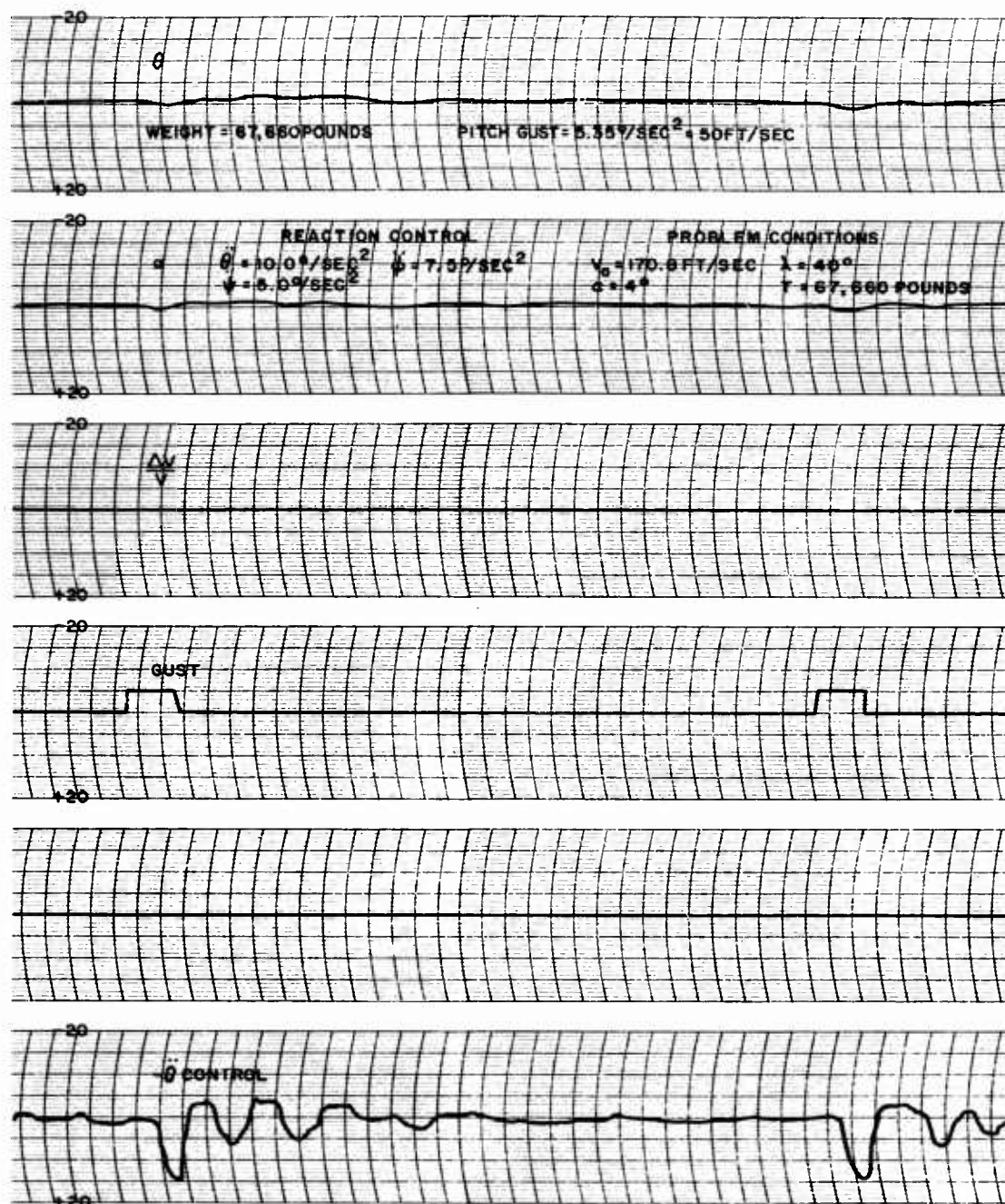
Figure 56b. Transition Longitudinal Traces
