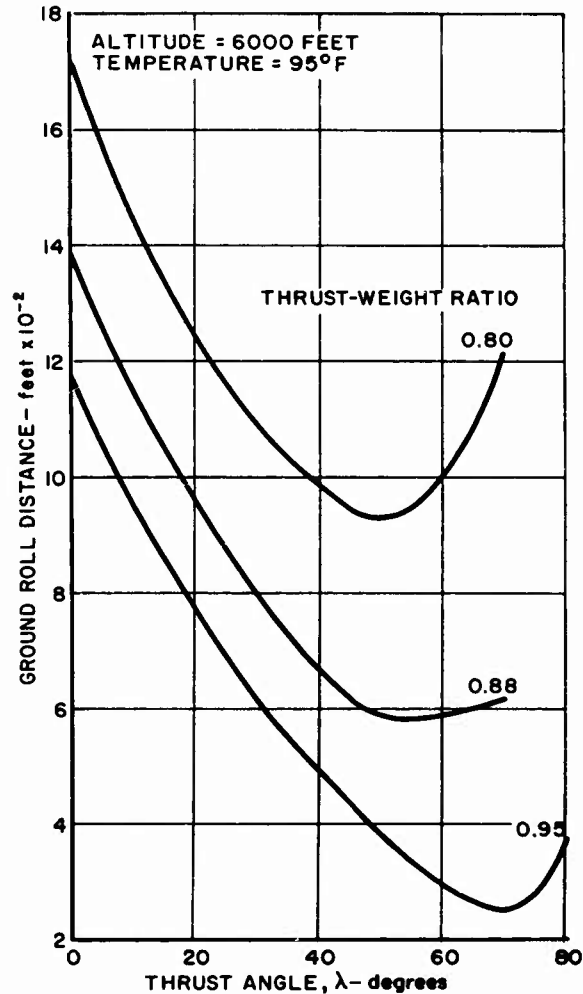
Figure 41. Short Take-Off Ground Roll vs Thrust Angle
