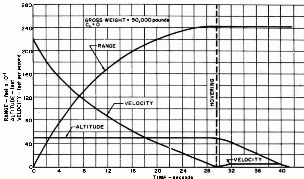
Figure 39. Landing Performance
