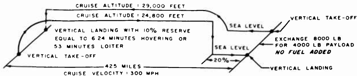
Figure 24. Basic Mission Profile
