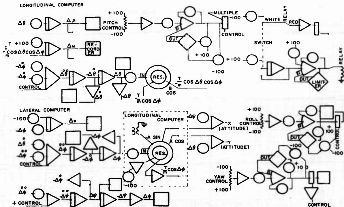
Figure 19. REAC Hovering Schematic Diagram
