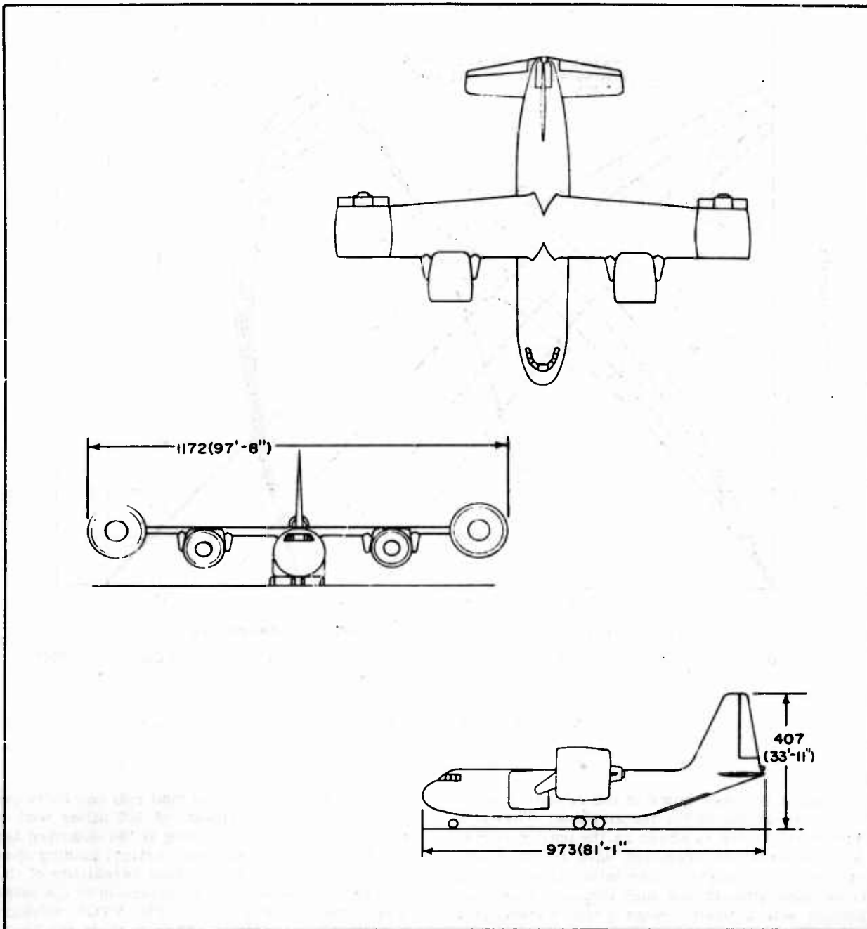
Figure 1. Assault Transport Basic Configuration
