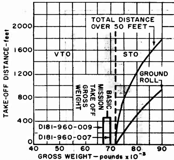
Figure 4 Take-Off Distance
