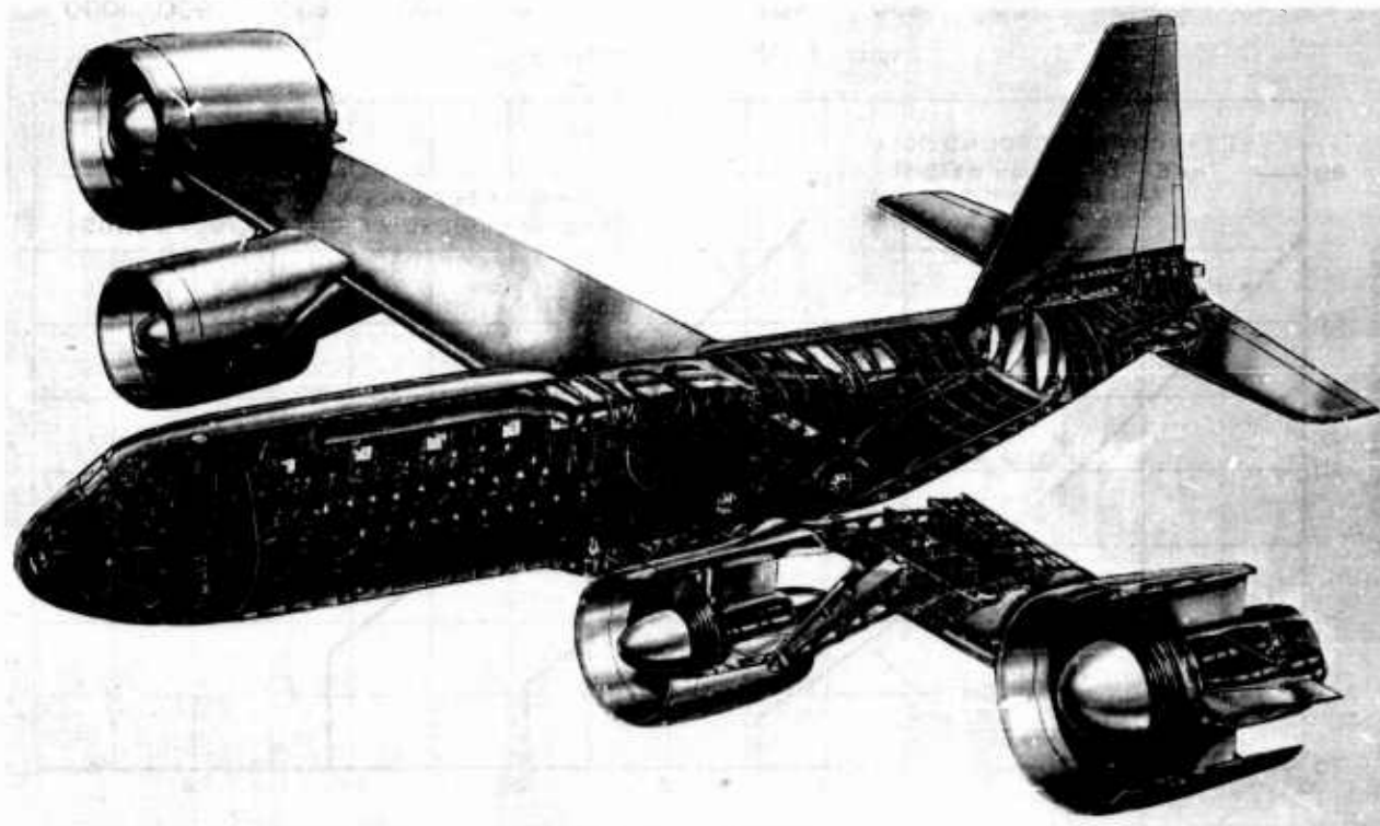
Figure 8. Cutaway of Assault Transport
