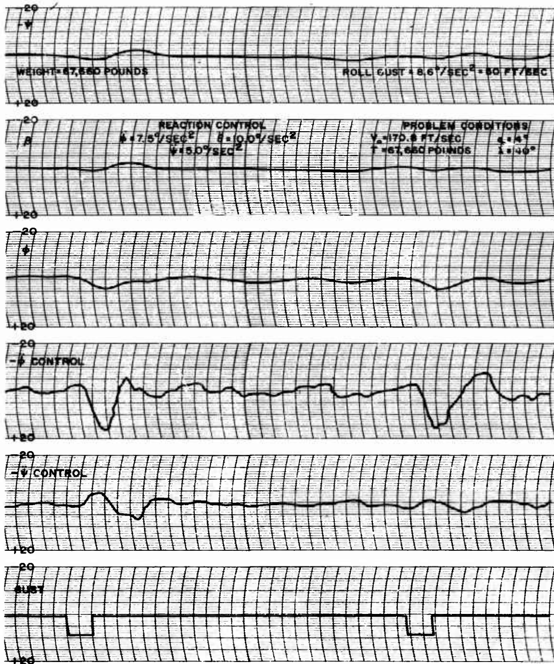
Figure 55a. Transition Lateral Traces
