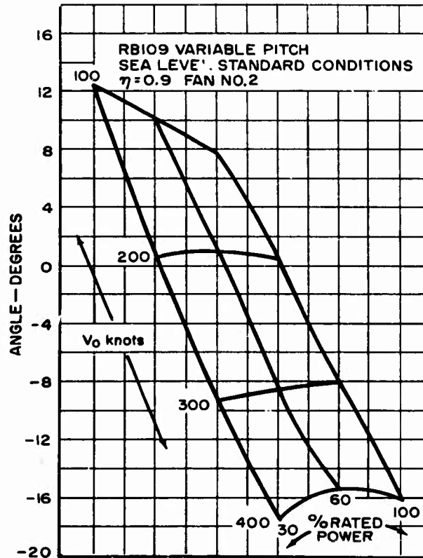
Figure 70. Pitch Change Required at Various Power Settings
