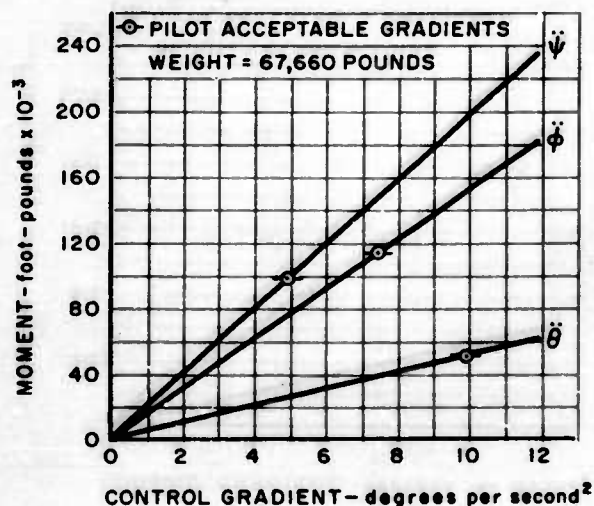
Figure 21. Reaction Control Moments Required in Hovering for Various Gradients
