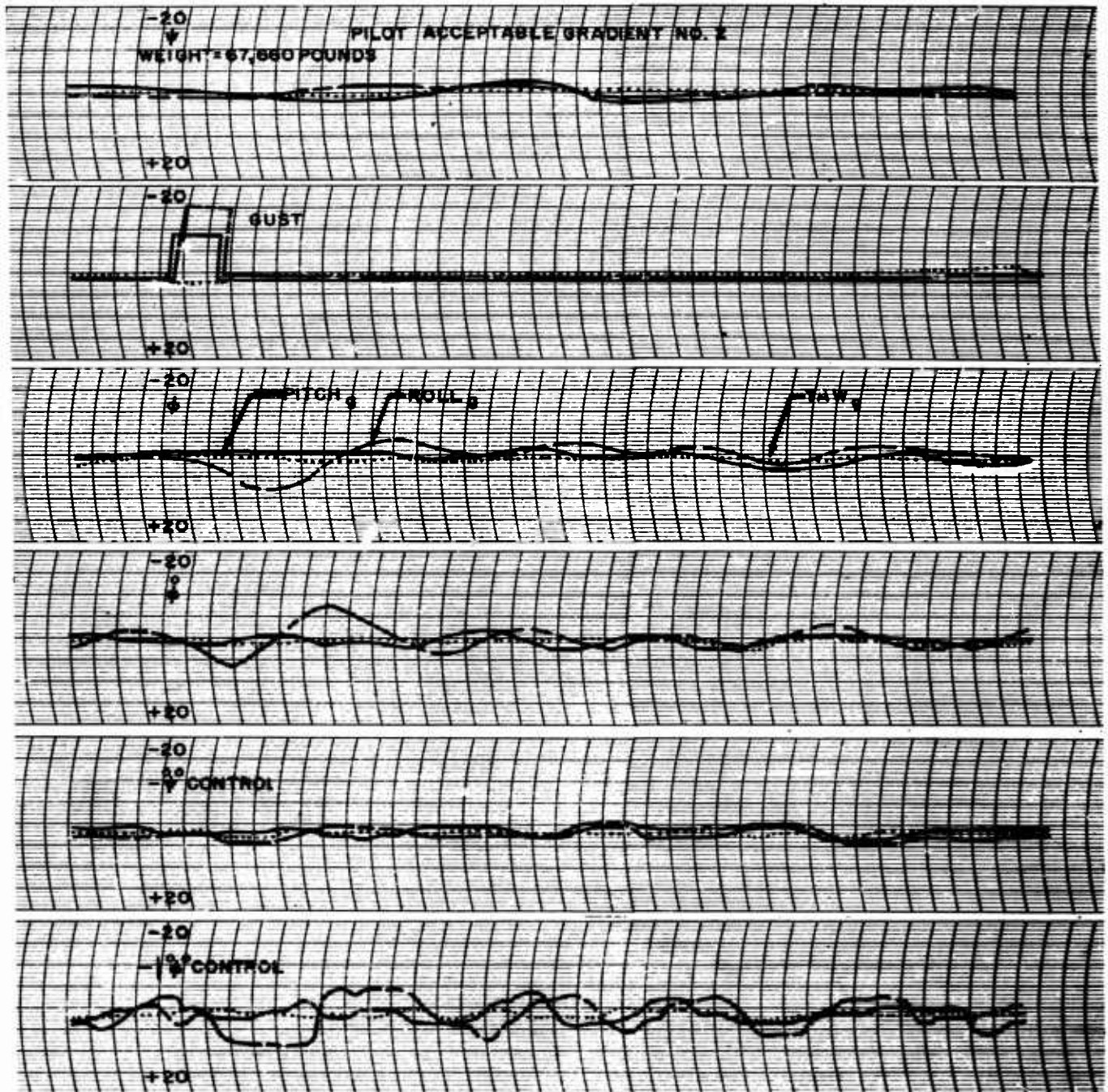
Figure 50a. Effect of Roll, Pitch, and Yaw Gusts at 50 feet per Second in Hovering. Lateral Dynamics
