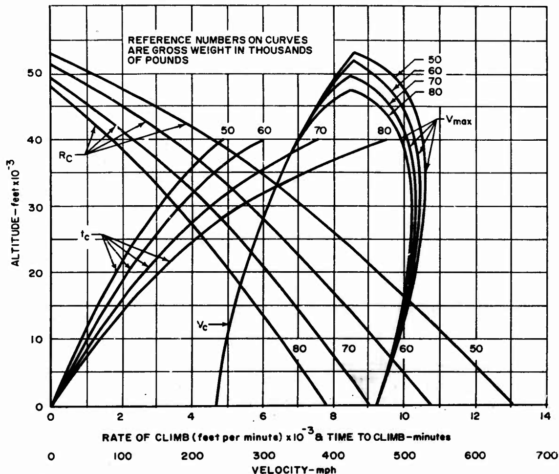
Figure 2. Classical Performance
