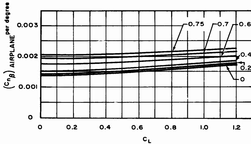
Figure 59. Airplane Directional Stability
