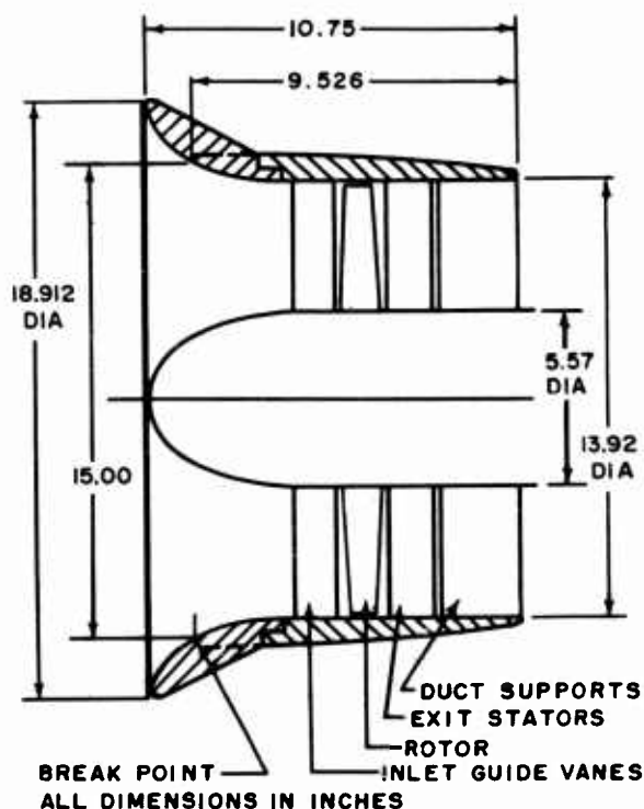
Figure 77. Wind Tunnel Model No. 1. Fixed Rotor Blade and Stators with Adjustable Inlet Guide Vanes
