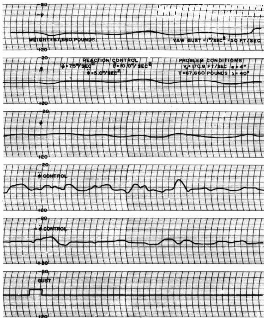
Figure 57a. Transition Lateral Traces
