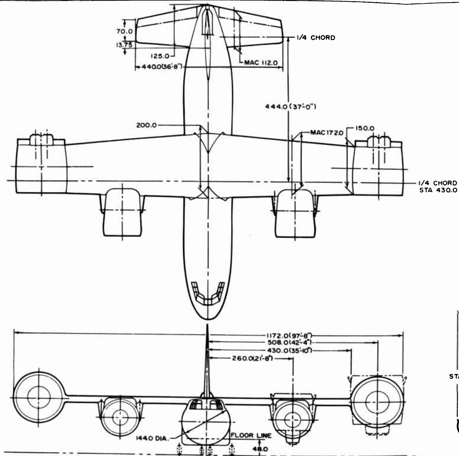
Figure 29. Assault Transport Configuration
