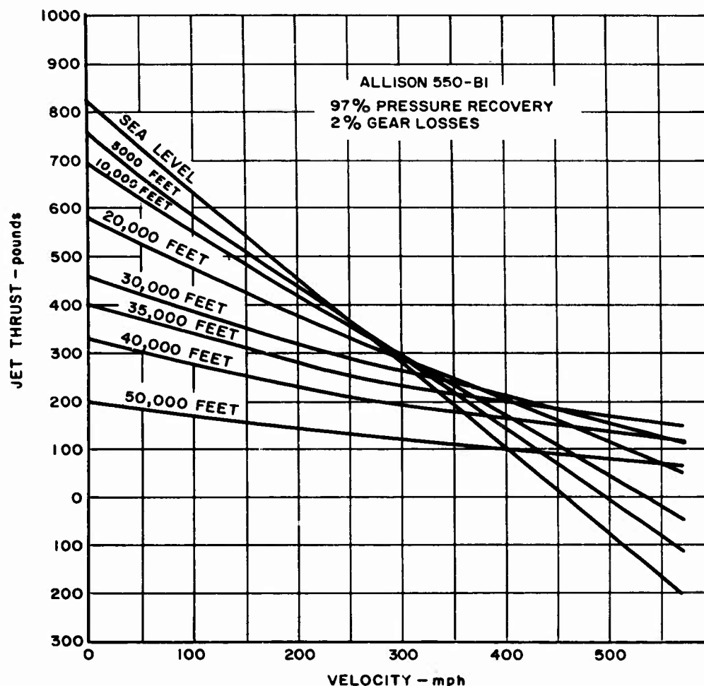
Figure 33. Residual Thrust
