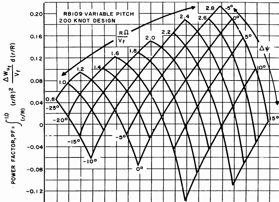
Figure 69. General Fan Performance Pitch Angle Variation
