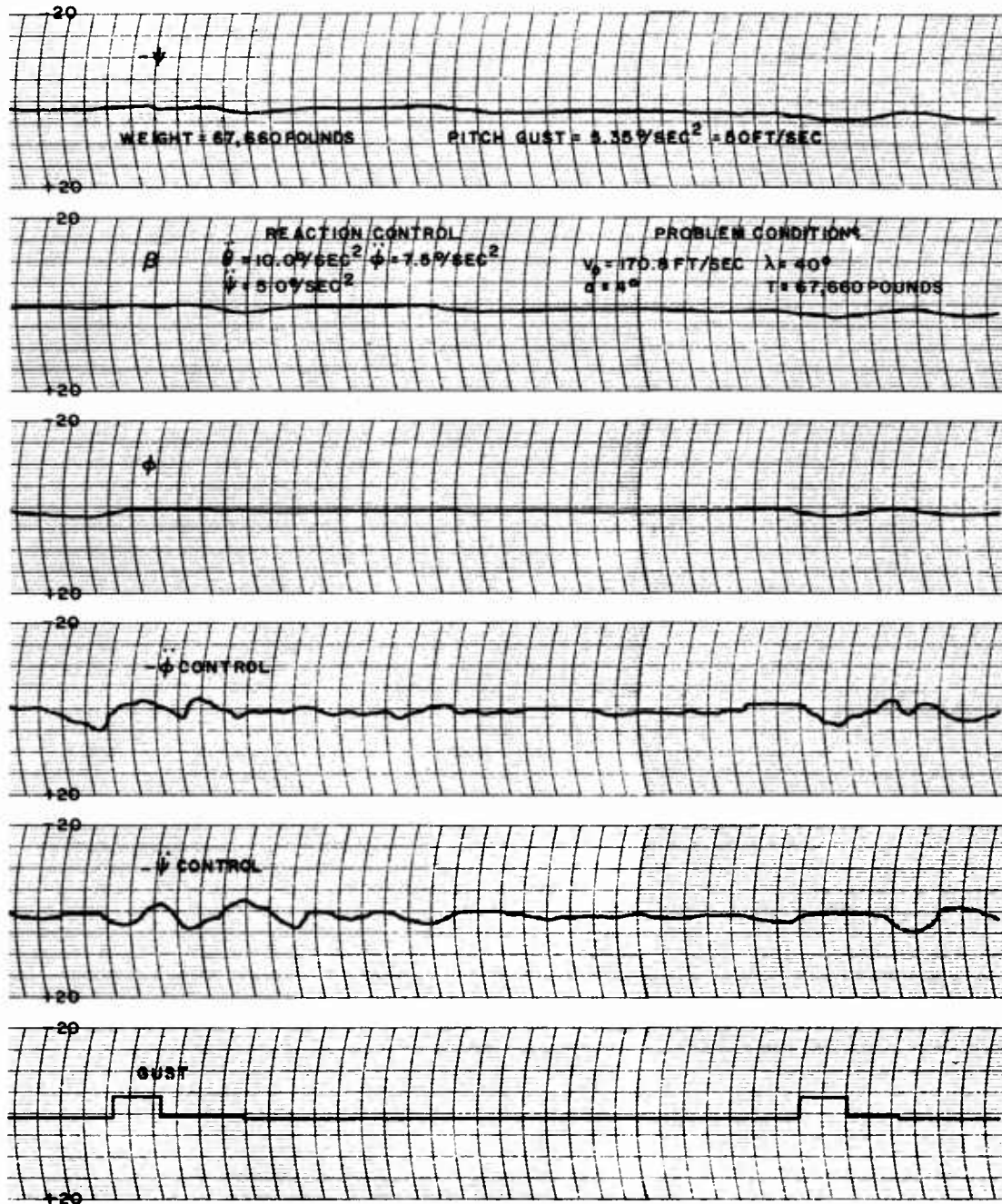
Figure 56a. Transition Lateral Traces
