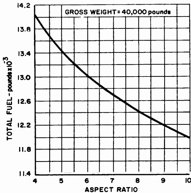
Figure 44. Total Fuel Required to Complete Basic Mission
