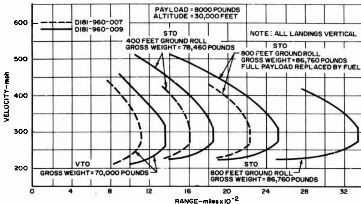
Figure 43. Ferry Range vs Speed
