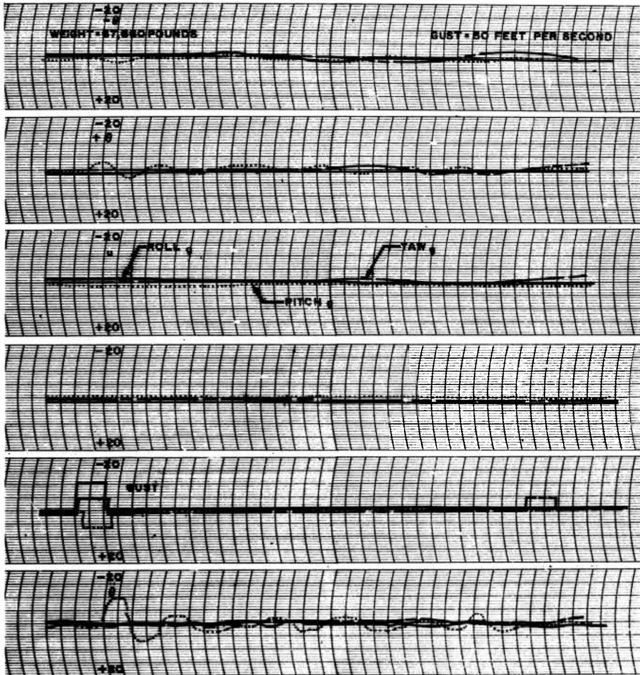
Figure 51b. Effect of Roll, Pitch, and Yaw Gusts in Hovering. Longitudinal Dynamics
