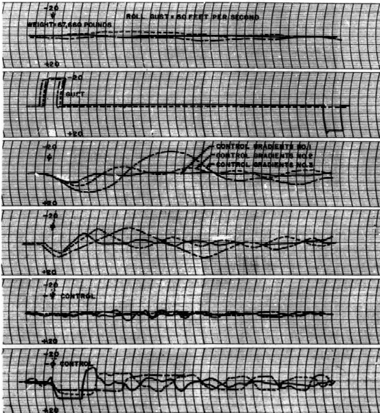
Figure 18a. Effect of Control Gradients in Hovering. Lateral Dynamics
