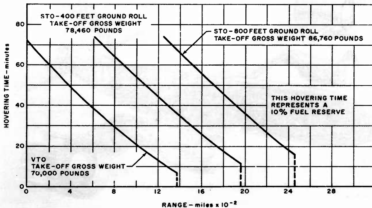
Figure 7. Range and Hovering Time
