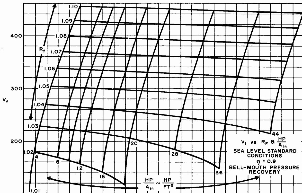
Figure 64. Static Momentum Data
