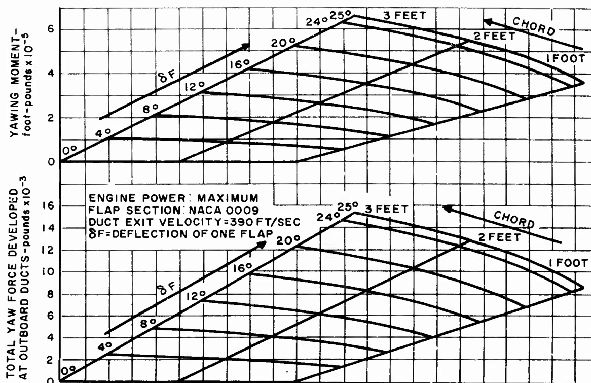
Figure 52. Yaw Reaction Control Forces and Moments Developed by Flaps at Exit of Outboard Ducts
