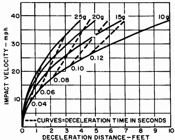
Figure 75. Deceleration Time
