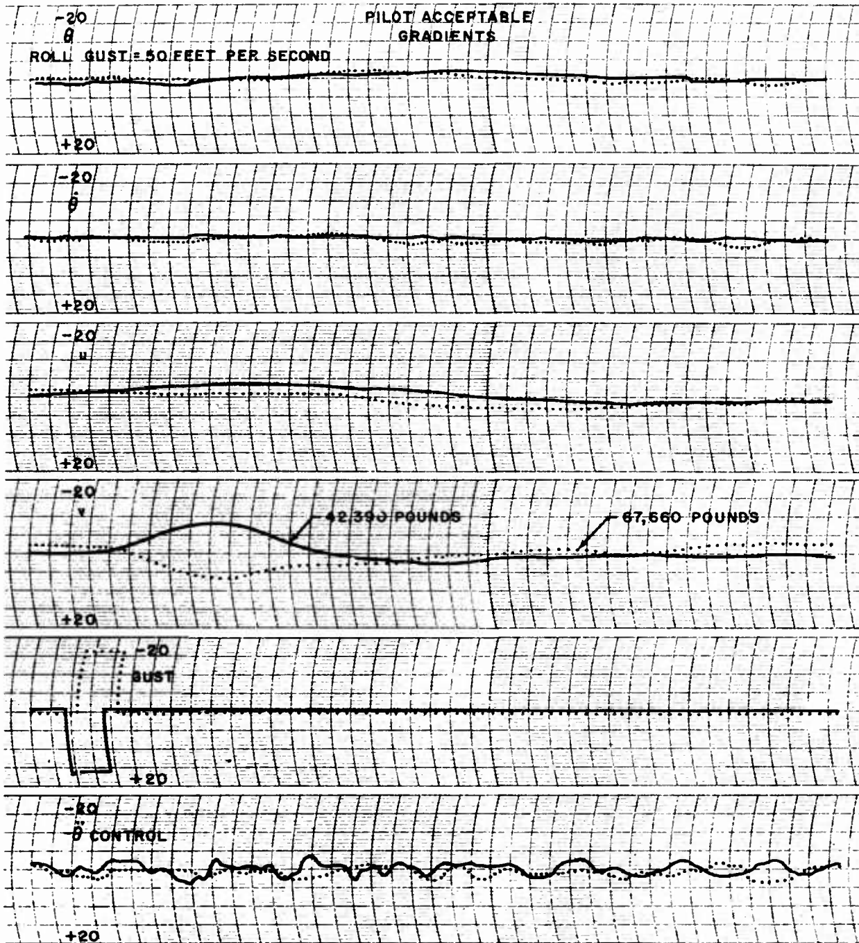
Figure 49b. Effect of Landing and Take-Off Weight in Hovering. Longitudinal Dynamics
