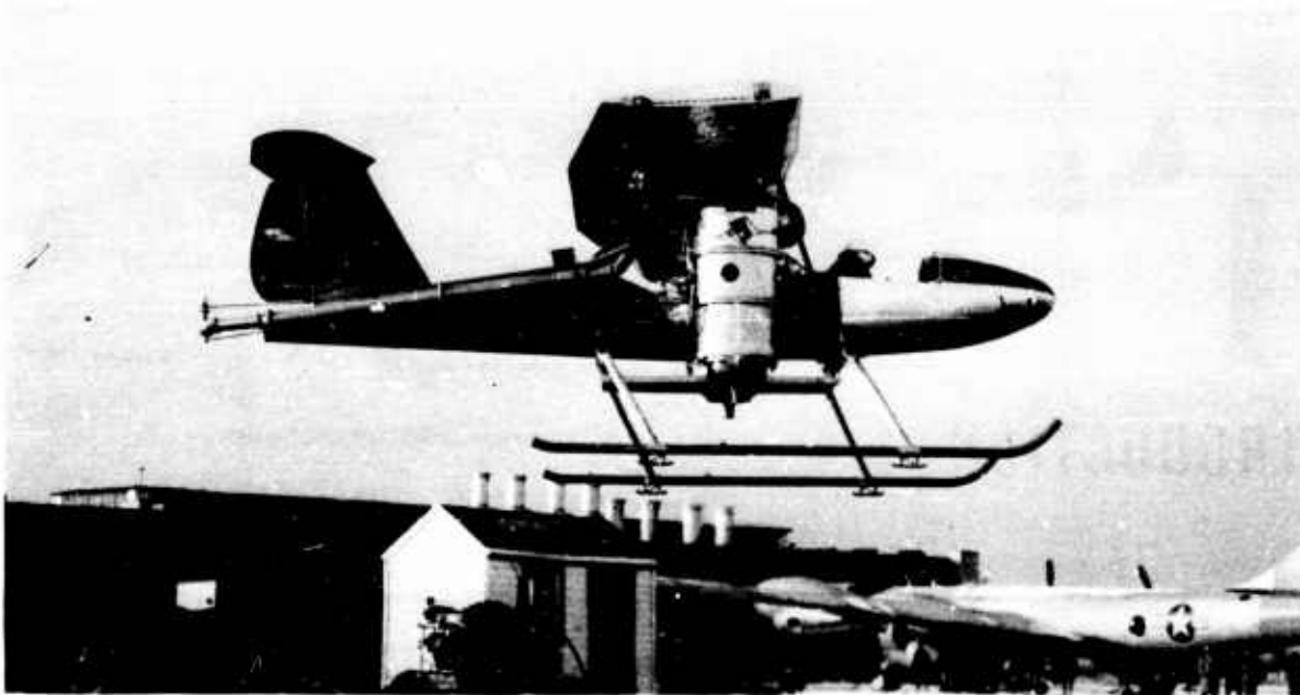
Figure 22. Bell Aircraft Air Test Vehicle
