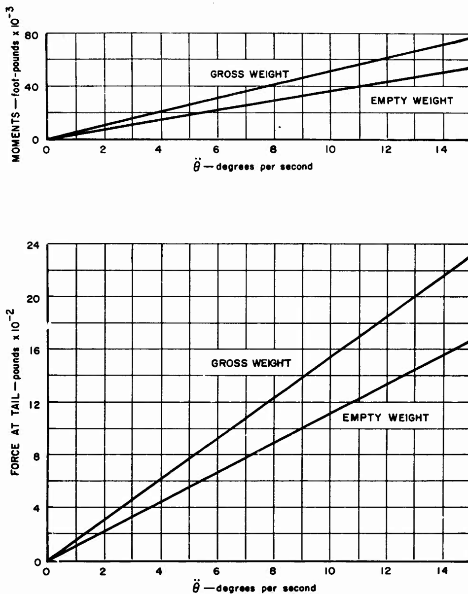
Figure 54. Pitch Reaction Control Forces and Moments Required for Various Pitch Gradients
