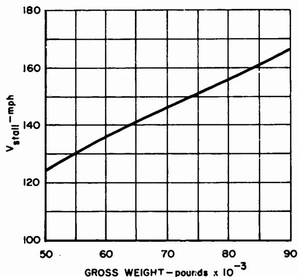
Figure 36. Power-Off Stall Speed
