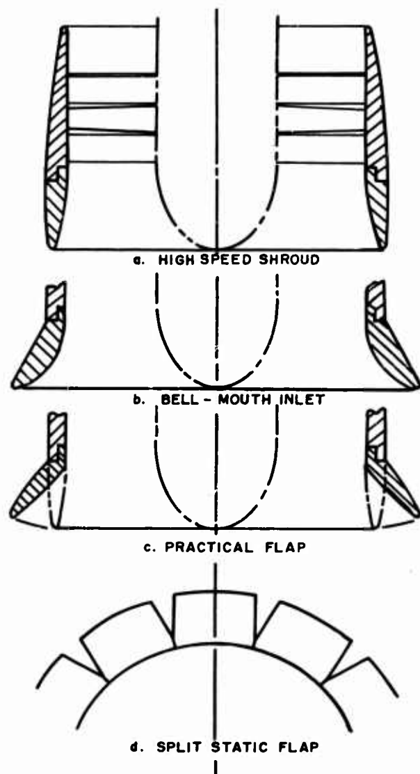
Figure 79. Wind Tunnel Model Duct Inlet Variations
