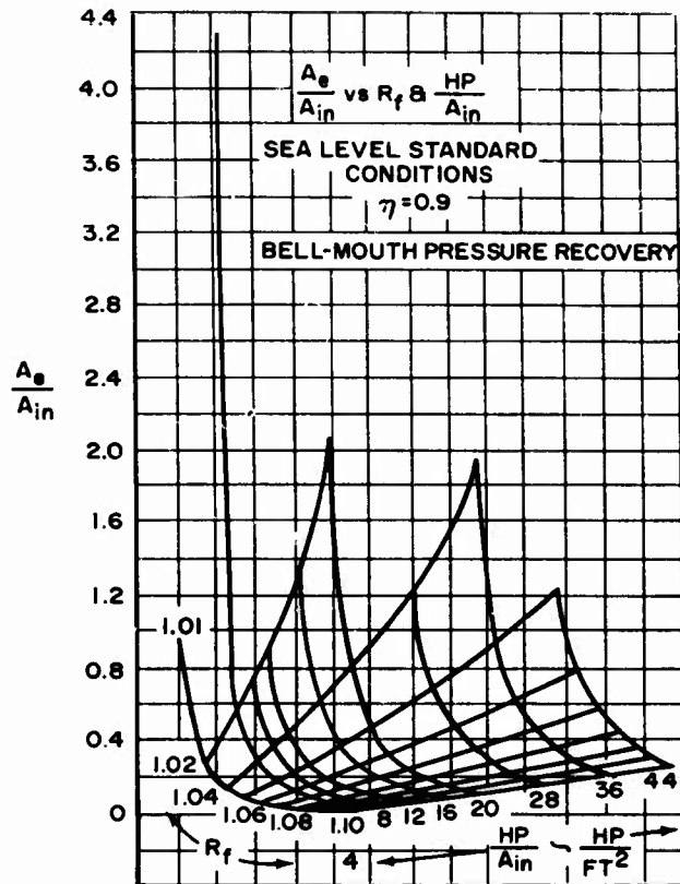
Figure 63. Static Momentum Data
