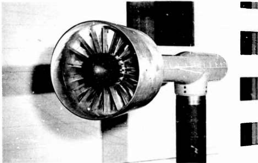
Figure 14. Assembled Model in Tunnel (University of Wichita)
