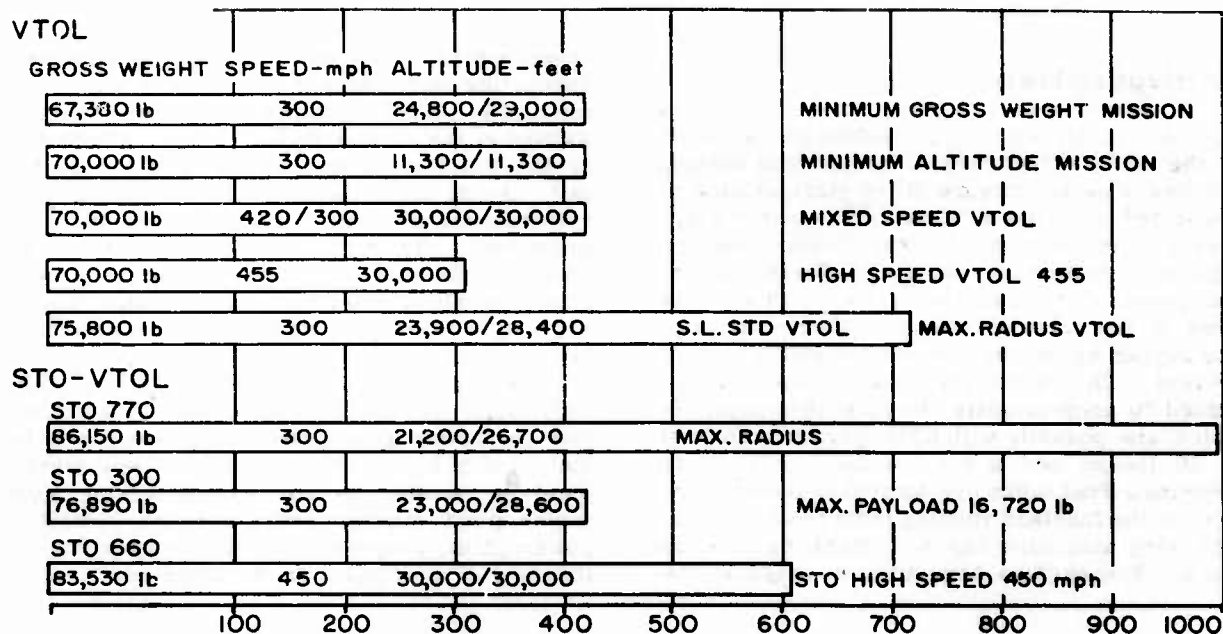
Figure 6. Mission Variations
