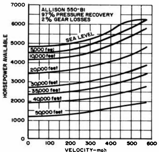
Figure 32. Power Available
