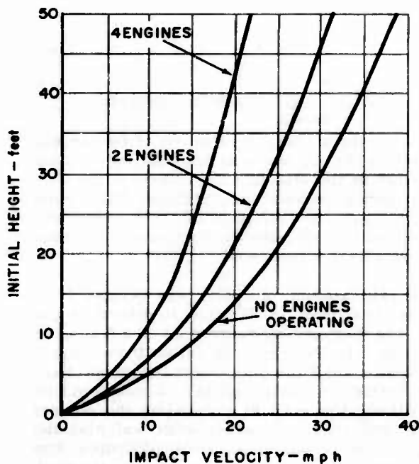
Figure 15. Engine Failure During Hovering
