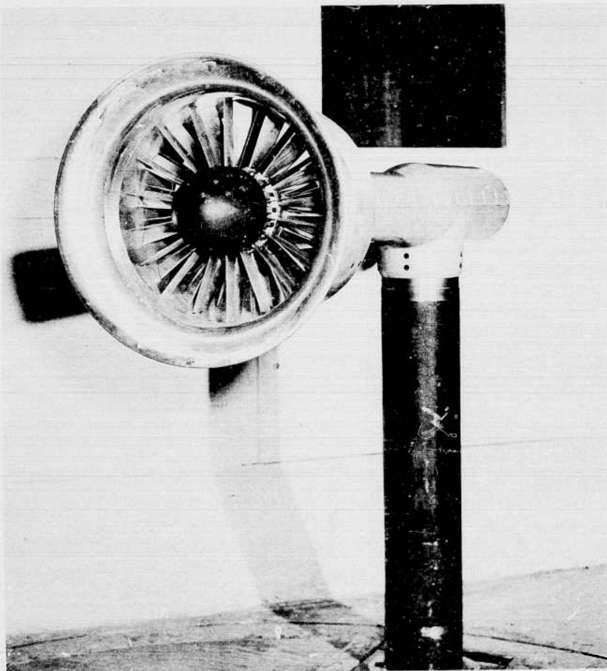
Figure 9b. Wind Tunnel Duct Model
