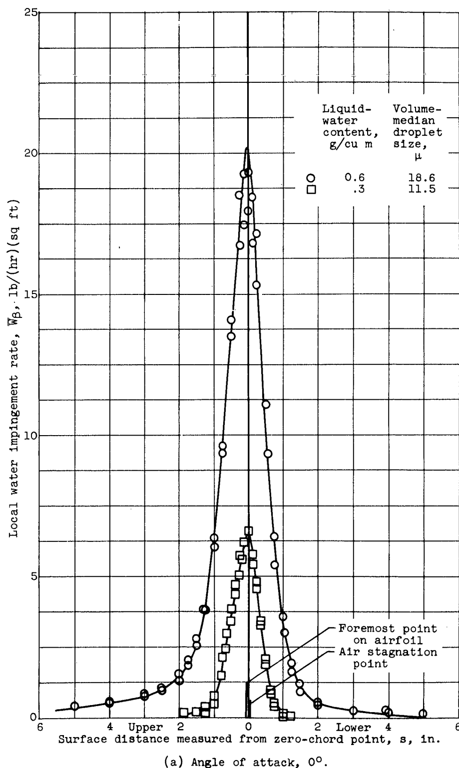
Figure 7. - Local water impingement rate on surface of full-chord NACA 65 1 -212 airfoil. Airspeed, 156 knots.
