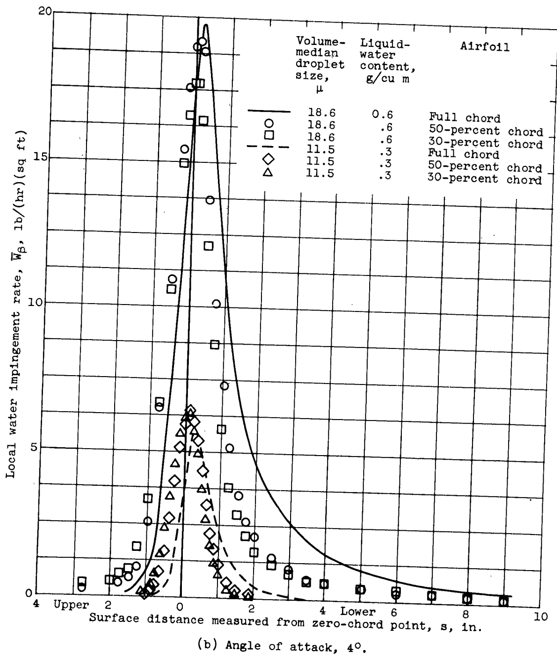
Figure 9. - Concluded. Comparison of local water impingement rate on surfaces of 30- and 50-percent truncated NACA 65 1 -212 airfoils with that for full-chord model. Flap undeflected; airspeed, 156 knots.
