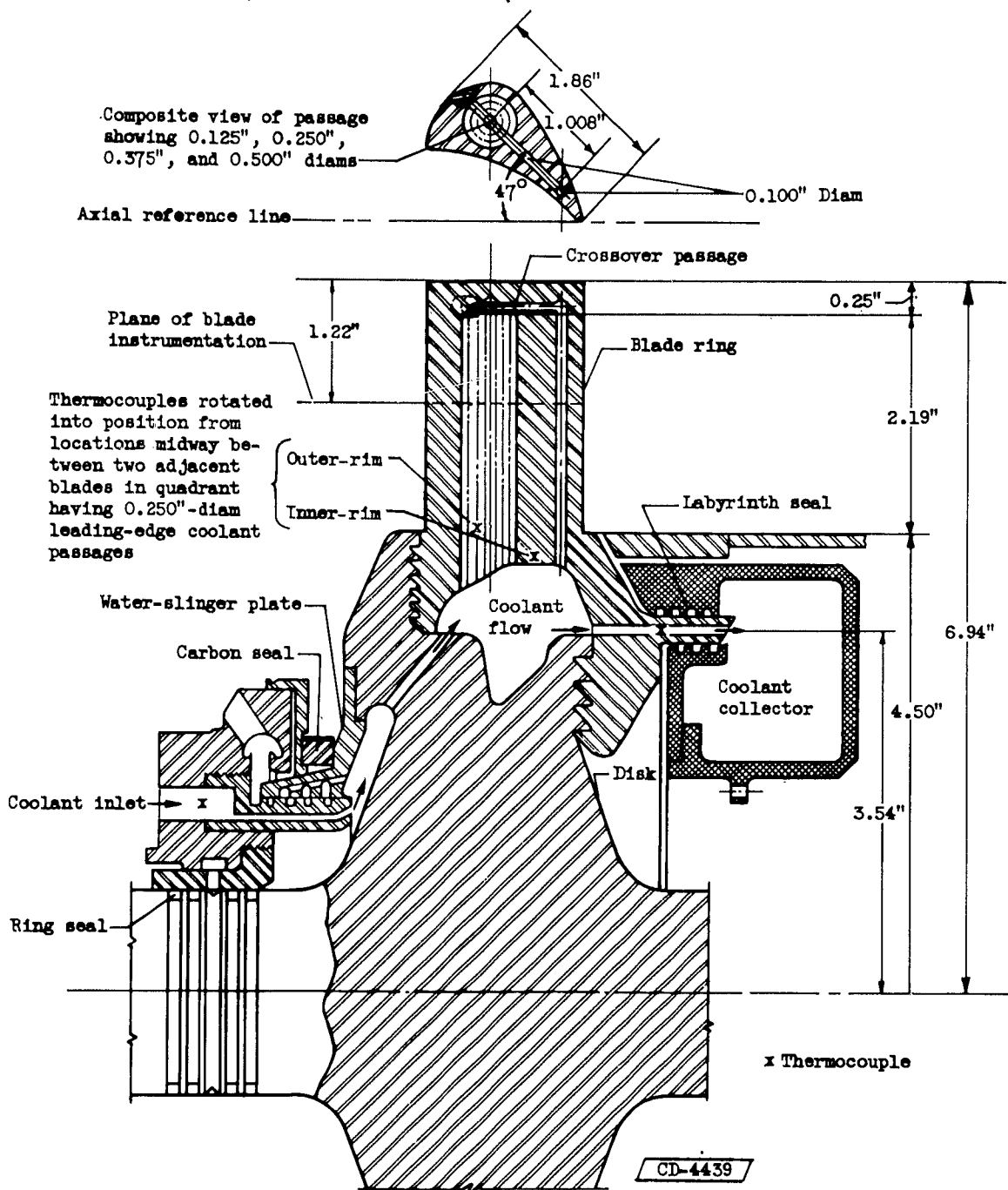
Figure 1. - Cross section of rotor and rotor-coolant system of loop-circuit liquid-cooled stainless-steel turbine showing instrumentation locations.
