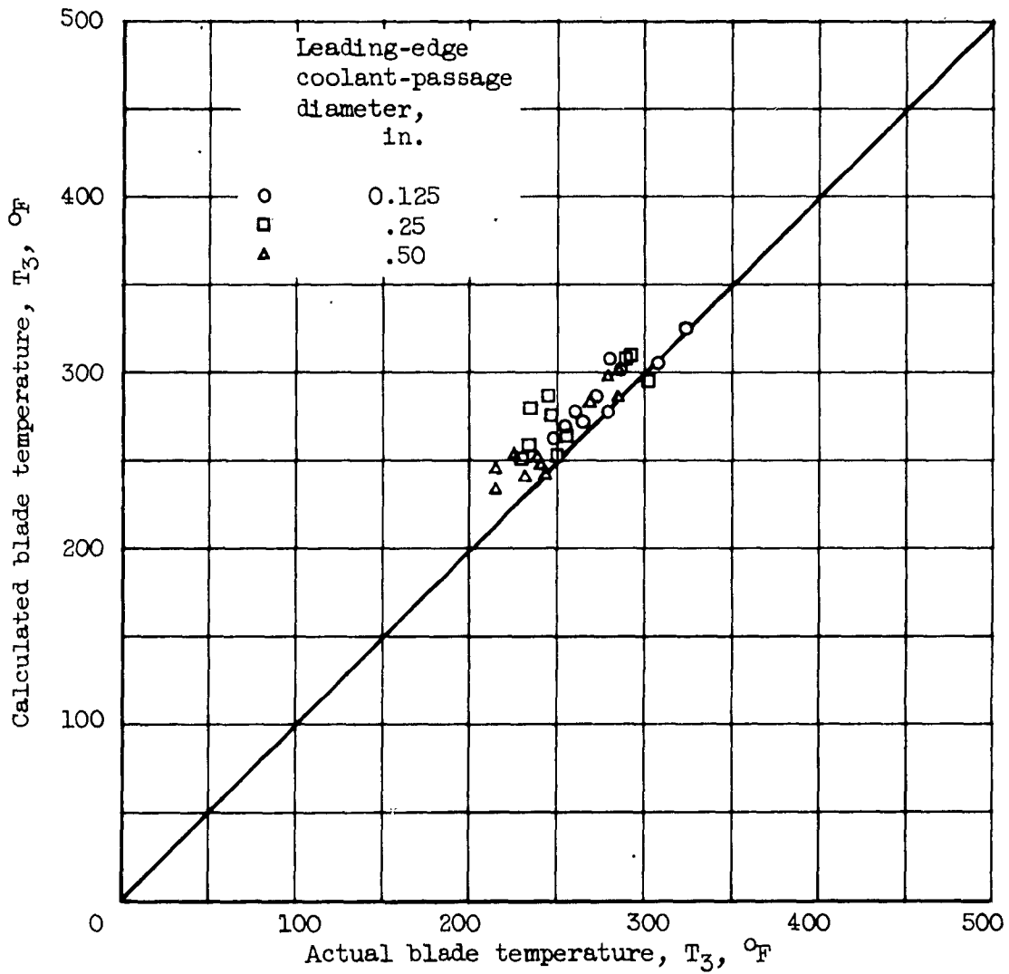
Figure 6. - Comparison of measured and calculated blade temperatures in trailing-edge portion of water-cooled blades.
