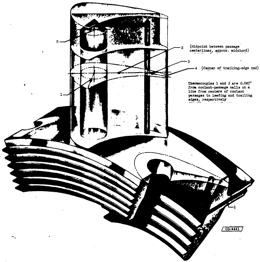
Figure 2. - Diagrammatic representation of rotor blade thermocouple locations on loop-circuit liquid-cooled stainless-steel turbine.
