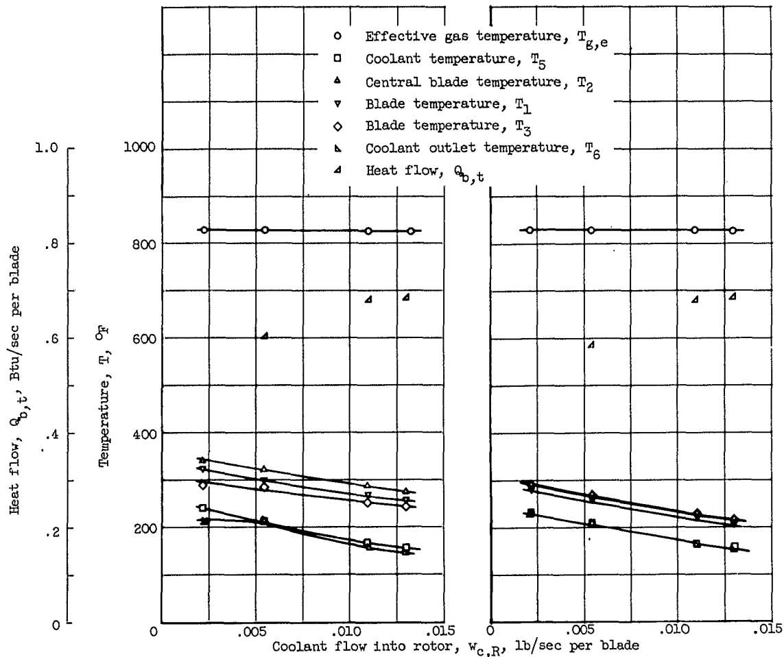
(a) Leading-edge coolant-passage diameter, 0.125 inch.
