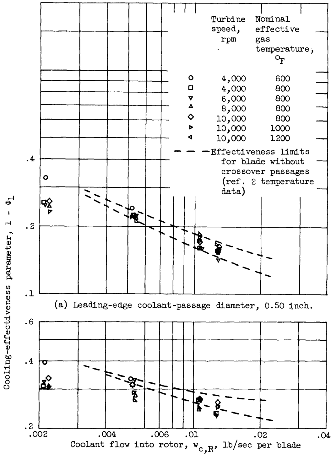
Figure 8. - Comparison of cooling effectiveness near leading edge for blades with and without crossover passages at blade tip.
