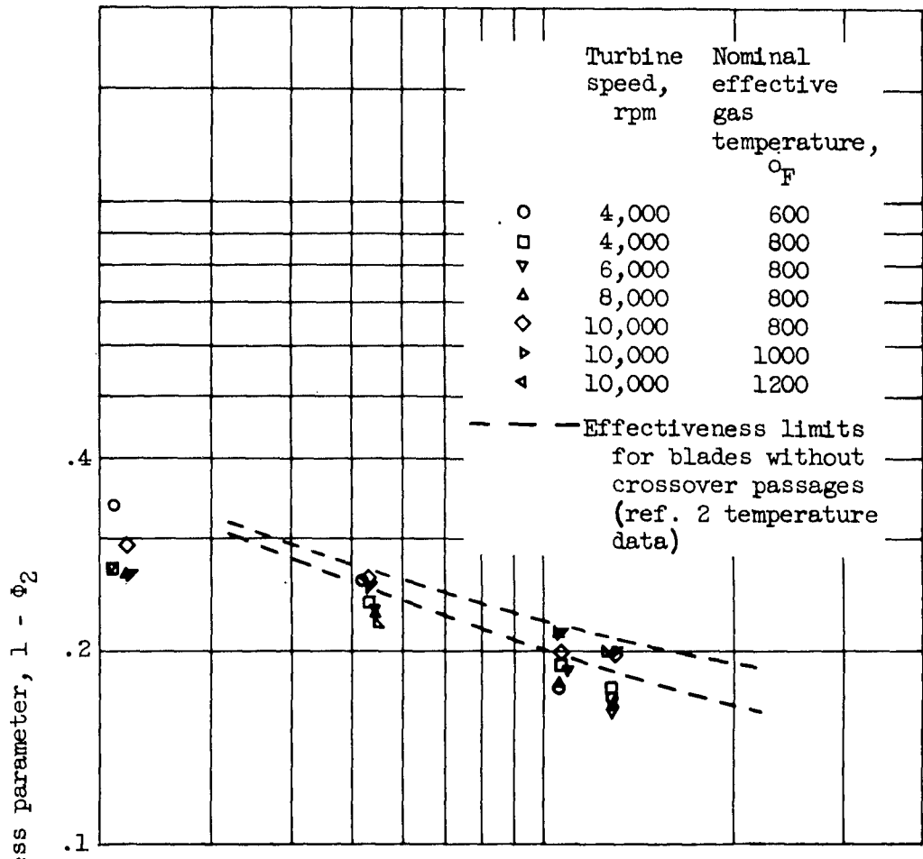
(a) Leading-edge coolant-passage diameter, 0.50 inch.
