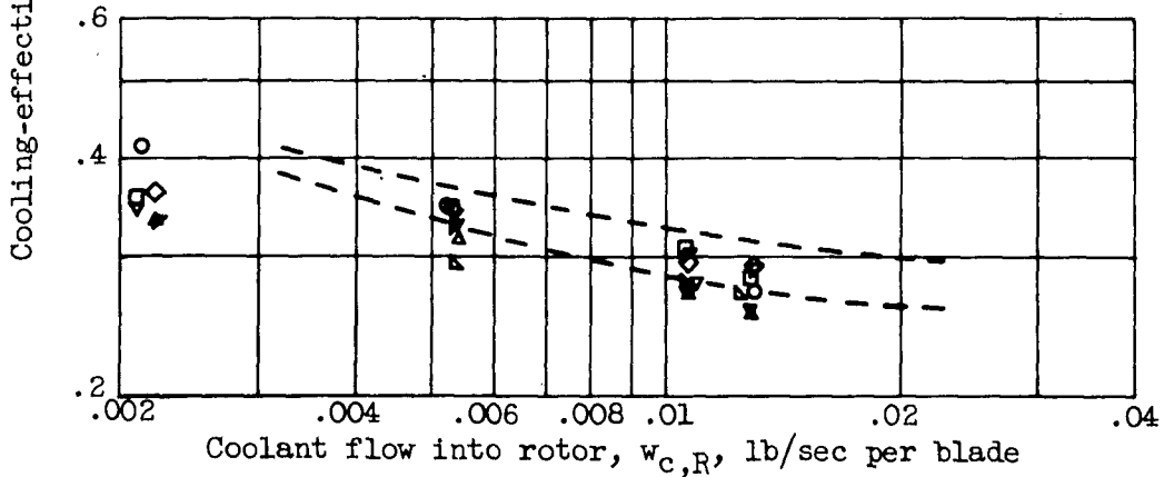
(b) Leading-edge coolant-passage diameter, 0.125 inch.
