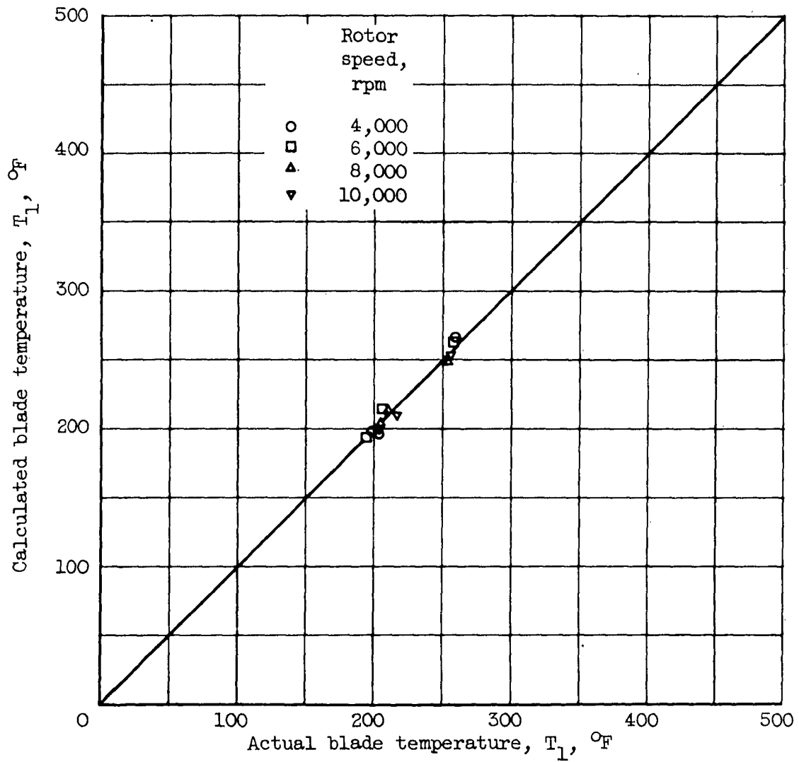
Figure 5. - Concluded. Comparison of measured and calculated blade temperatures in leading-edge portion of water-cooled blades.
