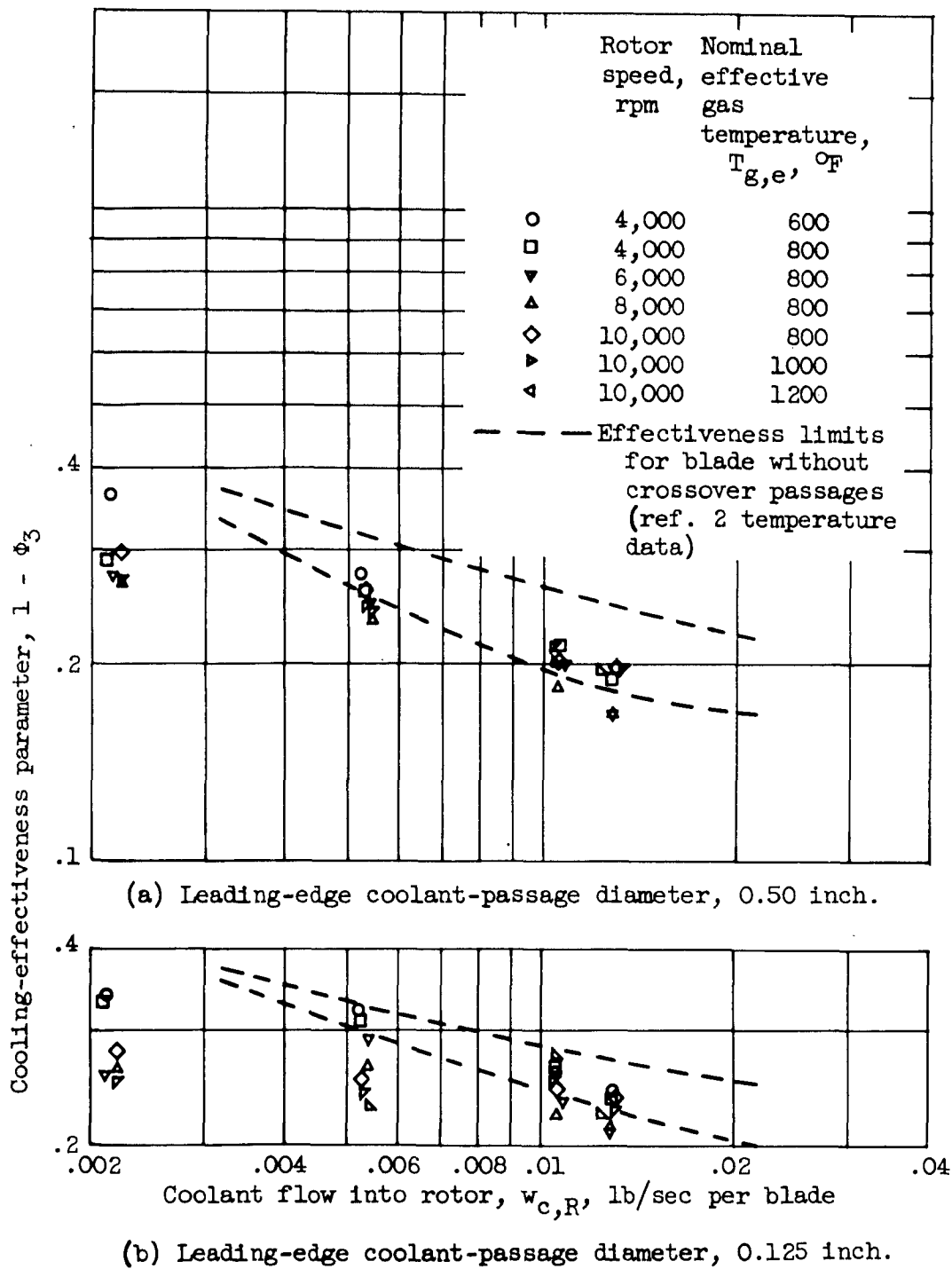
Figure 9. - Comparison of cooling effectiveness near trailing edge for blades with and without crossover passages at blade tip.
