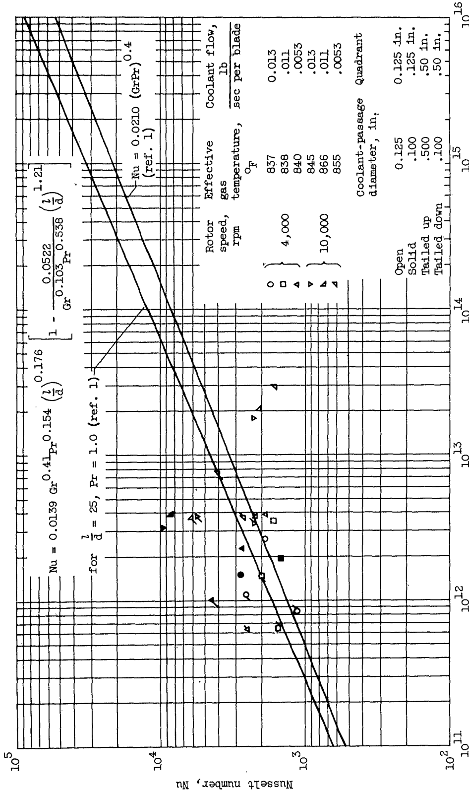
Figure 4. - Dimensionless heat-transfer correlation using calculated coolant-passage-surface temperature.
