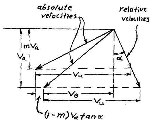
Fig. 20 Velocity Scheme
