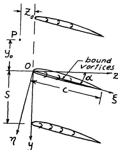
Fig. 16 Cascade Scheme
