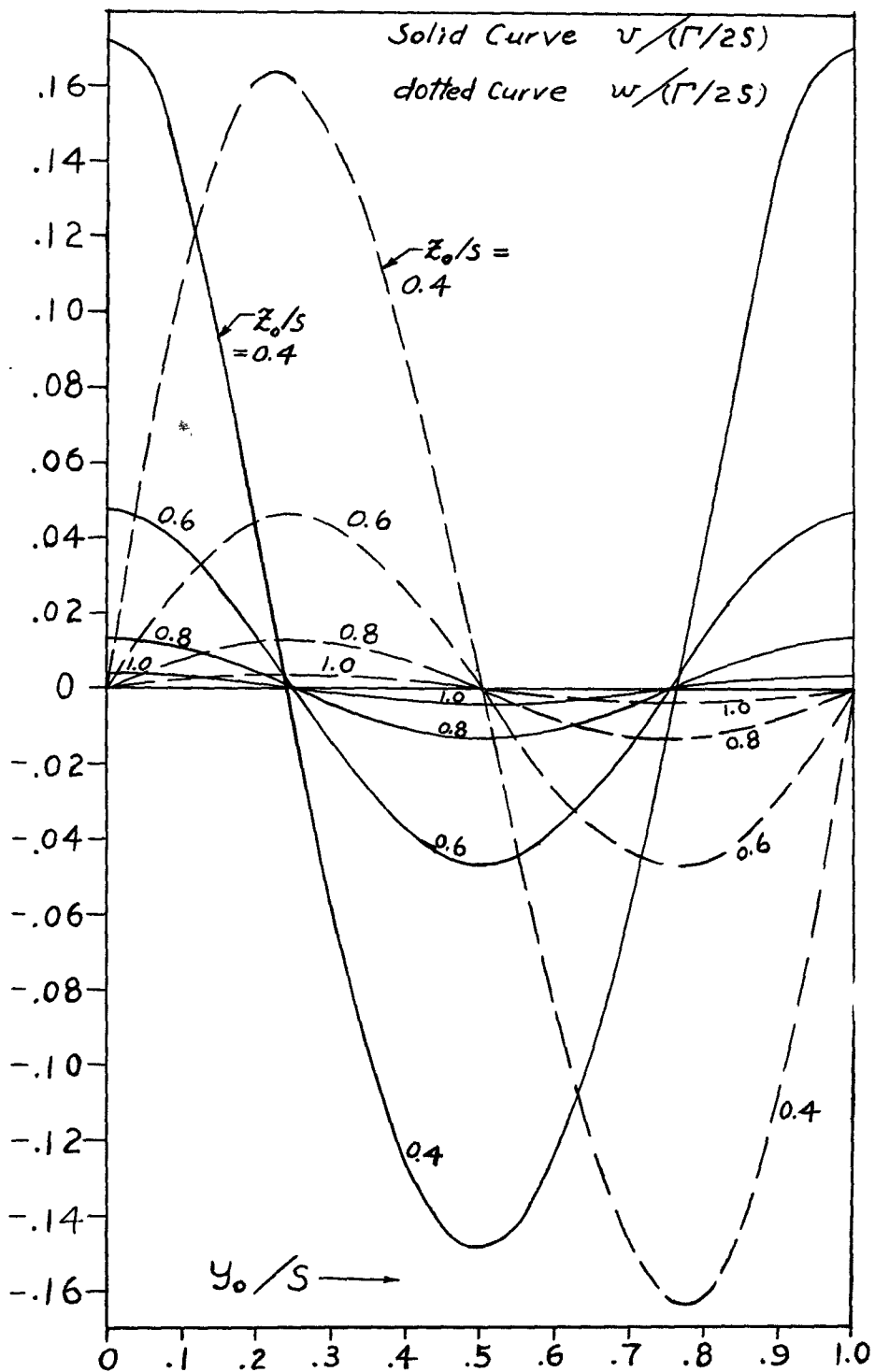
Fig.17. Induced Velocity due to Cascade of vortices
