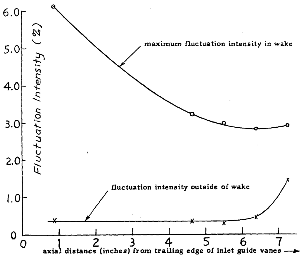
Fig. 13. FLUCTUATION INTENSITY BEHIND INLET GUIDE VANES
