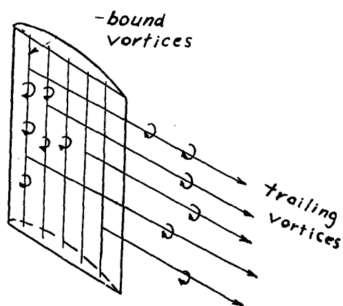
Fig. 15 Bound and Trailing Vortices
