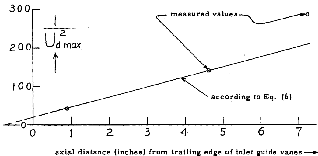
Fig. 12. DECAY OF WAKE BEHIND INLET GUIDE VANES
